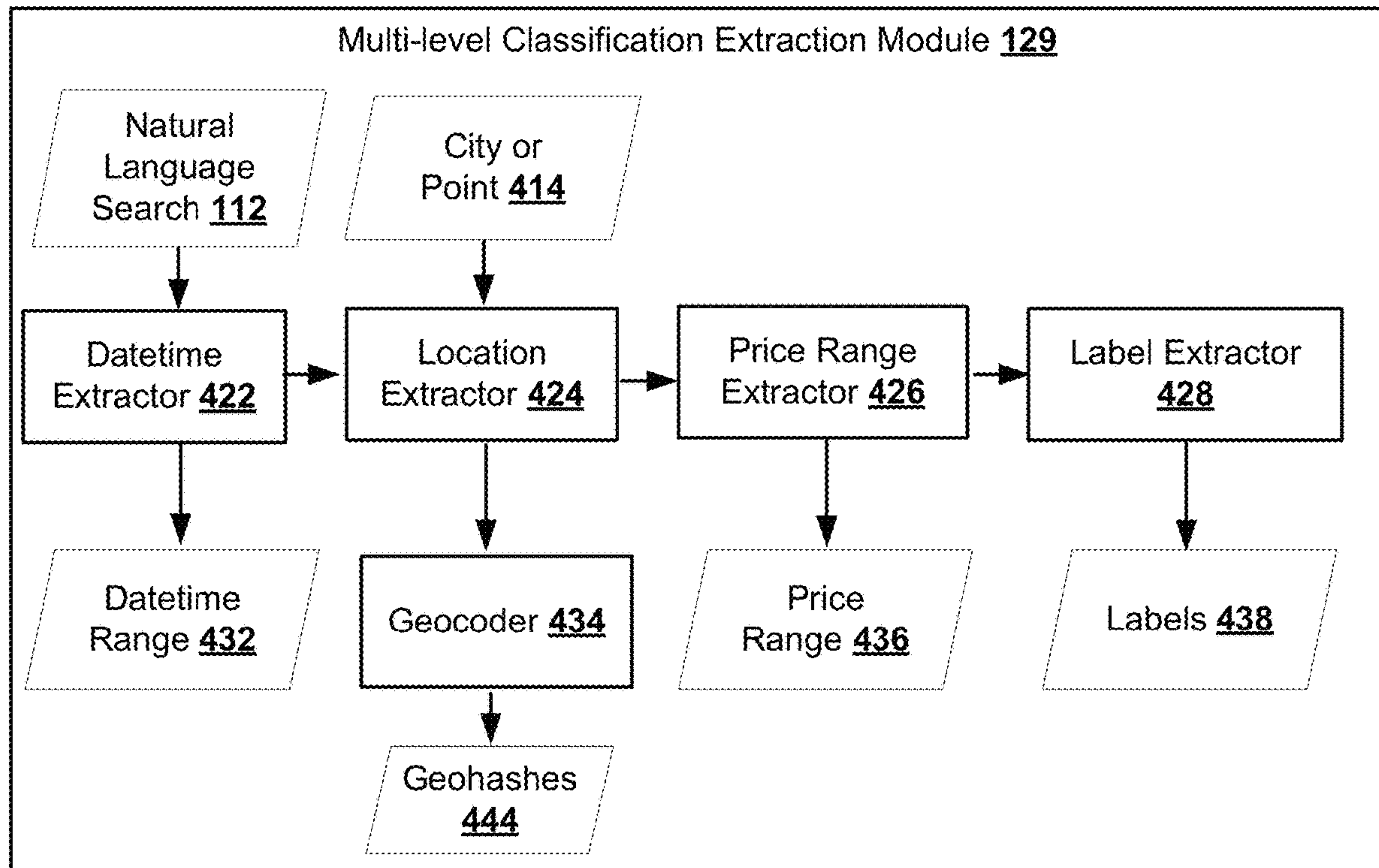
Fig. 4A Example for Local Search
