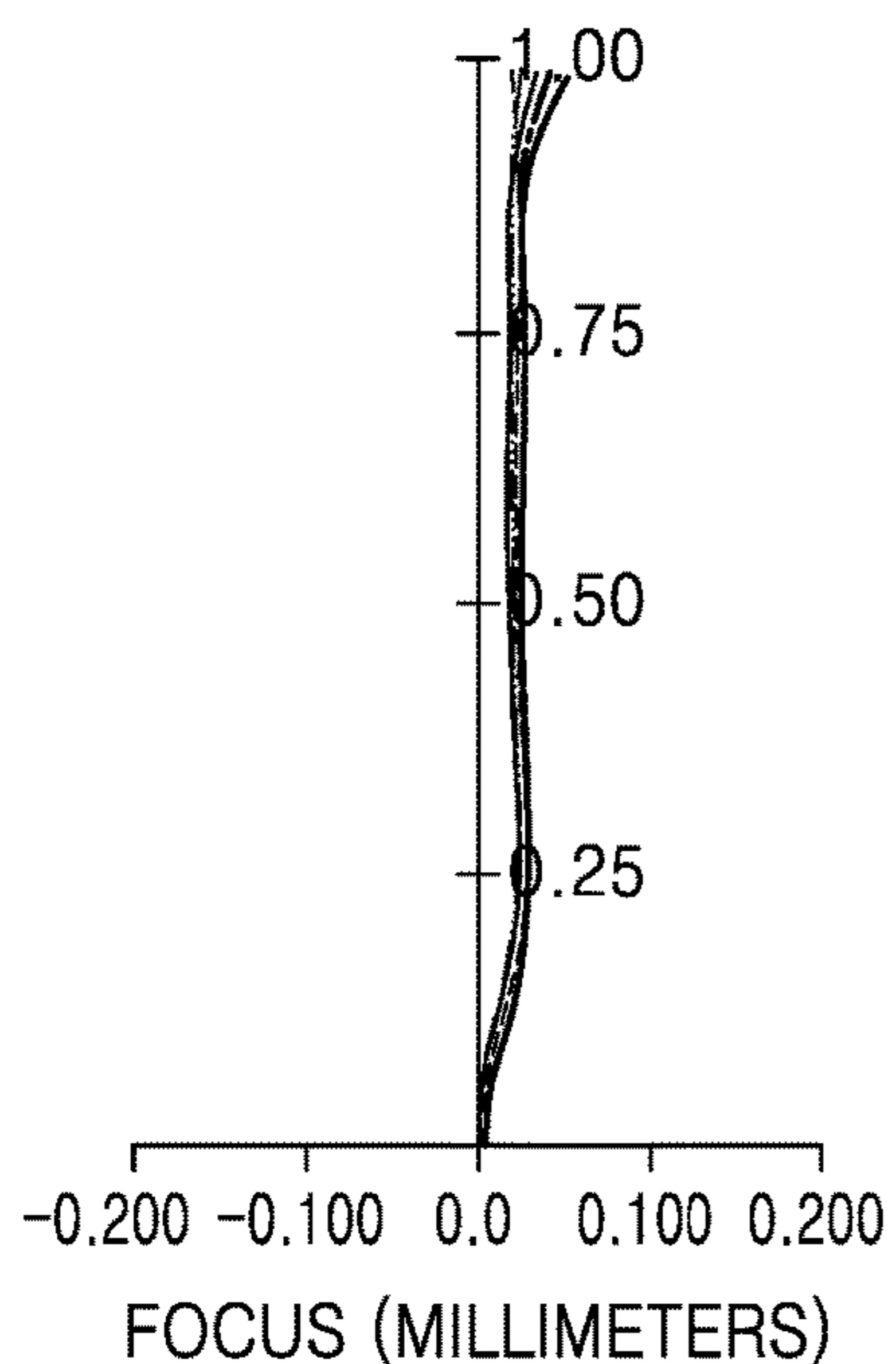
LONGITUDINAL SPHERICAL ABERRATION
