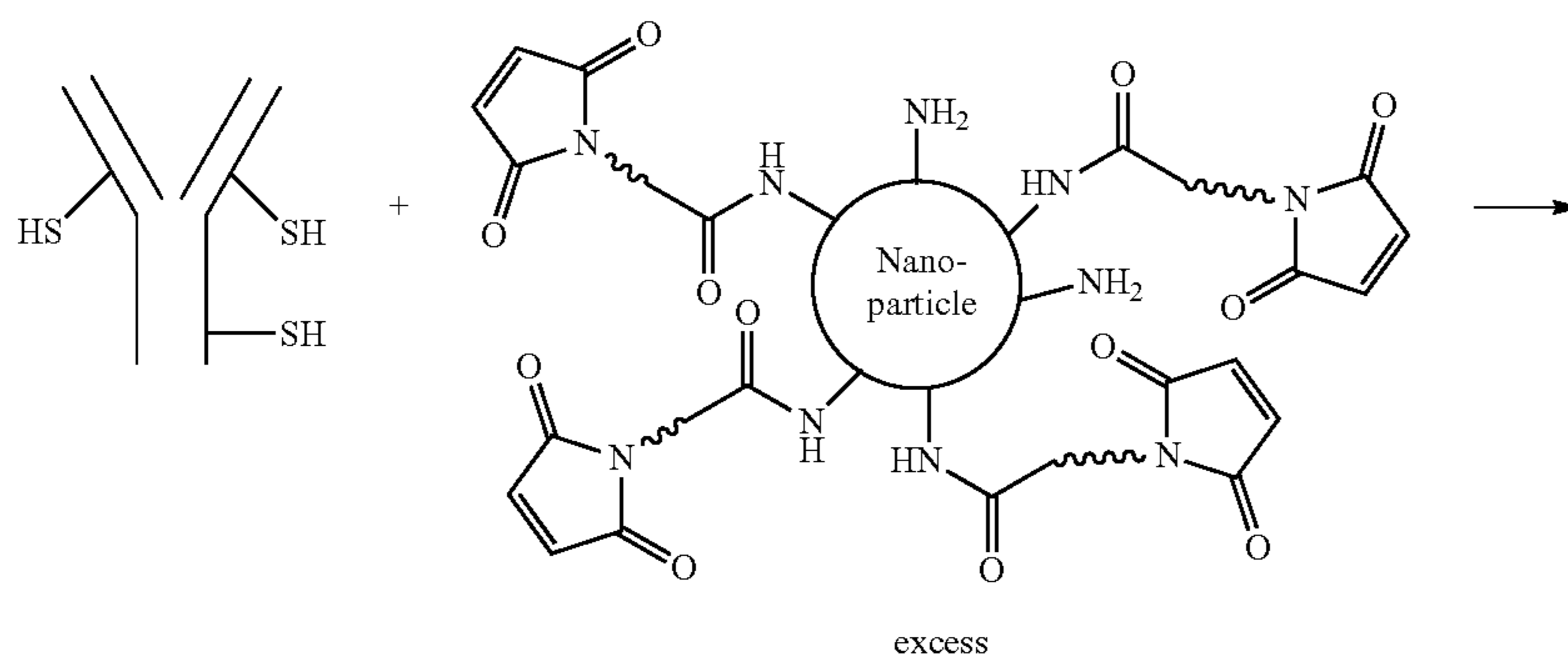
Scheme 21
