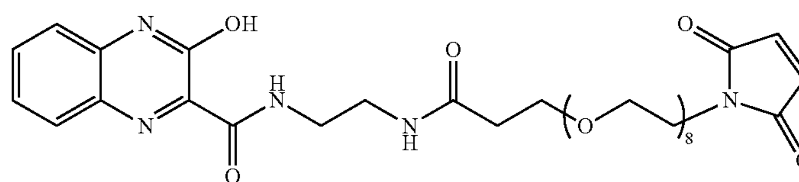
Scheme 14
