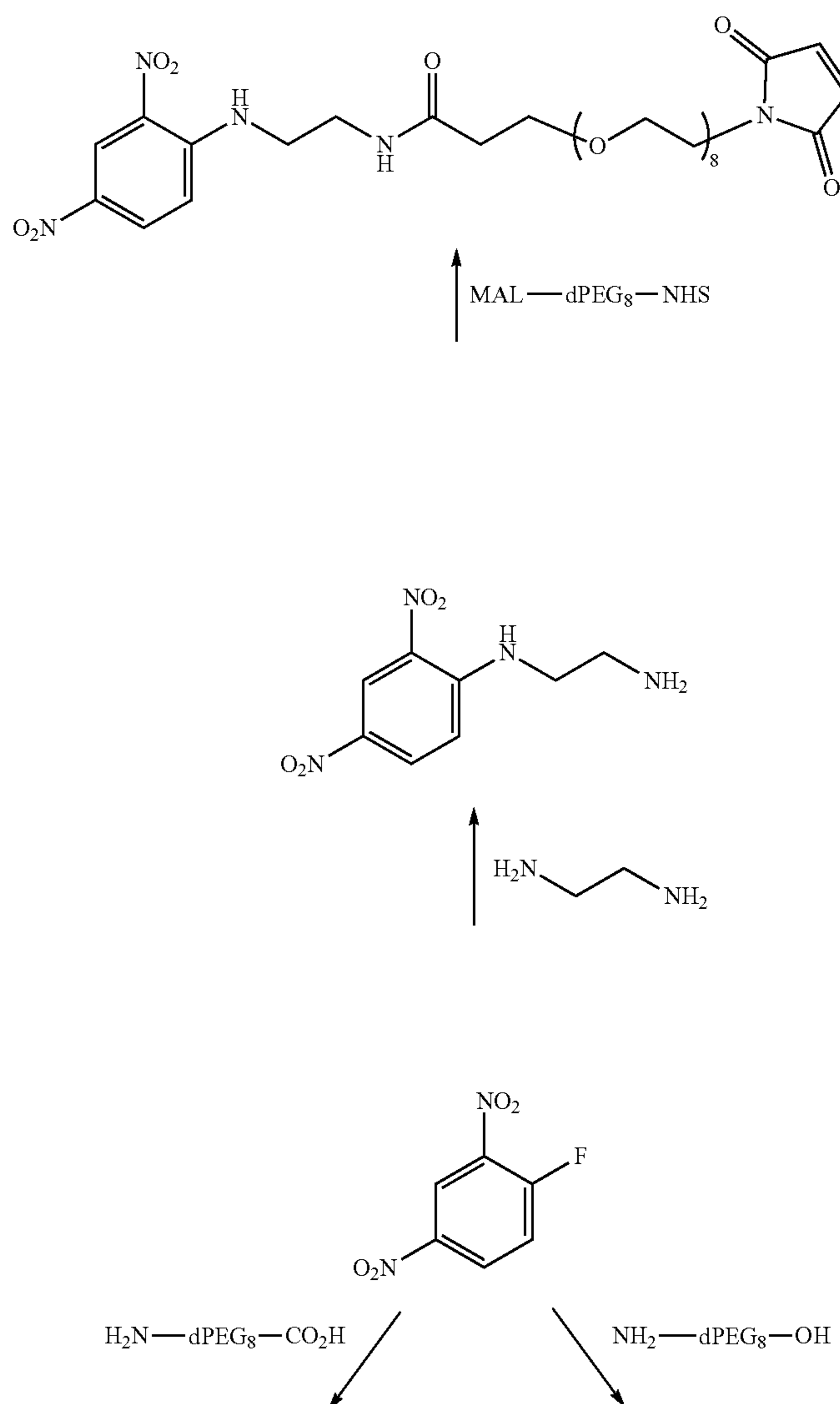
Scheme 2
