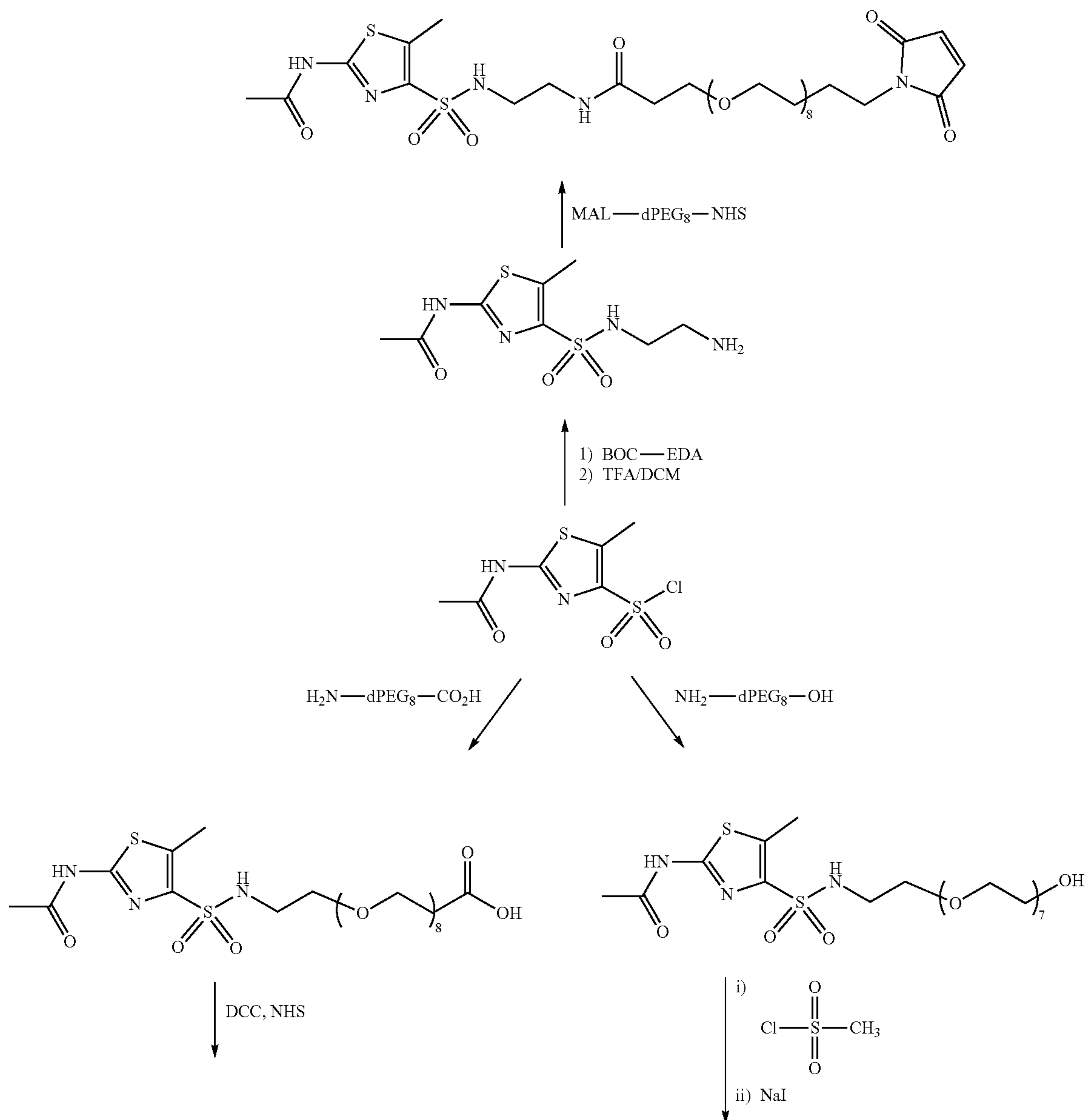
Scheme 10
