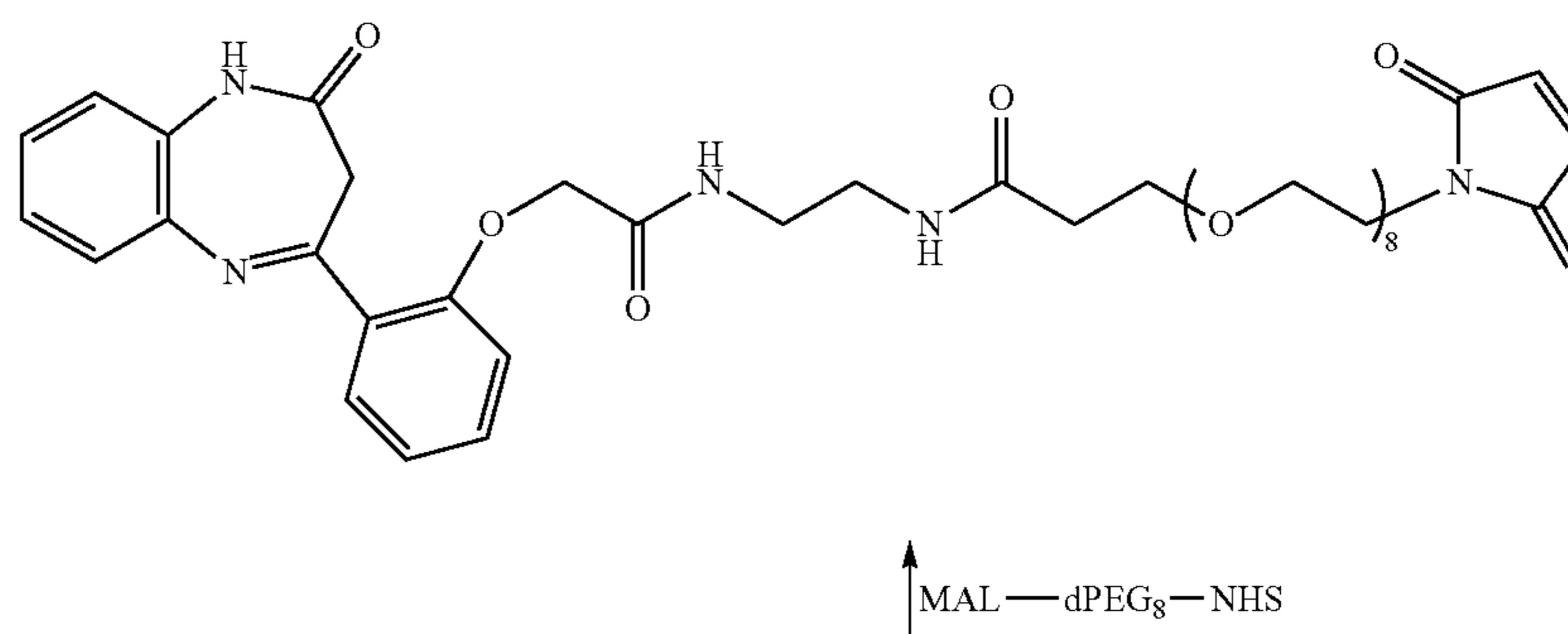
Scheme 16
