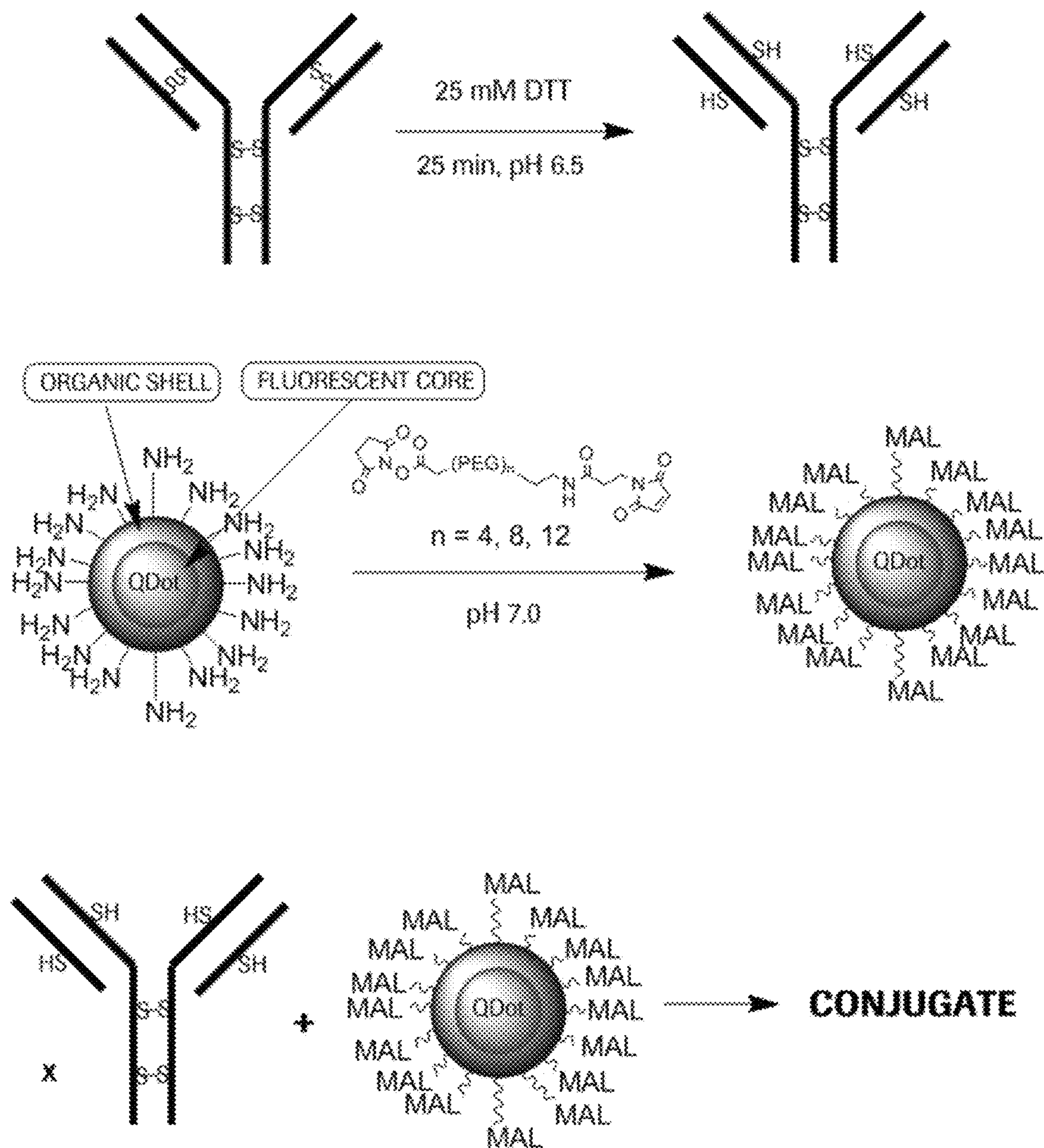
Scheme 24
