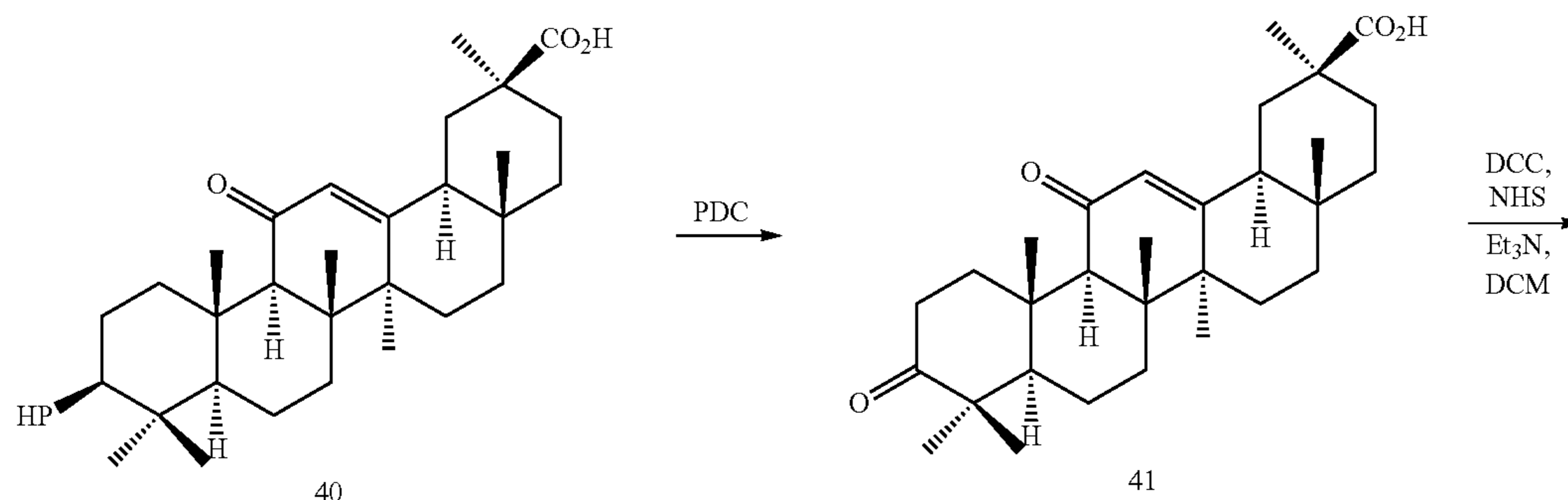
Scheme 6
