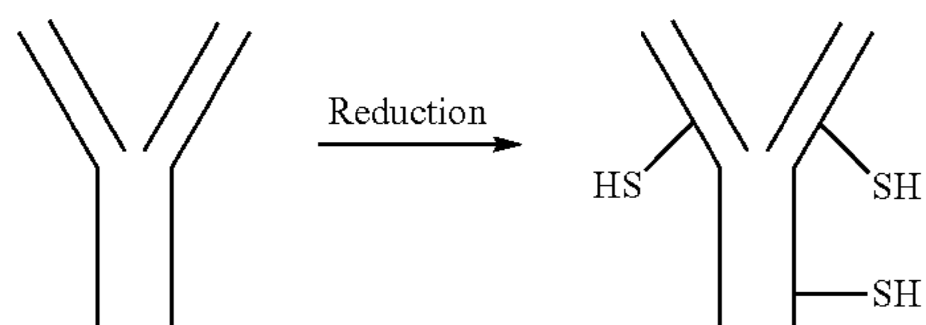
Scheme 20
