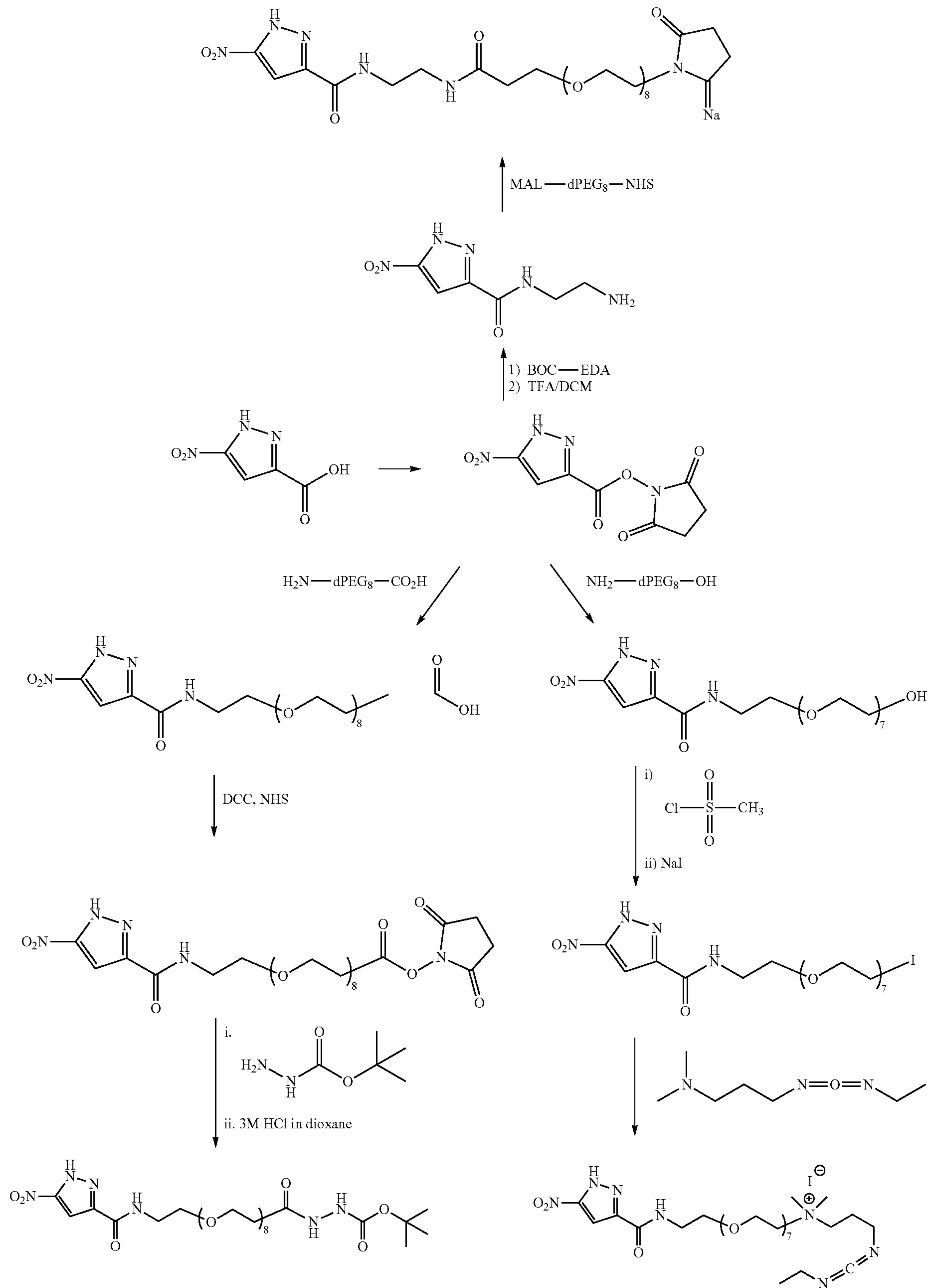
Scheme 1
