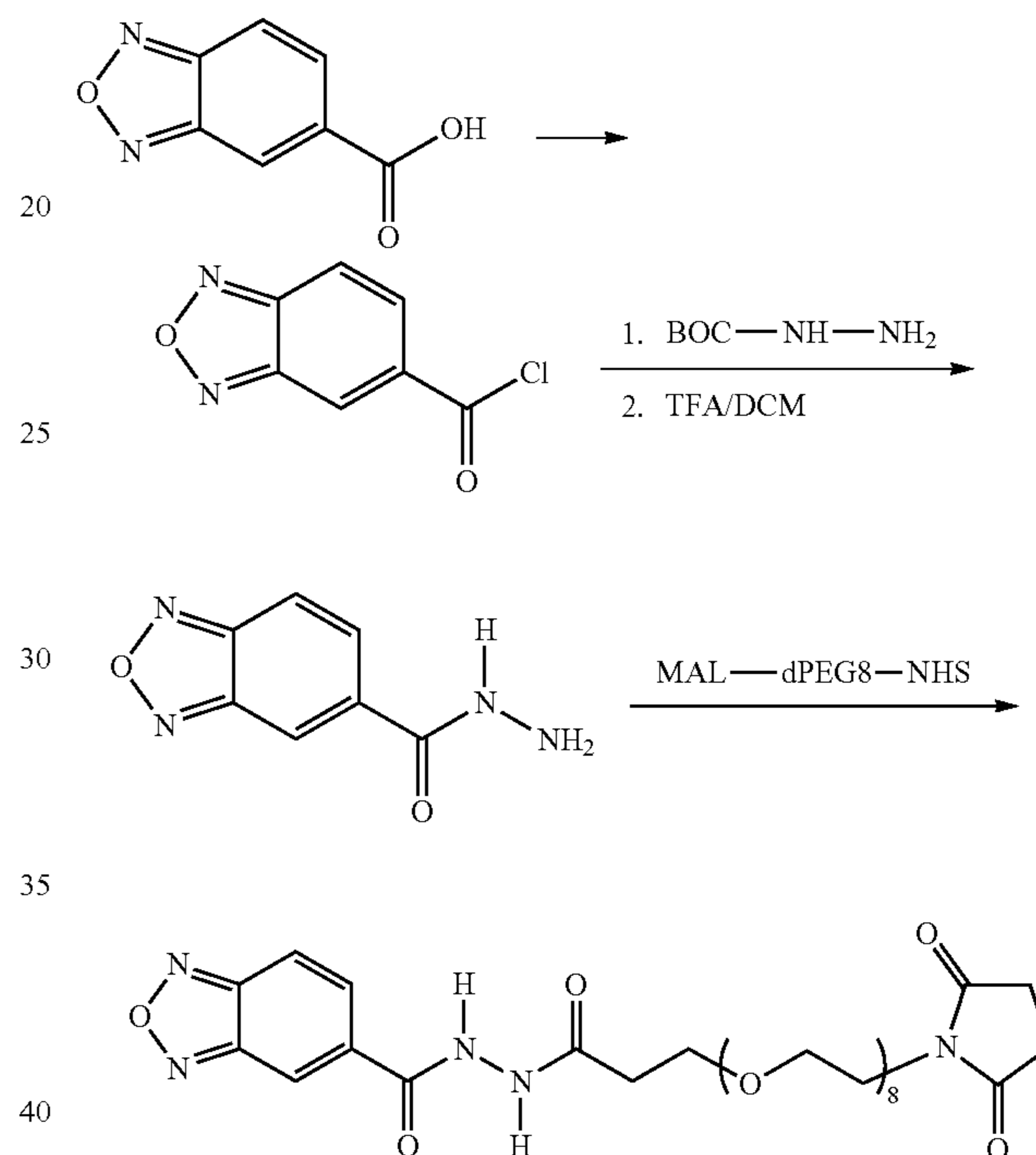
Scheme 5
