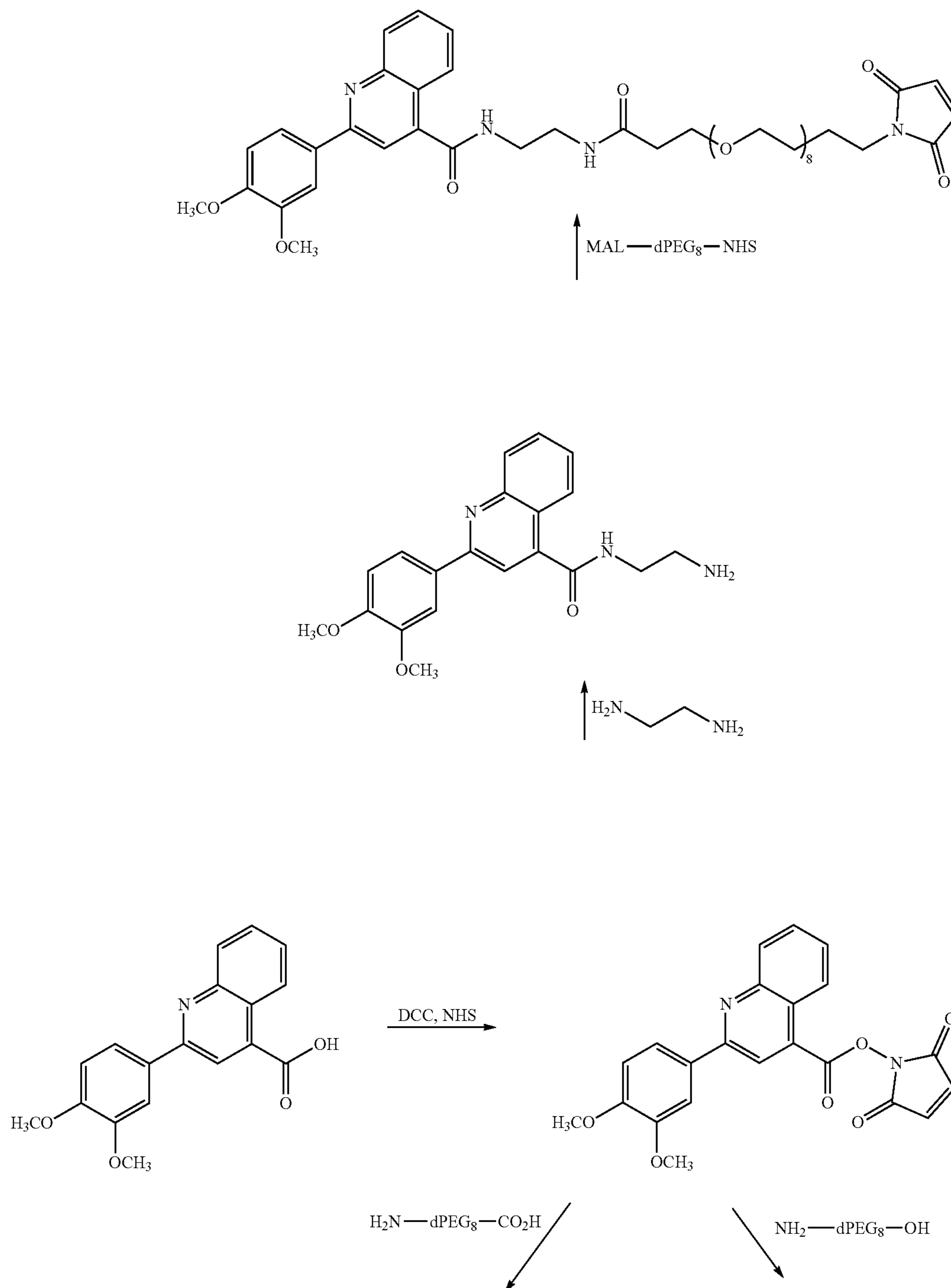
Scheme 13
