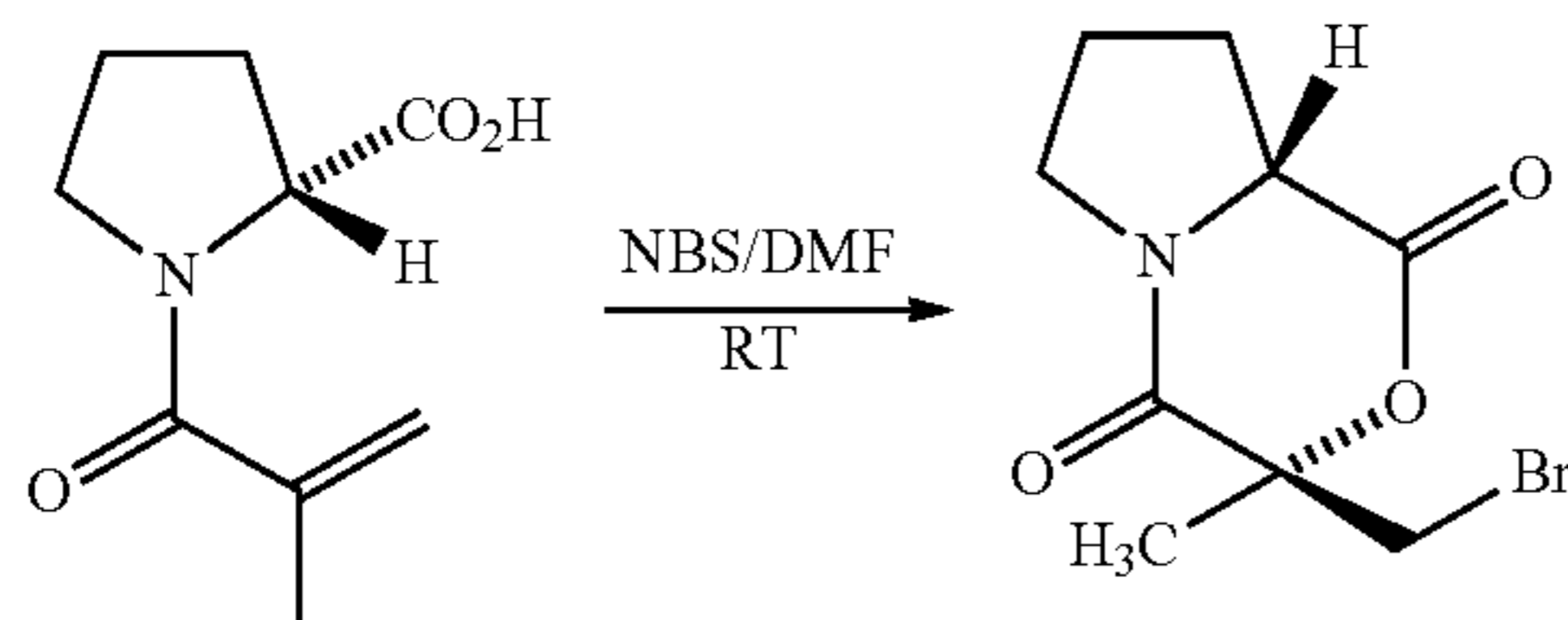
(3R,8aR)-3-Bromomethyl-3-methyl-tetrahydro-pyrrolo[2,1-c][1,4]oxazine-1,4-dione
