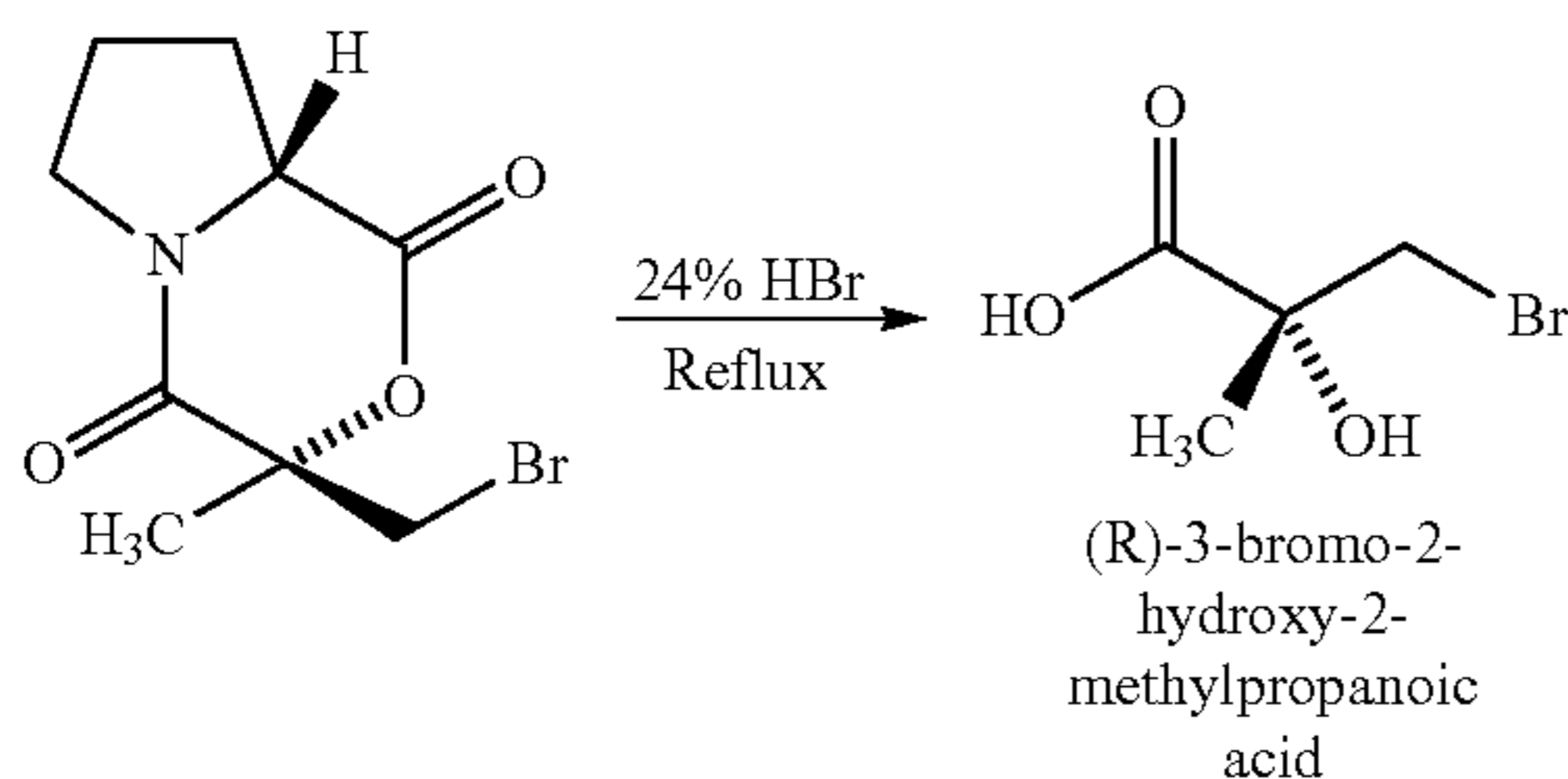
(2R)-3-Bromo-2-hydroxy-2-methylpropanoic Acid
