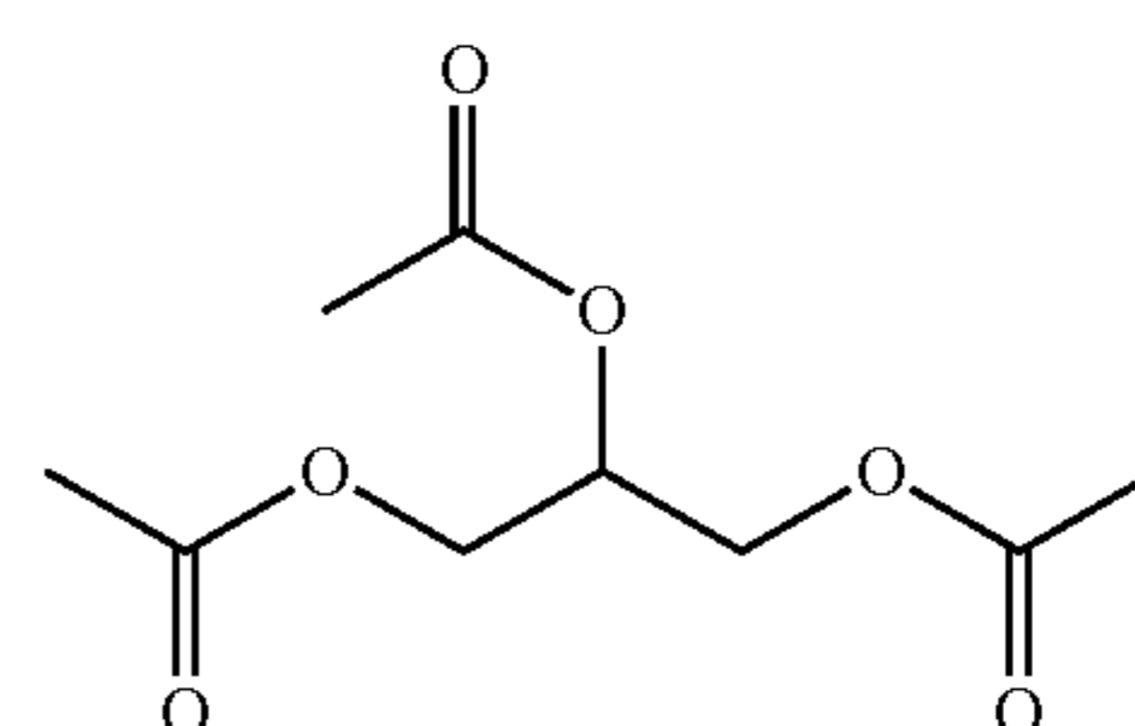
Triacetin
