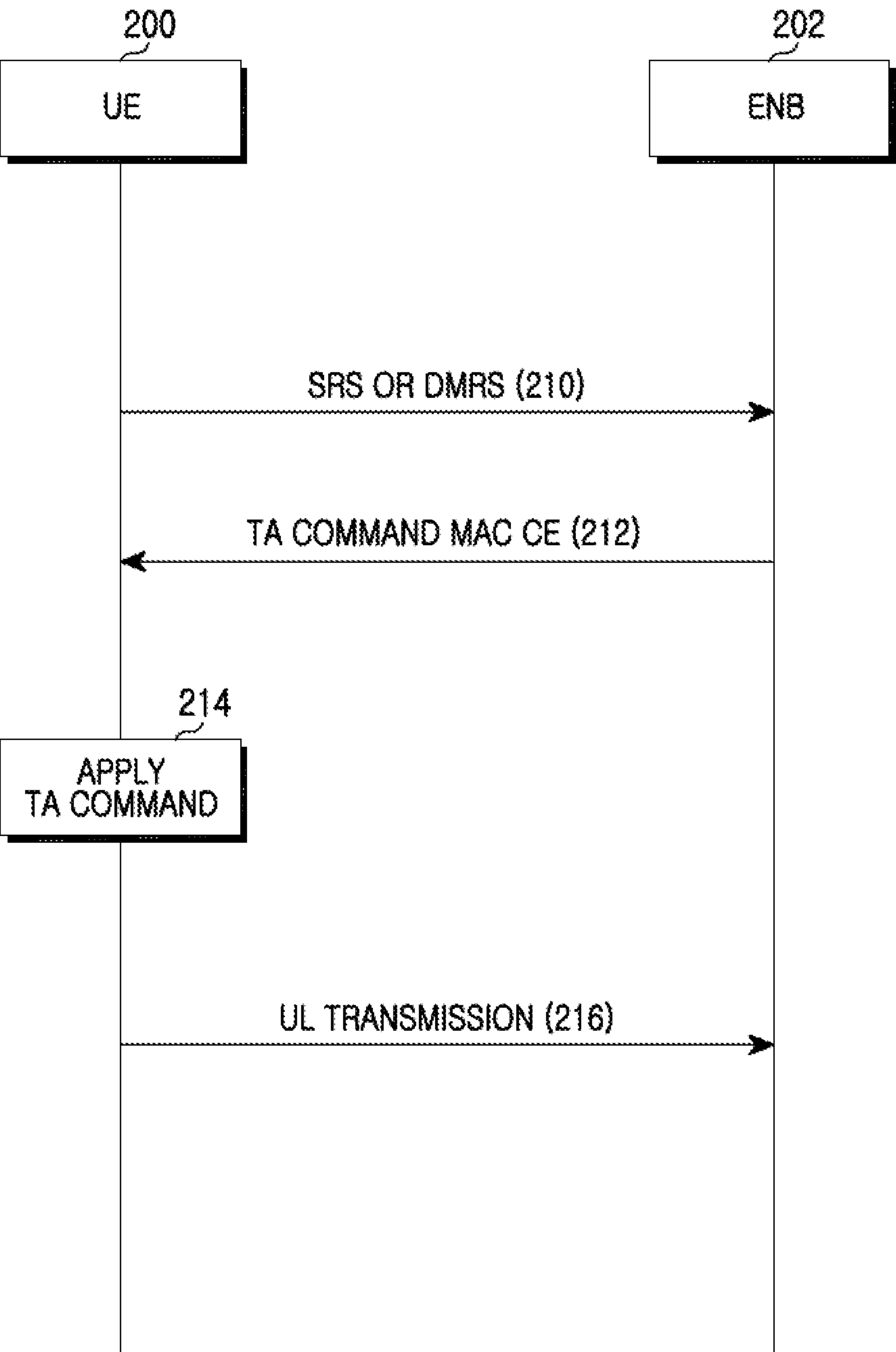
FIG.2 (PRIOR ART)
