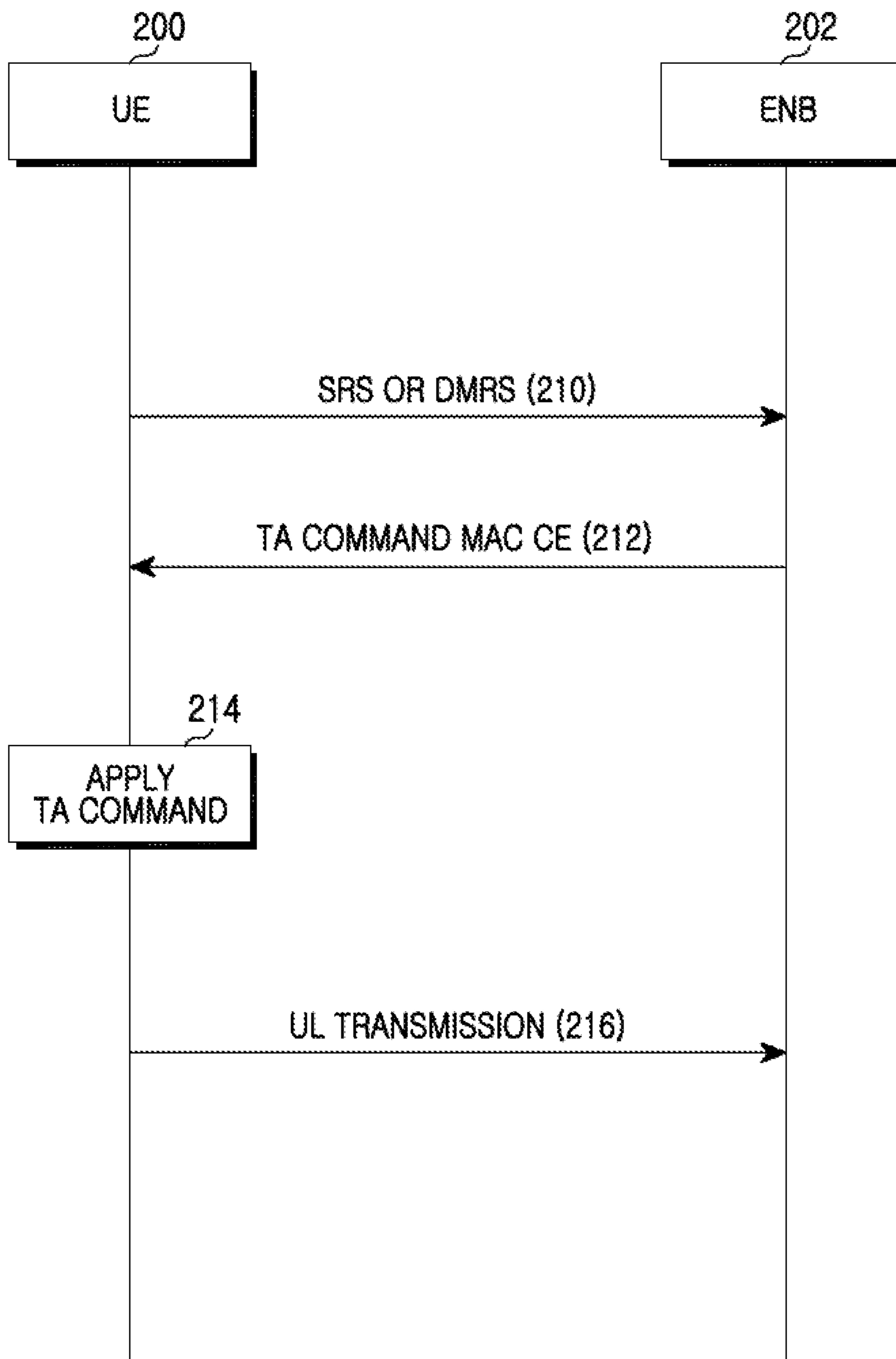
FIG. 2 (PRIOR ART)
