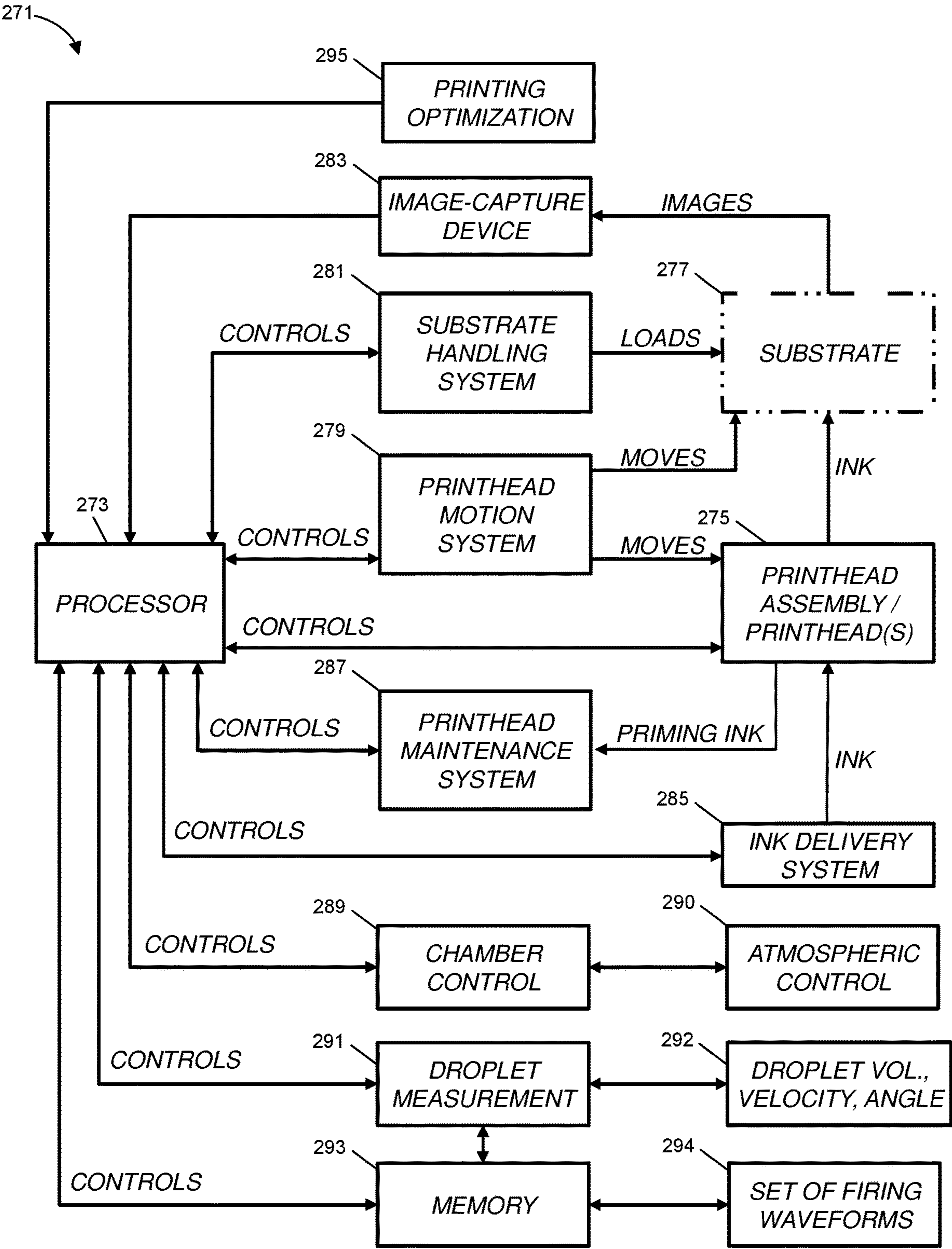
FIG. 2D
