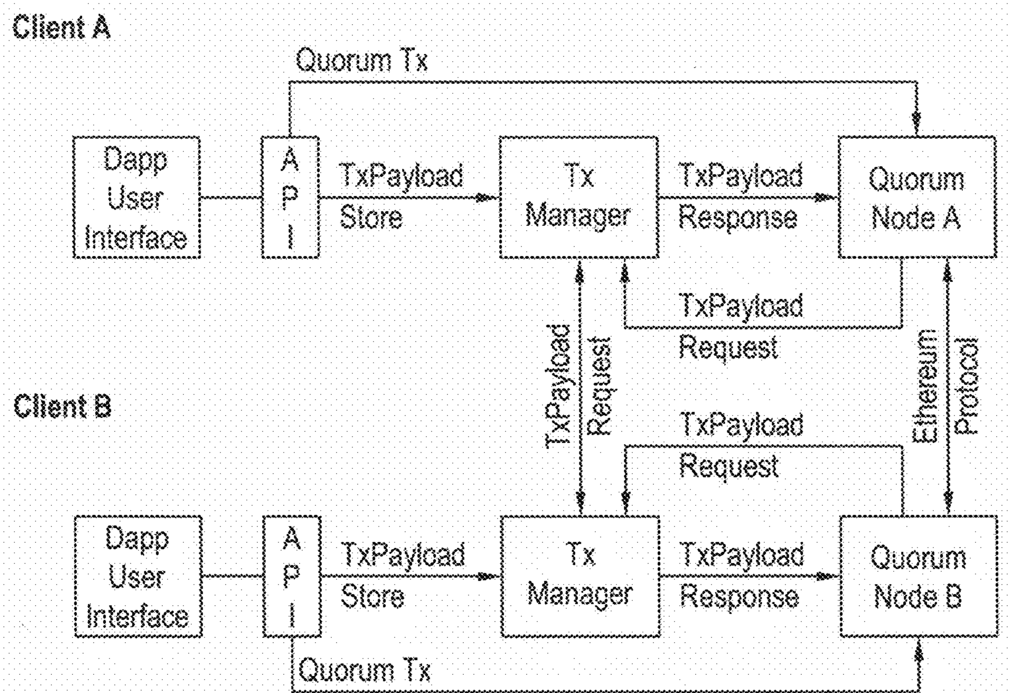
Permissioned System
