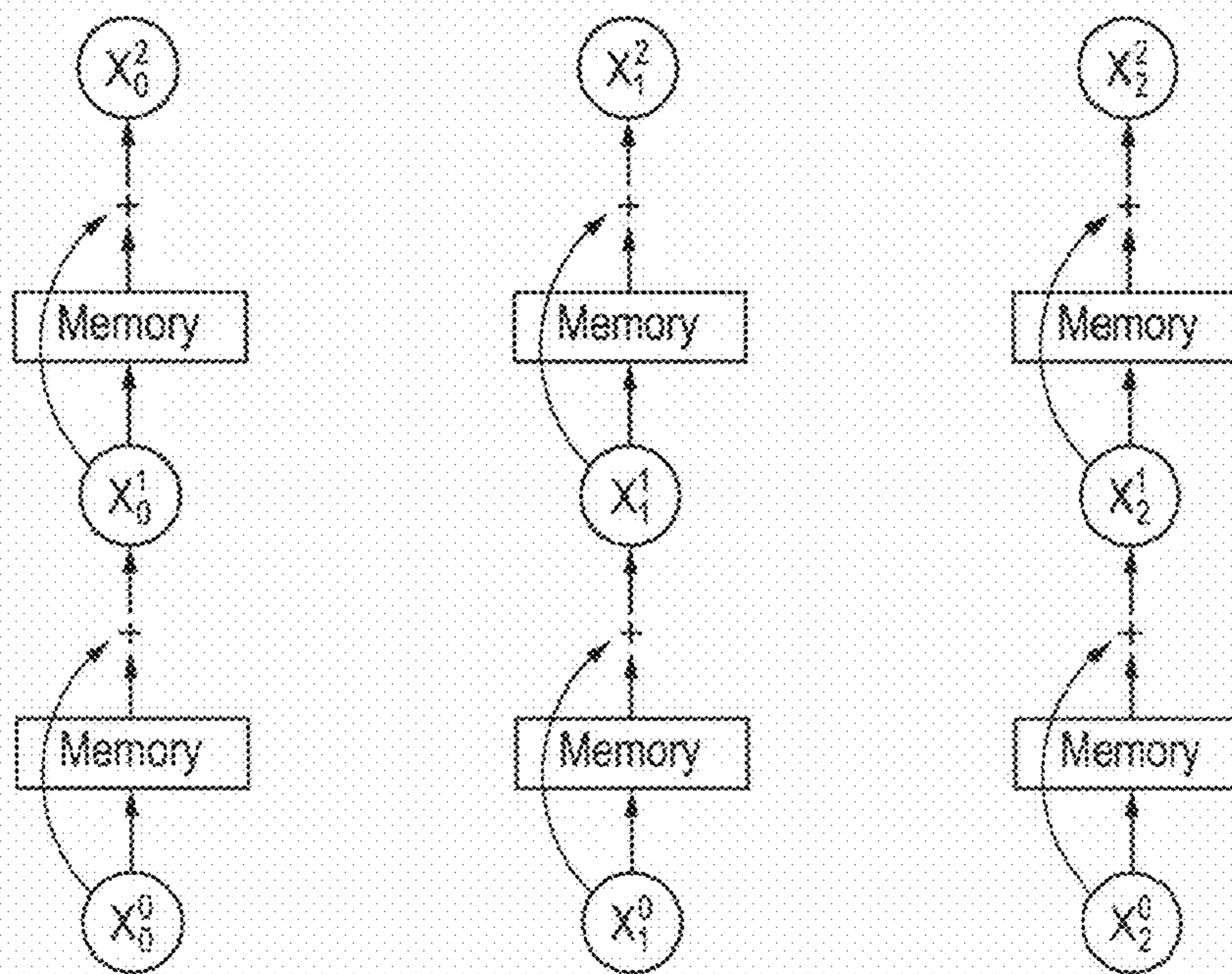
Neural Network
