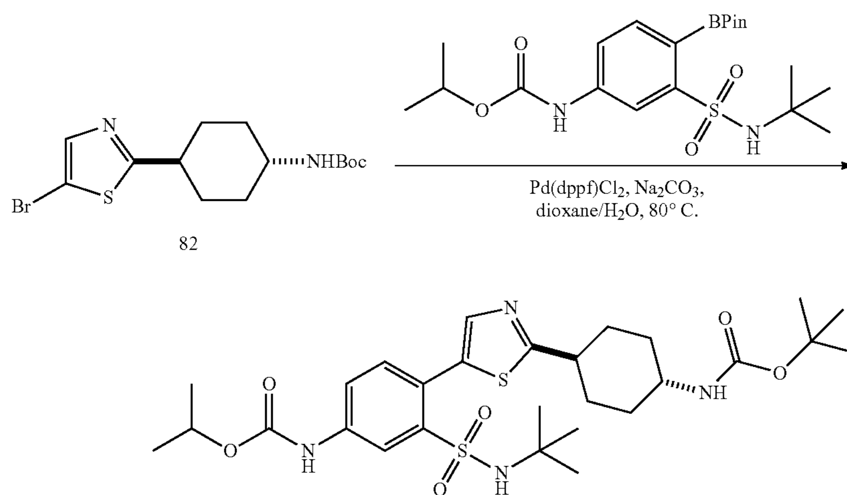
Scheme 14
