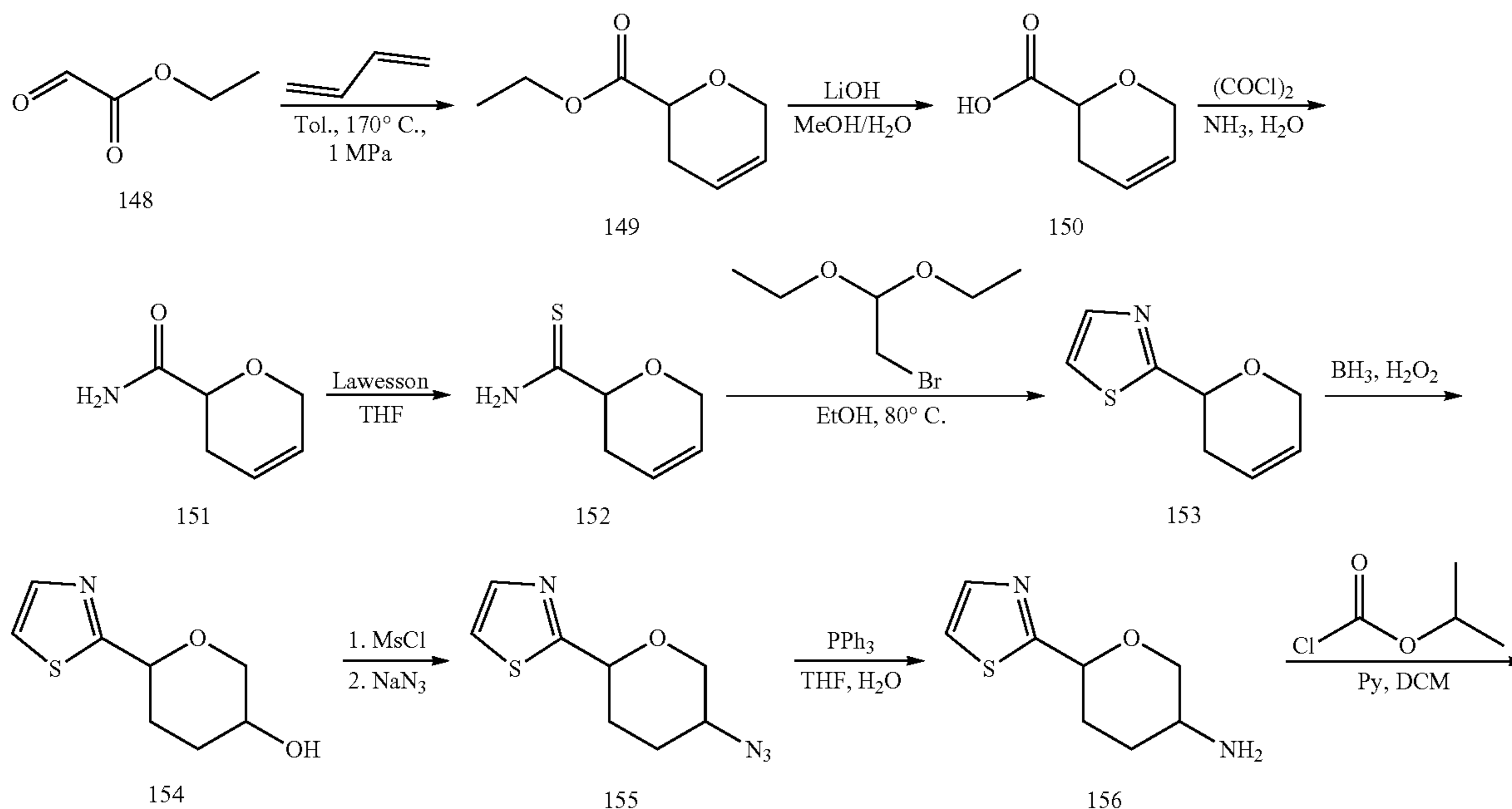
Scheme 20
