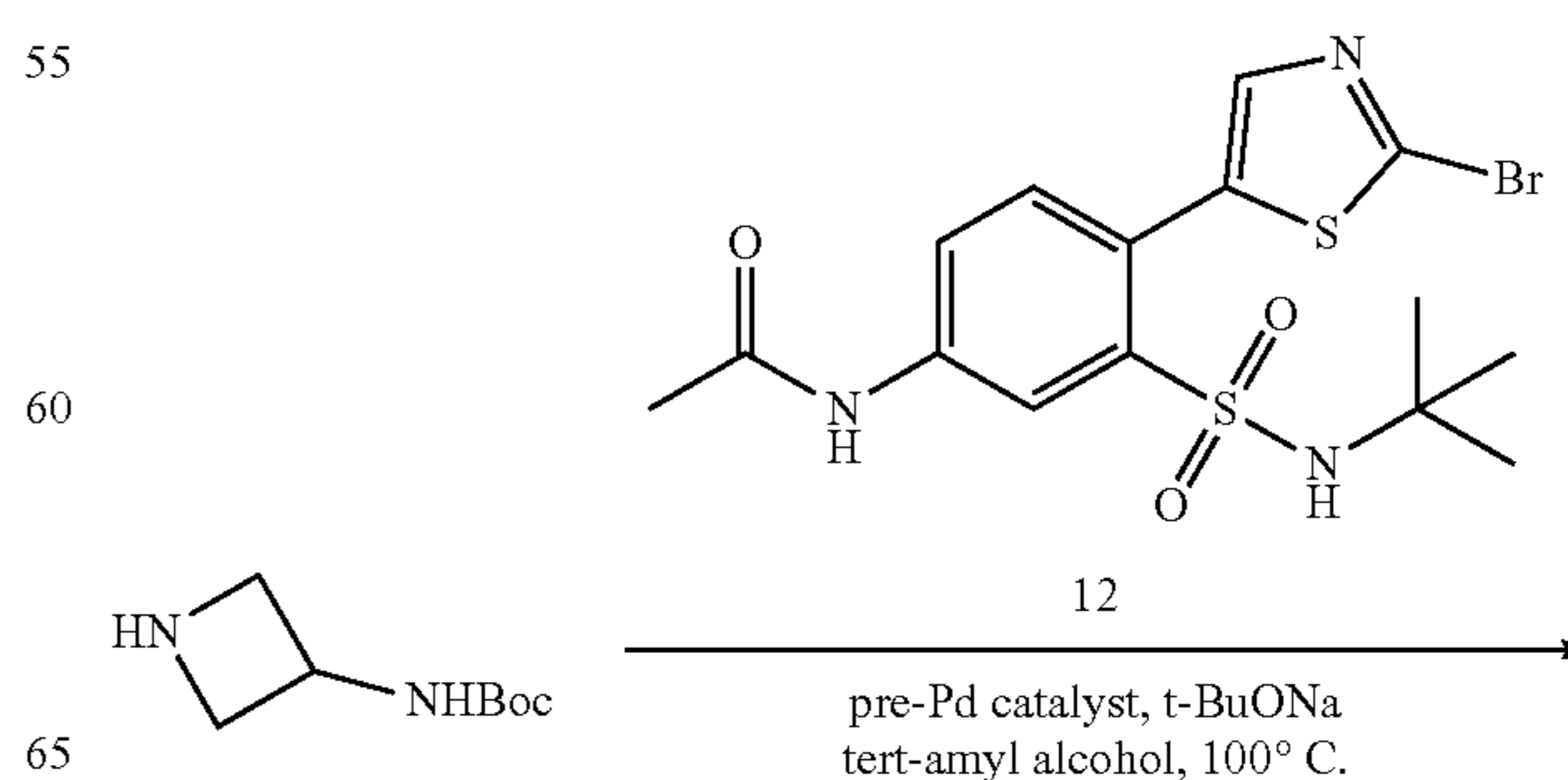
Scheme 15
