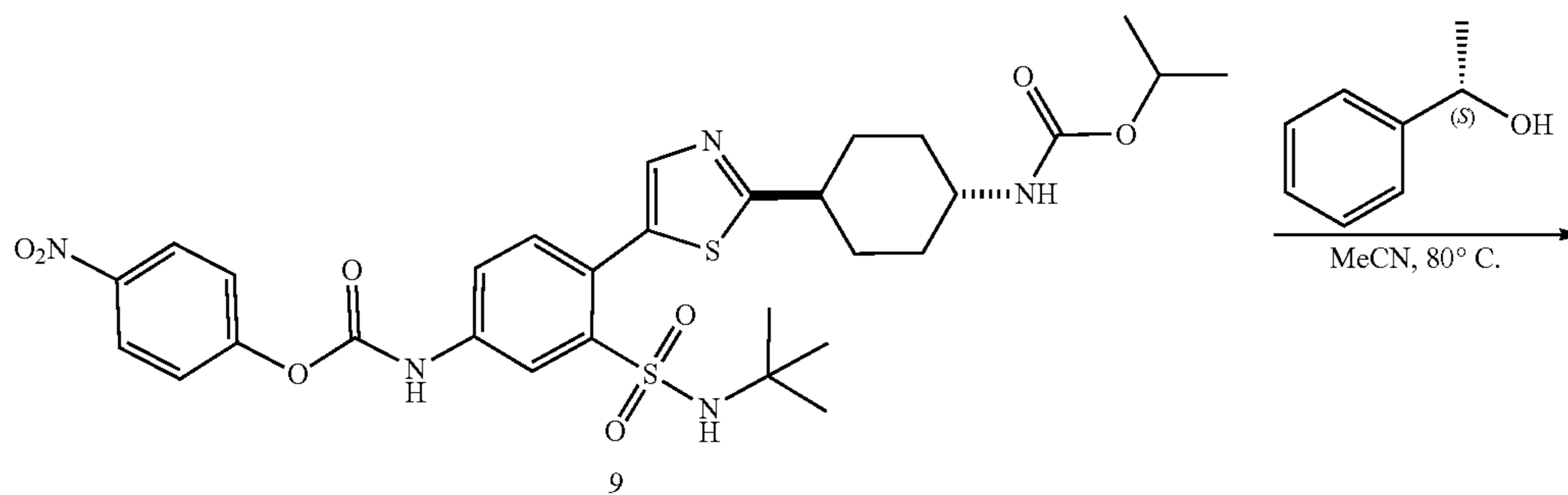
Scheme 30
