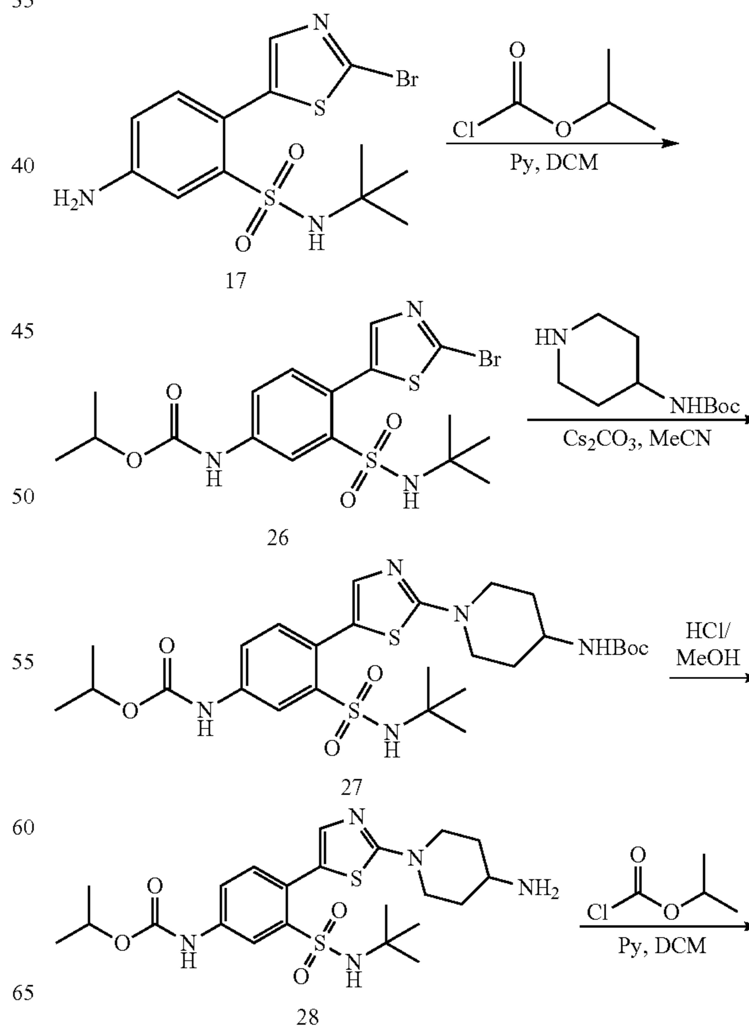
Scheme 28
