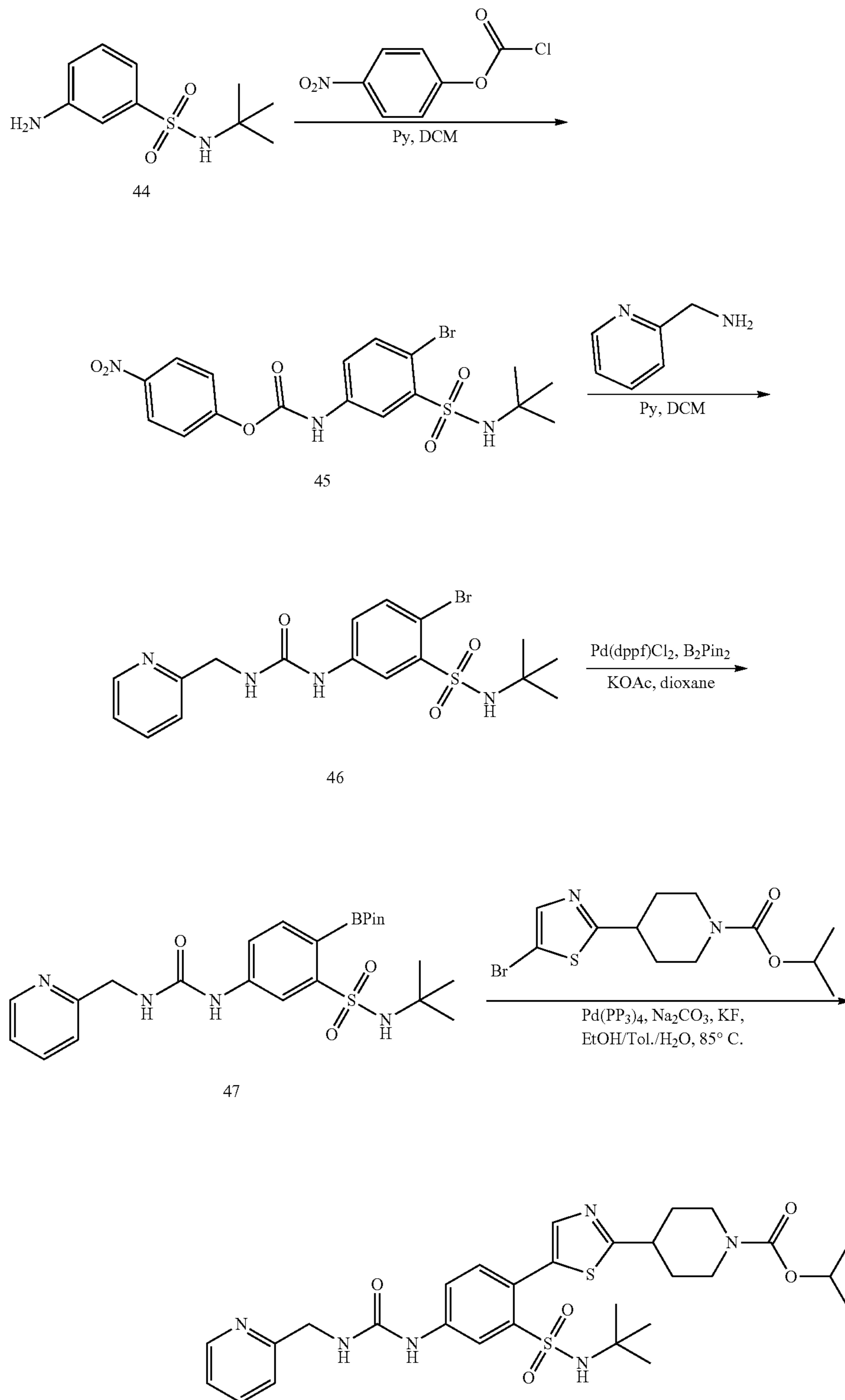
Scheme 3
