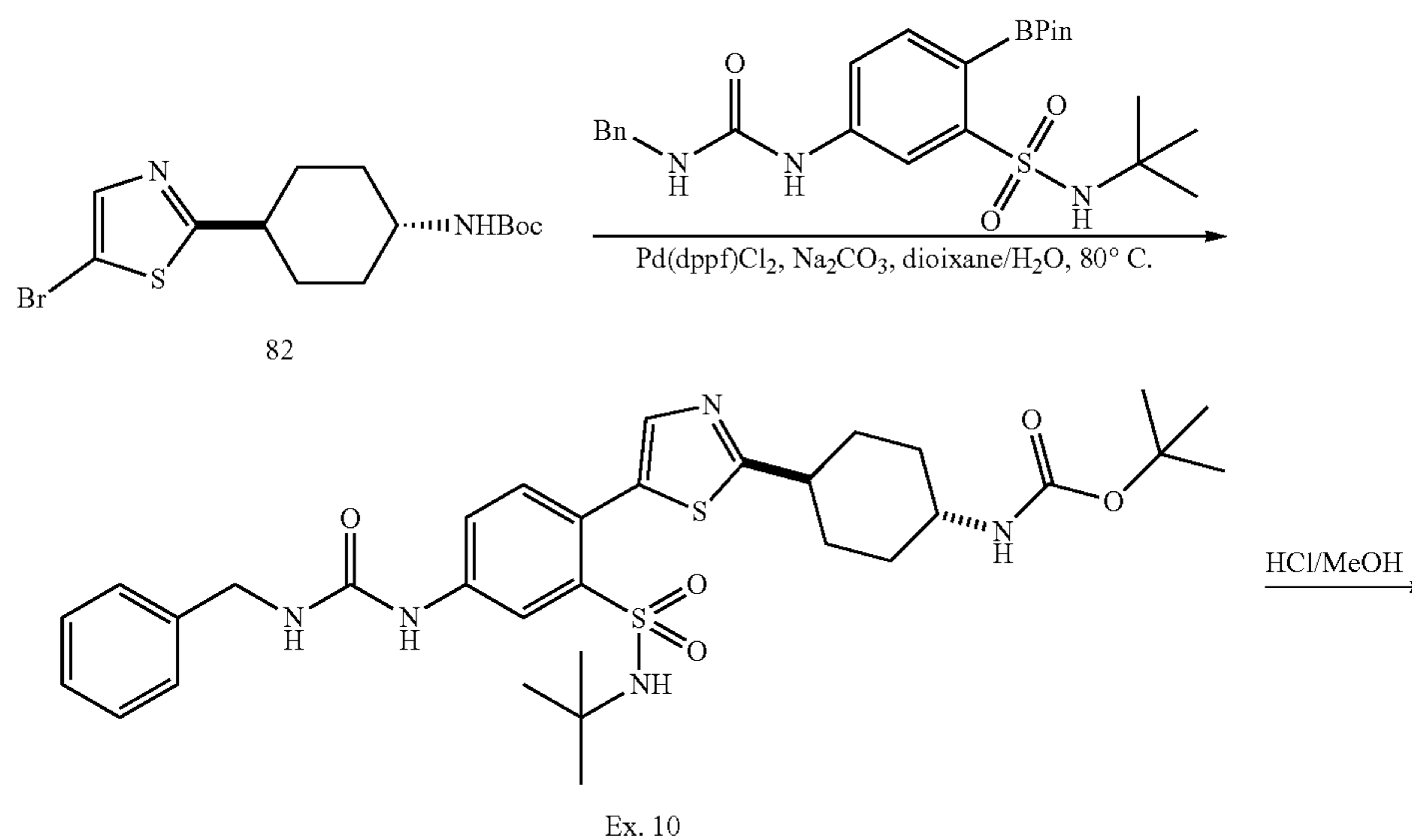
Scheme 8
