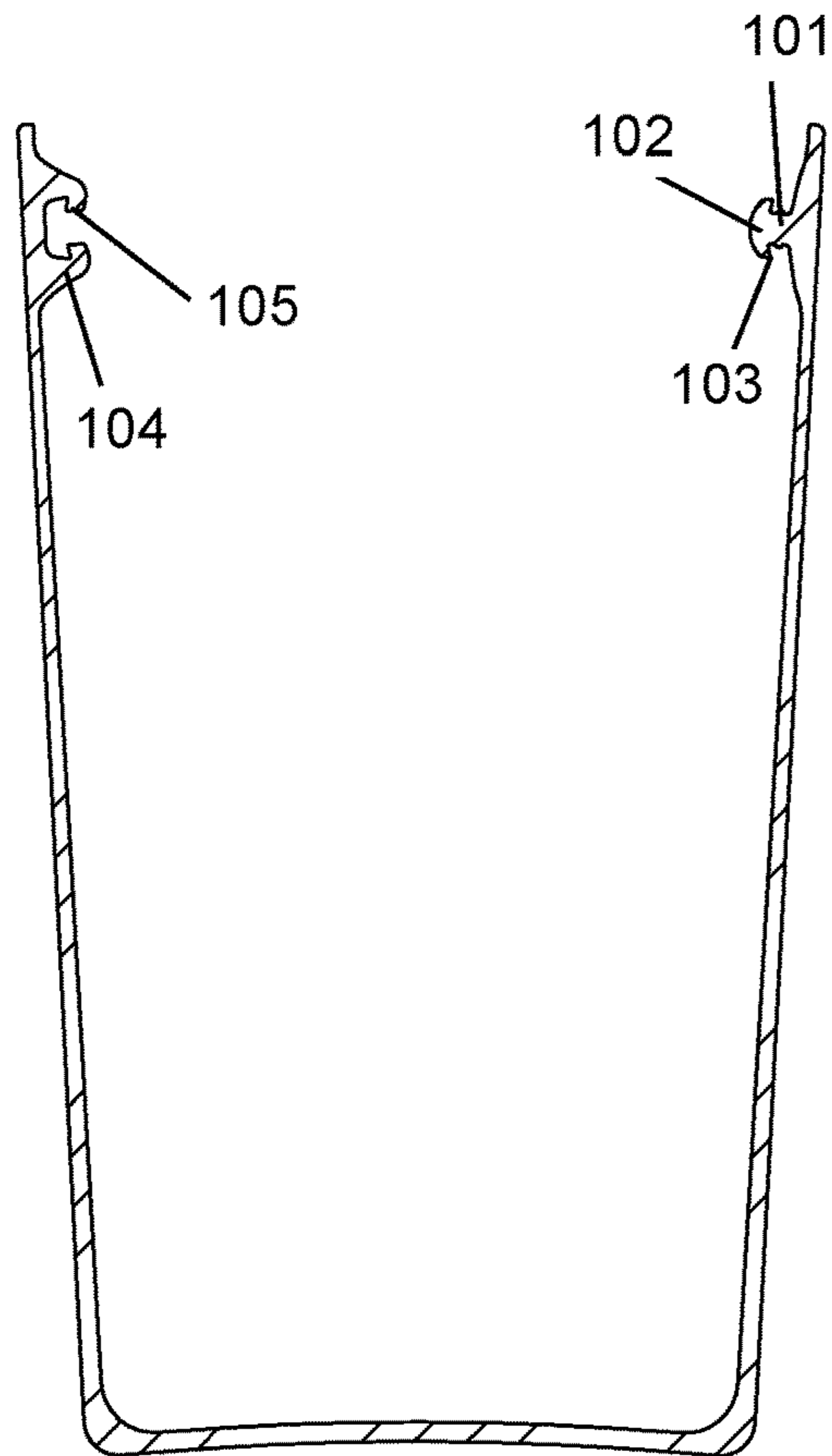
SECTION C-C
