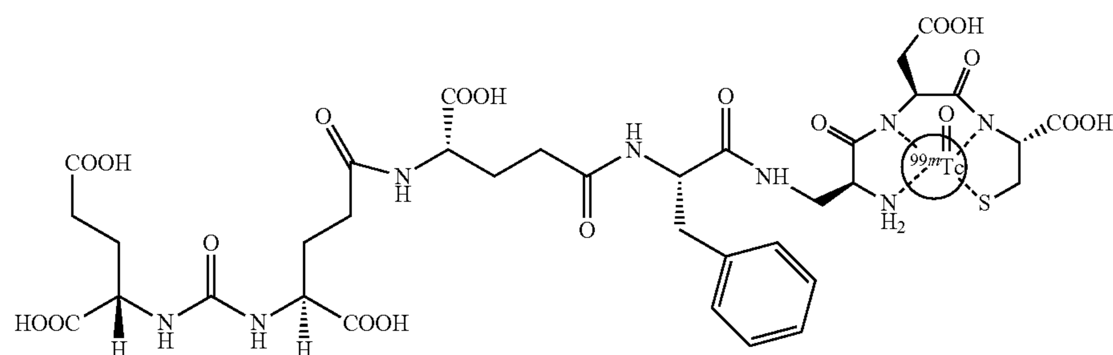
SK62- 99m Tc (7-atom linker, 1.0 mg),
