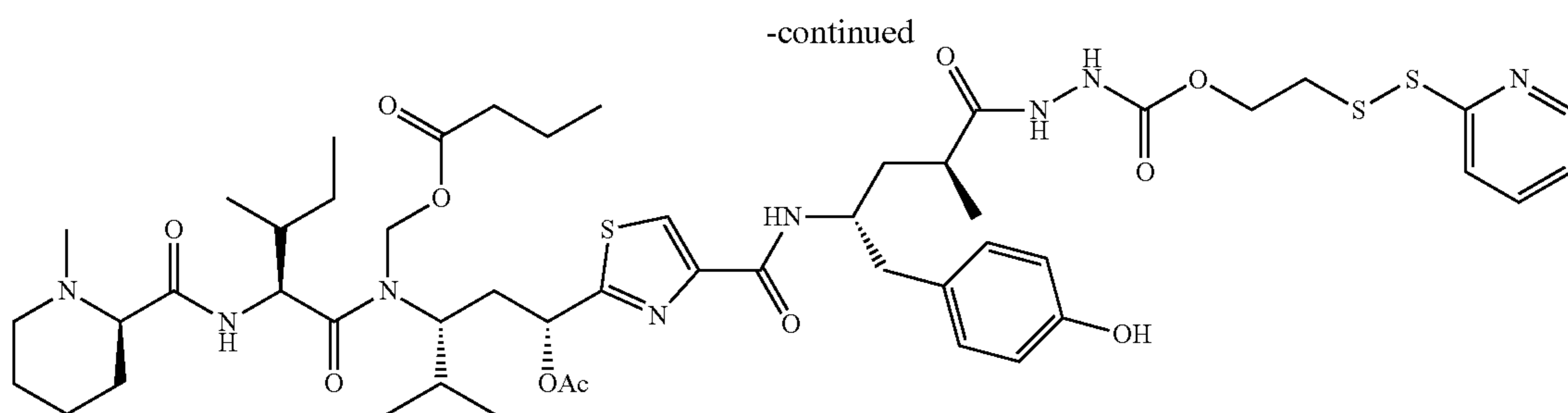
EC0312 C_{50}H_{72}N_8O_{11}S_3 Mol. Wt.: 1057.35
