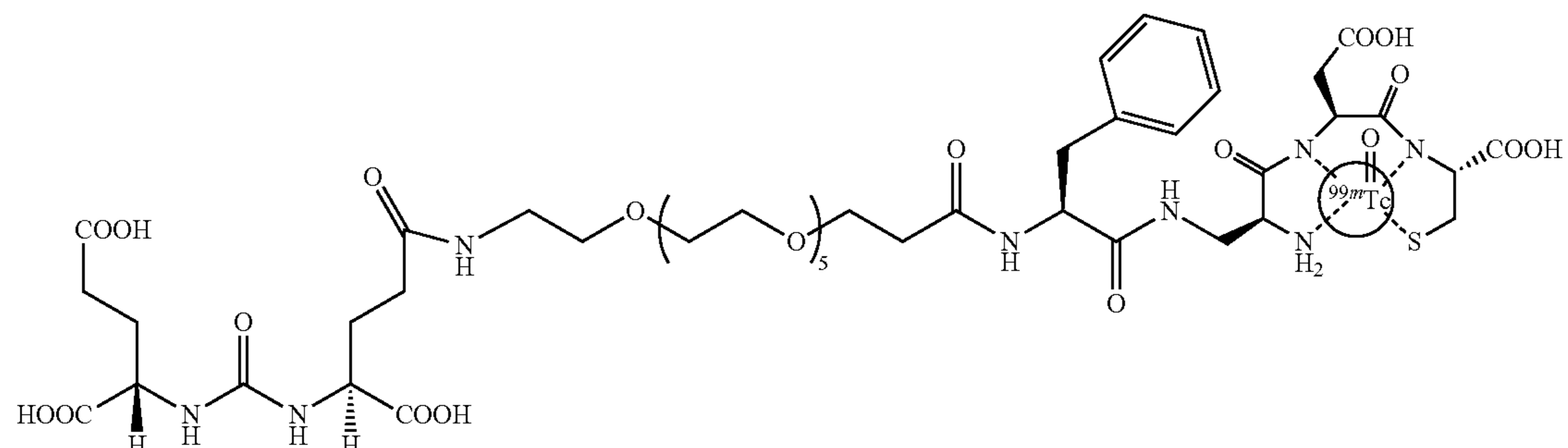
SK57- 99m Tc (24-atom linker, 1.8 mg)
