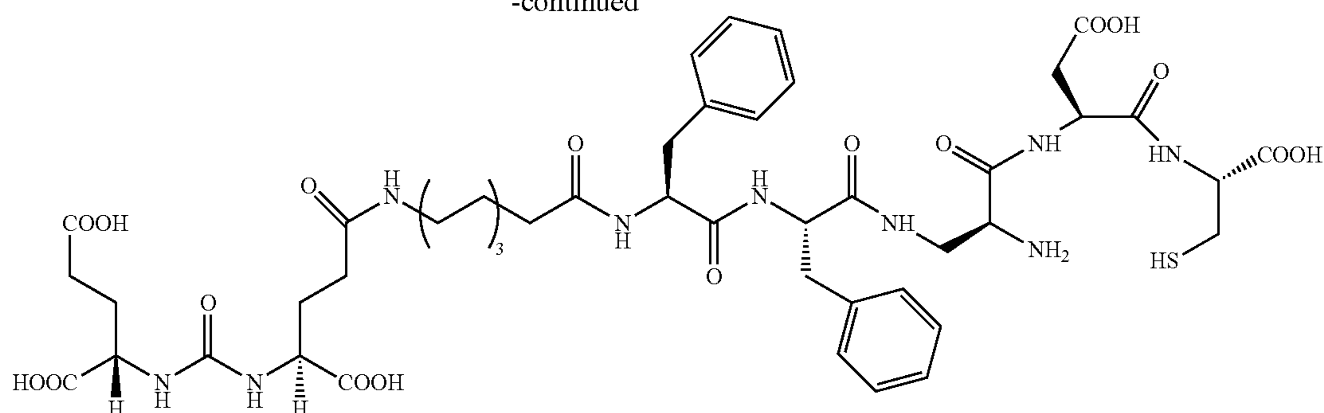
PC01SK28 C_{47}H_{65}N_9O_{17}S Mol. Wt.: 1060.13
