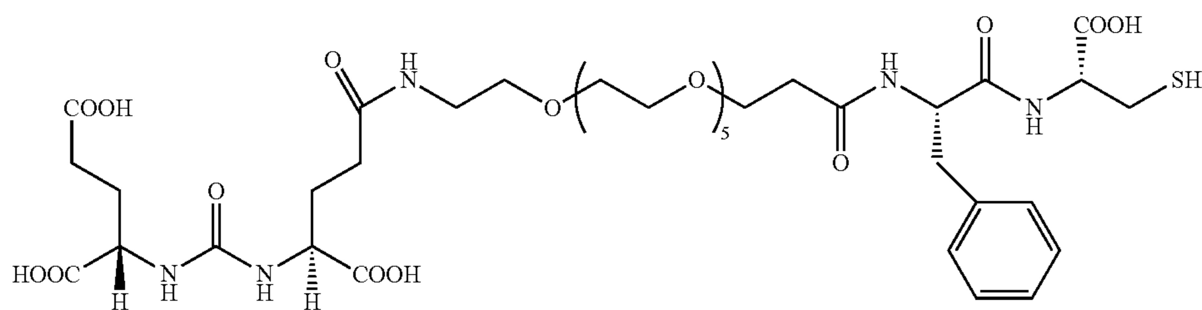
PC01SK54 C_{38}H_{59}N_5O_{18}S Mol. Wt.: 905.96
