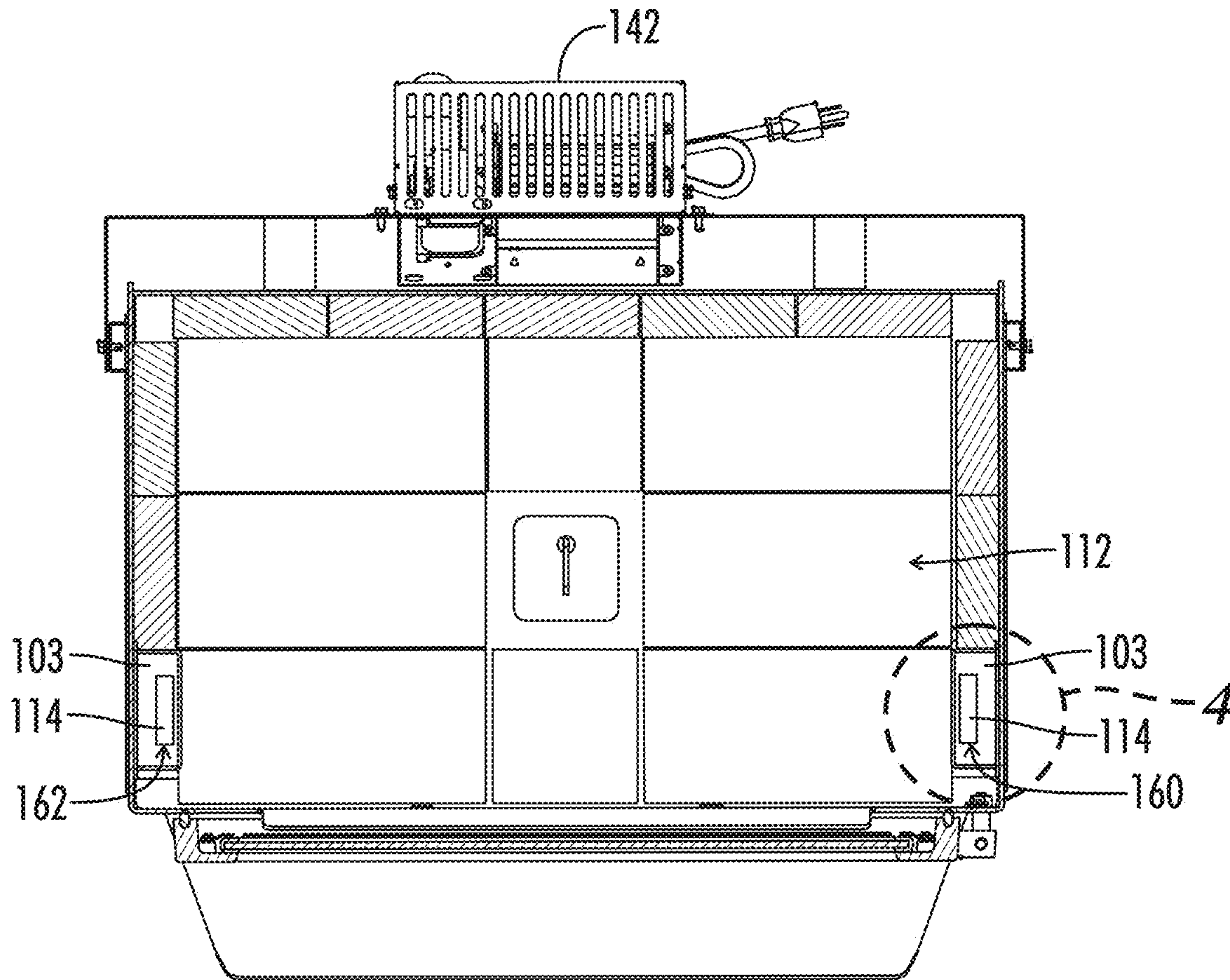
SECTION B-B
