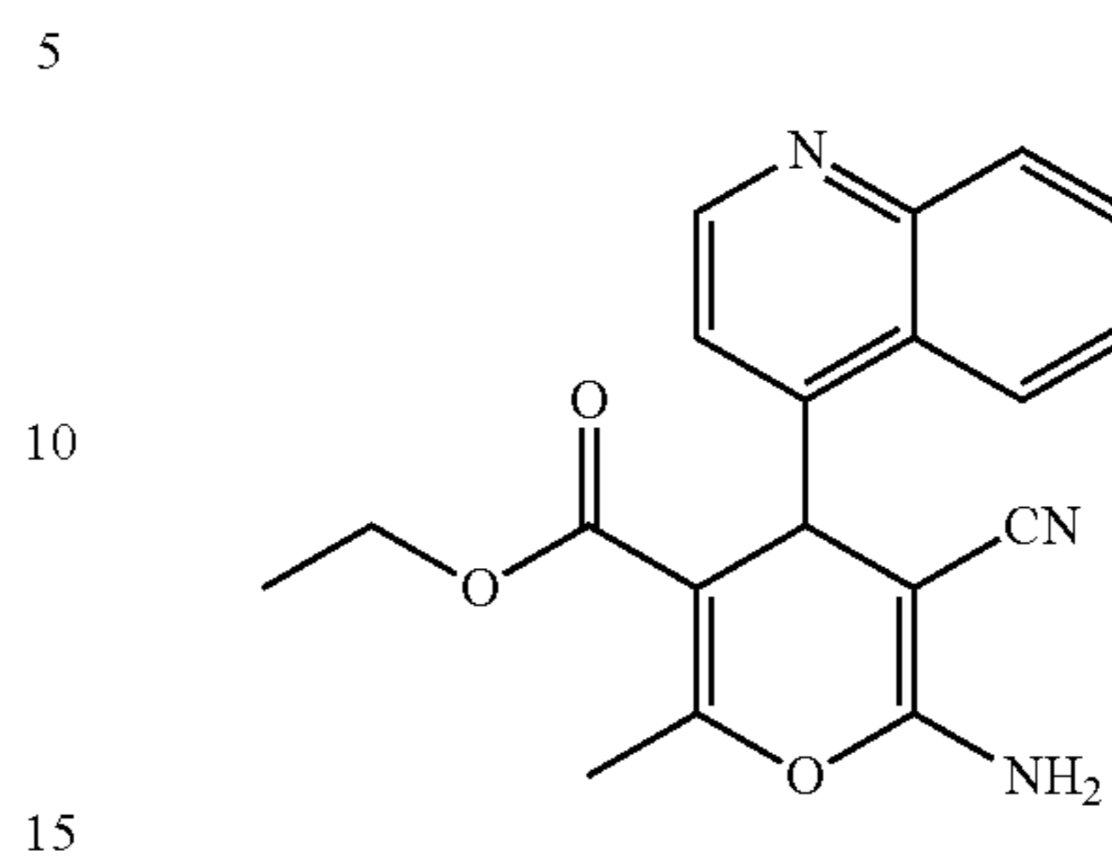
Ethyl 6-amino-5-cyano-2-methyl-4-(quinolin-4-yl)-4H-pyran-3-carboxylate
