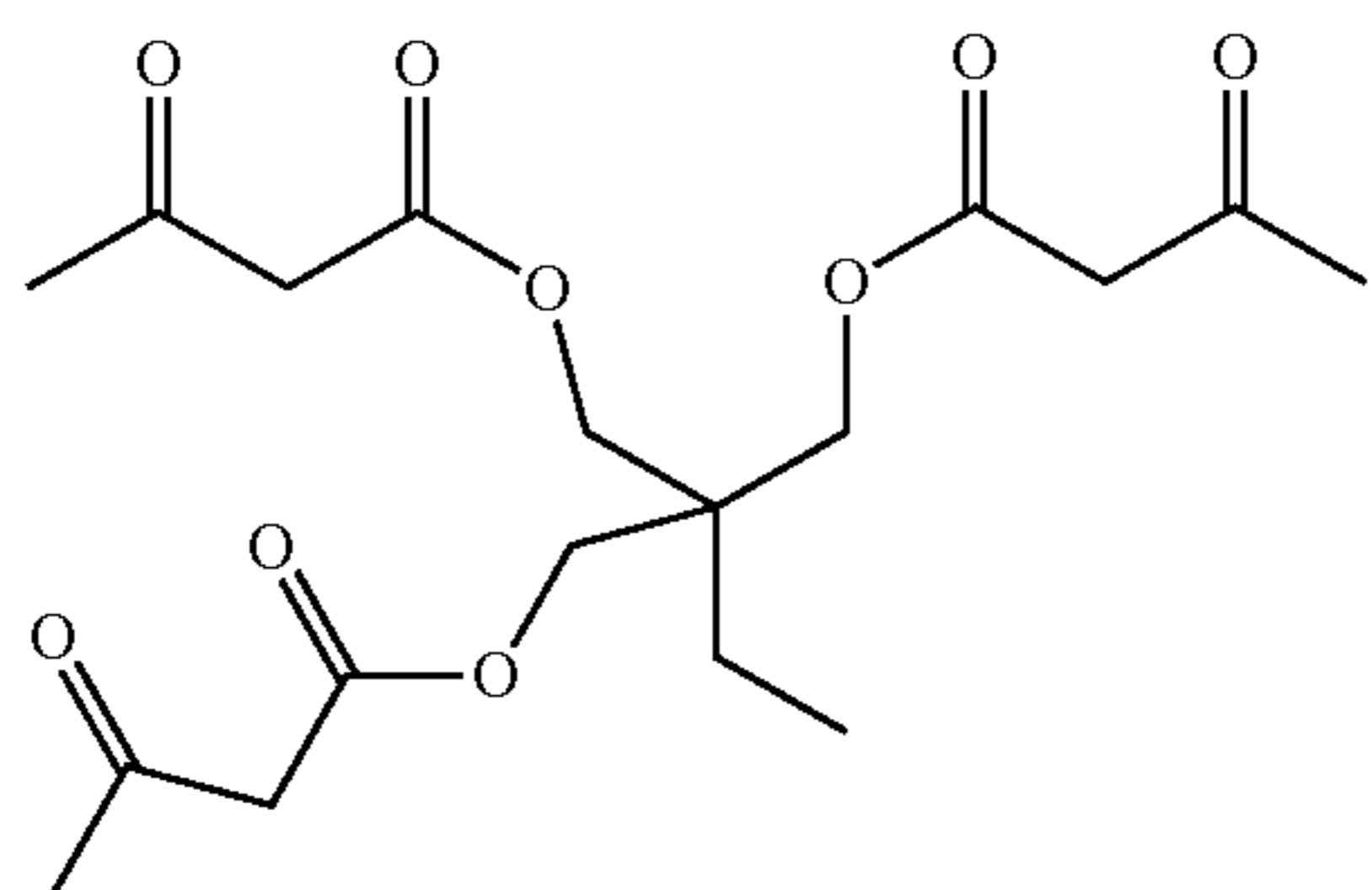
2-ethyl-2-(((3-oxobutanoyl)oxy)methyl)propane-1,3-diyl bis(3-oxobutanoate)
