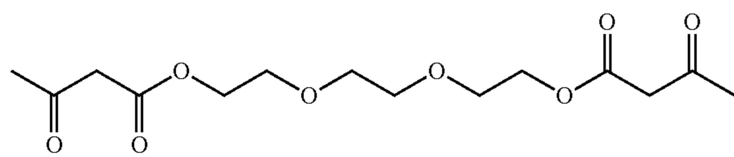
(ethane-1,2-diylbis(oxy))bis(ethane-2,1-diyl) bis(3-oxobutanoate)
