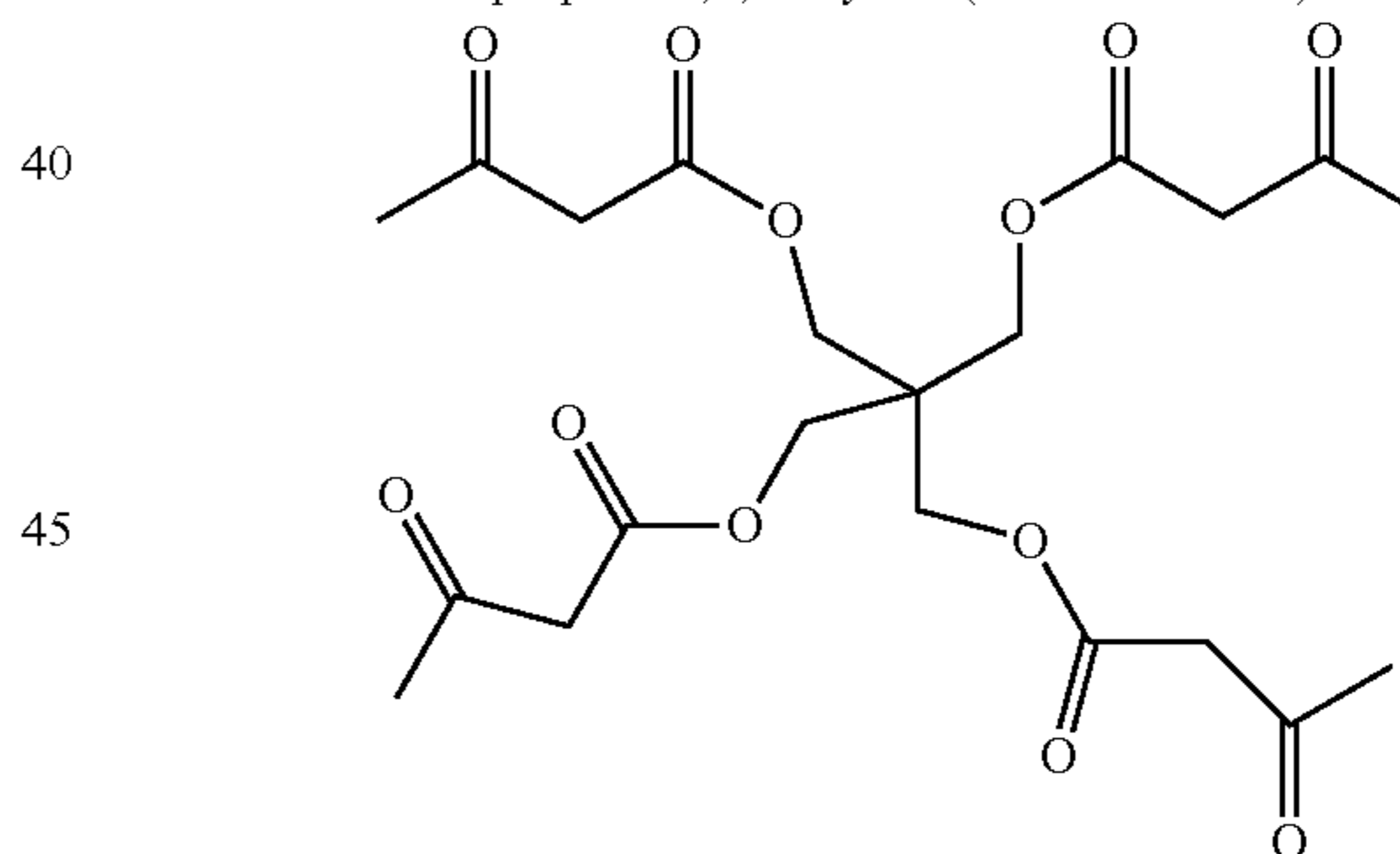
2,2-bis(((3-oxobutanoyl)oxy)methyl)propane-1,3-diyl bis(3-oxobutanoate)
