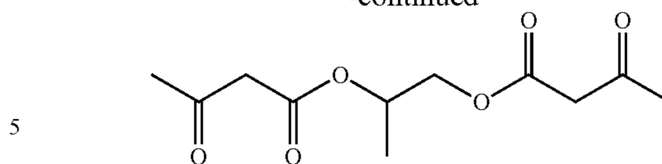
propane-1,2-diyl bis(3-oxobutanoate)
