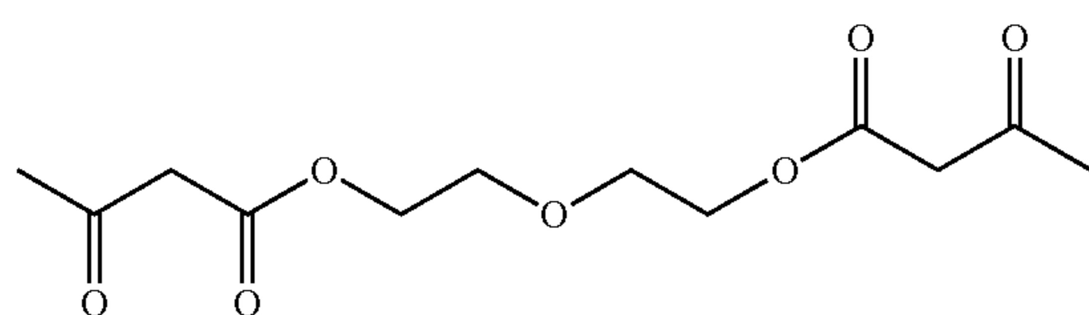
oxybis(ethane-2,1-diyl) bis(3-oxobutanoate)
