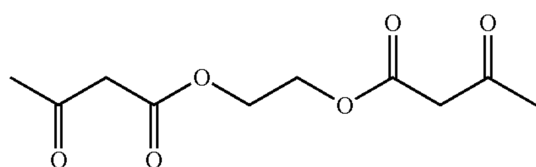
ethane-1,2-diyl bis(3-oxobutanoate)
