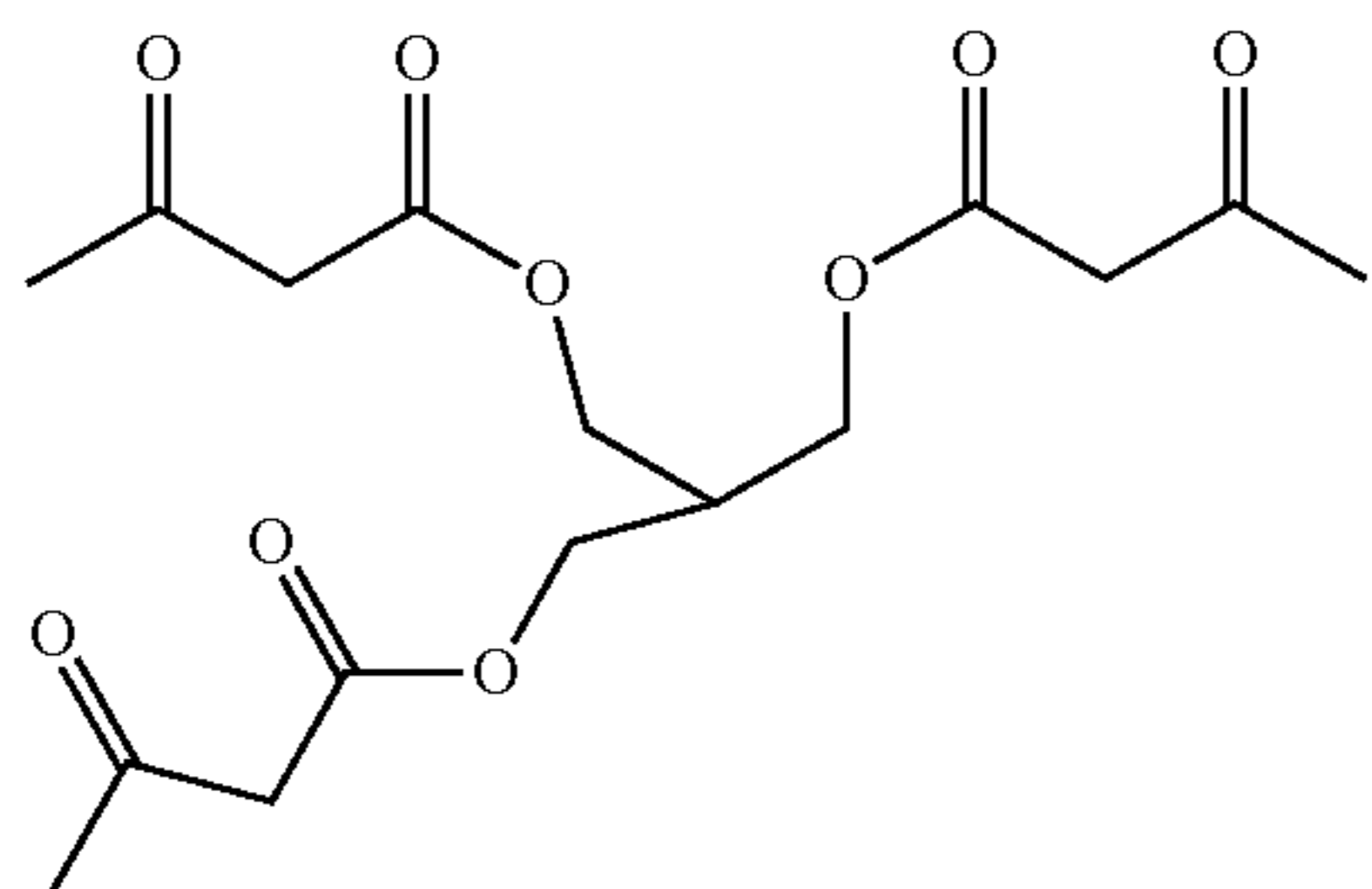
2-(((3-oxobutanoyl)oxy)methyl)propane-1,3-diyl bis(3-oxobutanoate)
