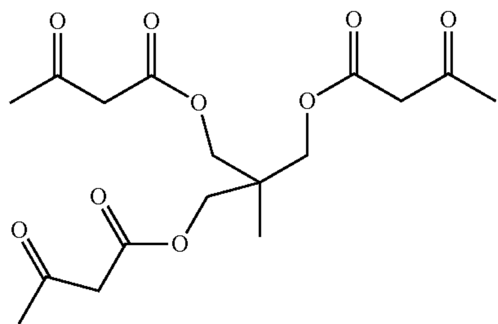
2-methyl-2-(((3-oxobutanoyl)oxy)methyl)propane-1,3-diyl bis(3-oxobutanoate)
