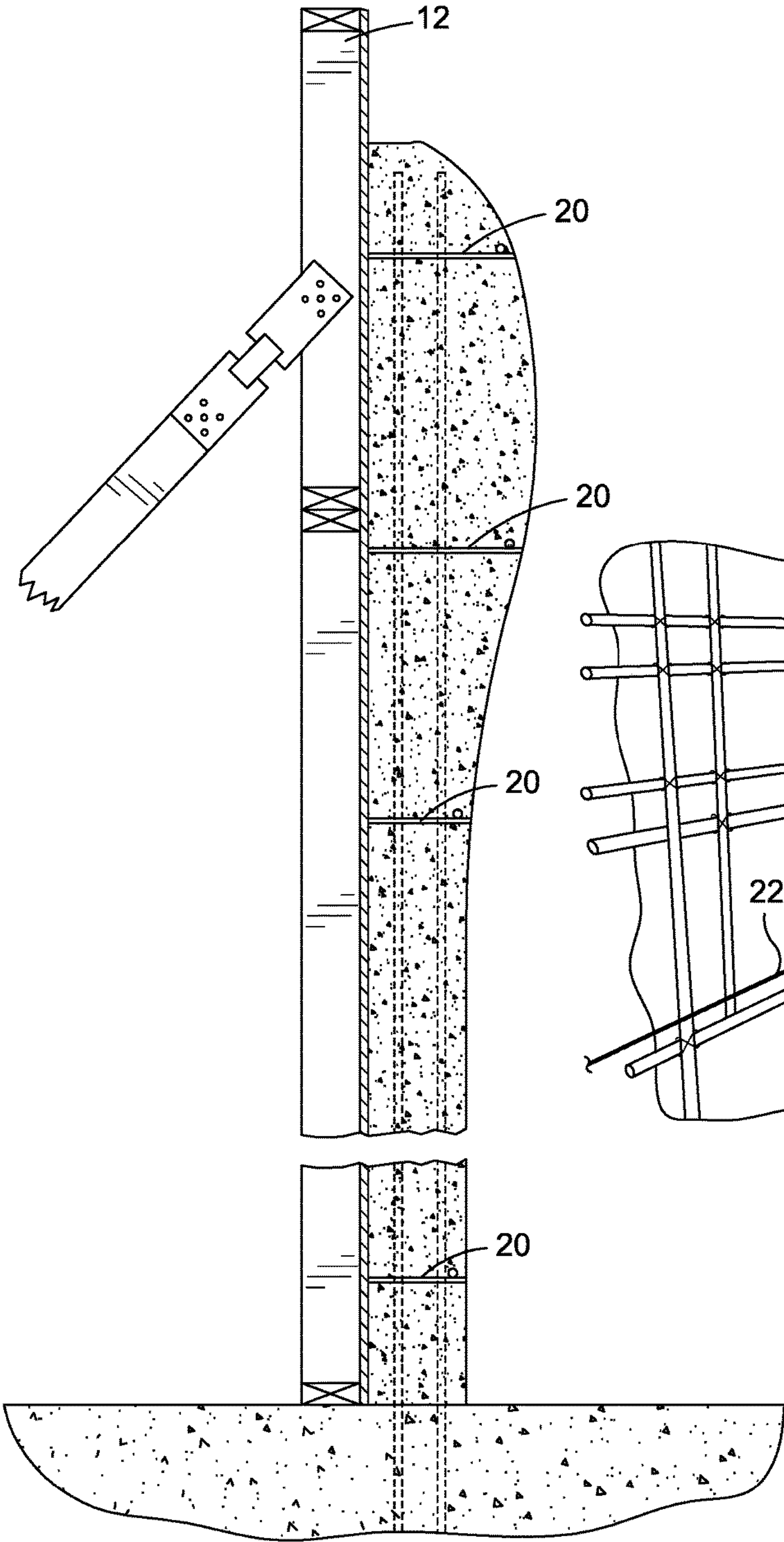
FIG. 1 (Prior Art)
