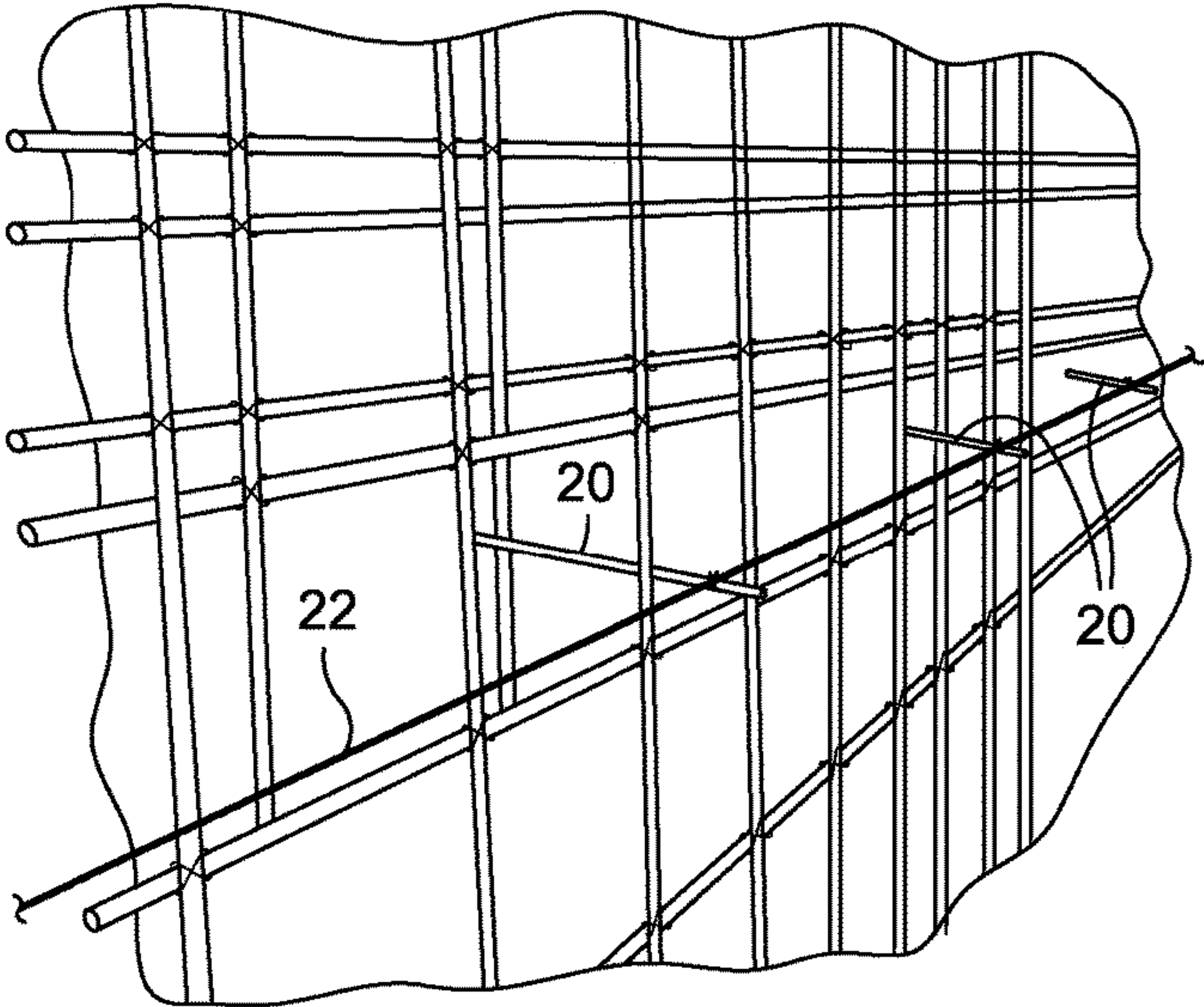
FIG. 2 (Prior Art)
