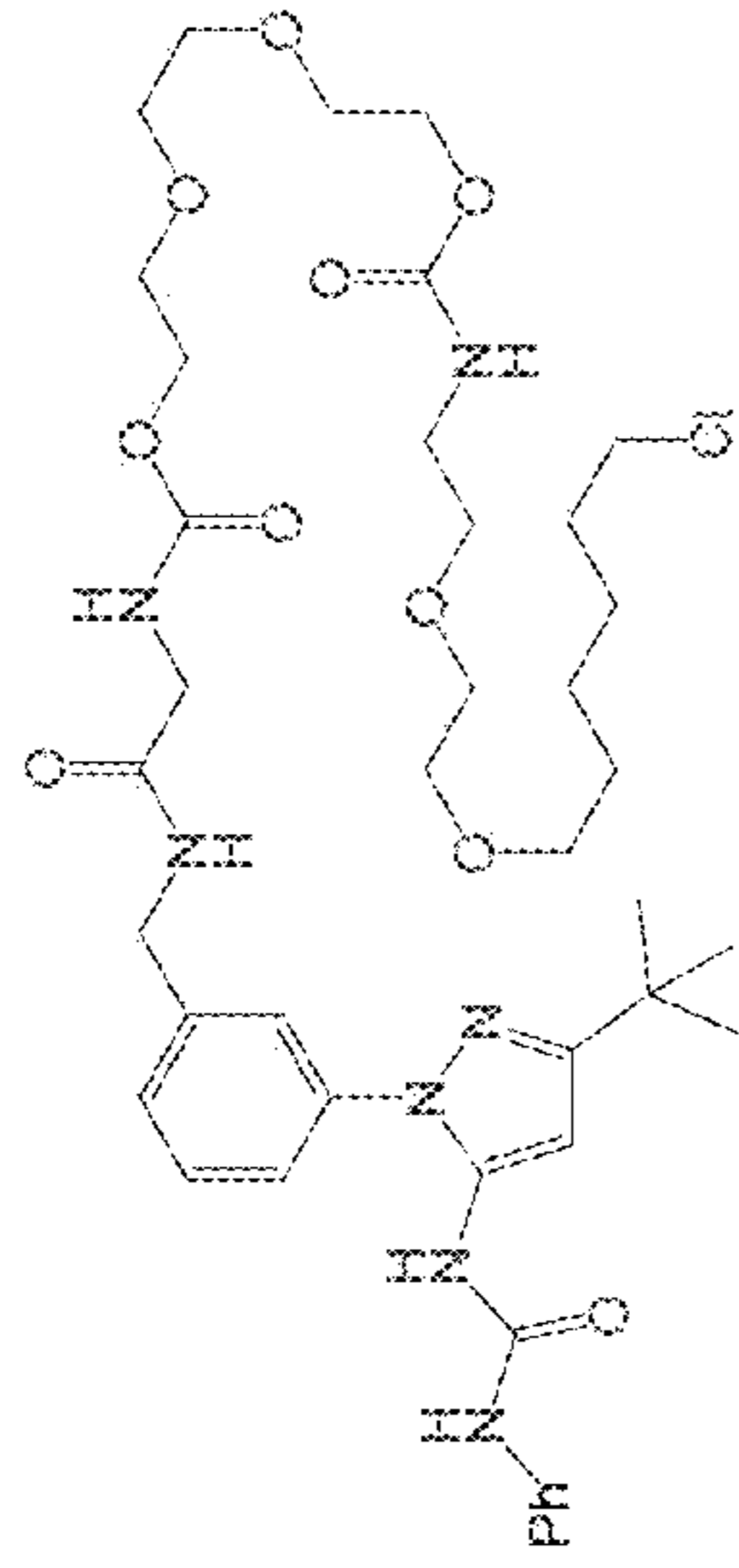
PBI-4834 (BIRB Carbamate Chloroalkane)
