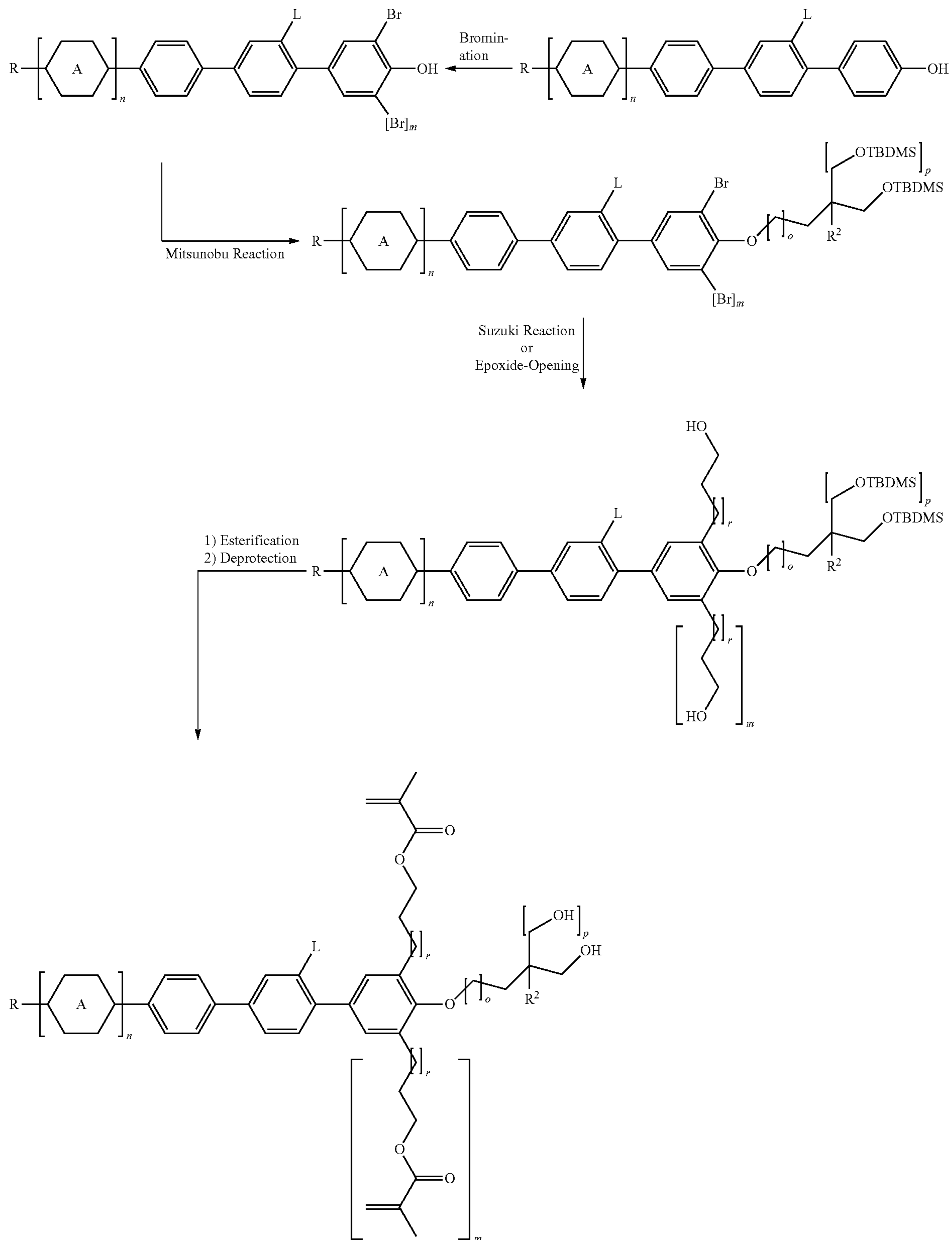
Scheme 2
