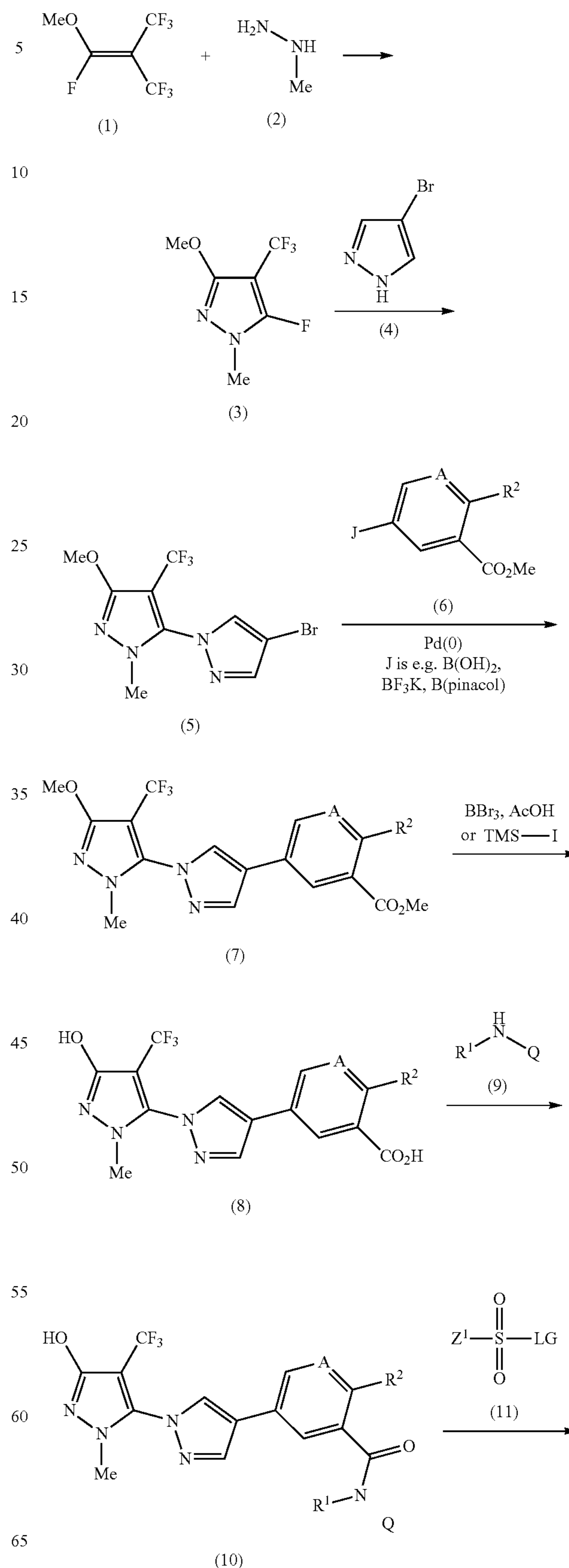
Scheme 1
