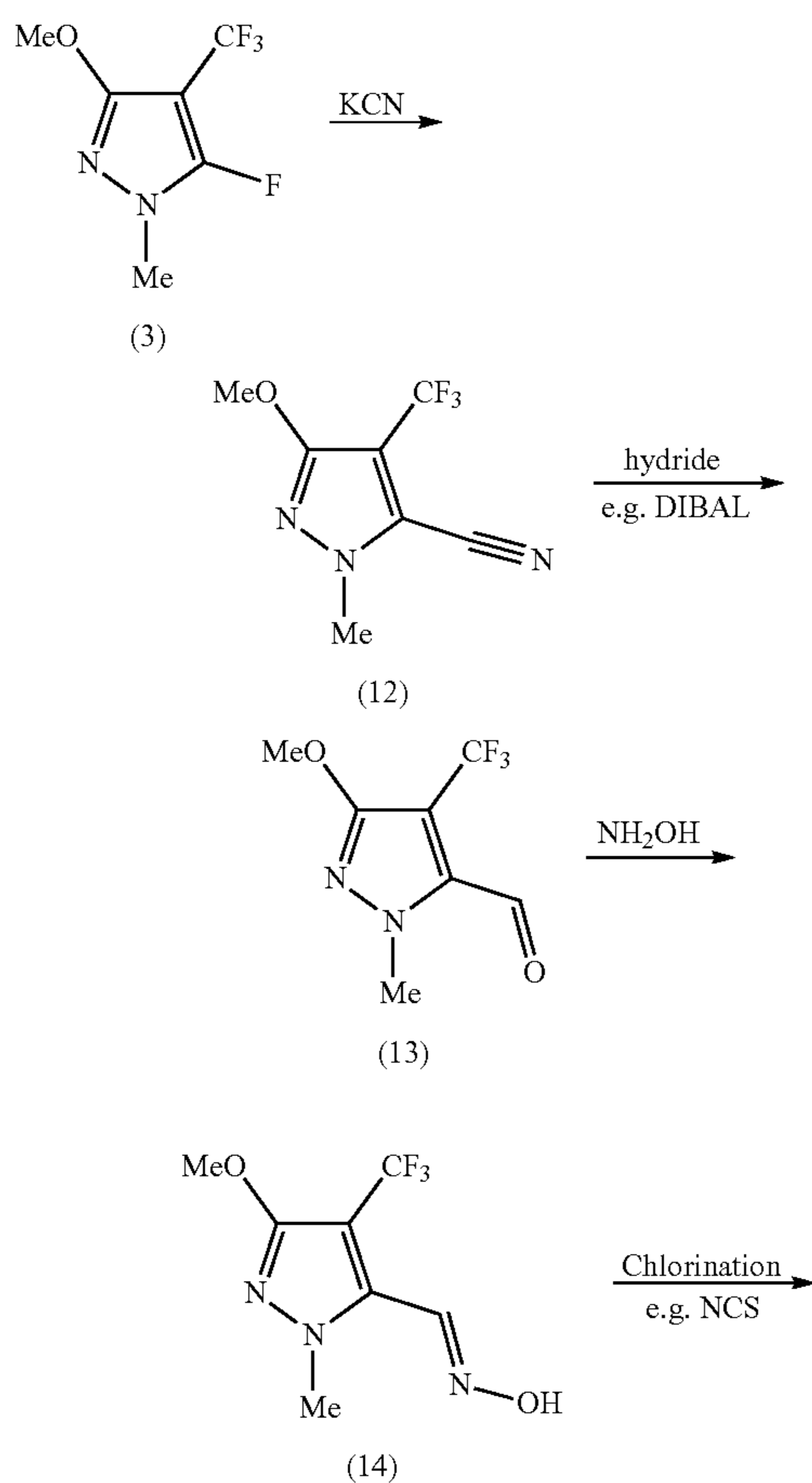
Scheme 2
