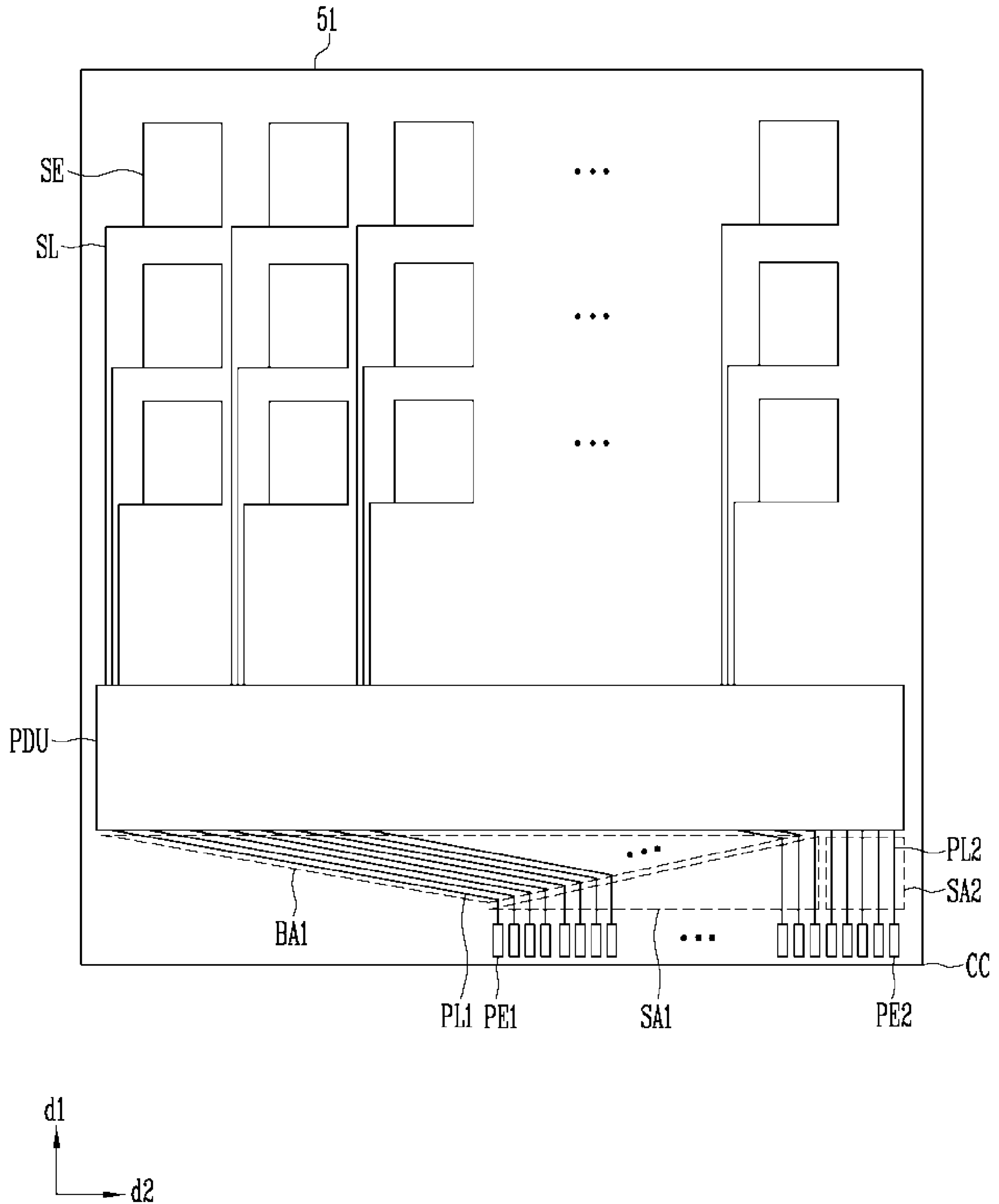
FIG. 3 (Related Art)
