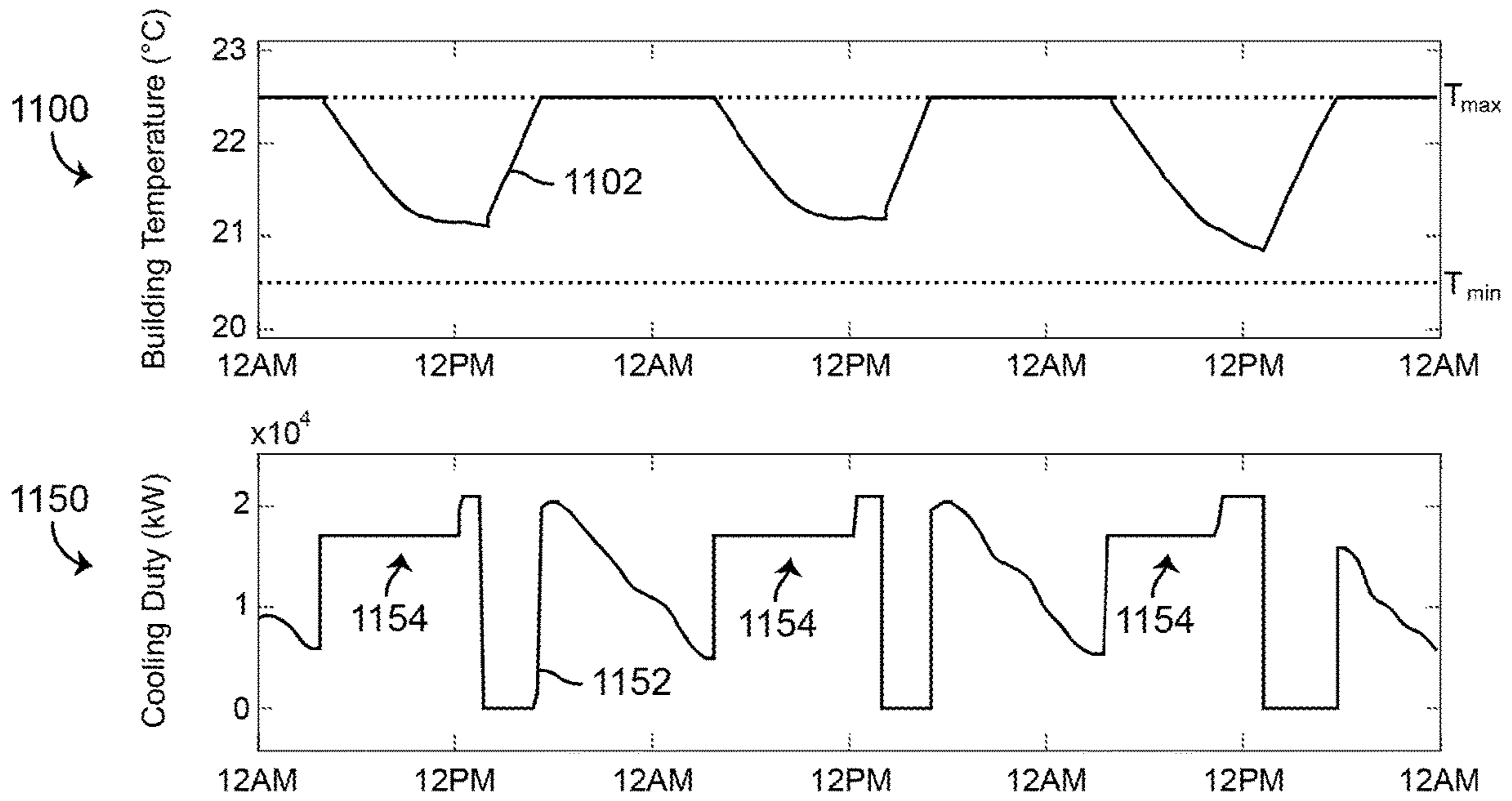
High-Level Optimization Result (With Airside Power Consumption Model)
