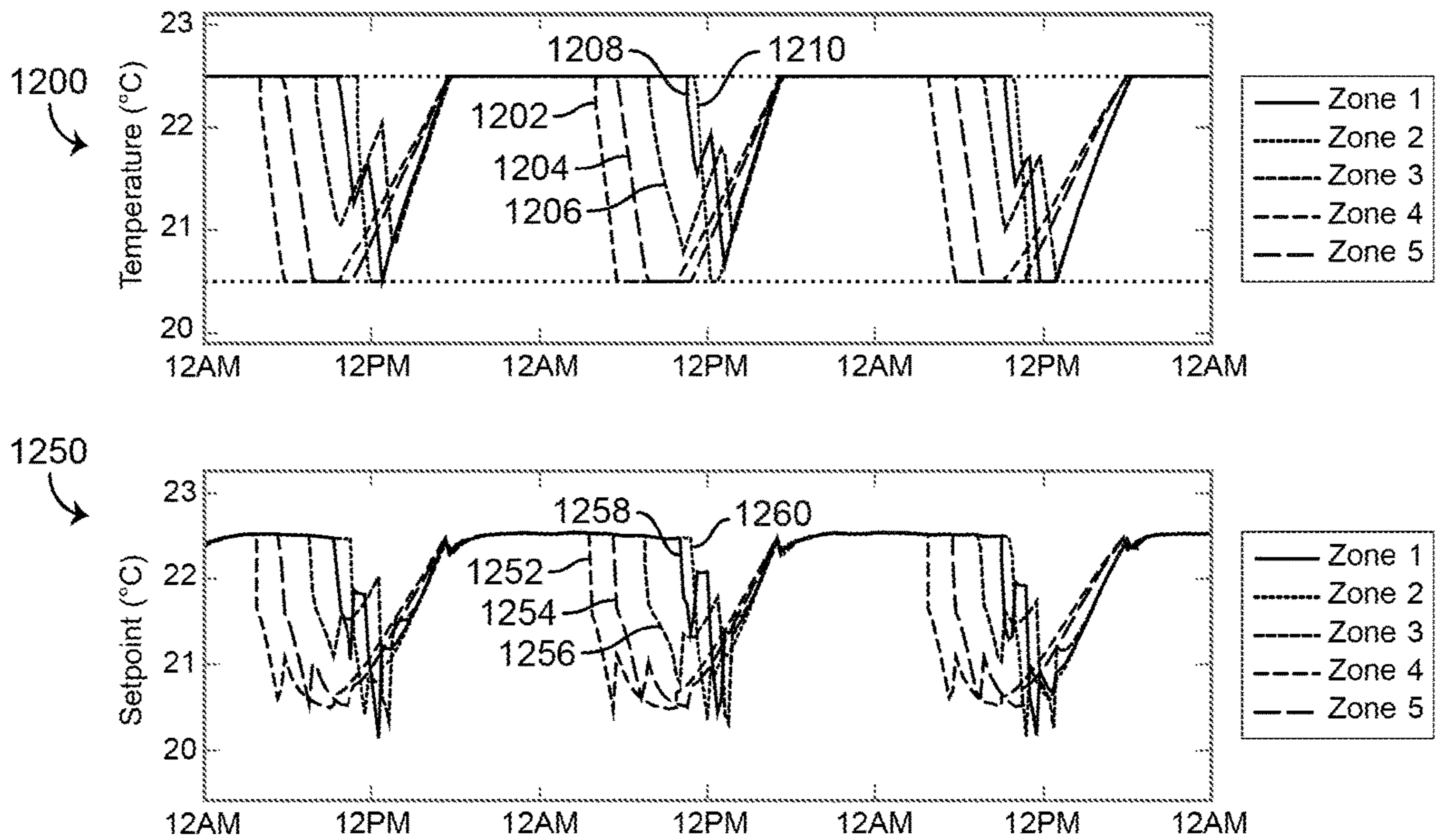
Low-Level Airside Optimization Result
