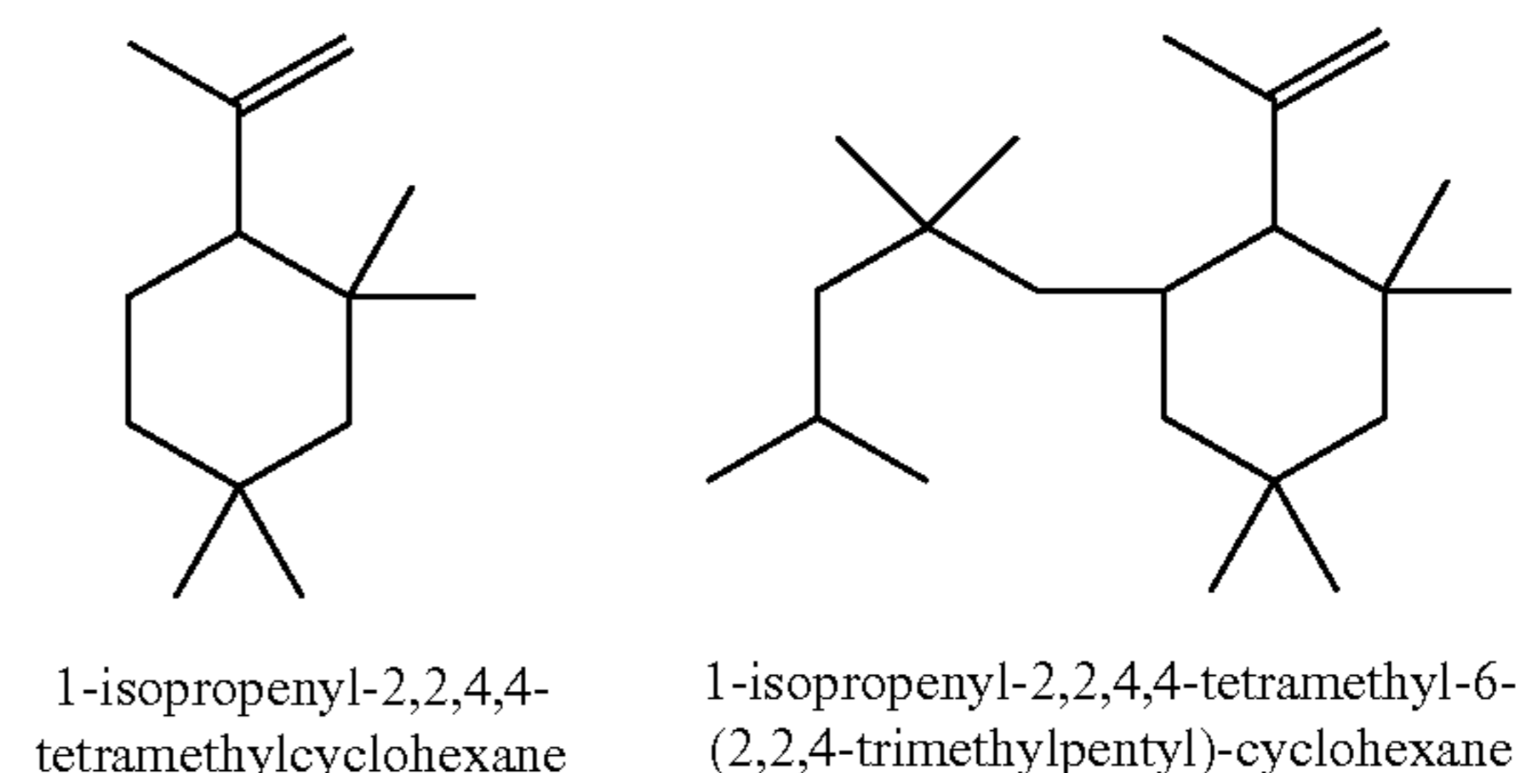
Scheme 1 - Molecular Structures of Cyclic Oligomers
