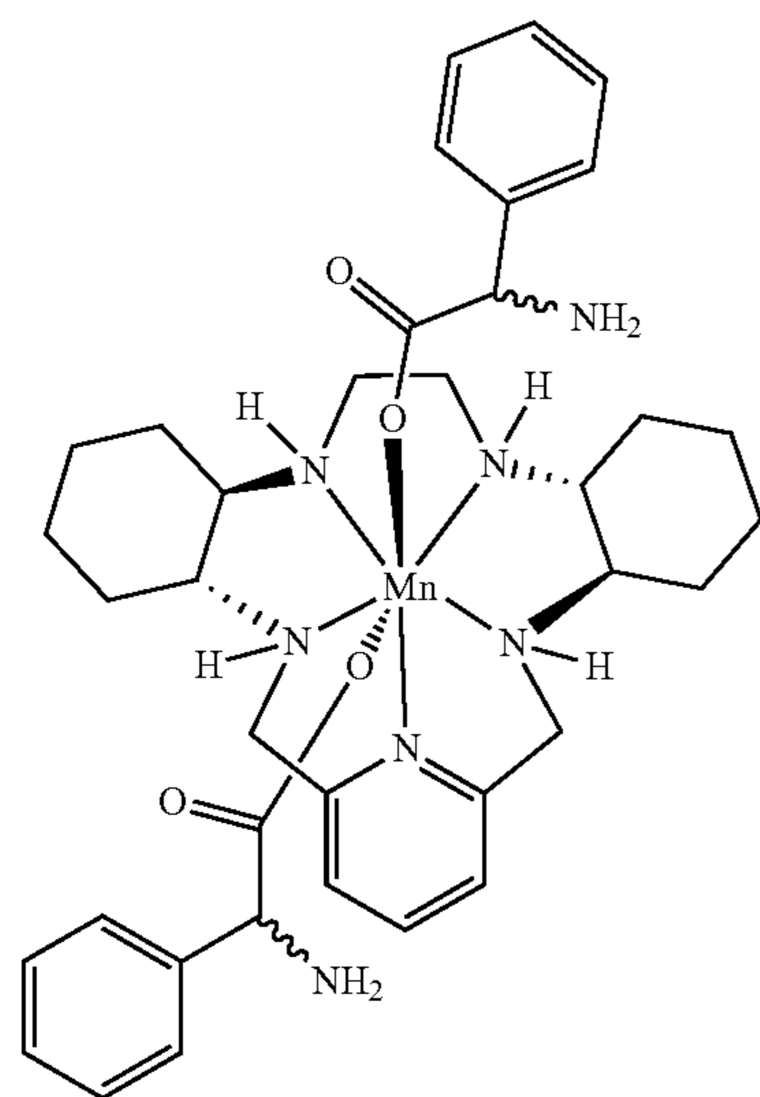
[Bis-(rac)-Phenylglycinato(GC4403)] \text{C}_{37}\text{H}_{51}\text{MnN}_7\text{O}_4 MW 712.80
