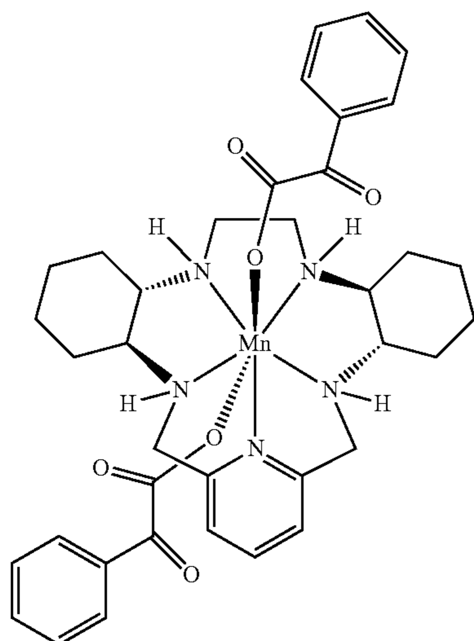
[Bis-Phenylglyoxylato(GC4419)] C_{37}H_{45}MnN_5O_6 MW 710.73
