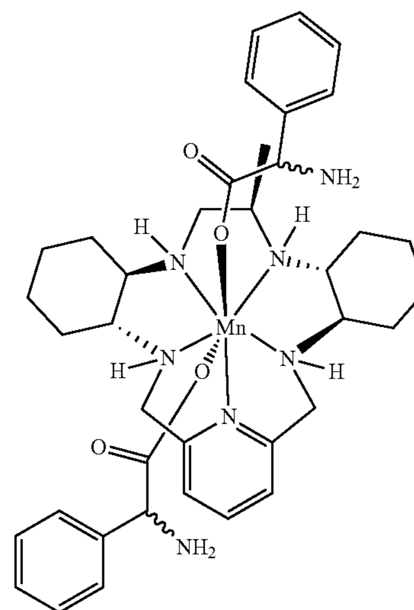
[Bis-(rac)-Phenylglycinato(GC4444)] C 38 H 53 MnN 7 O 4 MW 726.83
