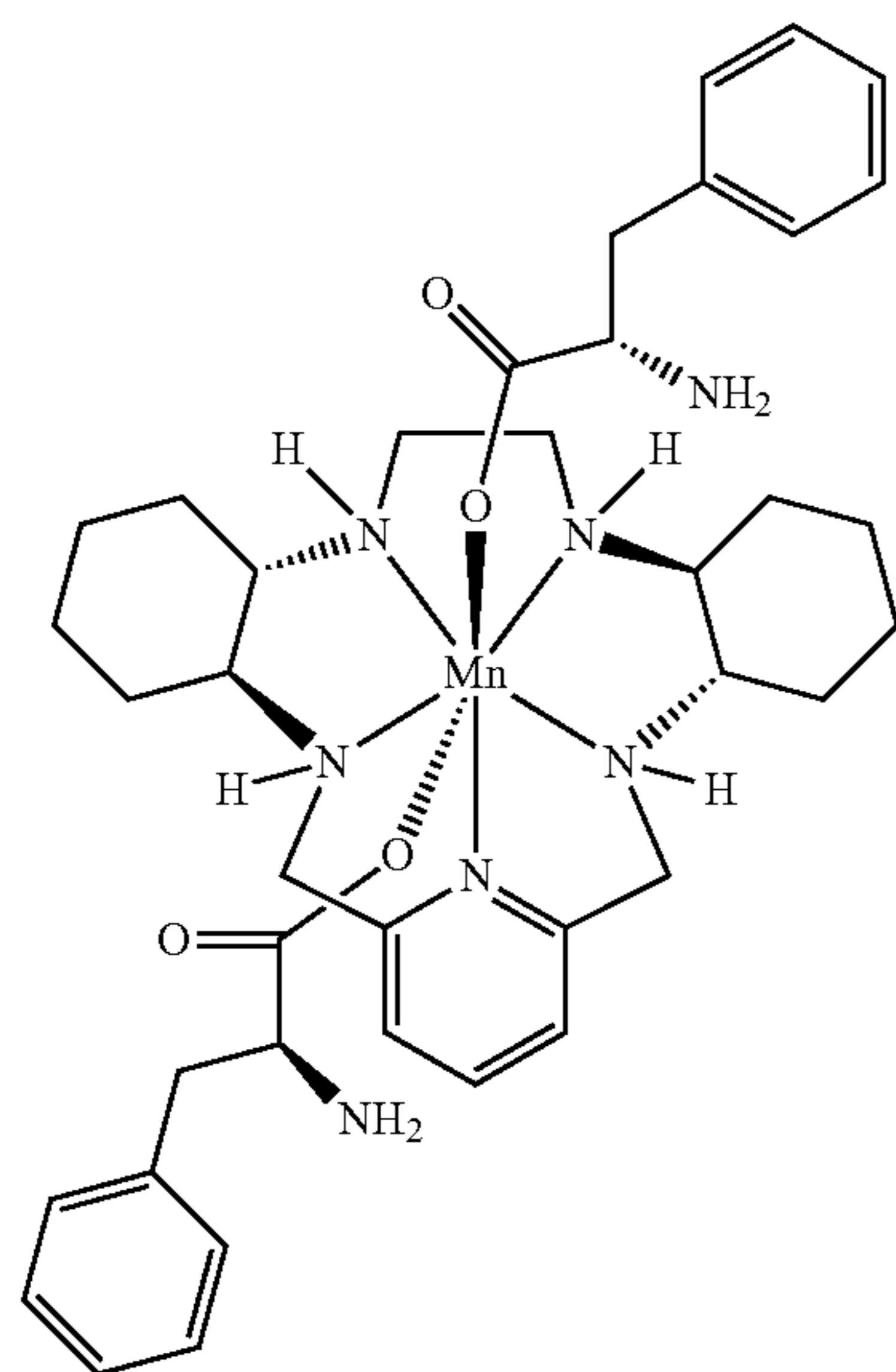
[Bis-(L)-Phenylalaninato(GC4419)] C_{39}H_{55}MnN_7O_4 MW 740.85
