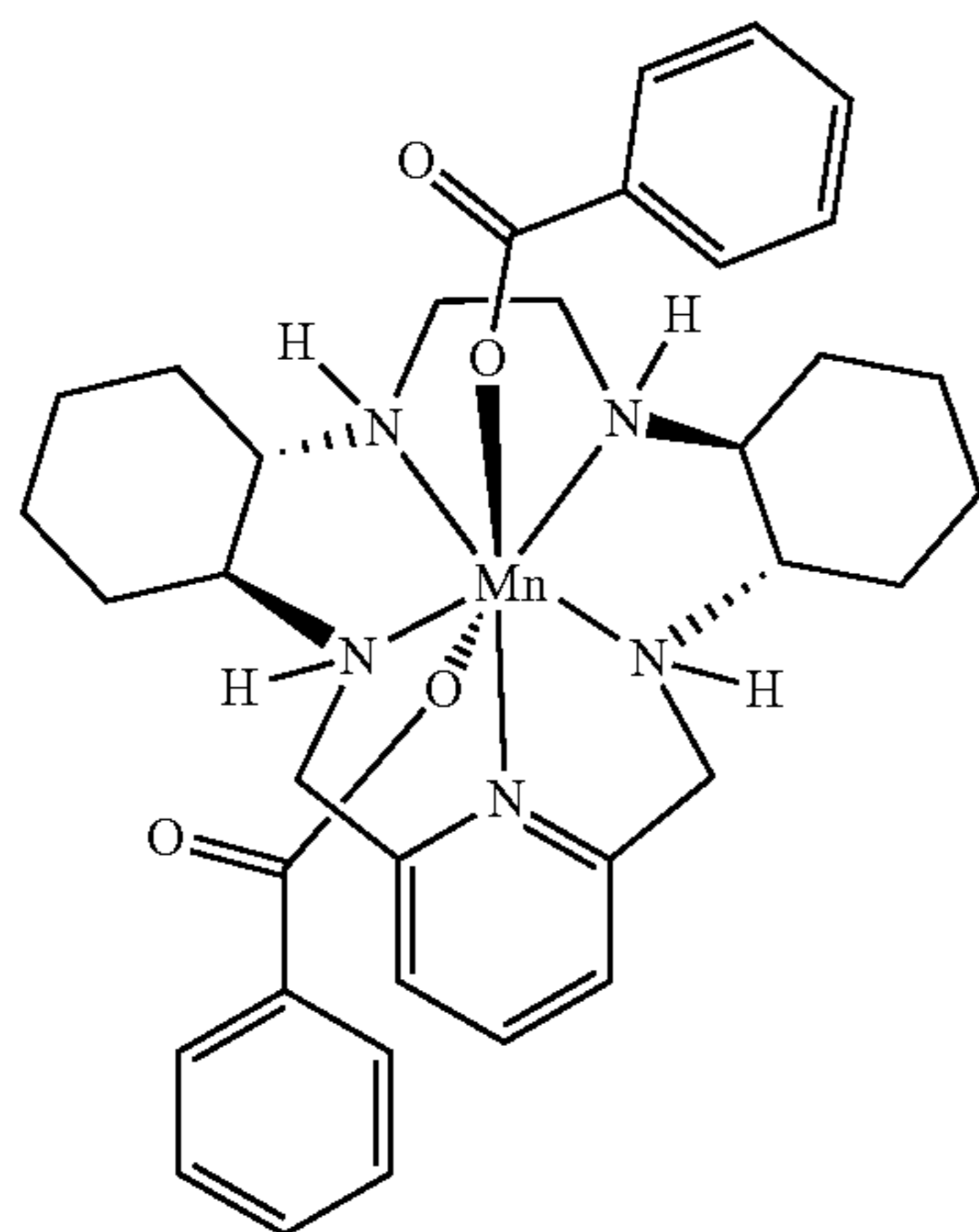
[Bis-Benzoato(GC4419)] C_{35}H_{45}MnN_5O_4 MW 654.71
