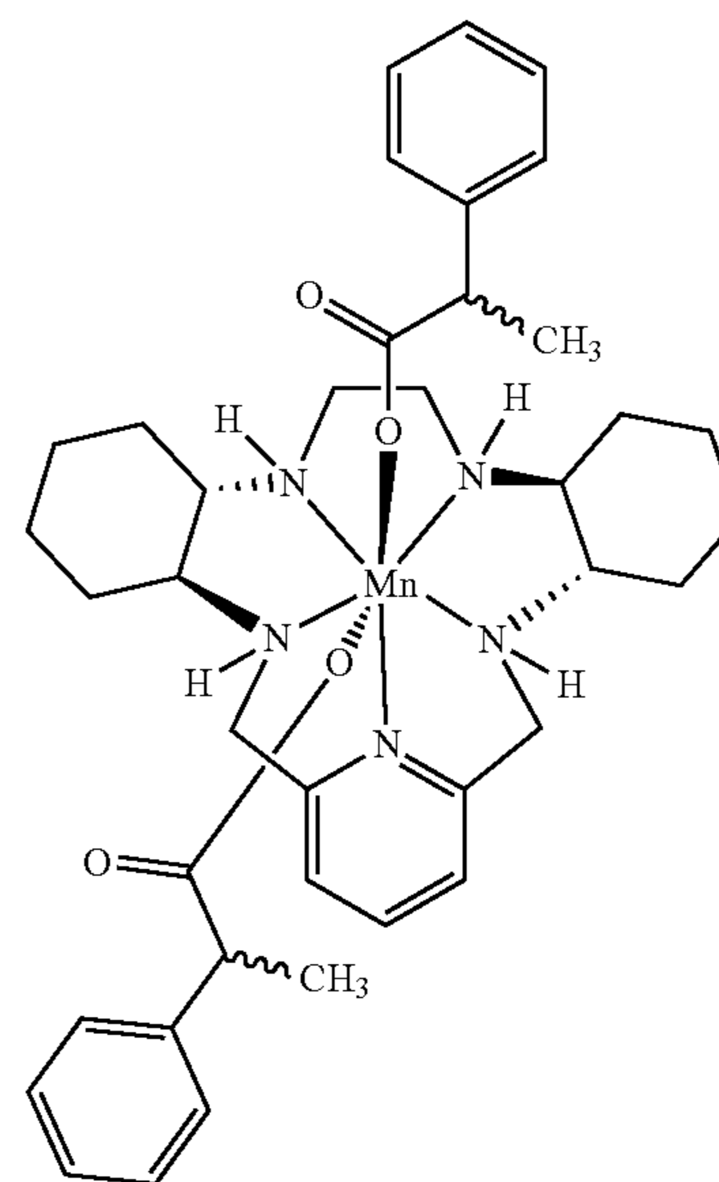
[Bis-(rac)-2-Phenylpropionato(GC4419)] C_{39}H_{53}MnN_5O_4 MW 710.82
