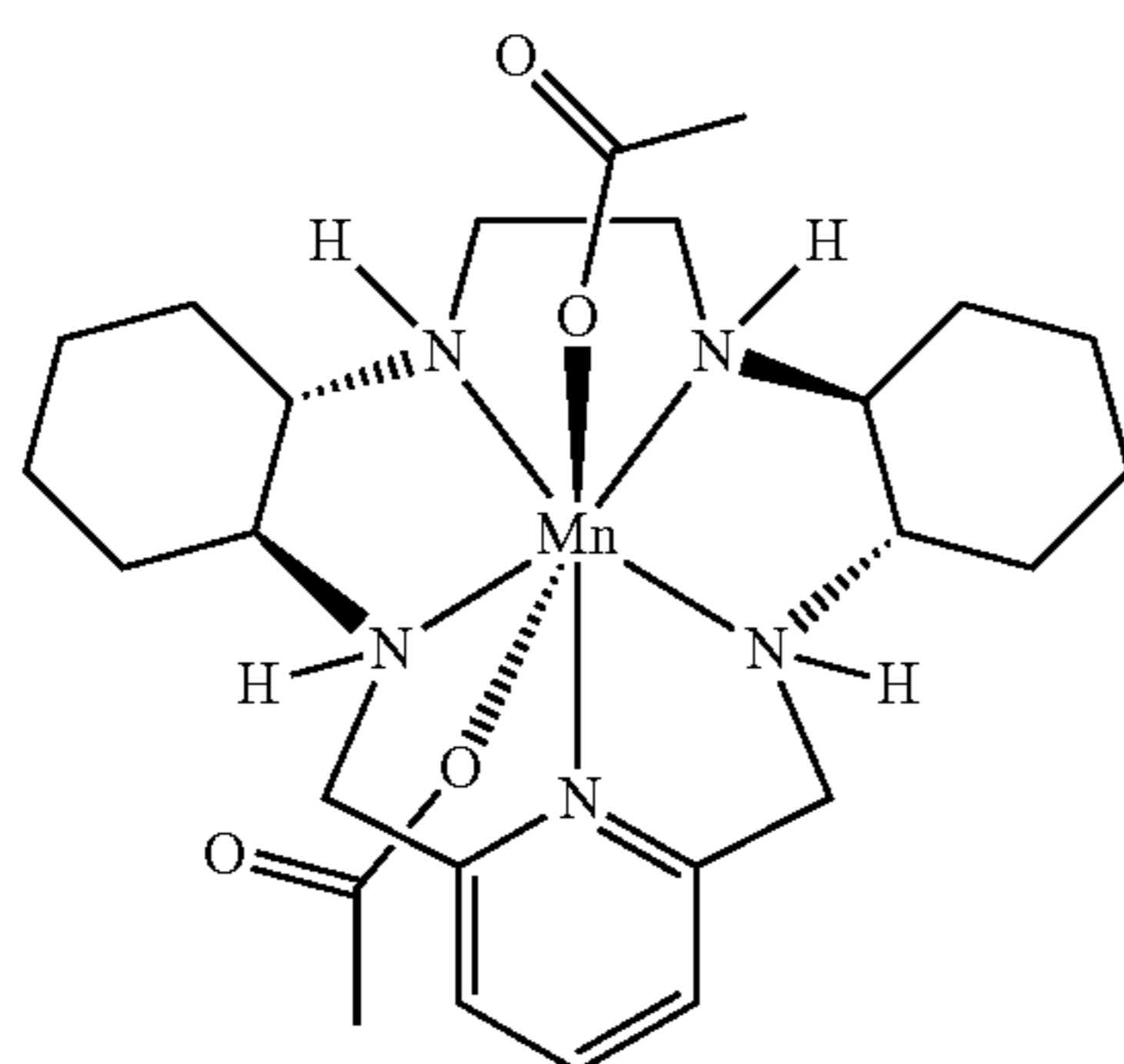
[Bis-Acetato(GC4419)] C 25 H 41 MnN 5 O 4 MW 530.57
