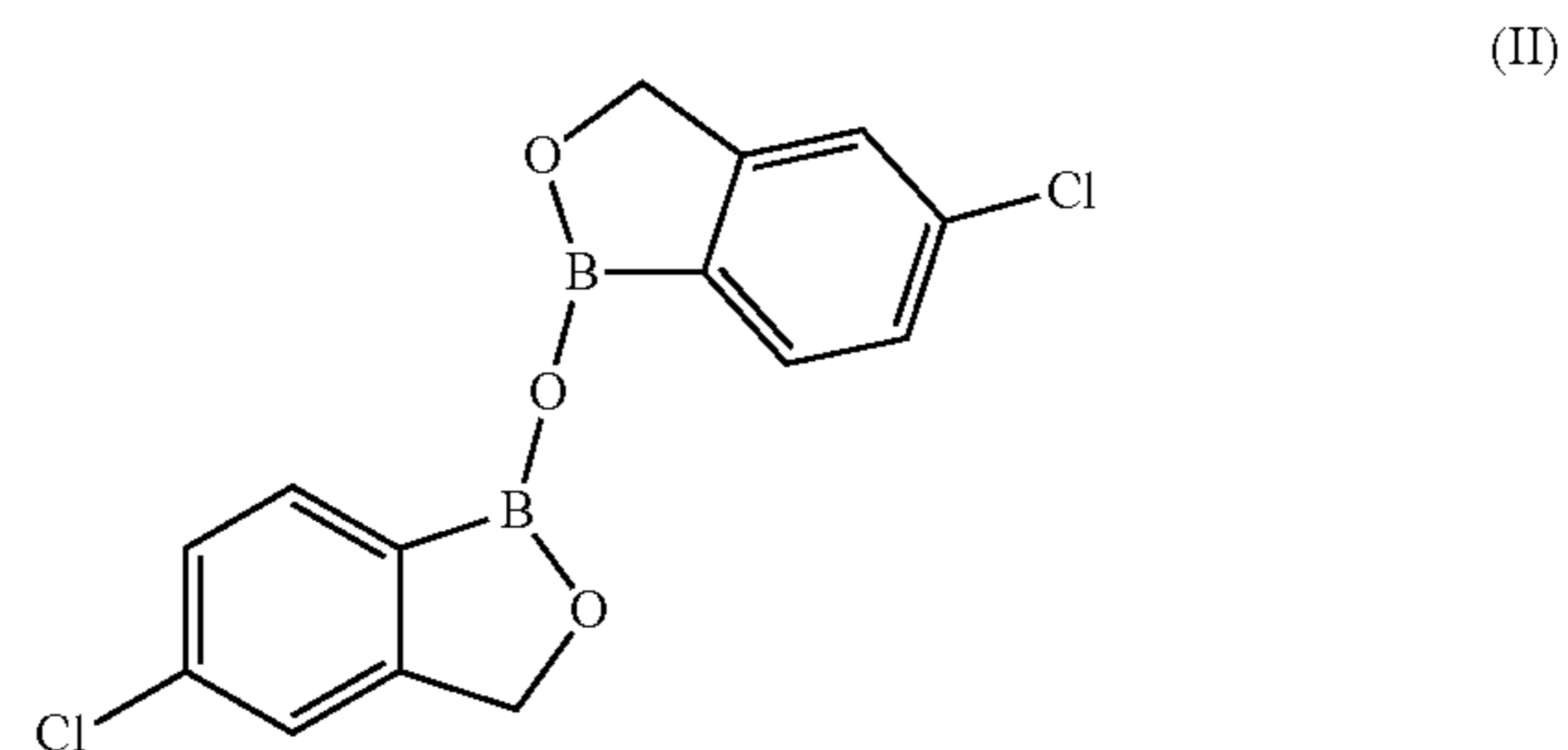
1,1'-oxybis(5-chloro-1,3-dihydrobenzo[c][1,2]oxaborole).
