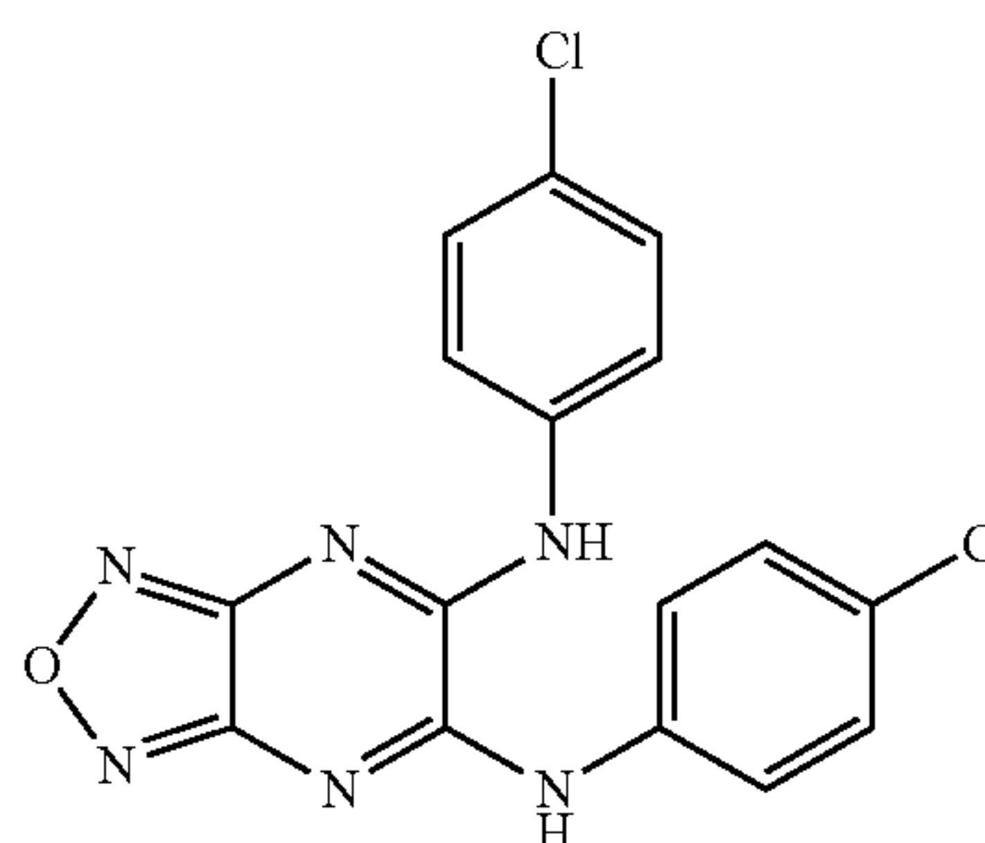
(4-chlorophenyl){6-[(4-chlorophenyl)amino] (1,2,5-oxadiazolo[3,4-e]pyrazin-5-yl)}amine
