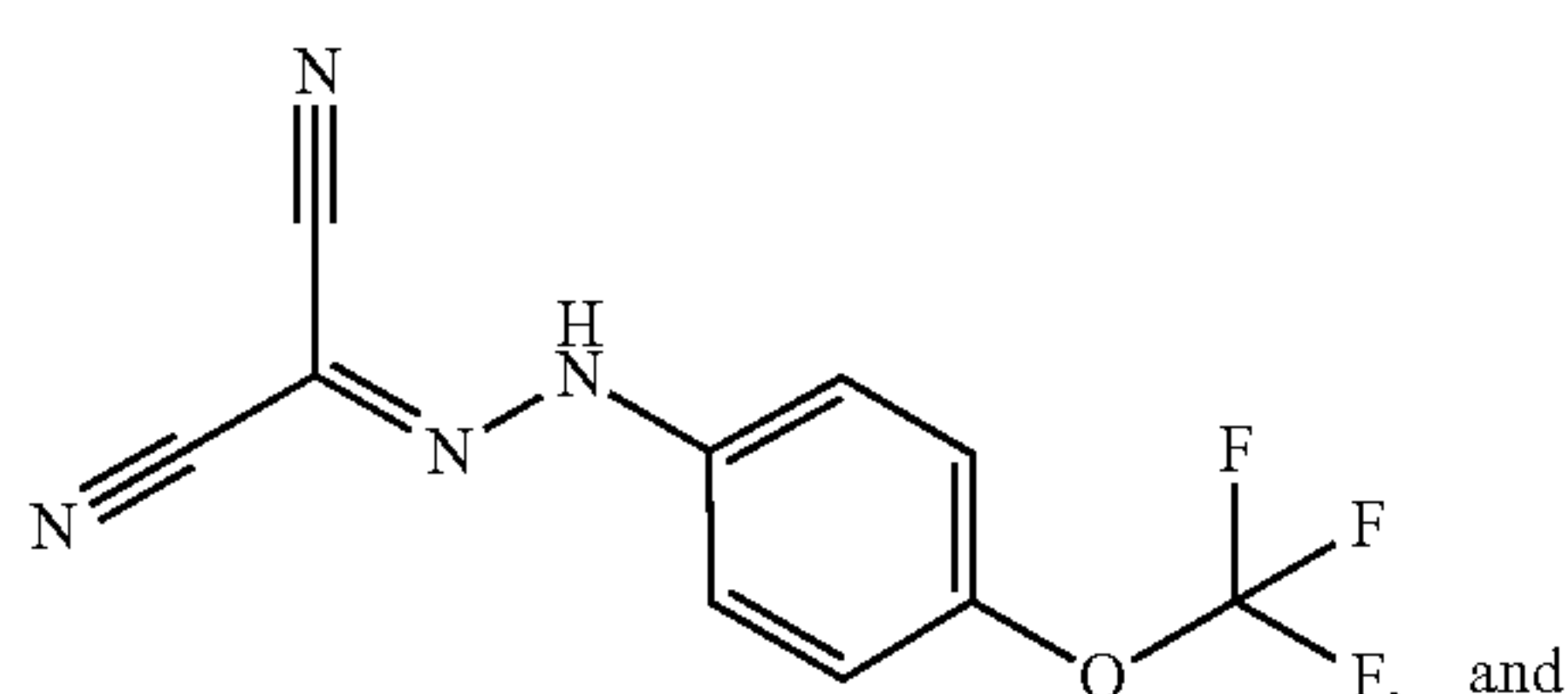
Carbonyl cyanide p-trifluoromethoxyphenylhydrazone
