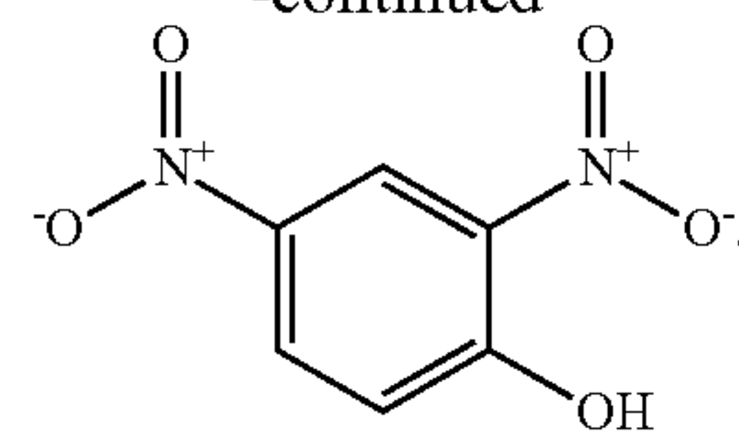
2,4-dinitrophenol
