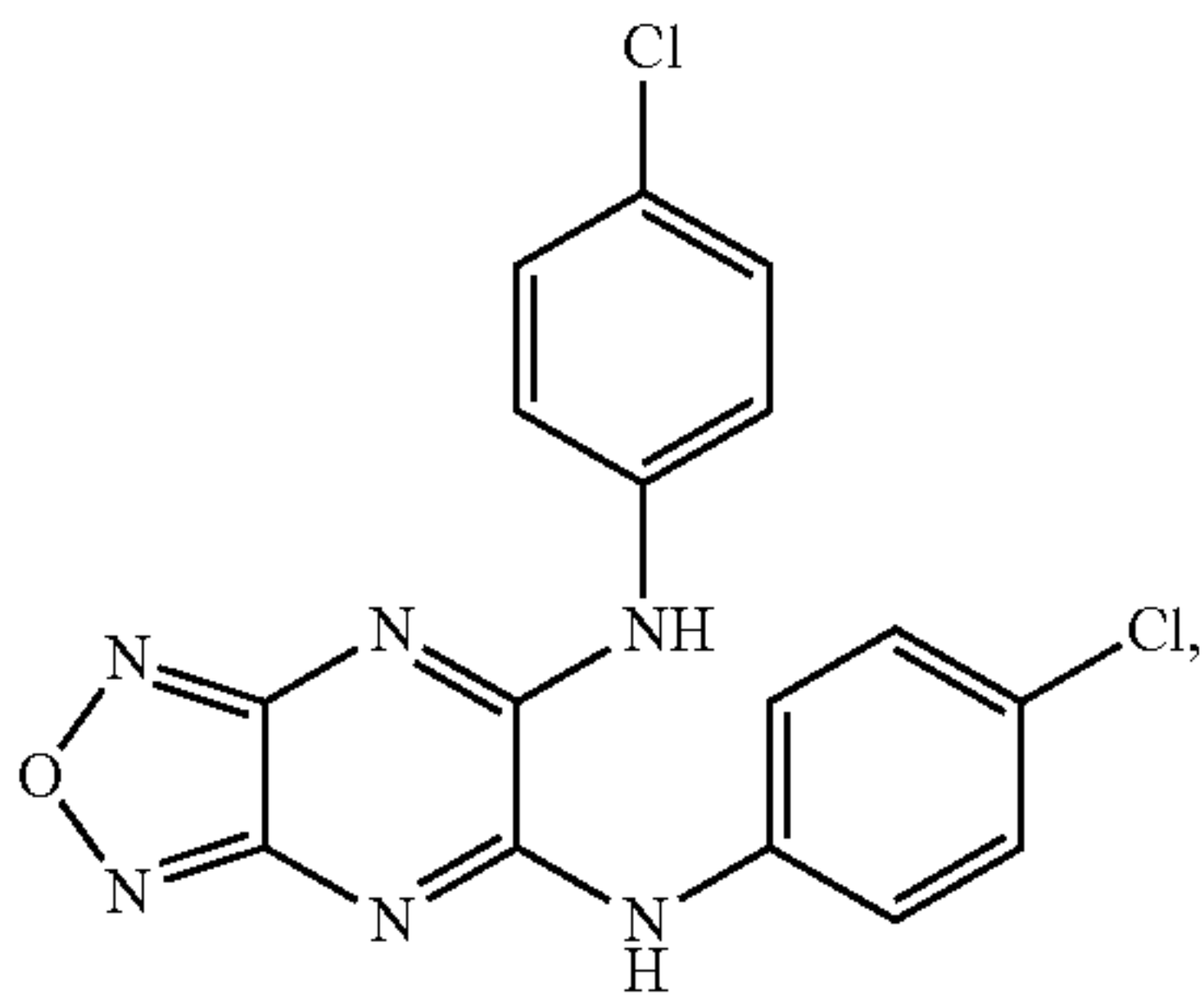
(4-chlorophenyl){6-[(4-chlorophenyl)amino] (1,2,5-oxadiazolo[3,4-e]pyrazin-5-yl)}amine
