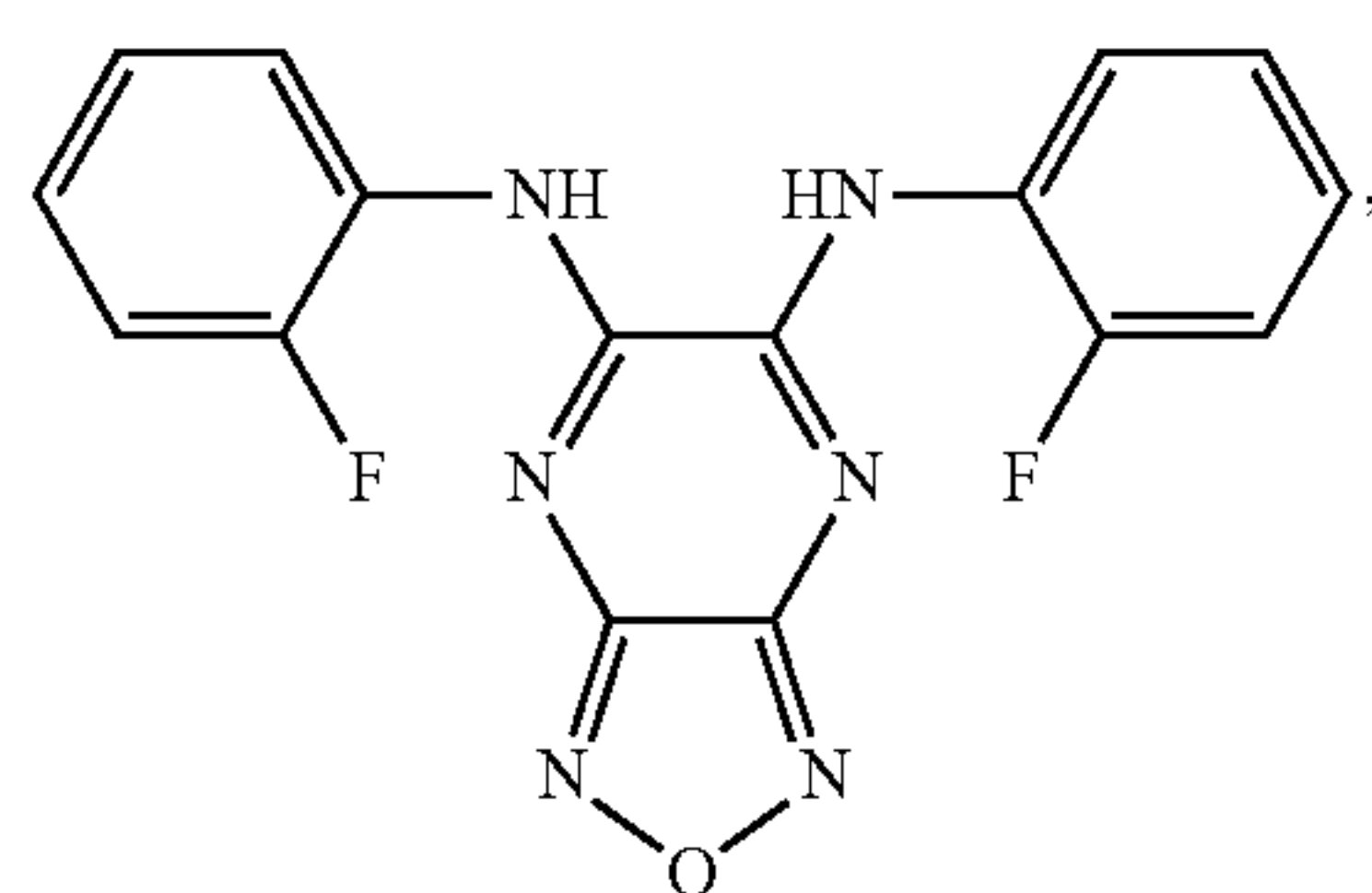
(2-fluorophenyl){6-[(2-fluorophenyl)amino] (1,2,5-oxadiazolo[3,4-e]pyrazin-5-yl)}amine
