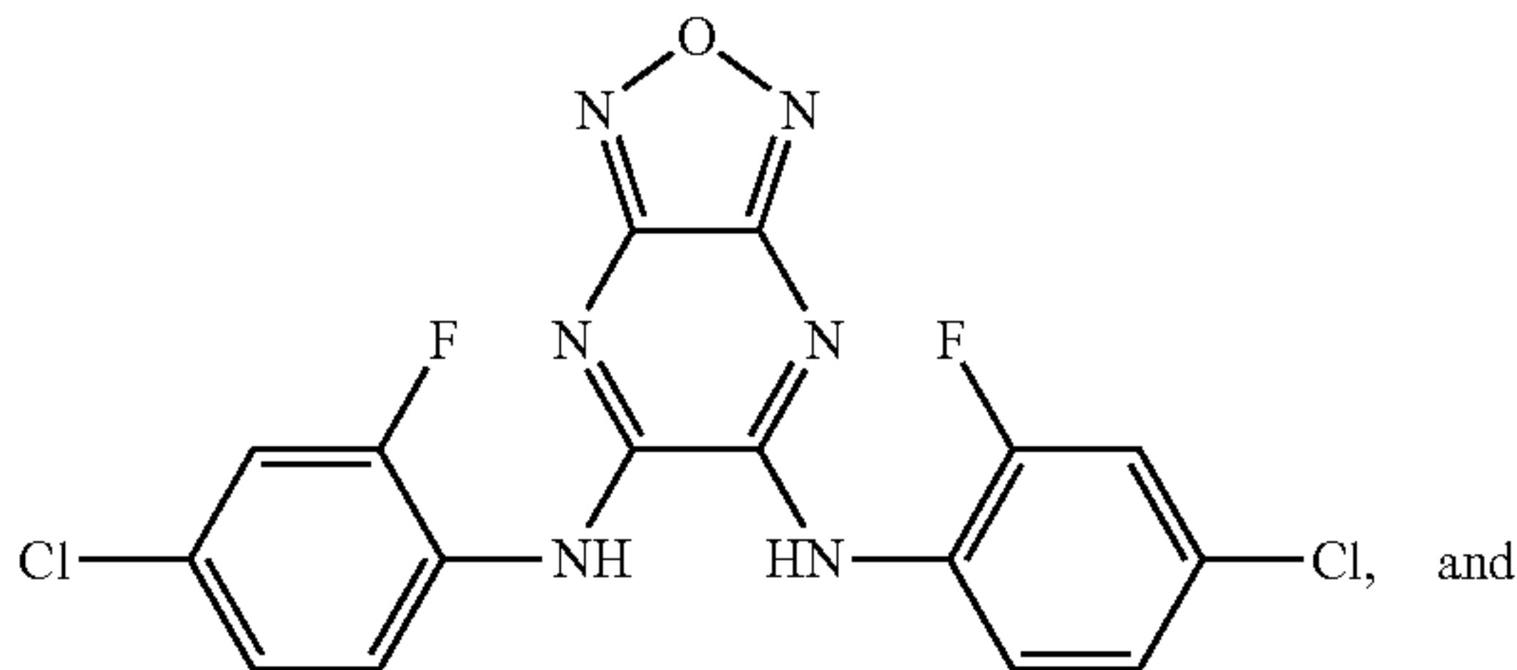
BAM15F
