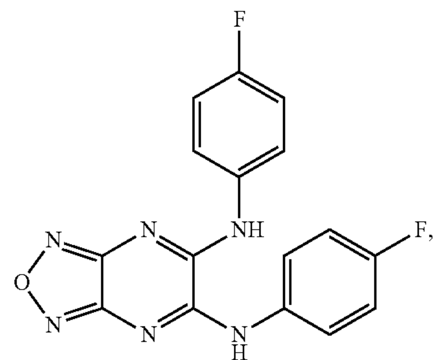
(4-fluorophenyl){6-[(4-fluorophenyl)amino] (1,2,5-oxadiazolo[3,4-e]pyrazin-5-yl)} amine
