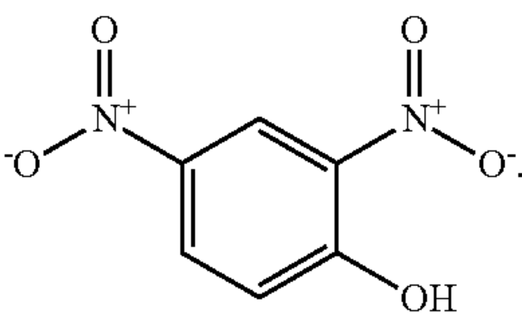
2,4-dinitrophenol
