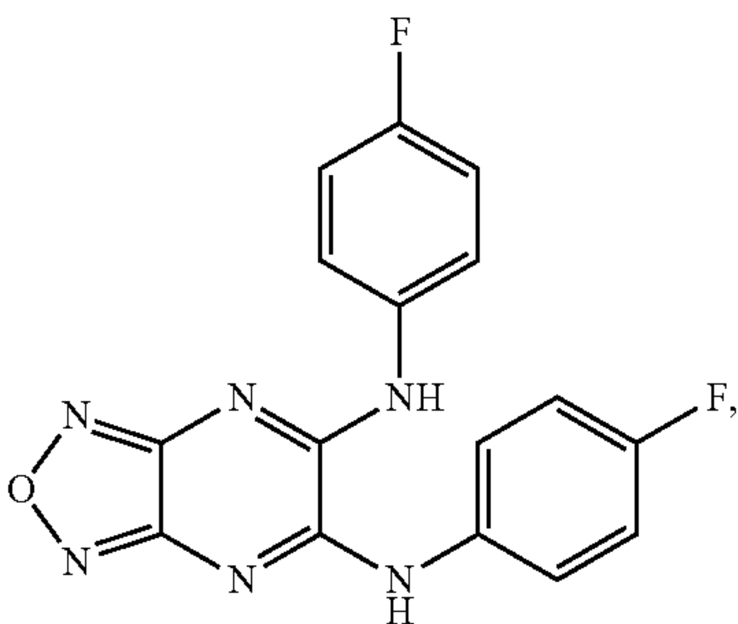
(4-fluorophenyl){6-[(4-fluorophenyl)amino] (1,2,5-oxadiazolo[3,4-e]pyrazin-5-yl)} amine
