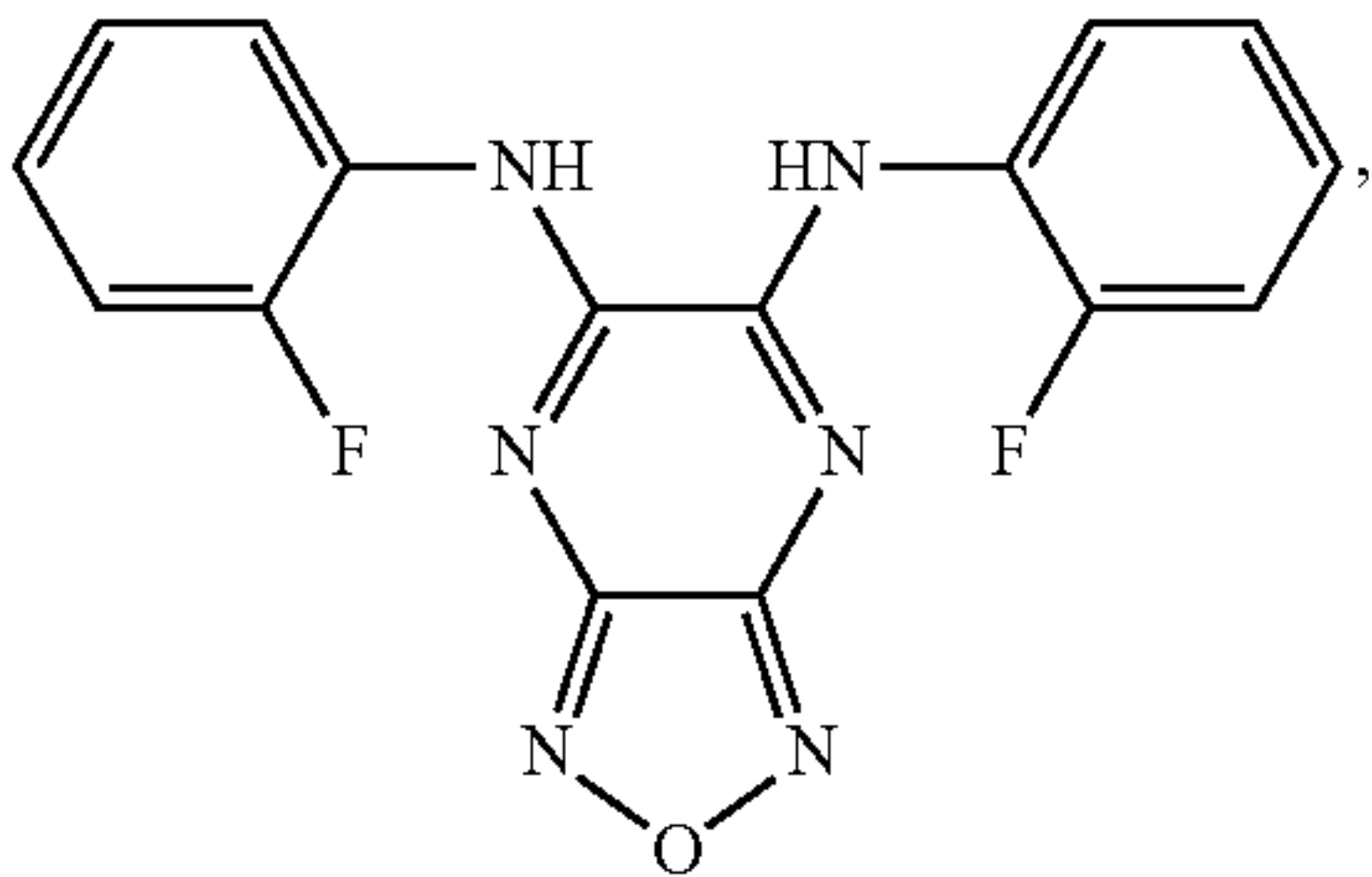
(2-fluorophenyl){6-[(2-fluorophenyl)amino] (1,2,5-oxadiazolo[3,4-e]pyrazin-5-yl)}amine
