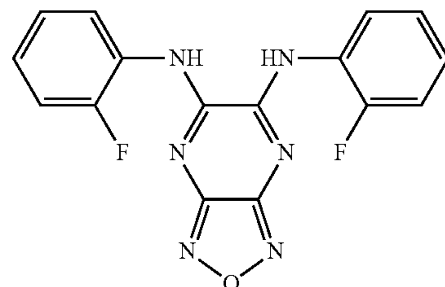
(2-fluorophenyl){6-[(2-fluorophenyl)amino] (1,2,5-oxadiazolo[3,4-e]pyrazin-5-yl)}amine
