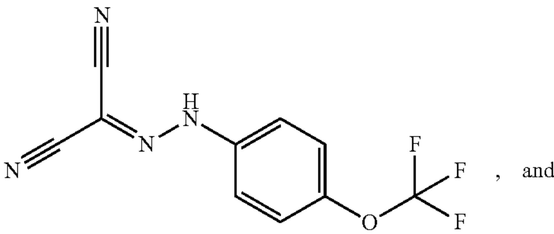
Carbonyl cyanide p-trifluoromethoxyphenylhydrazone FCCP
