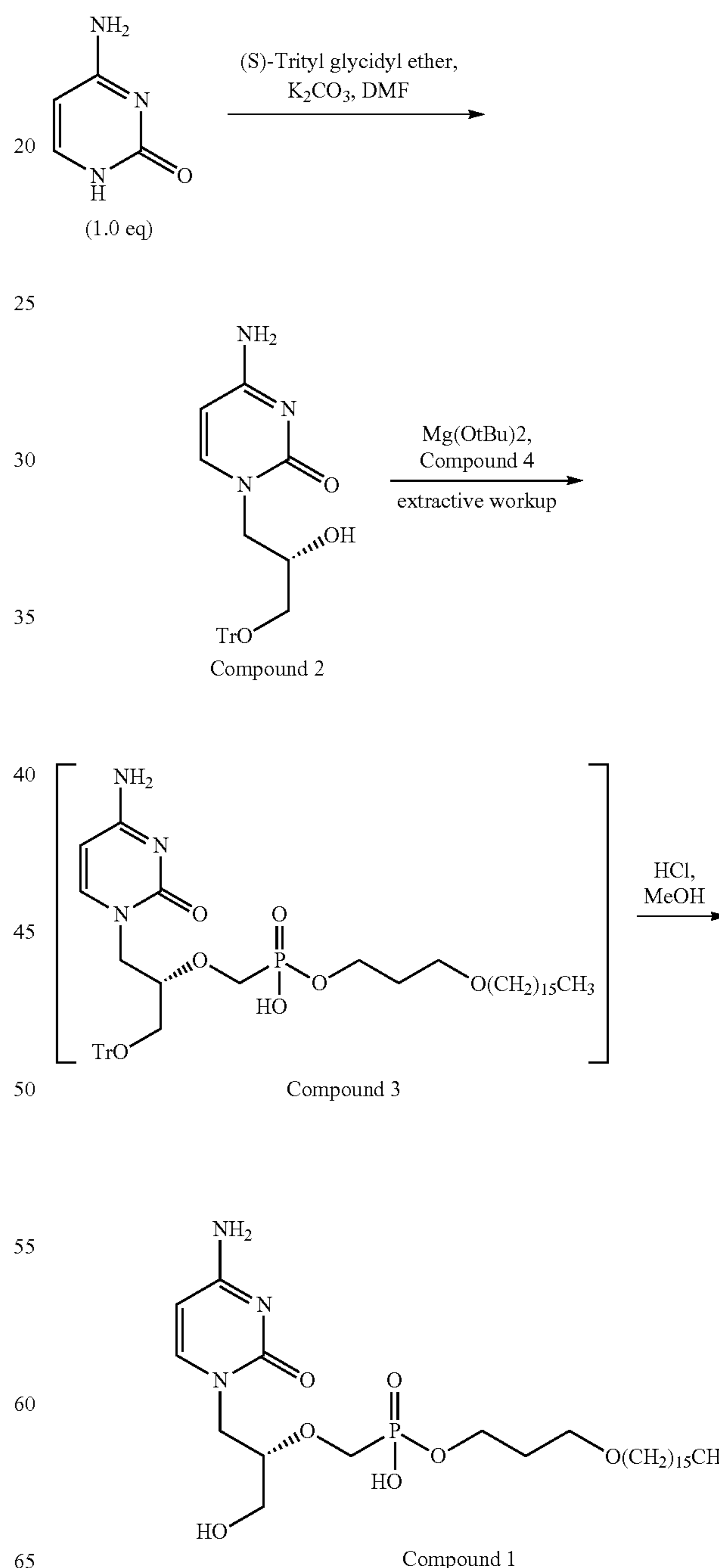
Scheme 1
