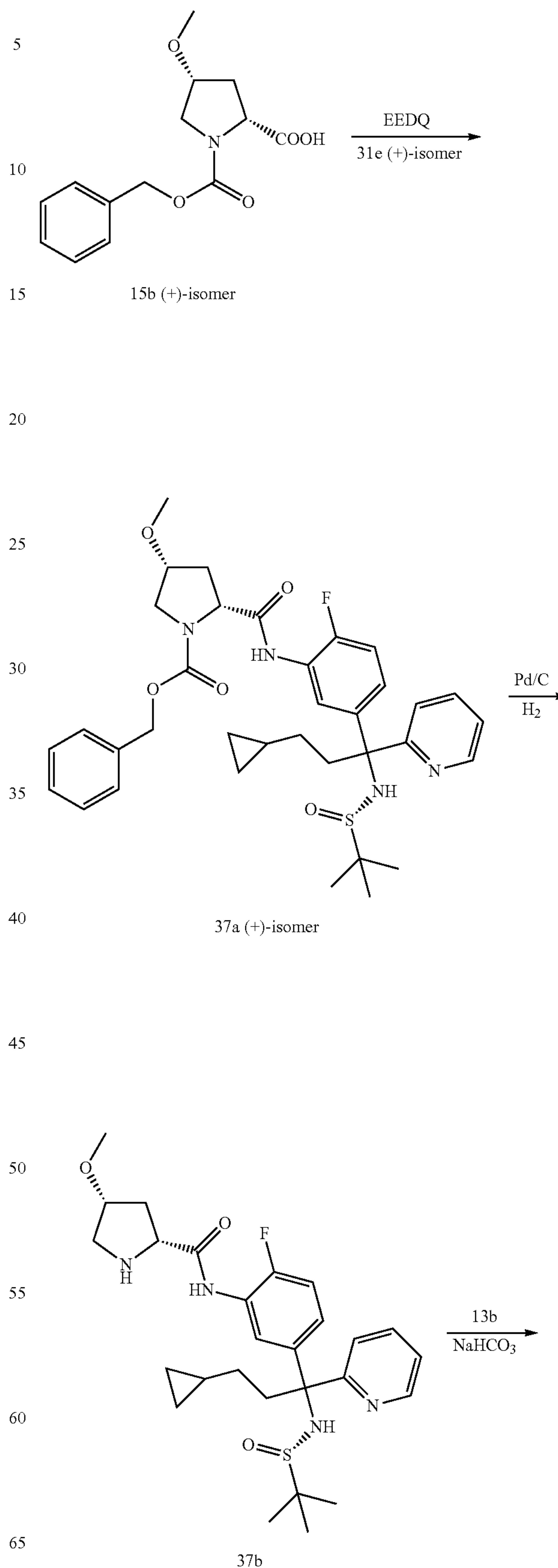
Scheme 37
