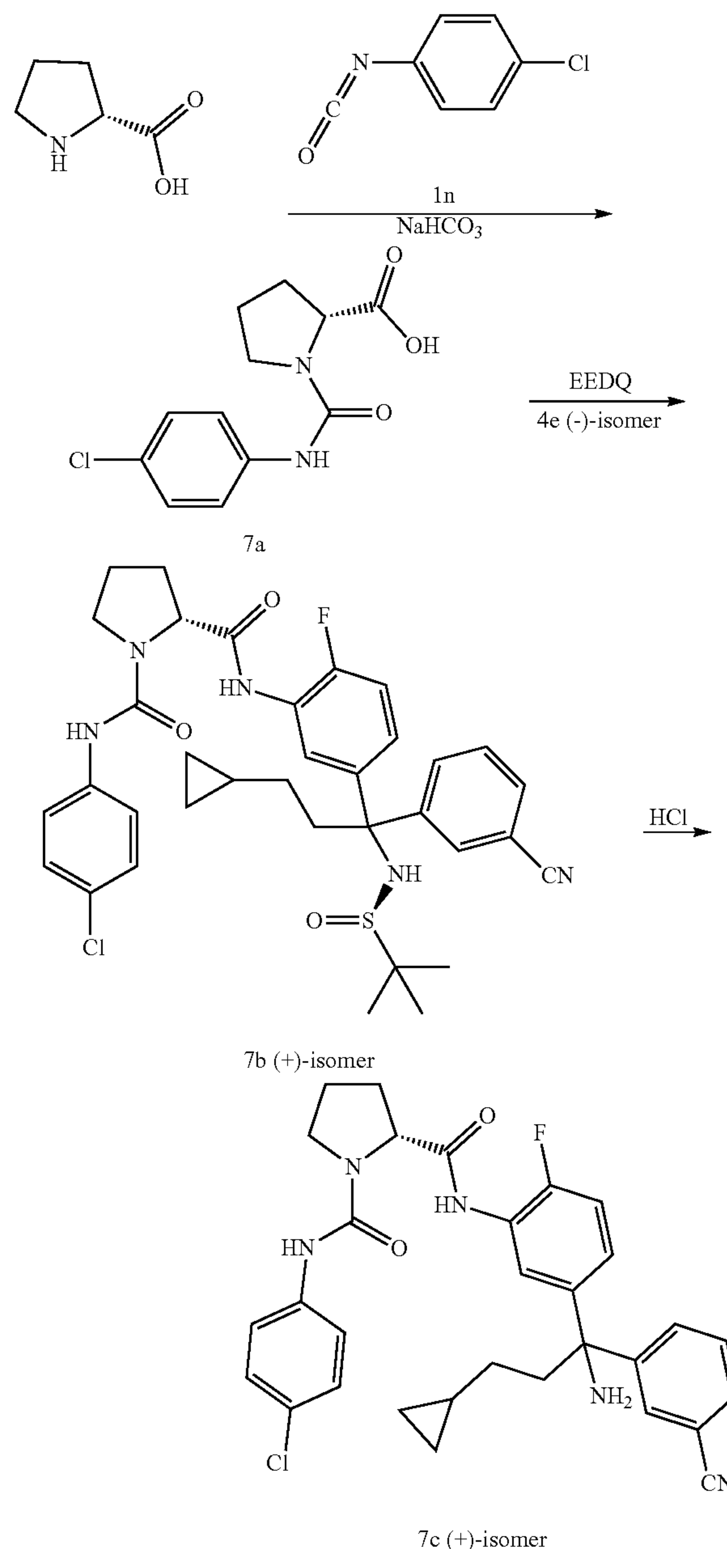
Scheme 7
