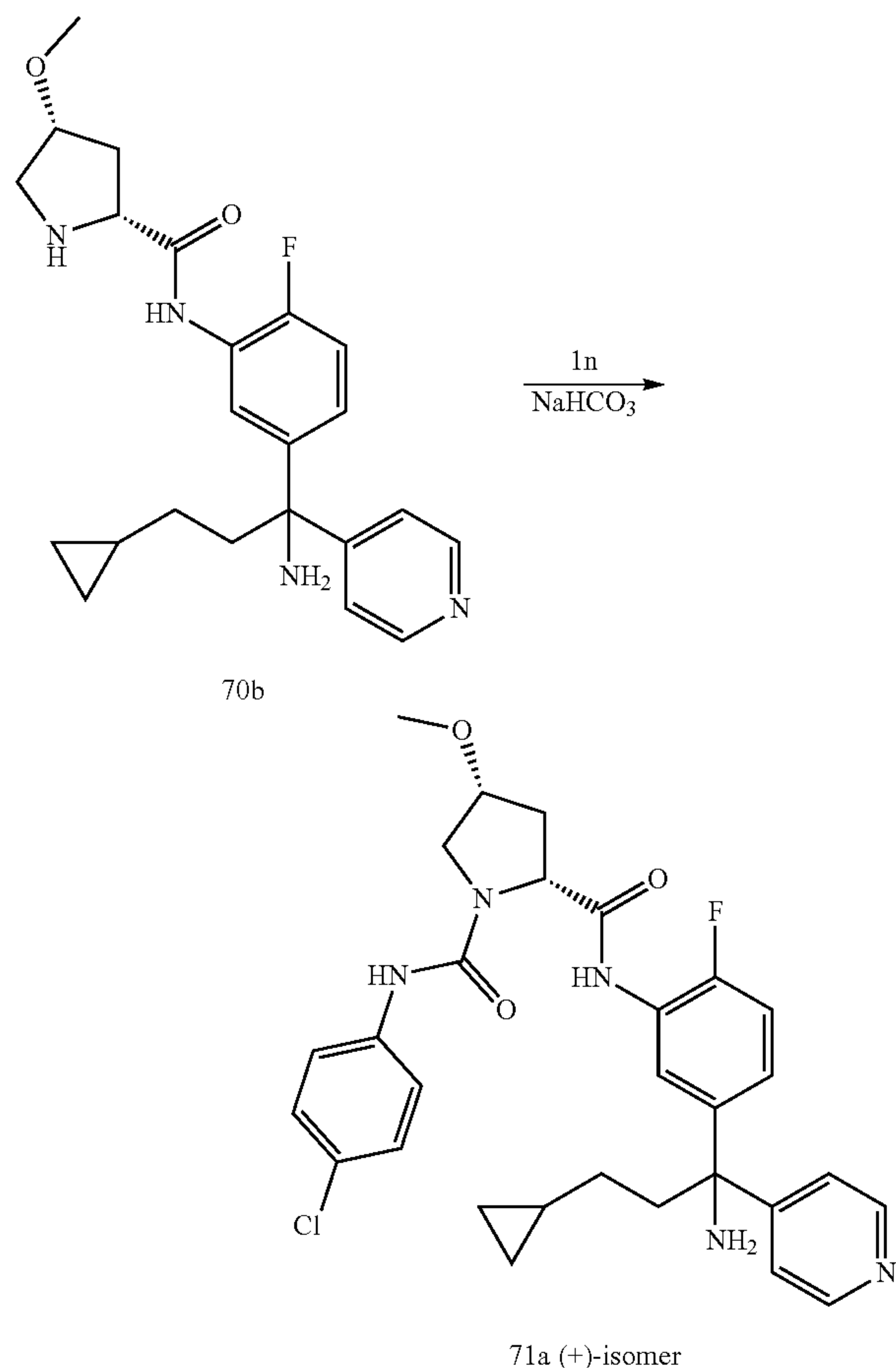
Scheme 71
