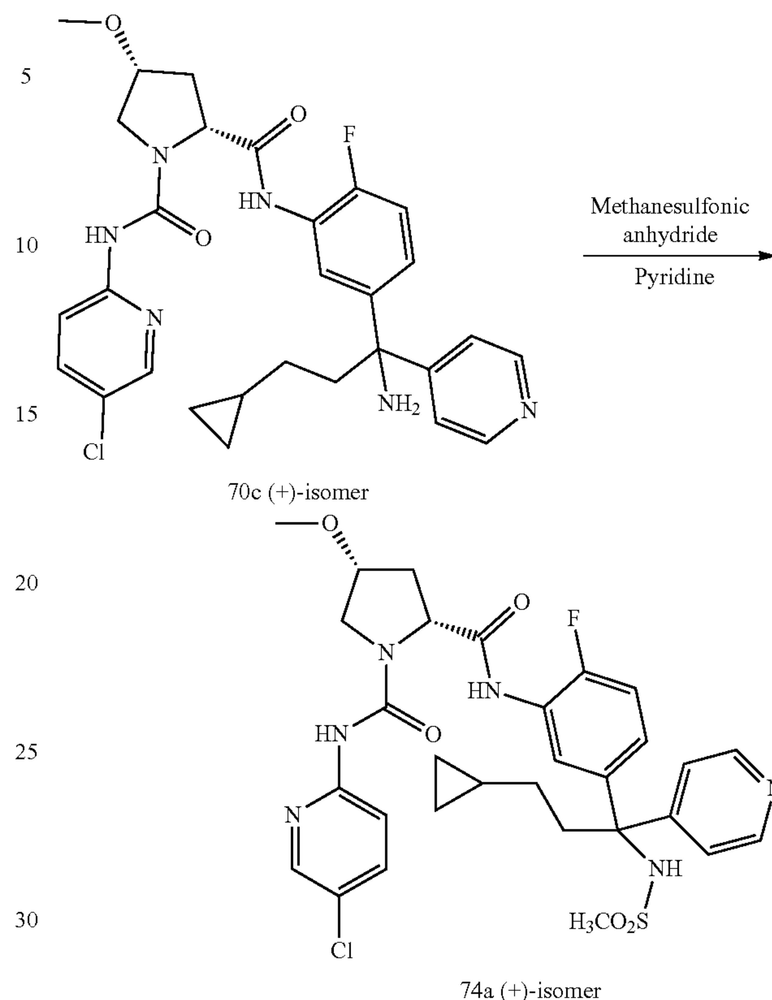
Scheme 74
