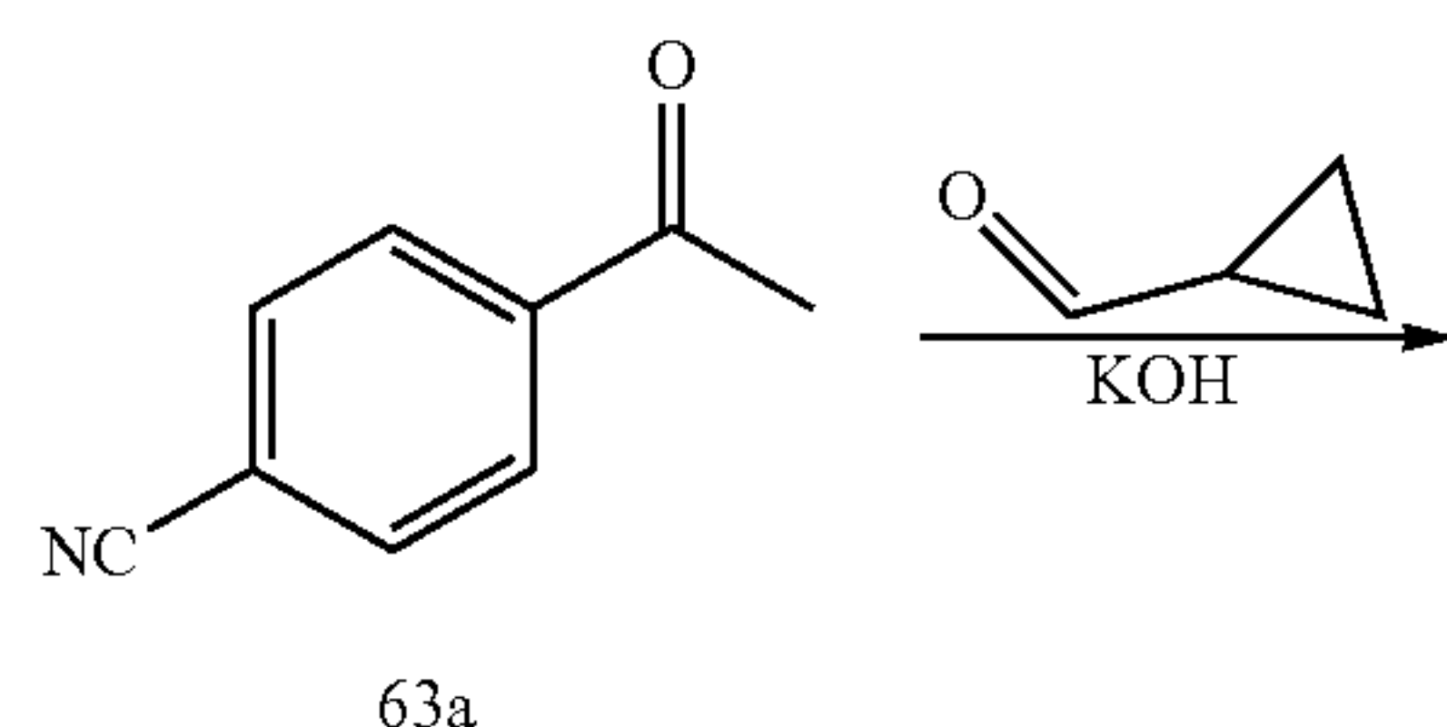
Scheme 63
