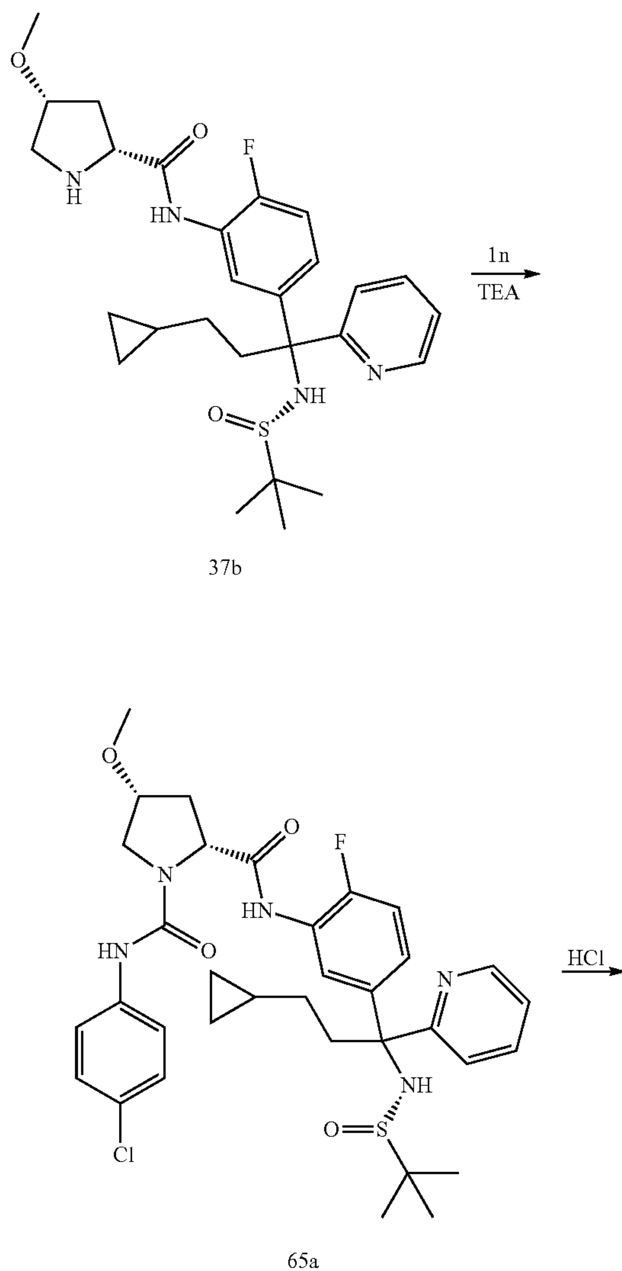
Scheme 65
