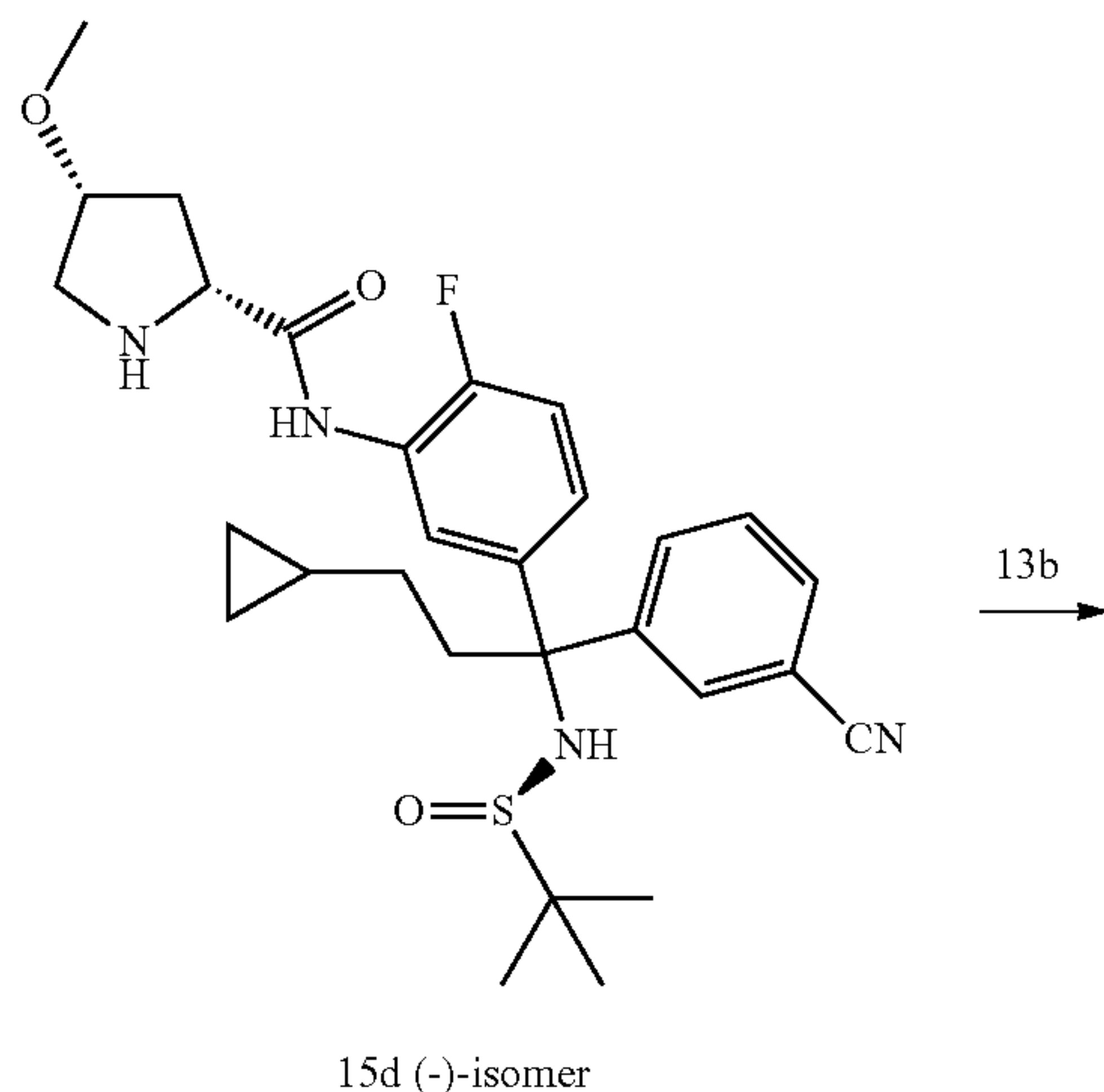
Scheme 18
