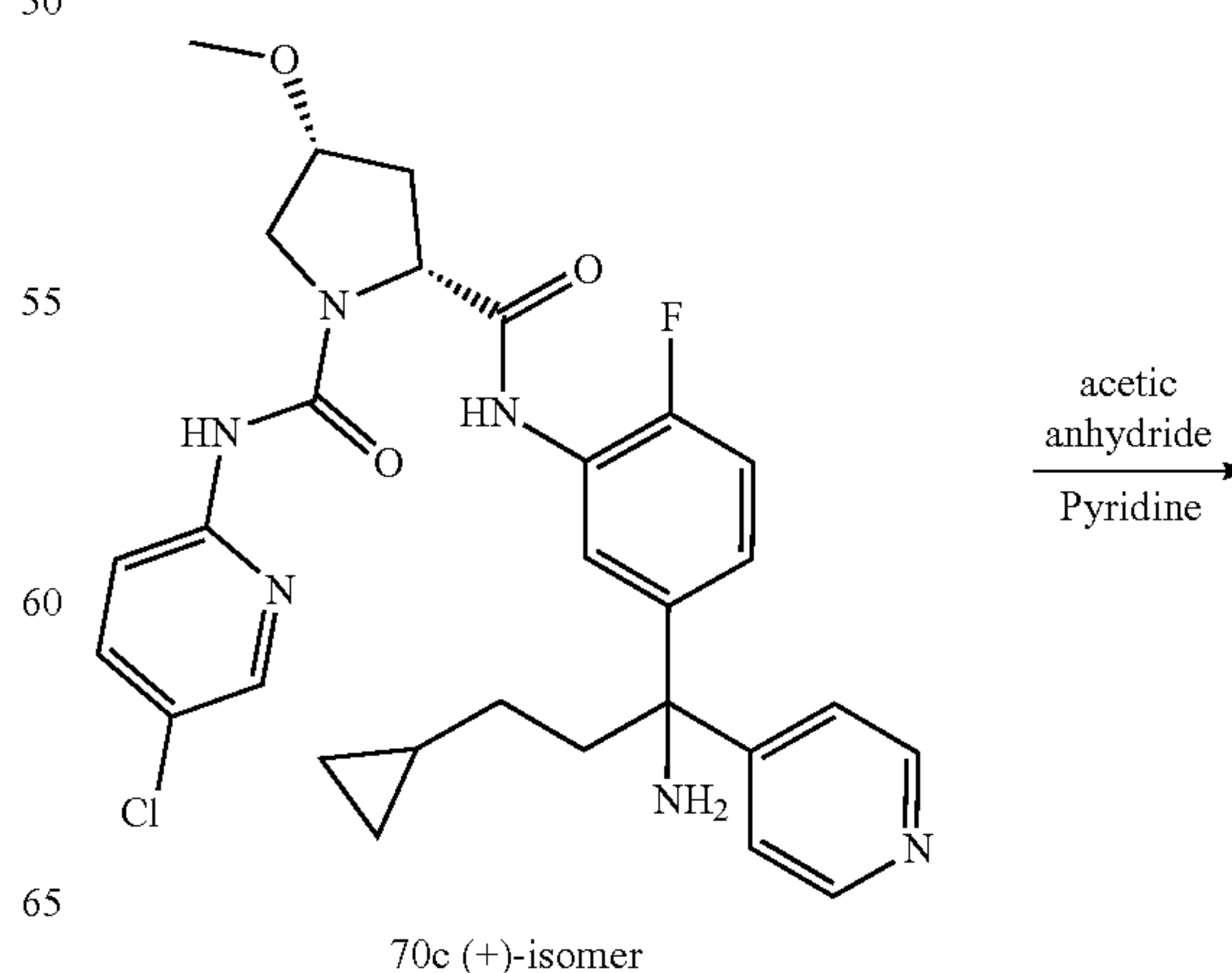
Scheme 73
