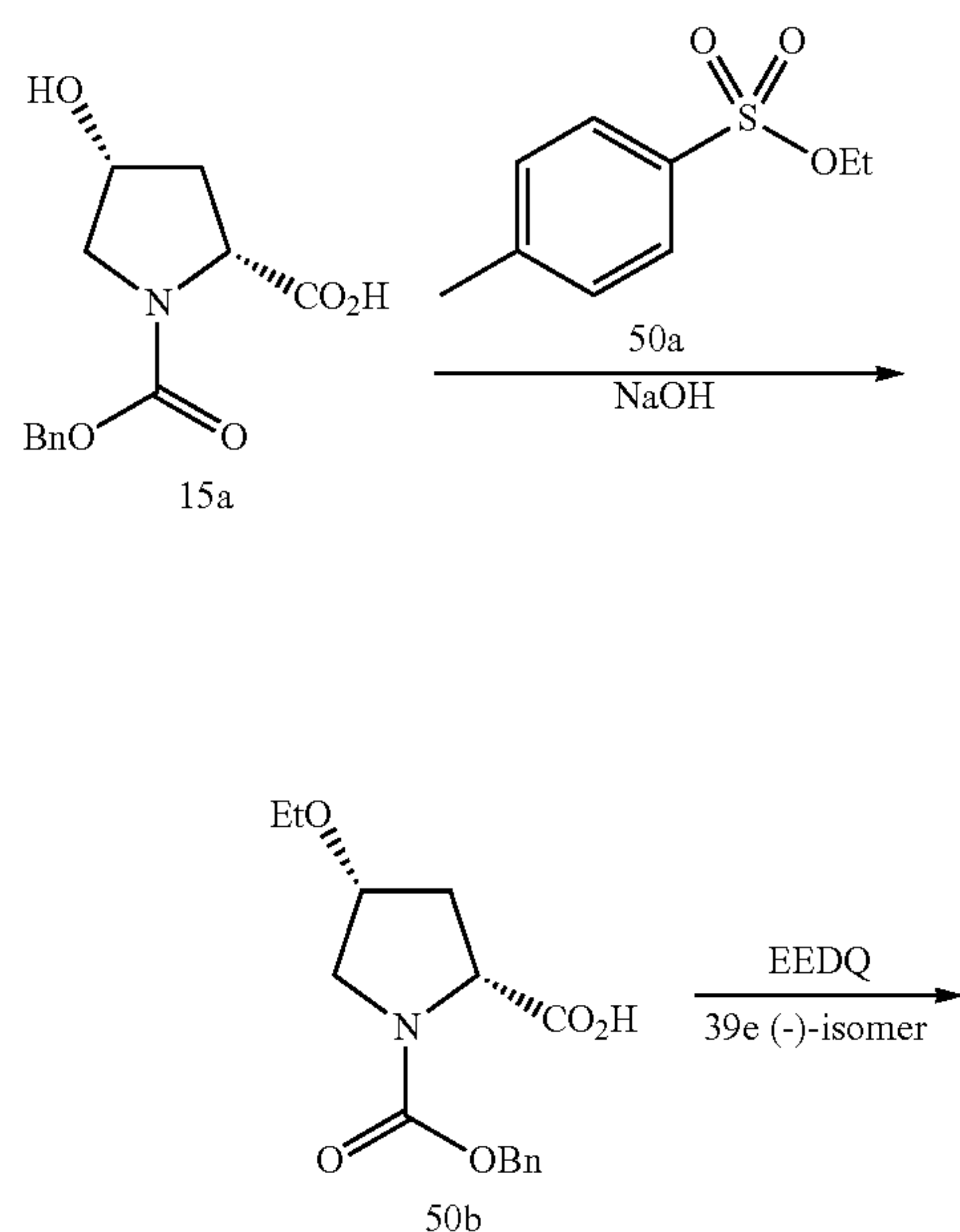
Scheme 50
