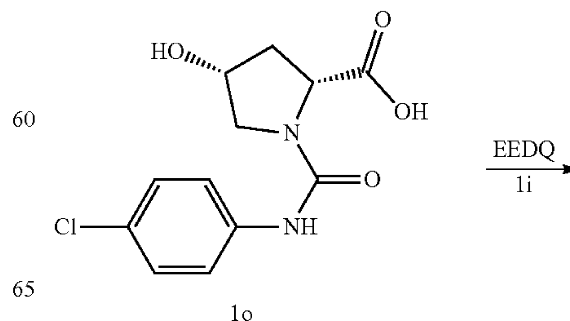
Scheme 3
