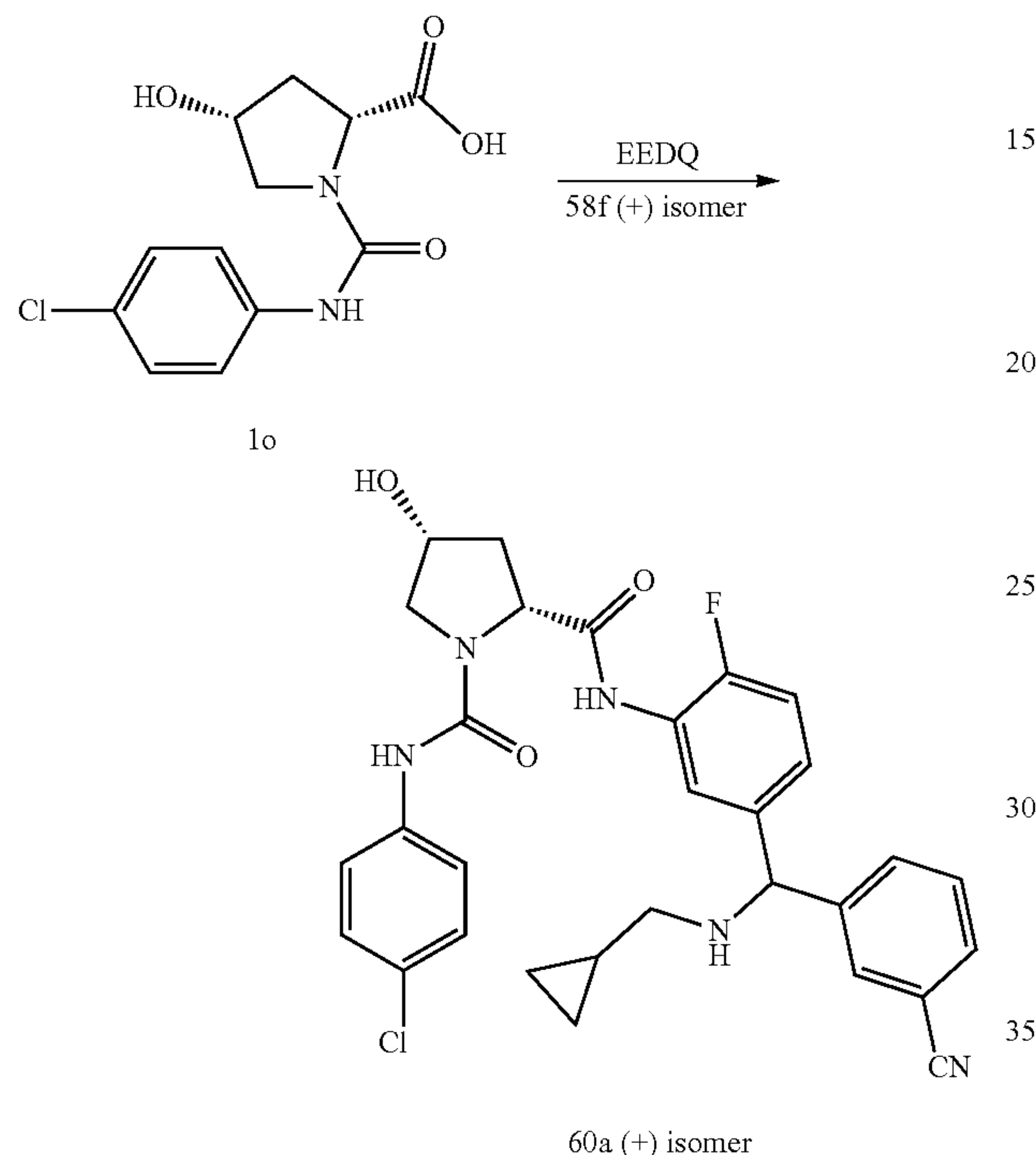
Scheme 60
