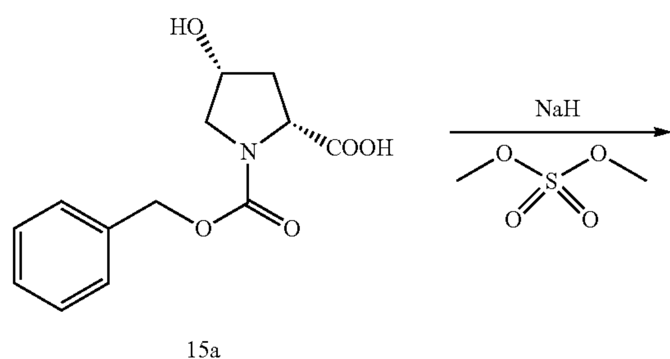
Scheme 15
