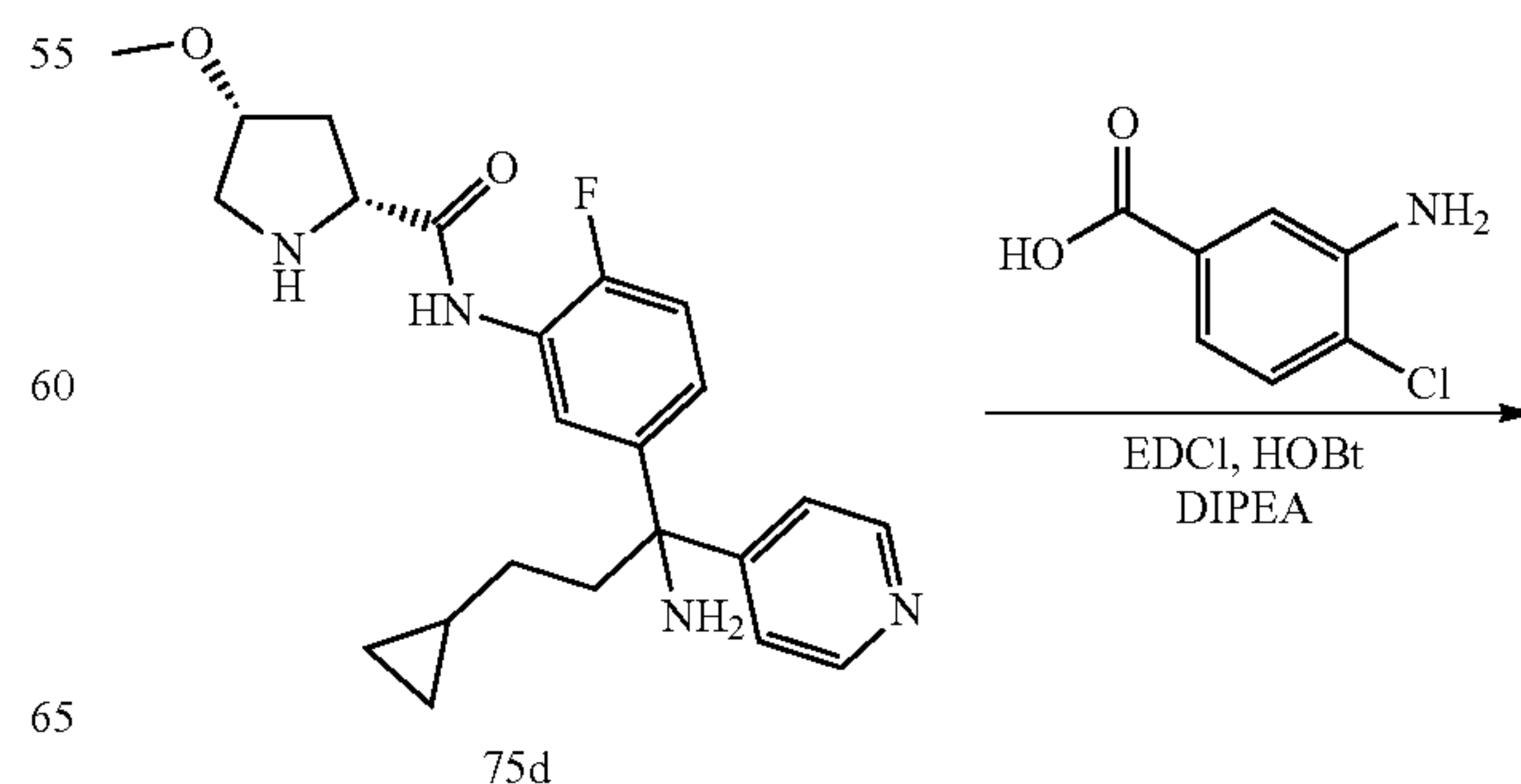
Scheme 84
