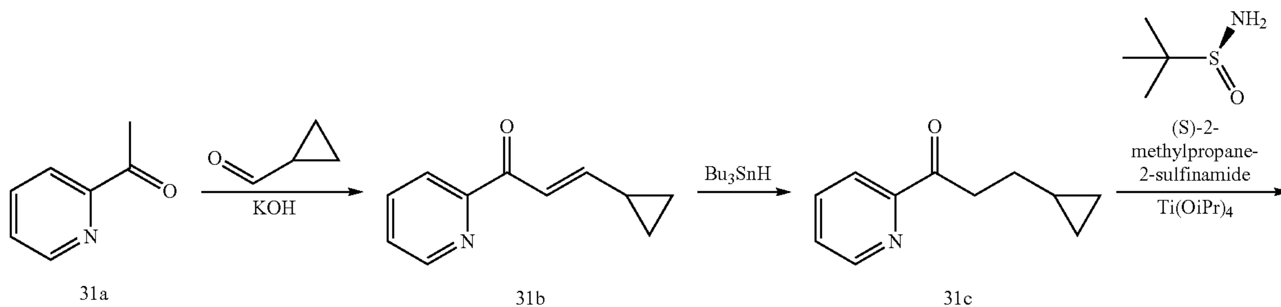
Scheme 31
