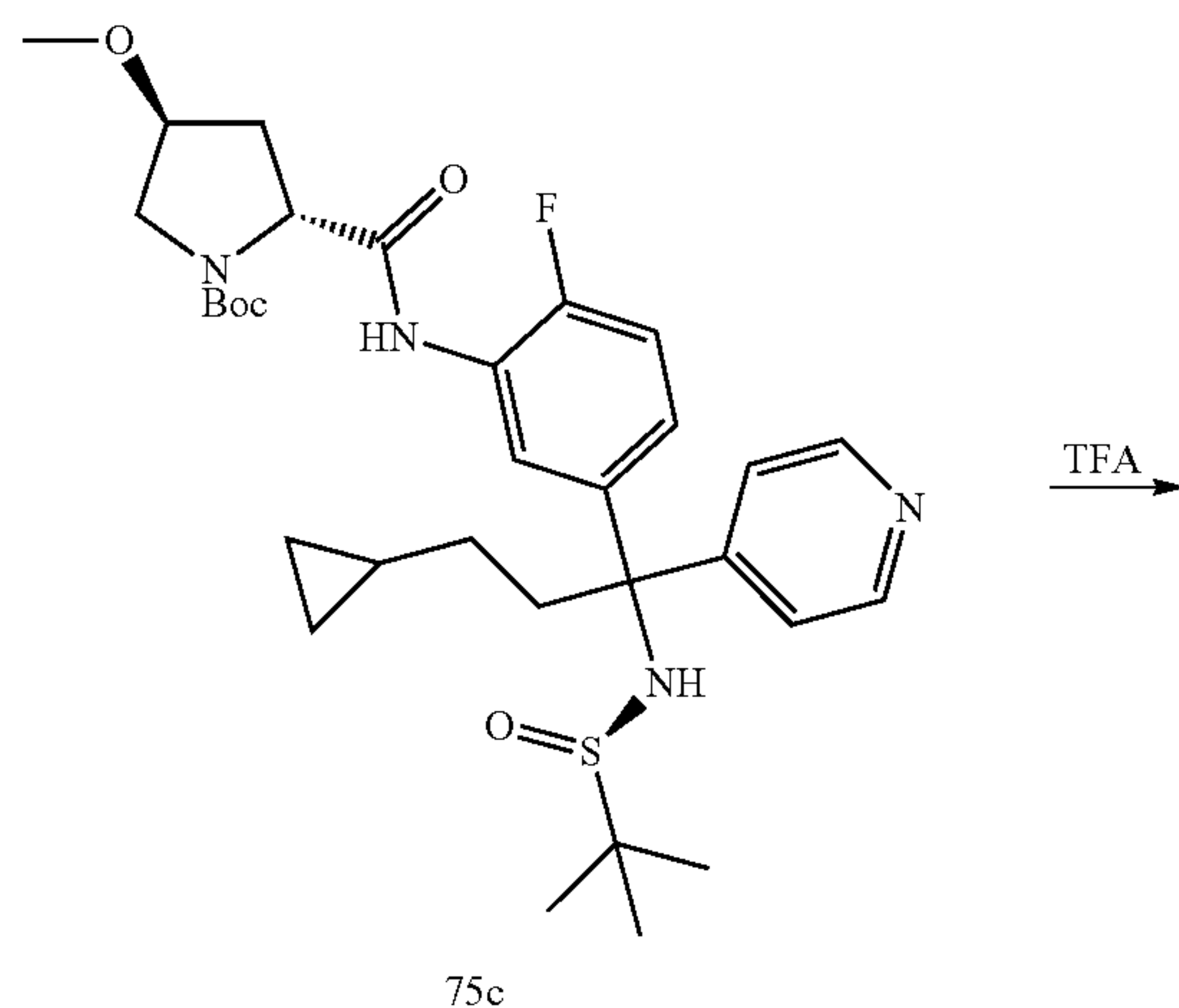
Scheme 87
