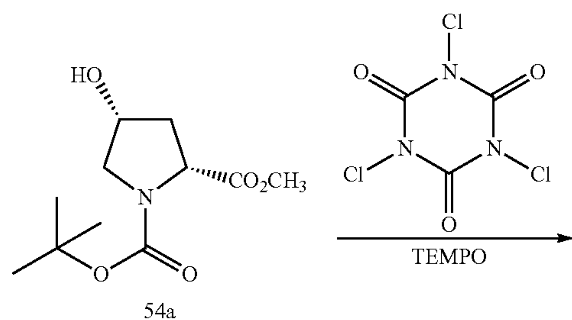
Scheme 54
