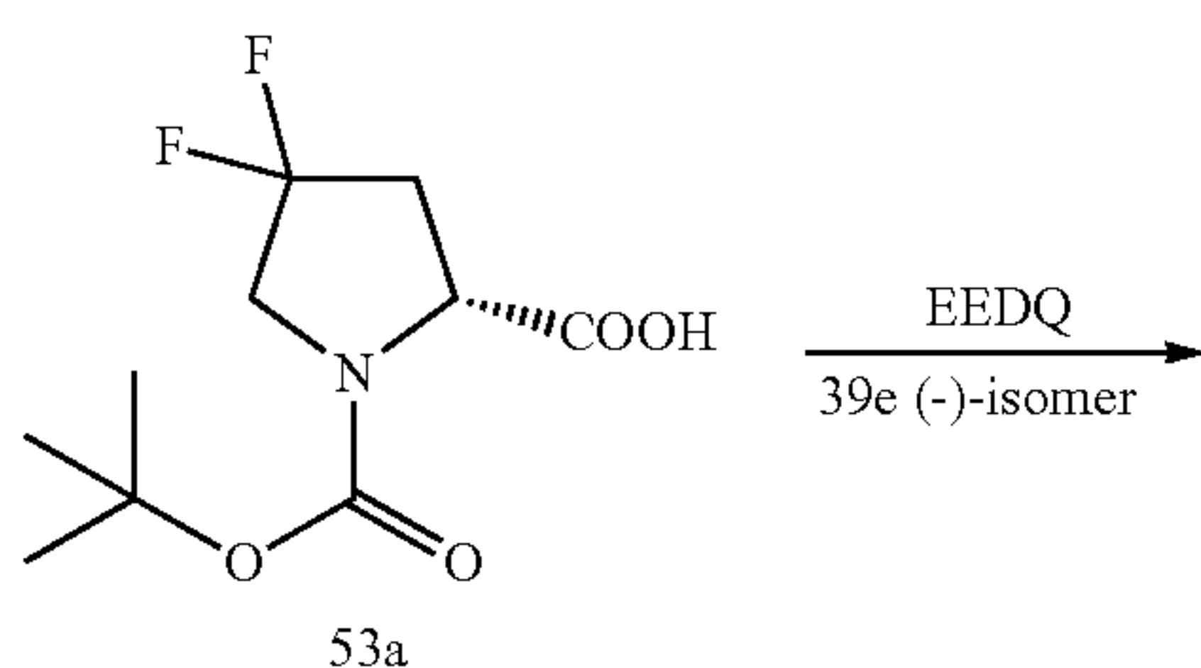
Scheme 53
