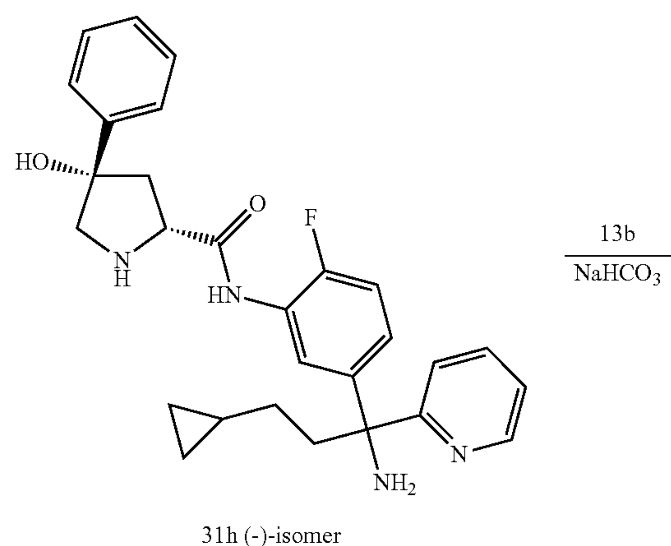
Scheme 32
