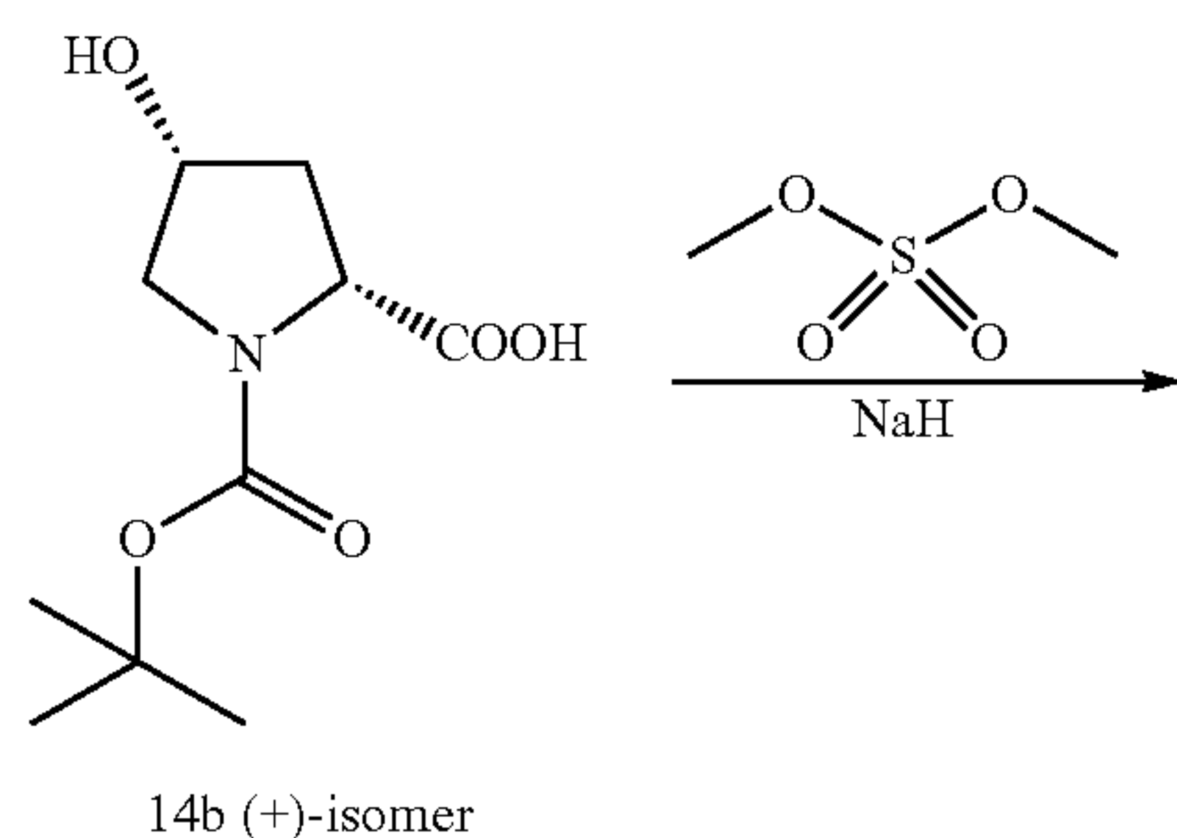
Scheme 36
