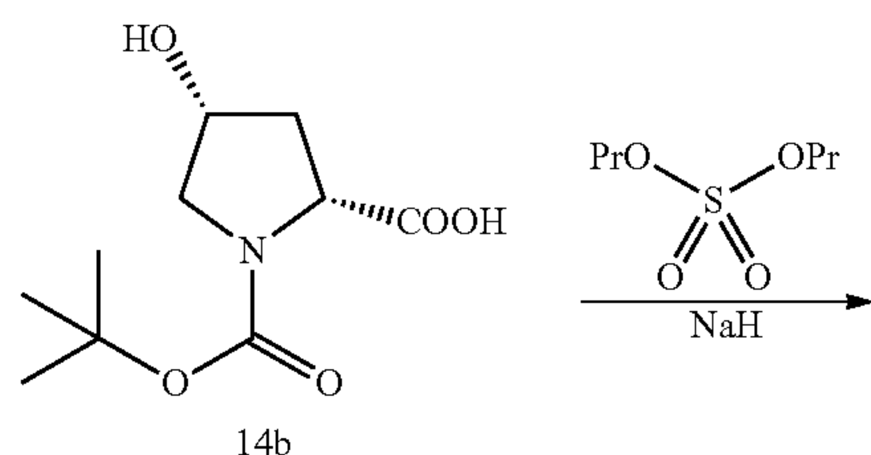
Scheme 52
