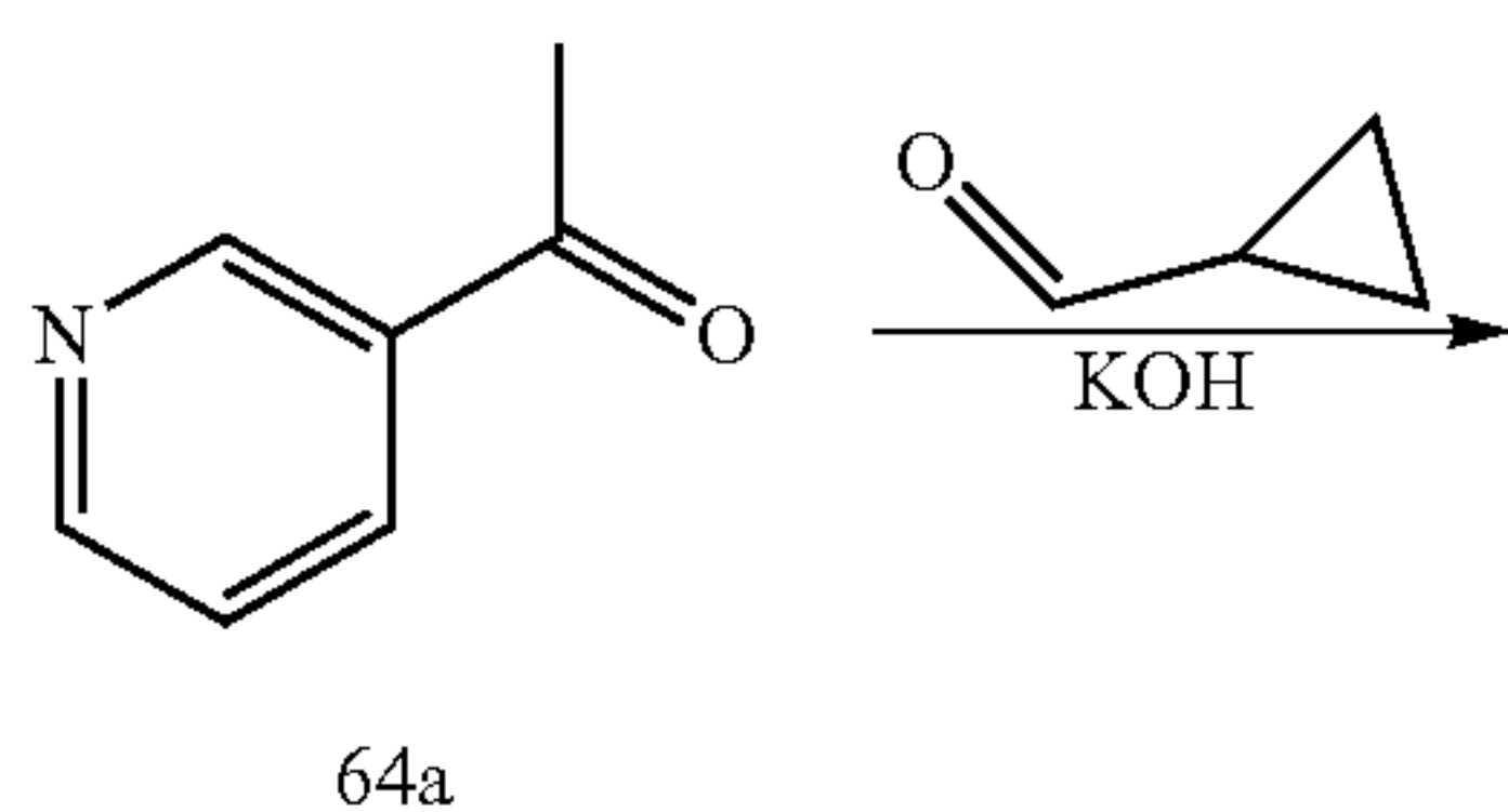
Scheme 64
