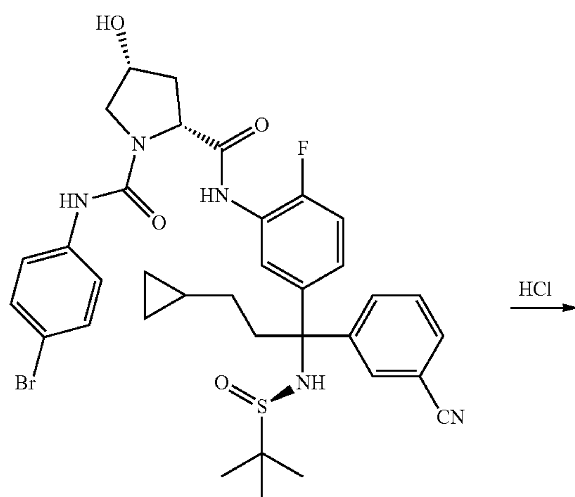
23a (-)-isomer
