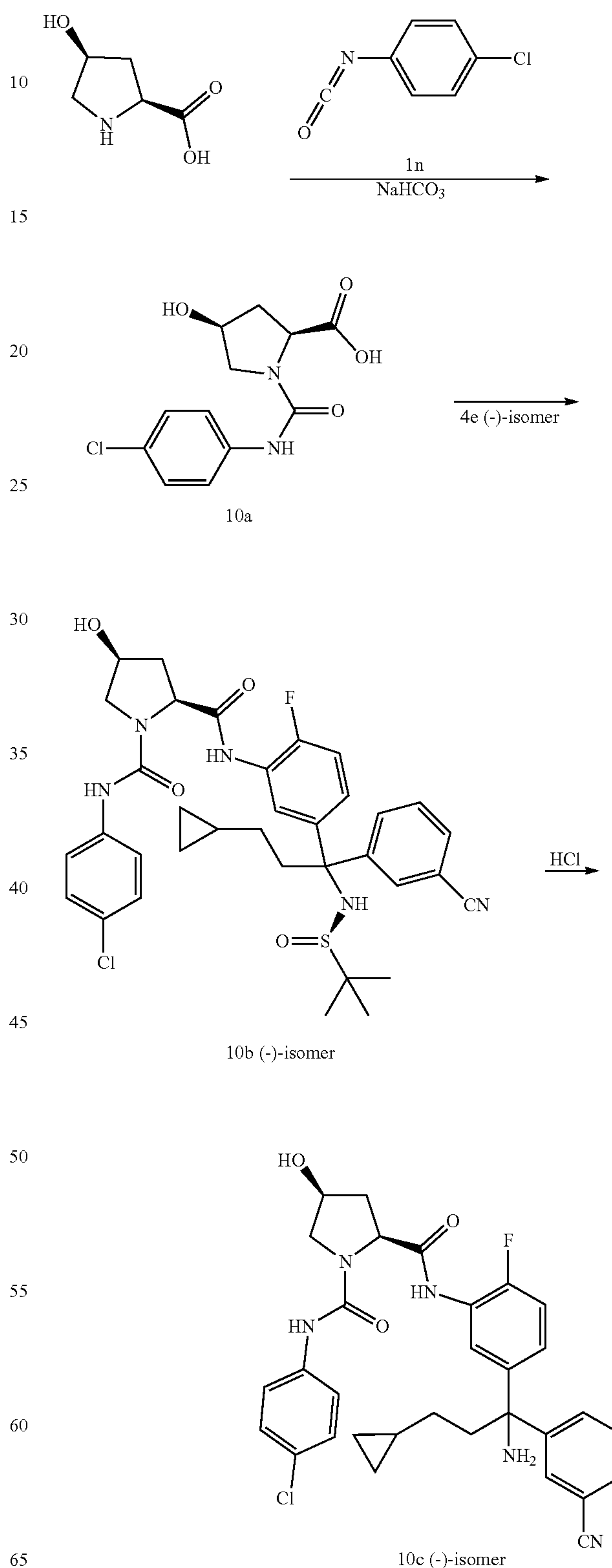
Scheme 10
