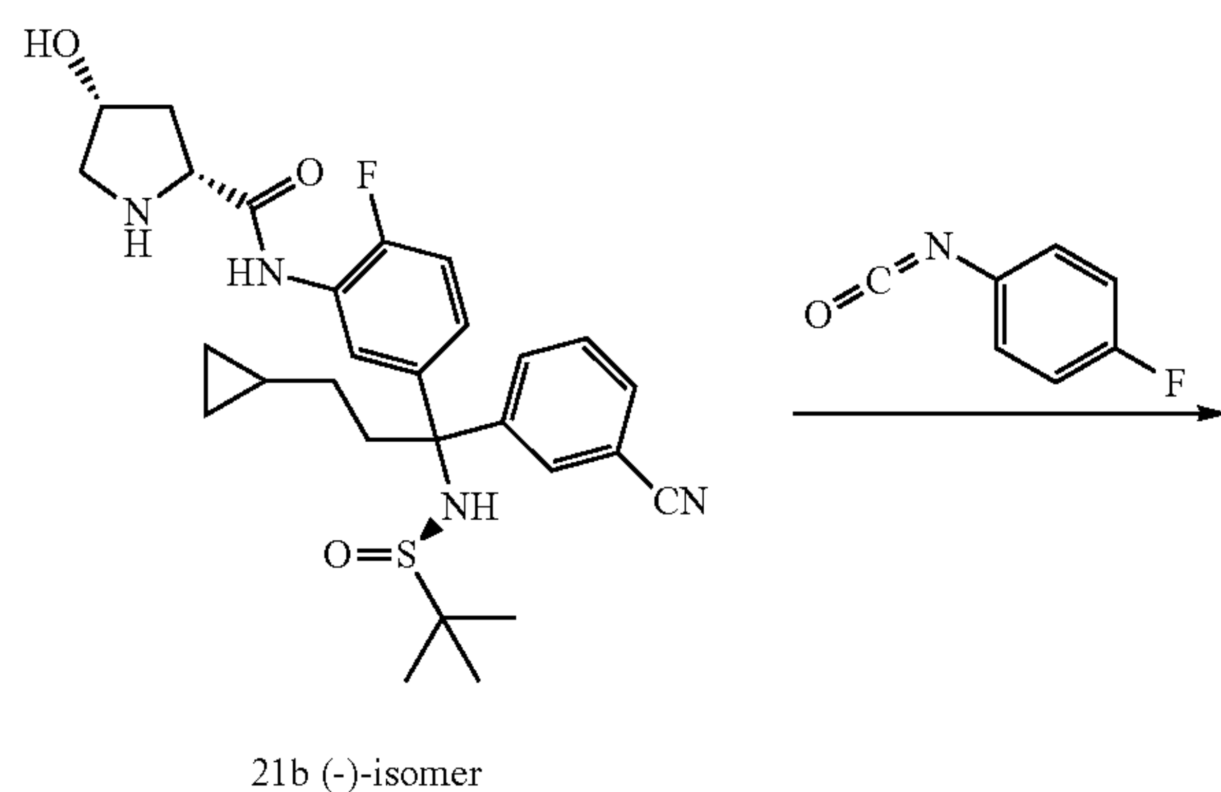
Scheme 24
