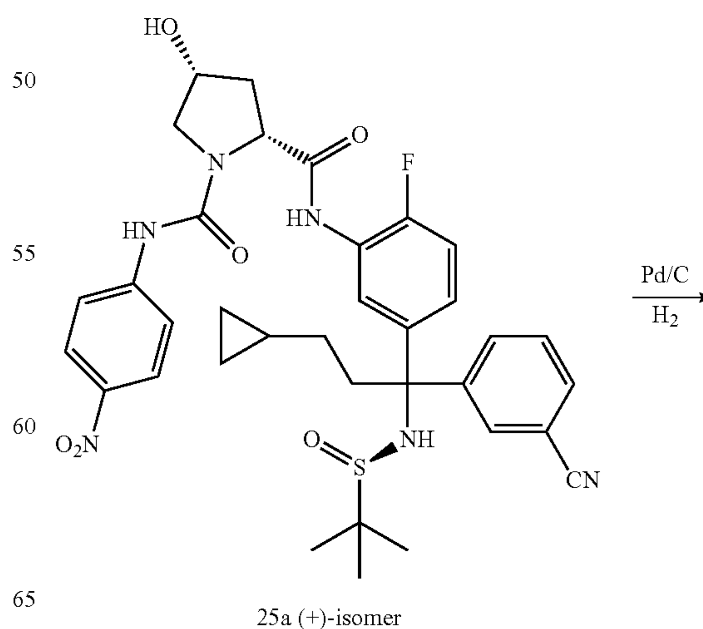
Scheme 28
