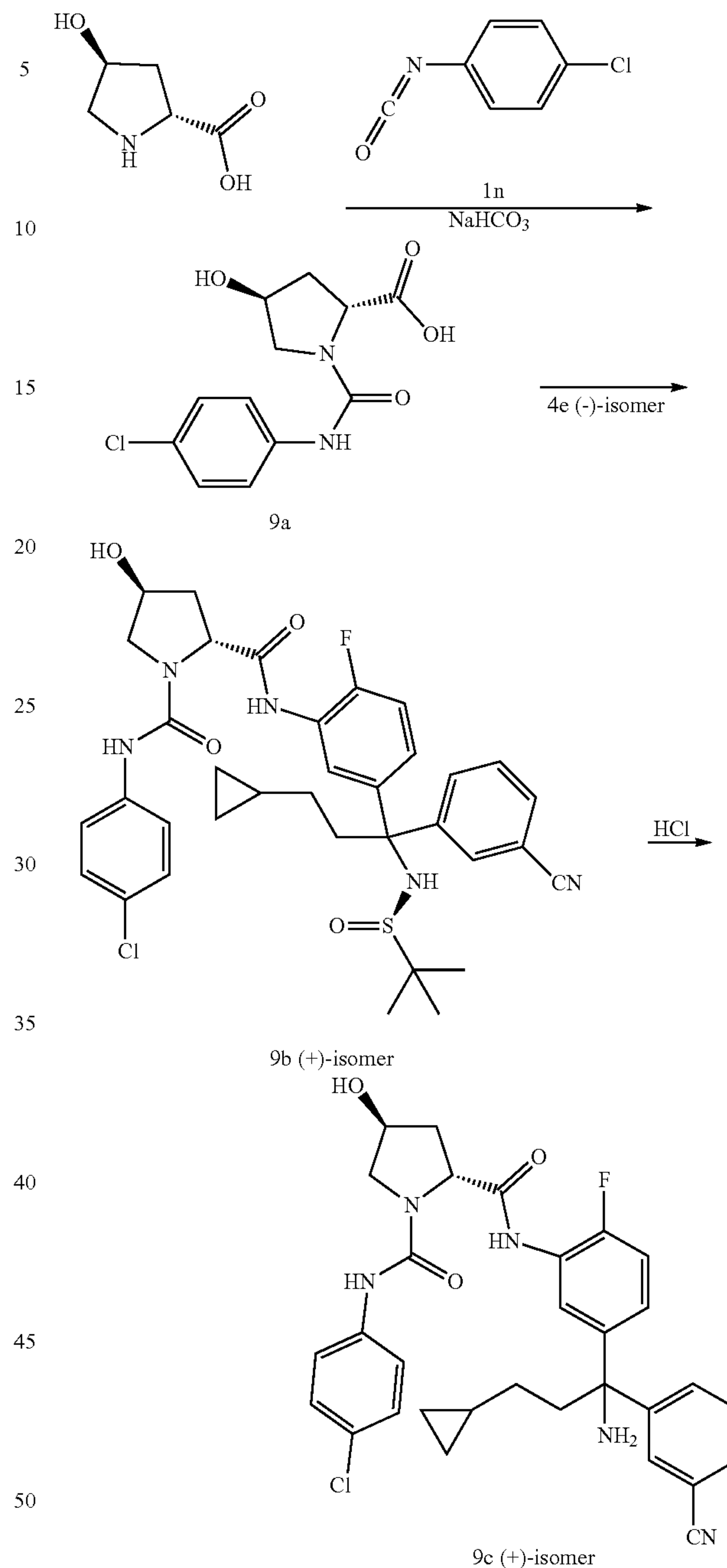
Scheme 9
