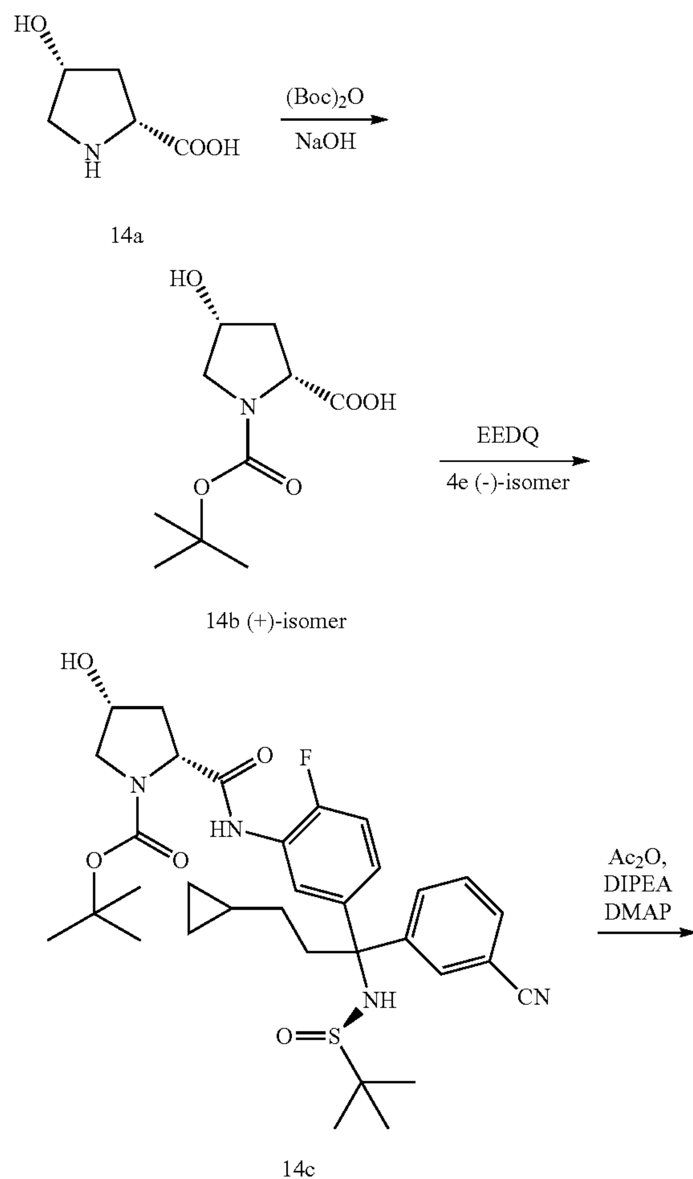
Scheme 14
