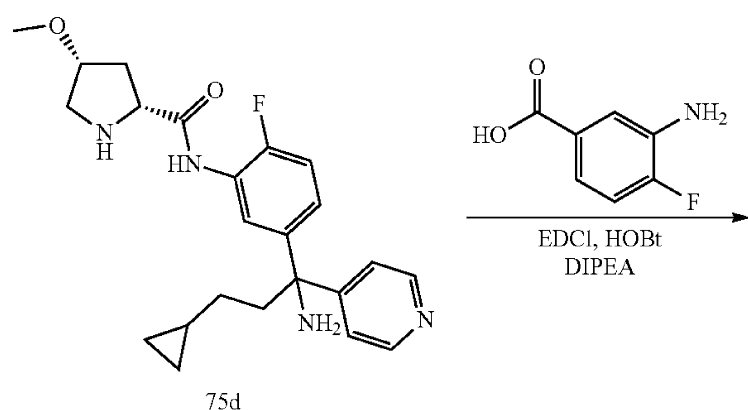
Scheme 85
