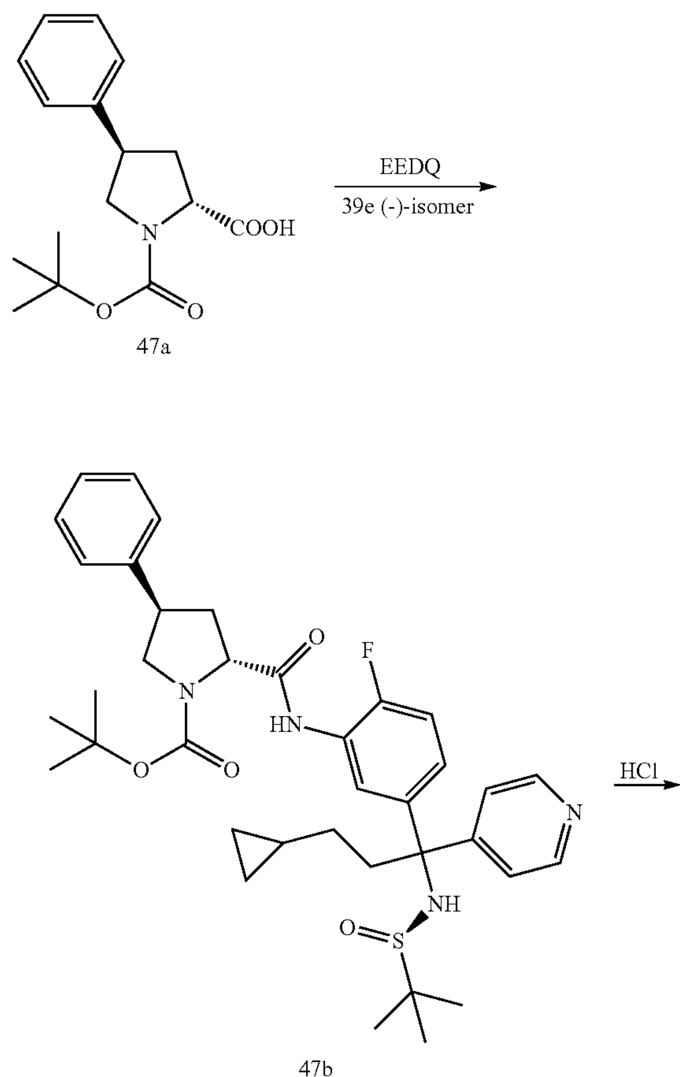
Scheme 47
