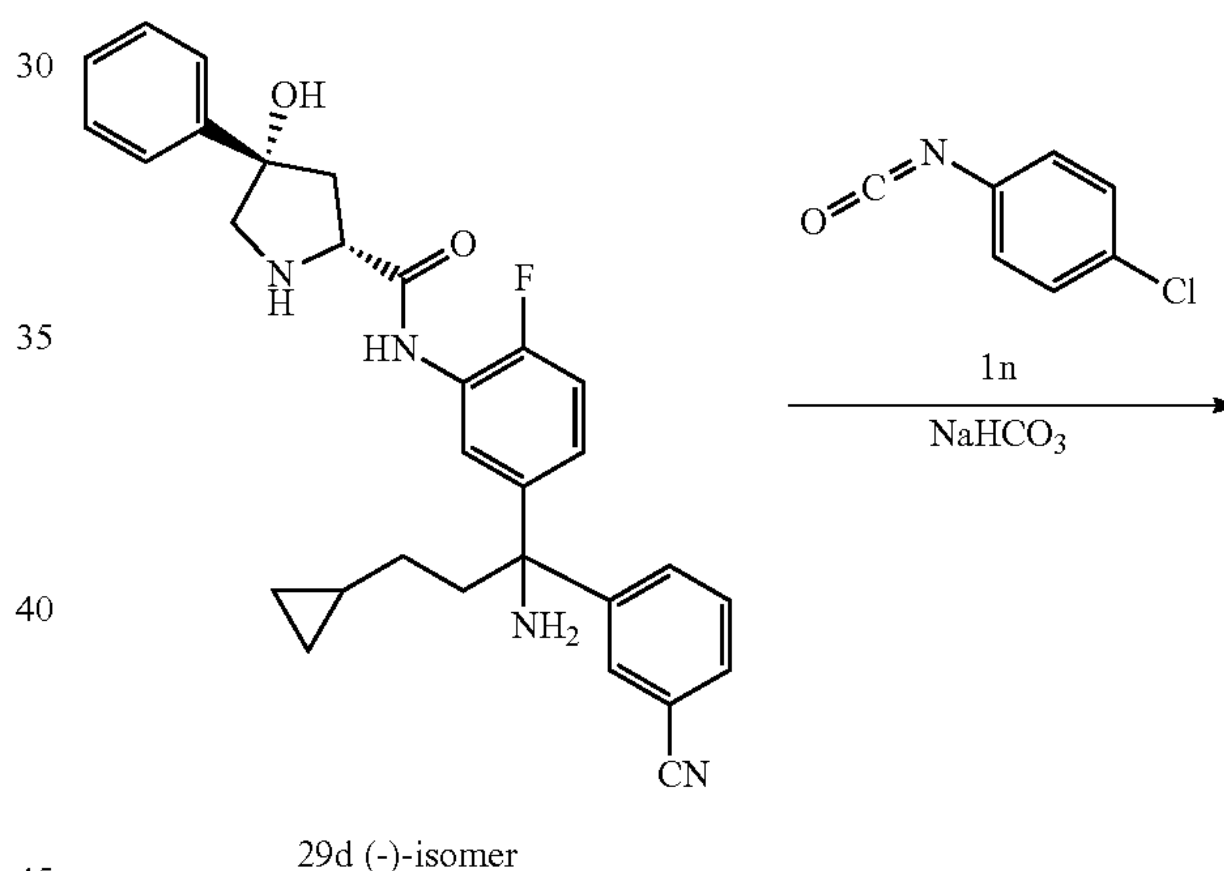
Scheme 30
