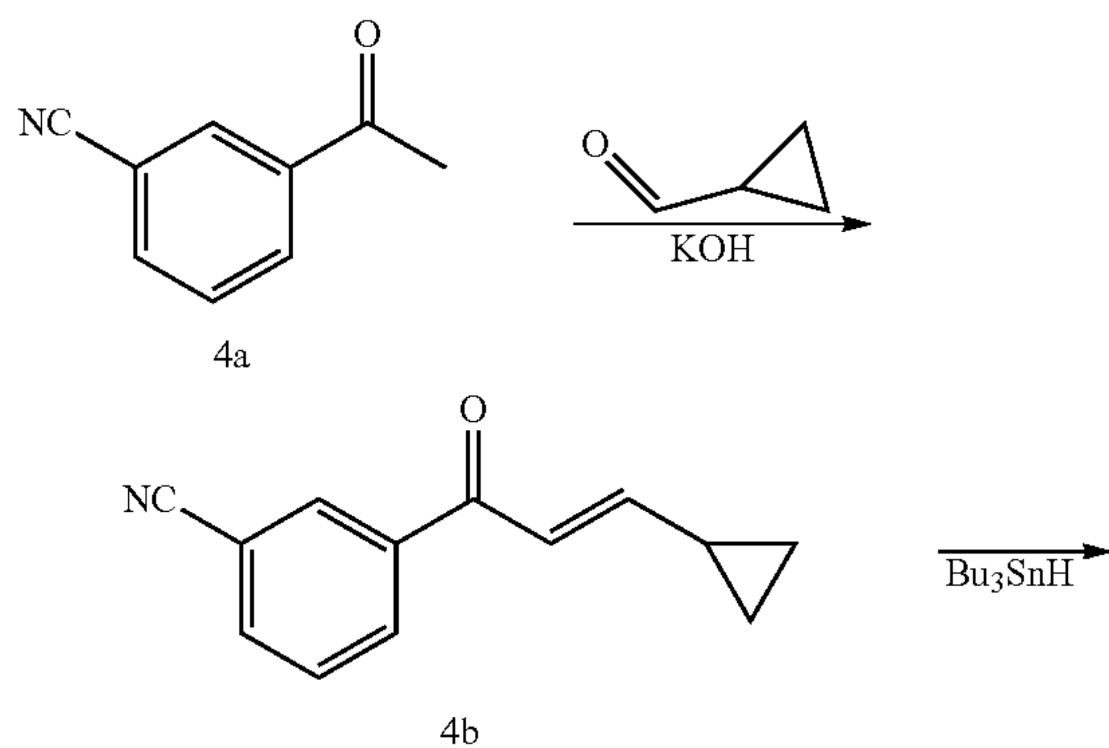
Scheme 4
