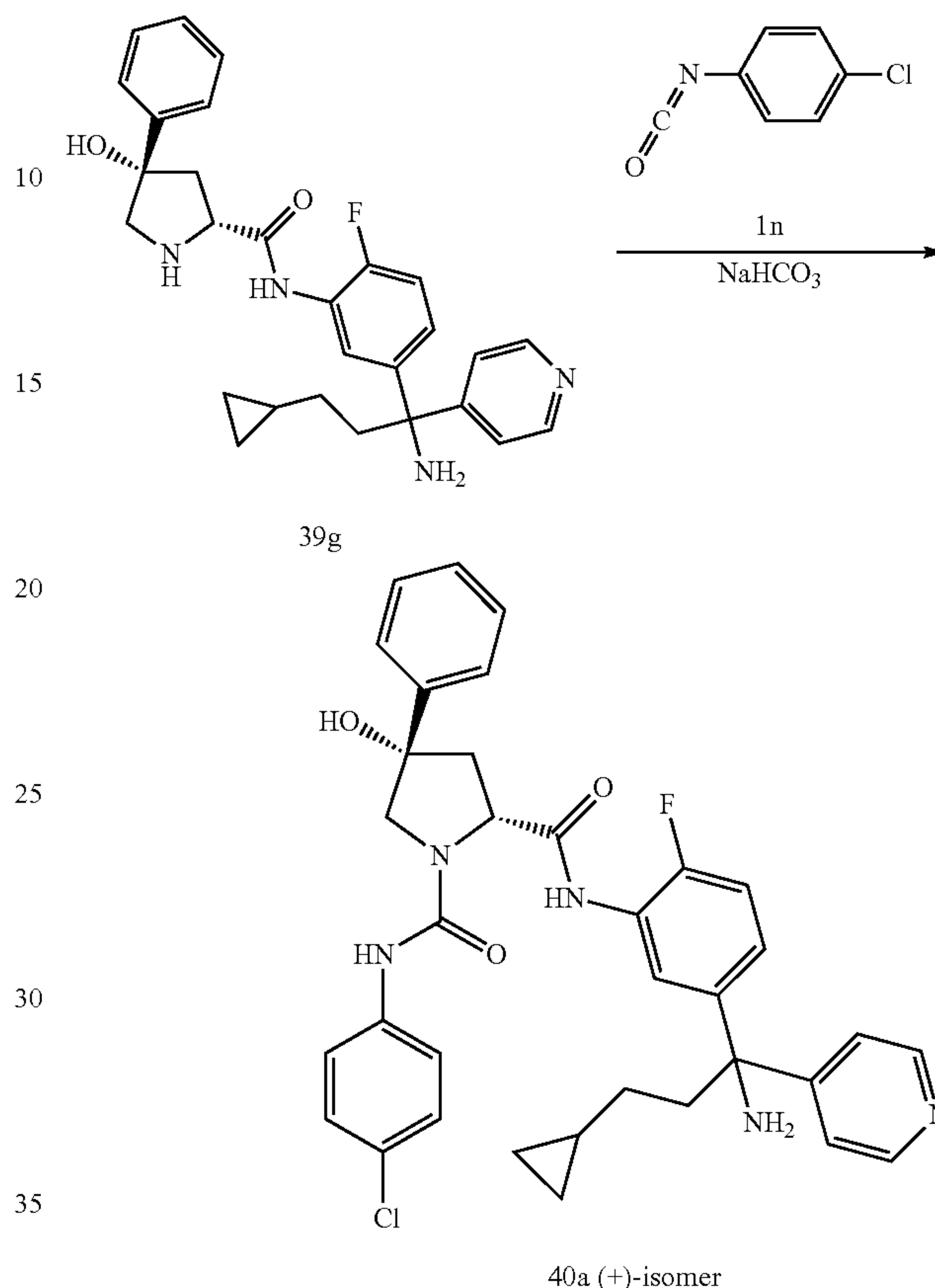
Scheme 40
