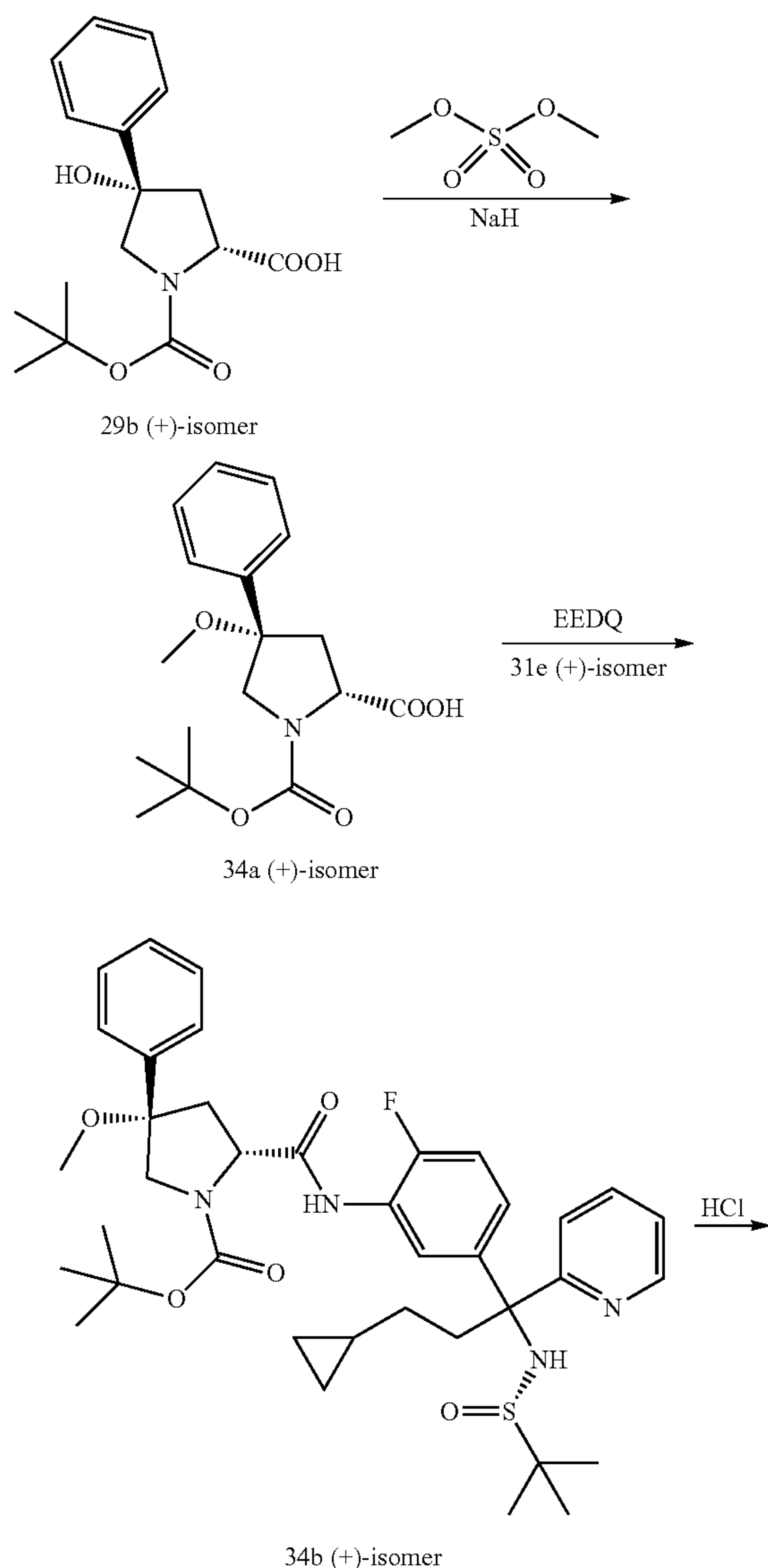
Scheme 34
