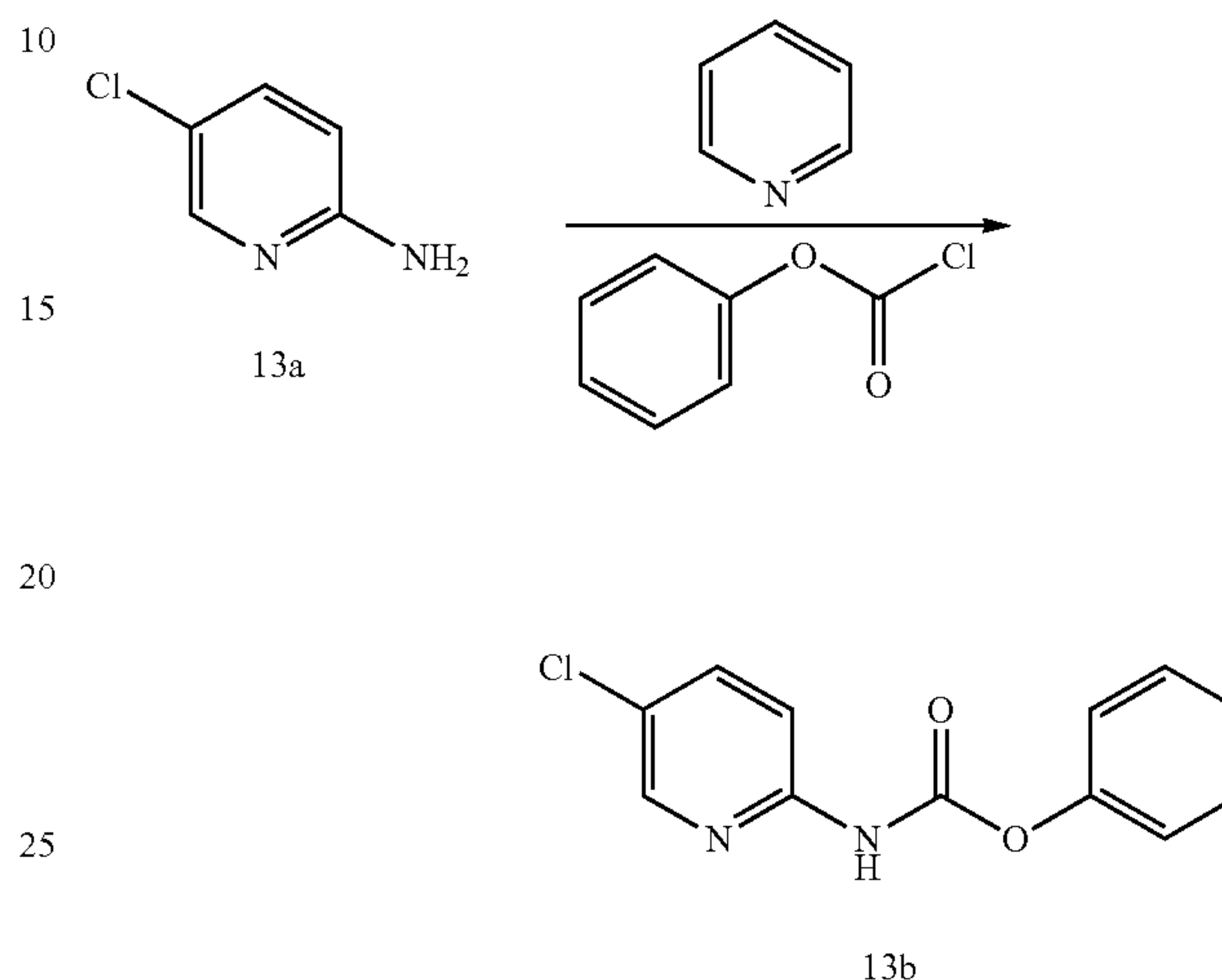
Scheme 13
