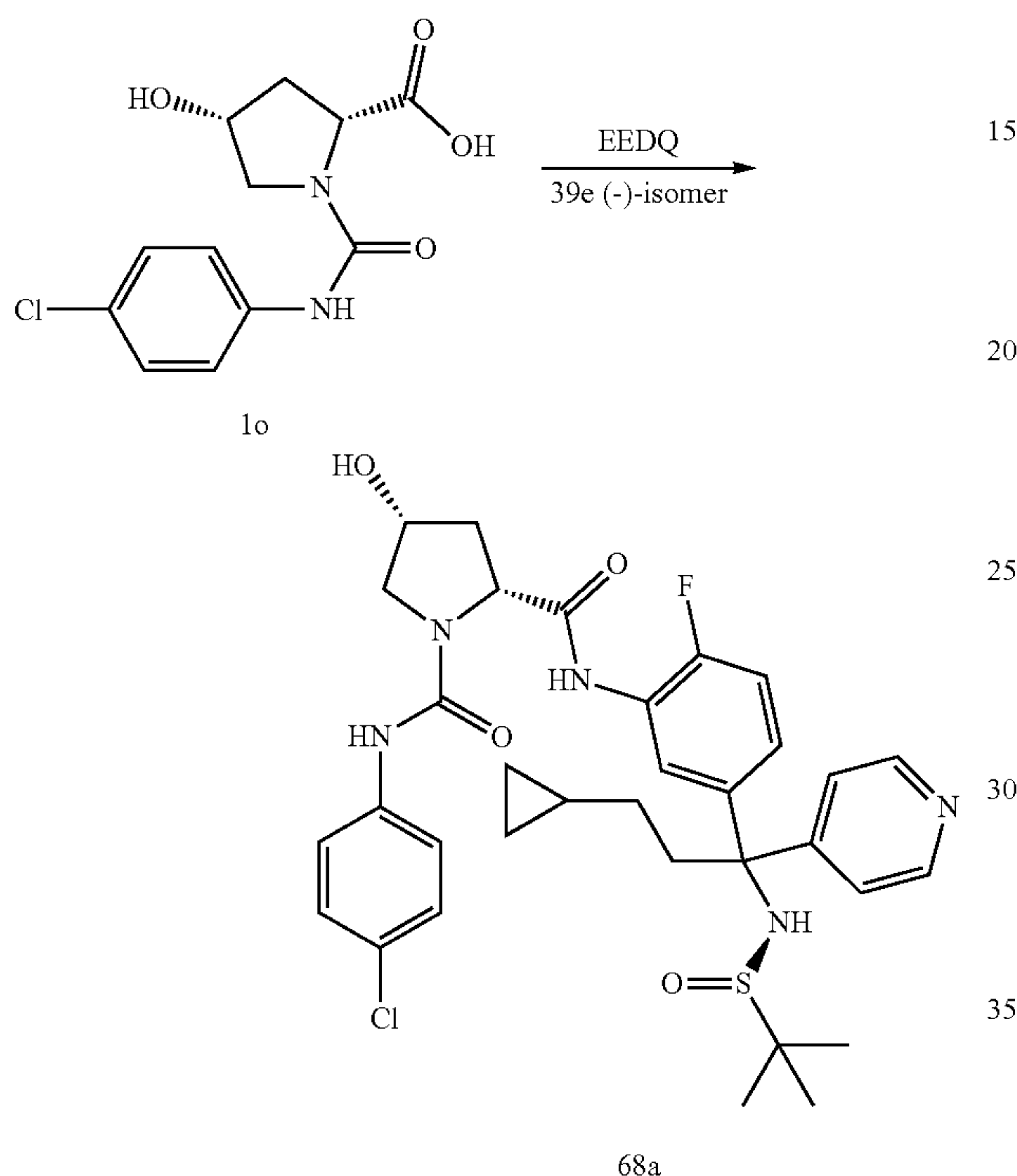
Scheme 68
