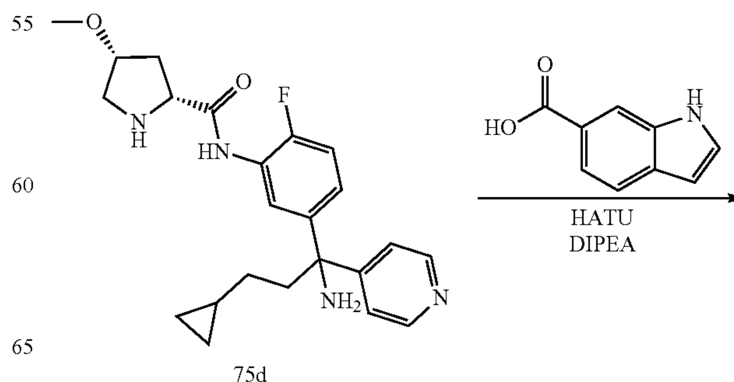
Scheme 82
