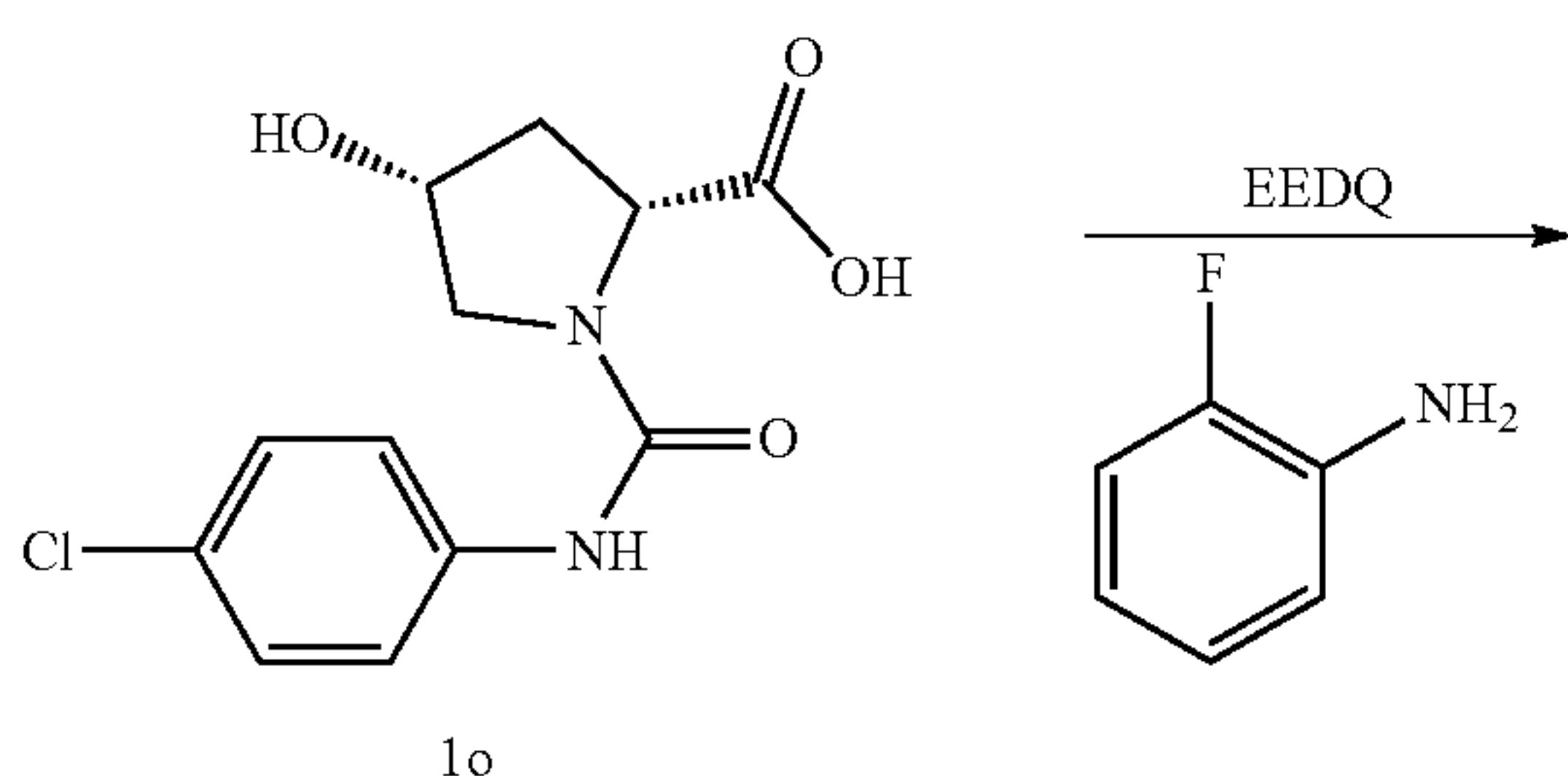
Scheme 2
