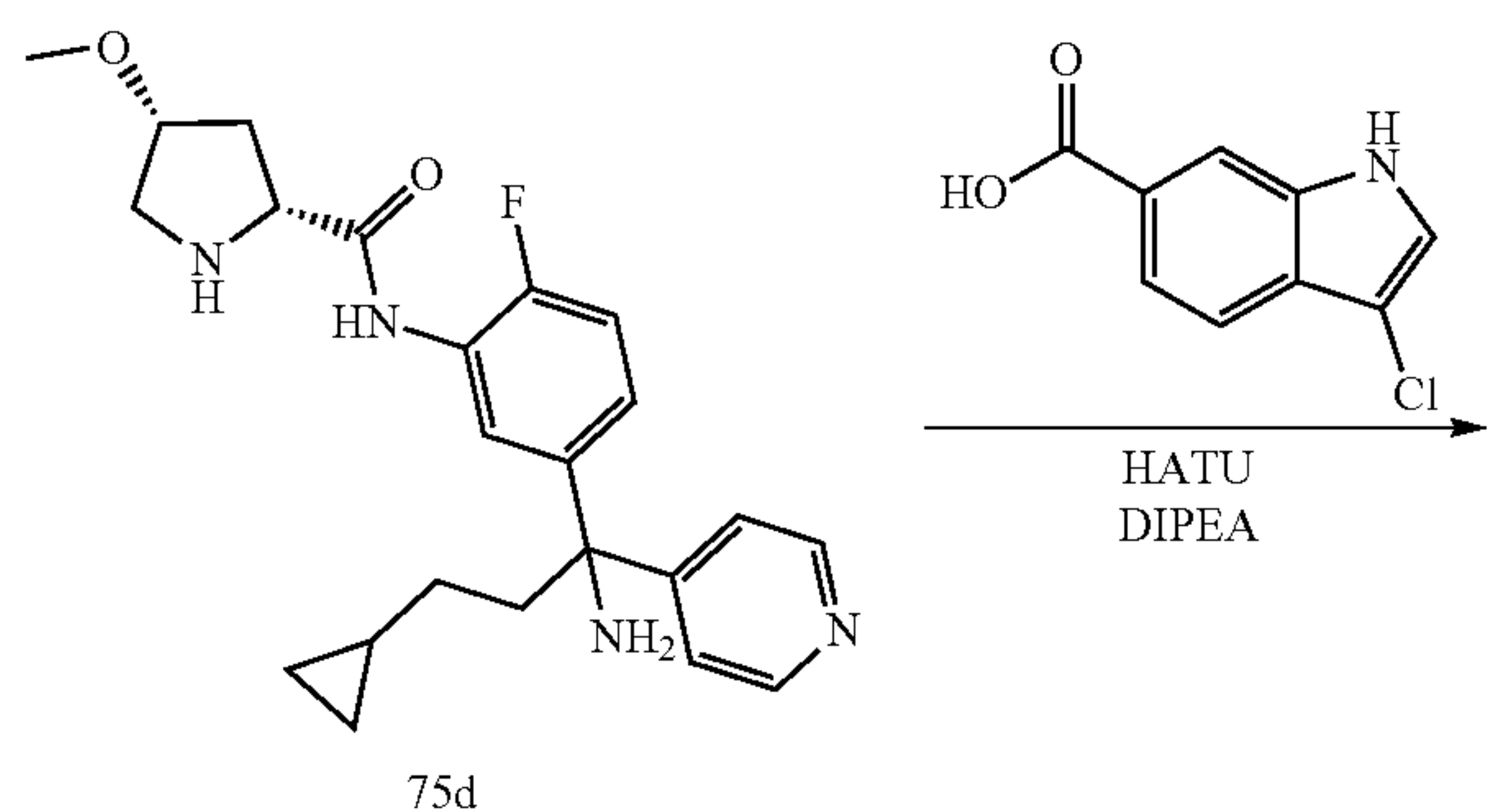
Scheme 83
