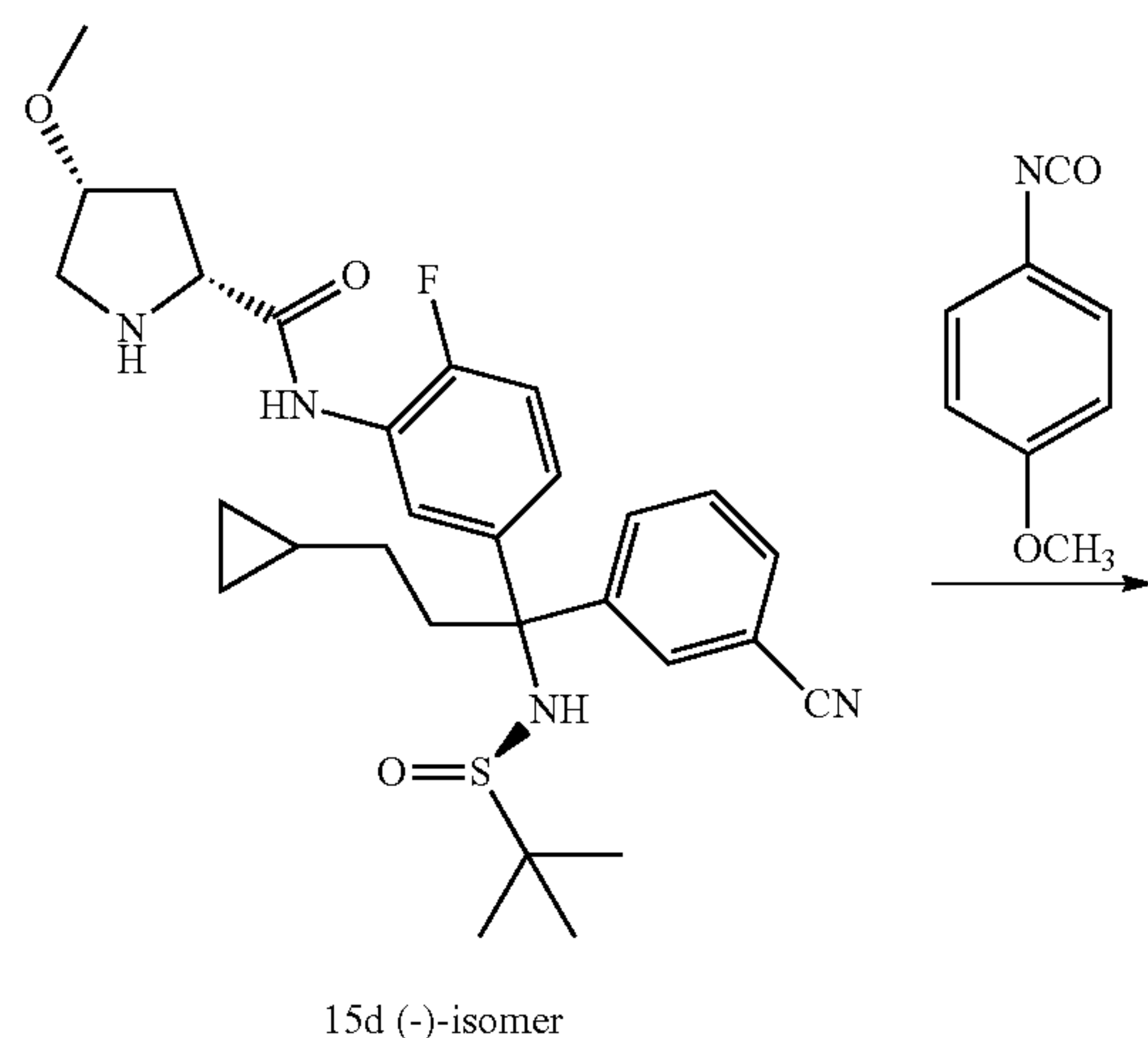
Scheme 16
