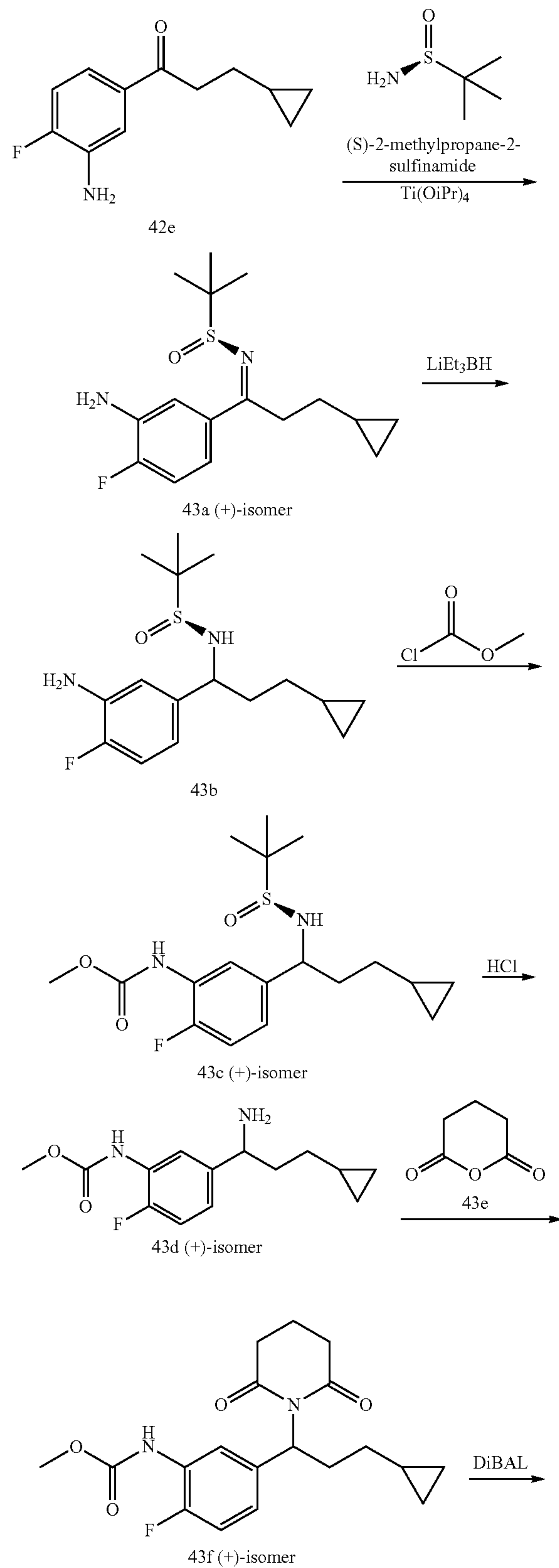
Scheme 43
