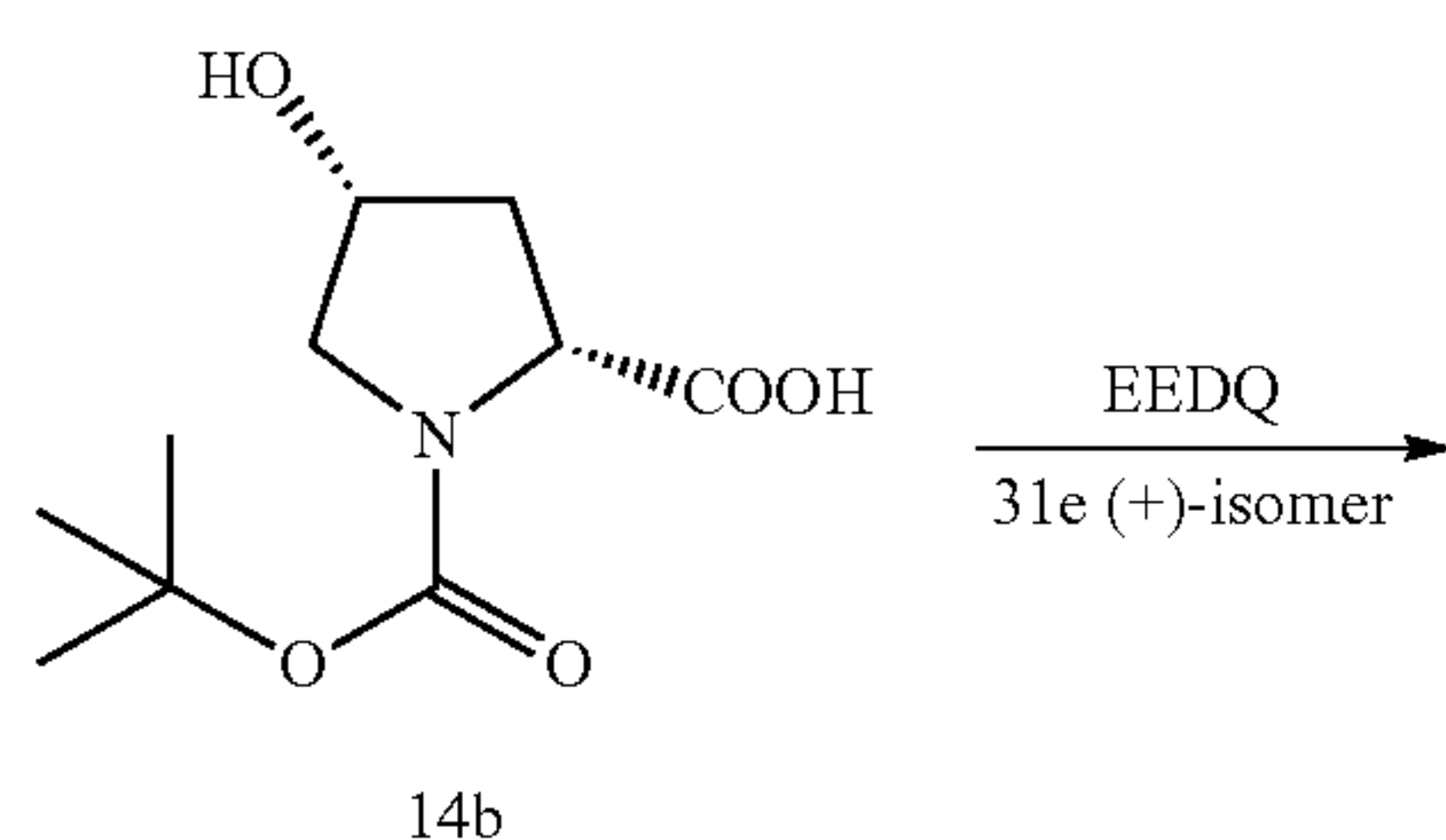
Scheme 62
