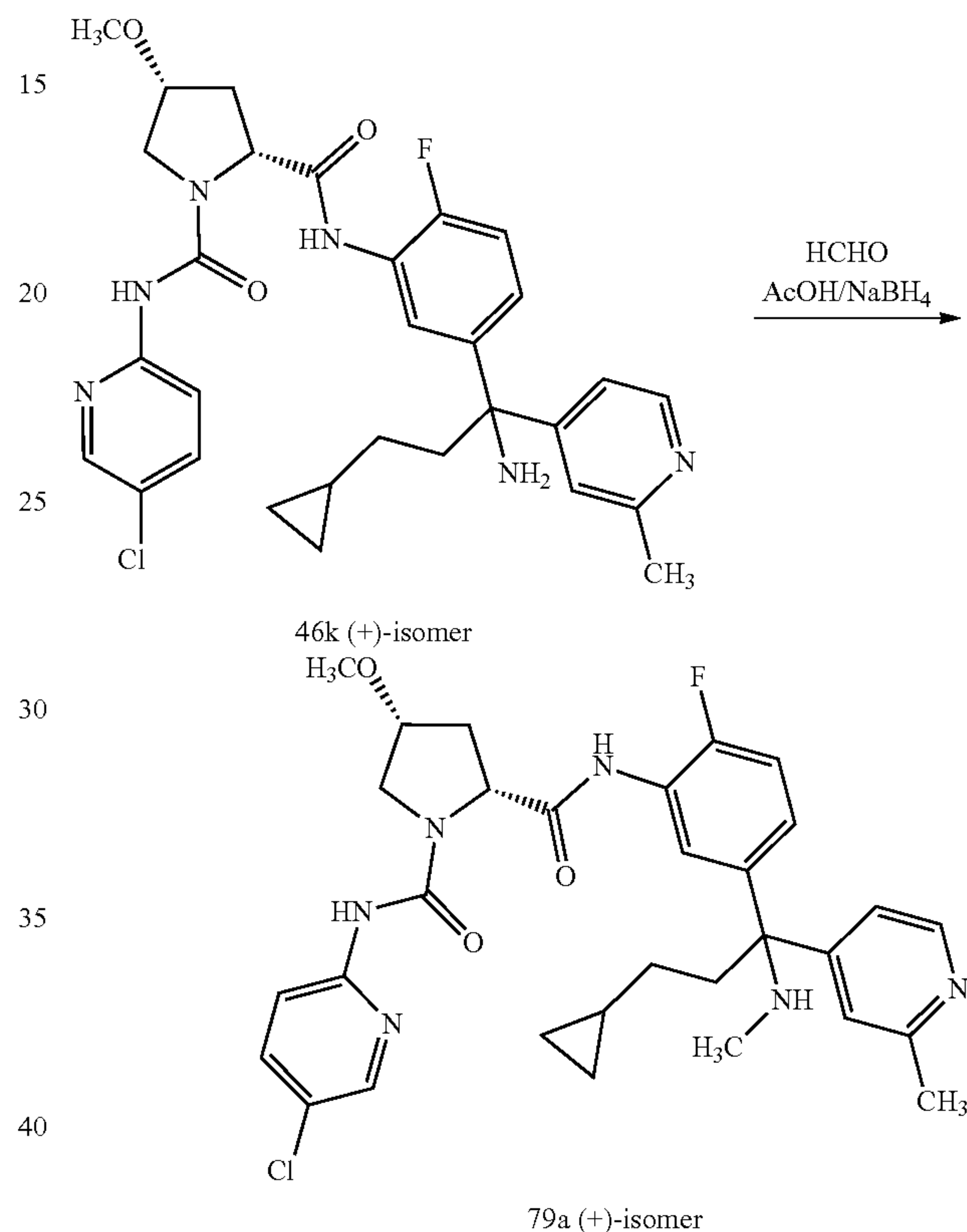
Scheme 79
