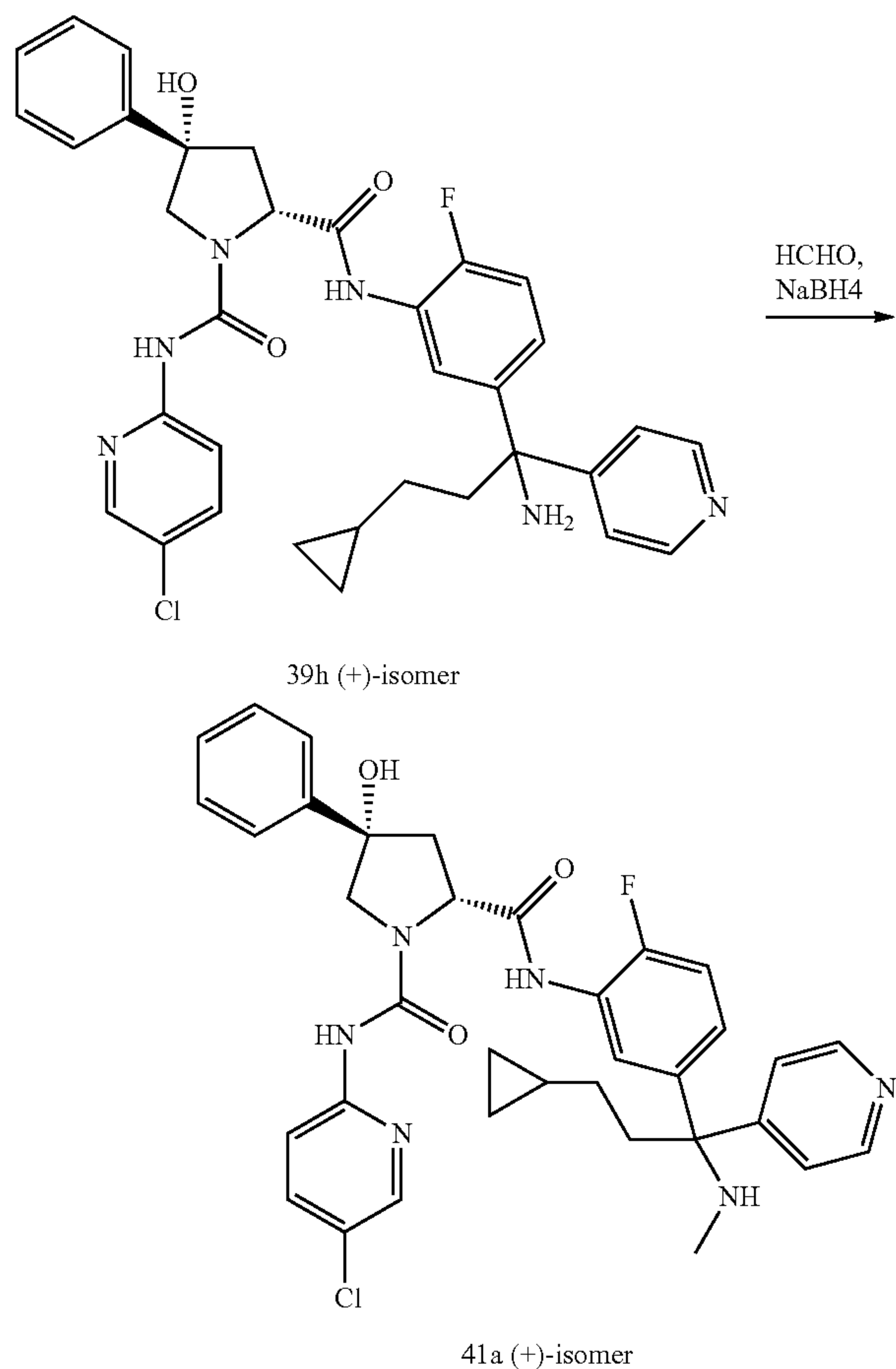
Scheme 41
