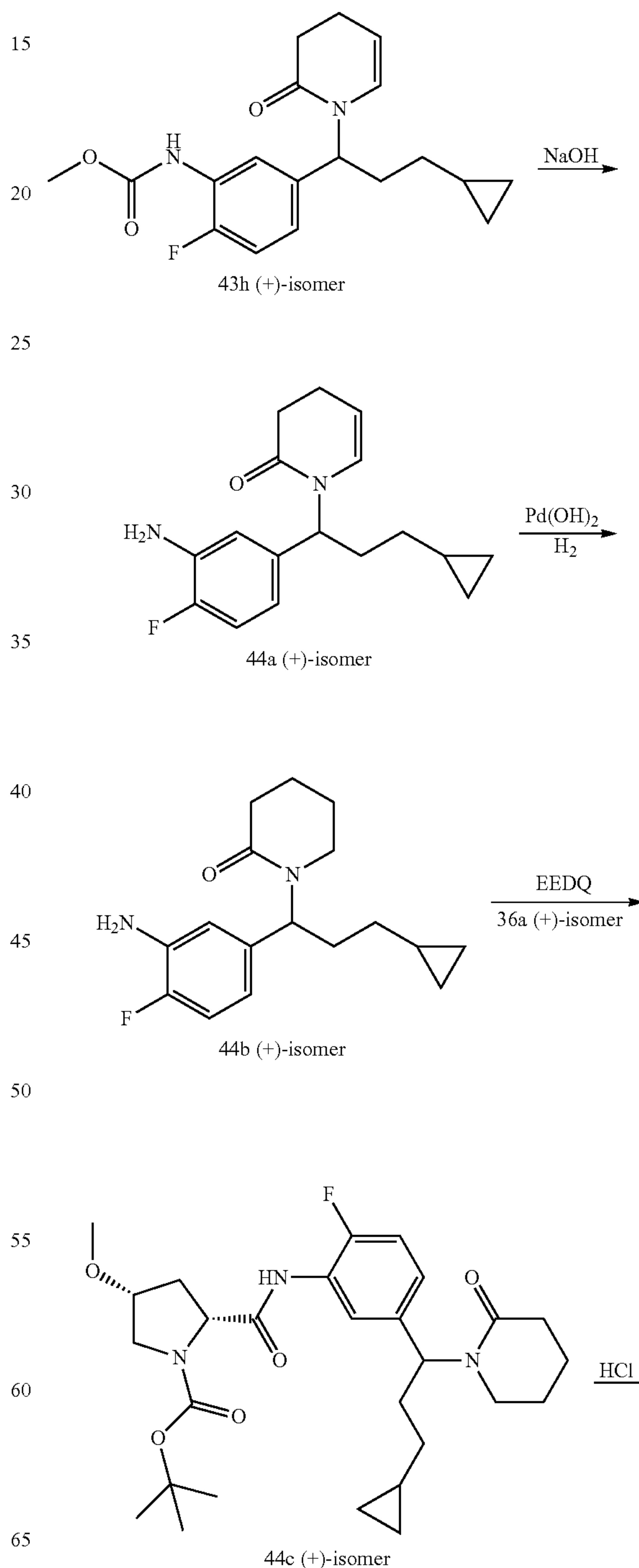
Scheme 44
