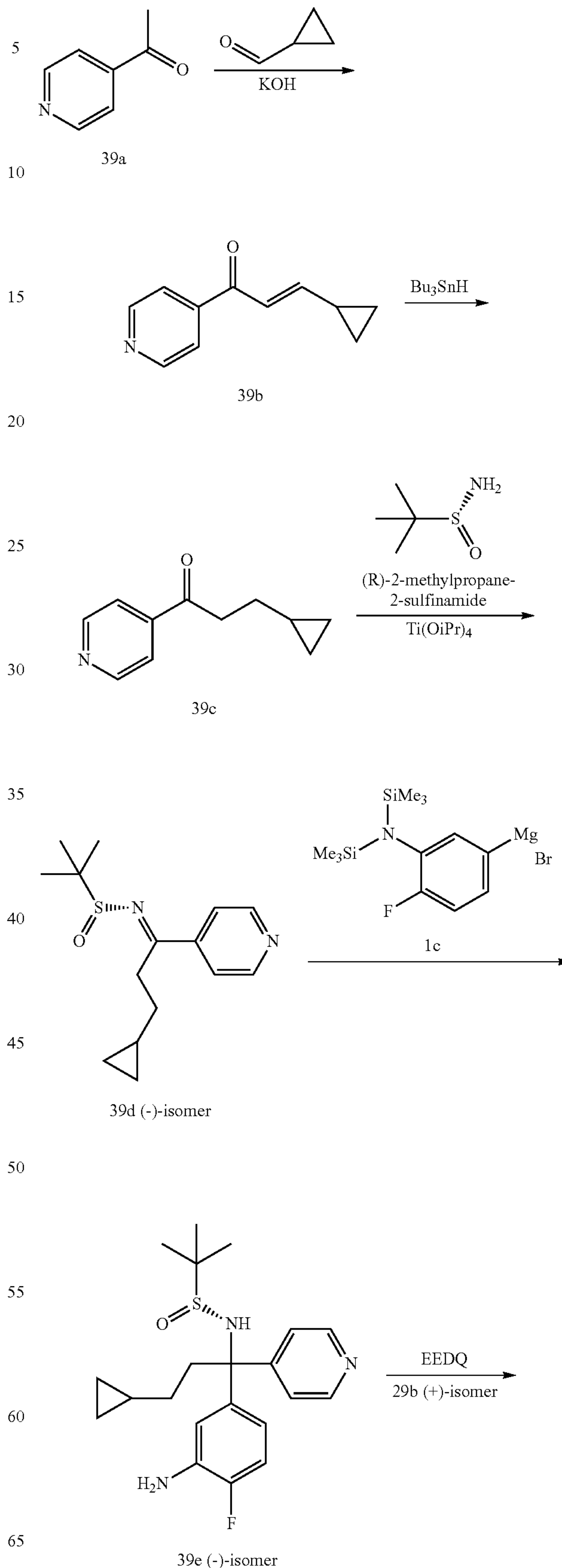
Scheme 39
