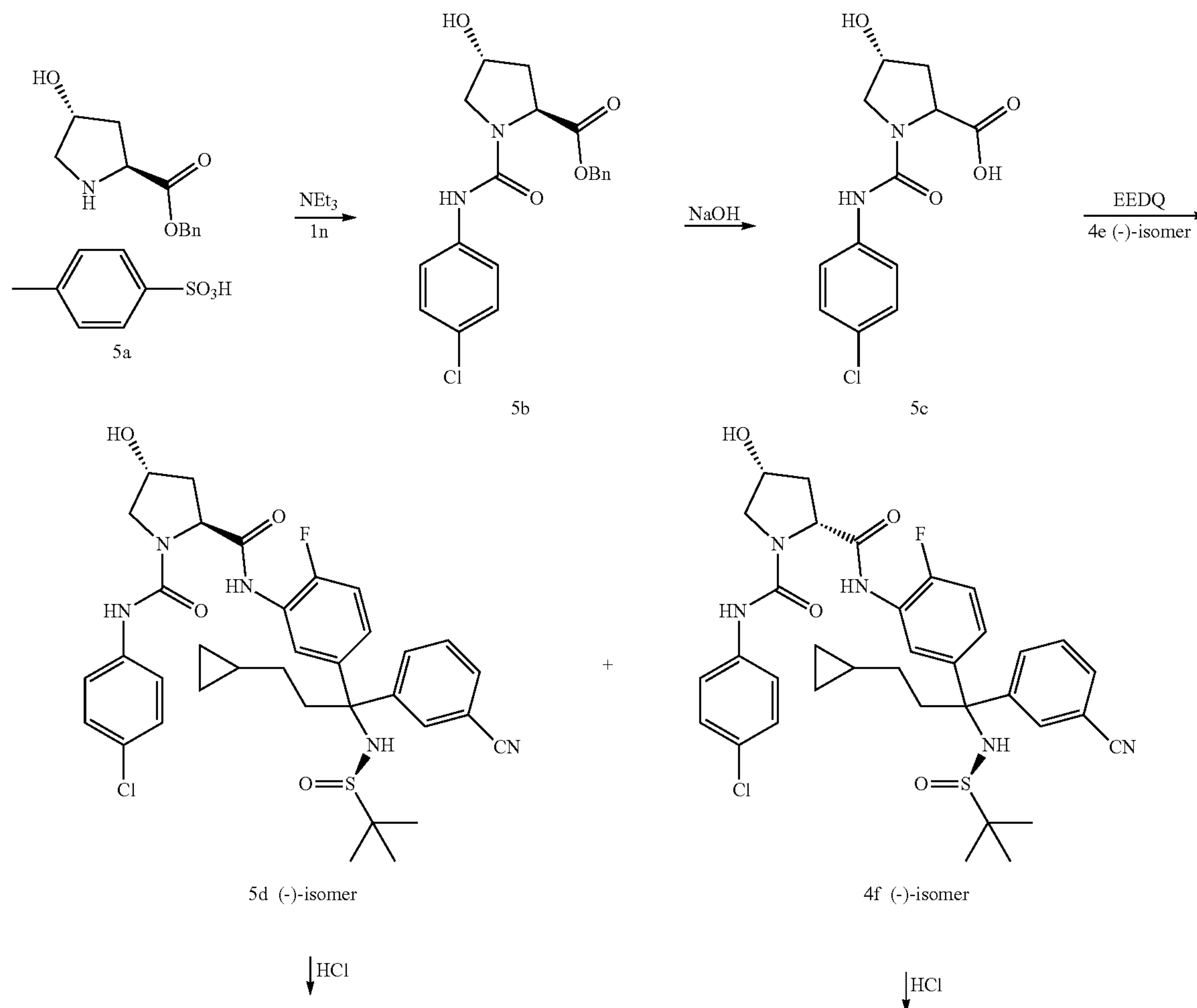
Scheme 5
