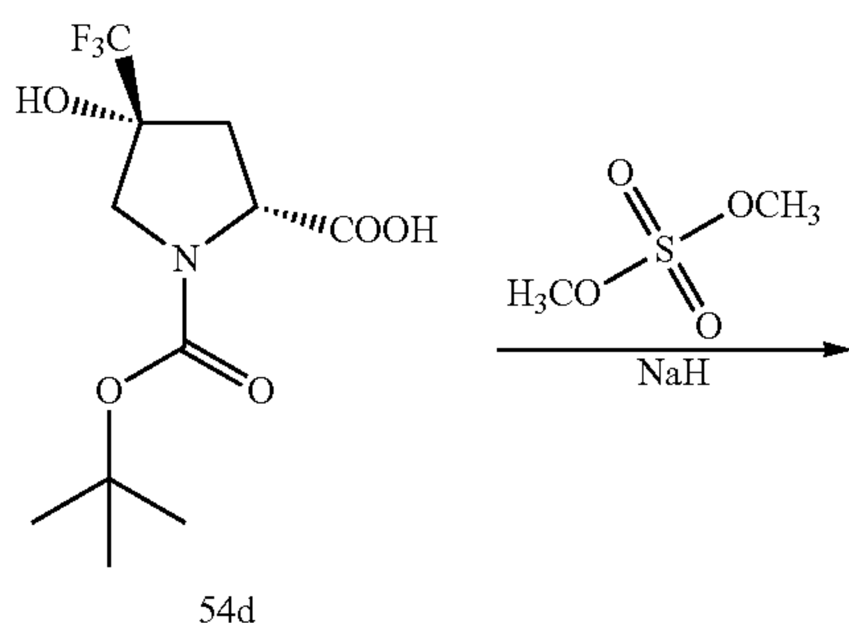
Scheme 57
