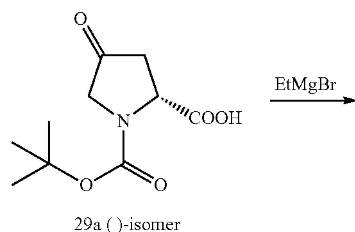
Scheme 38
