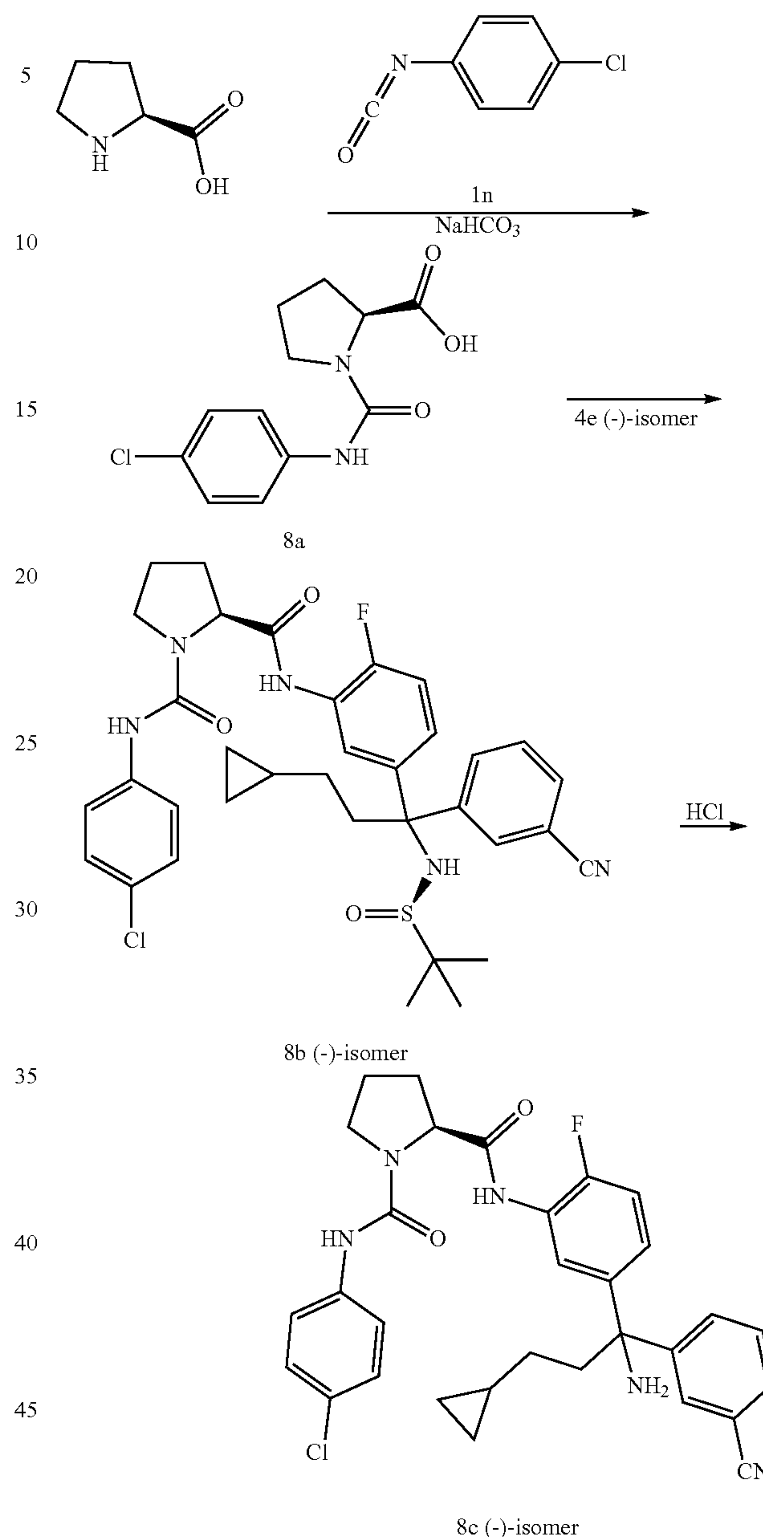
Scheme 8
