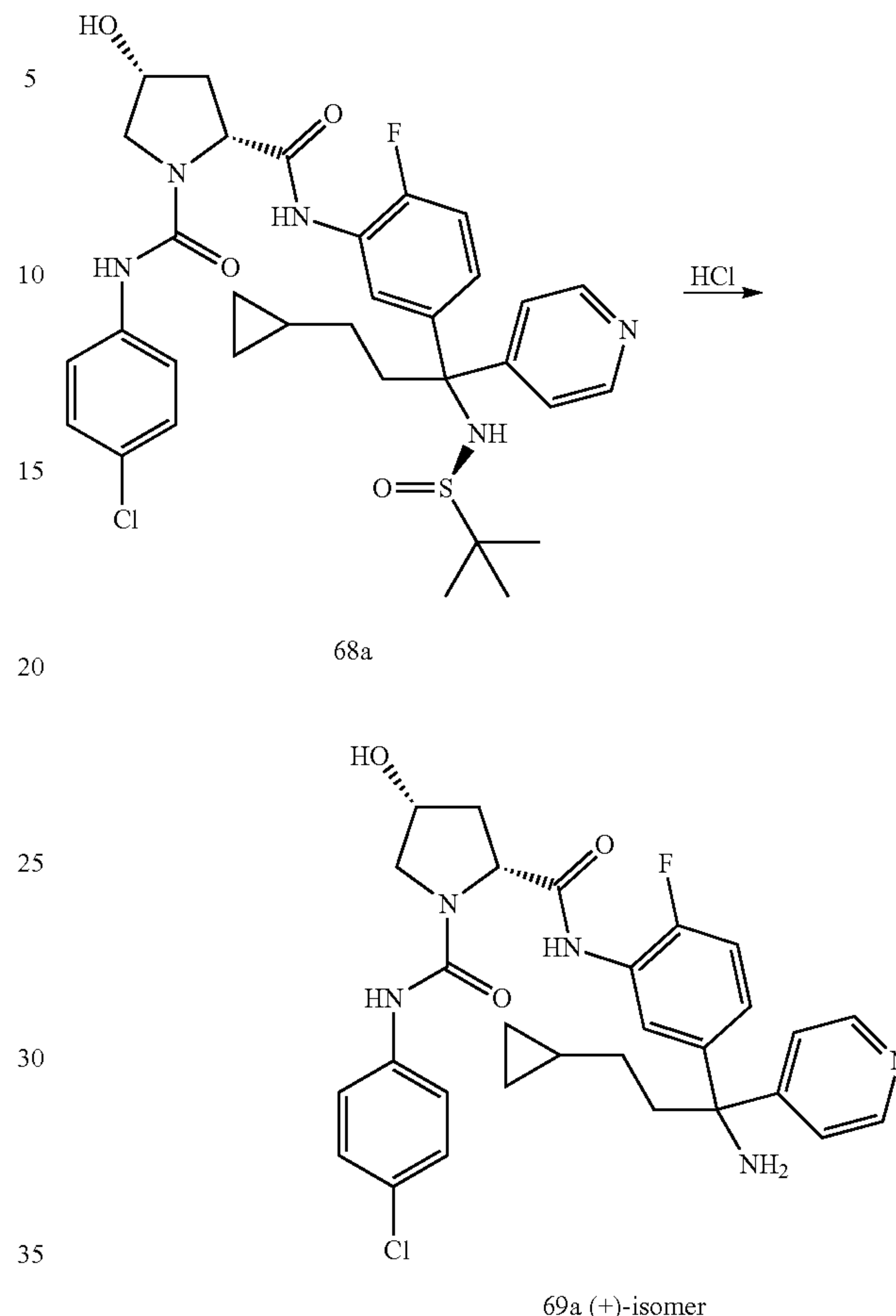
Scheme 69
