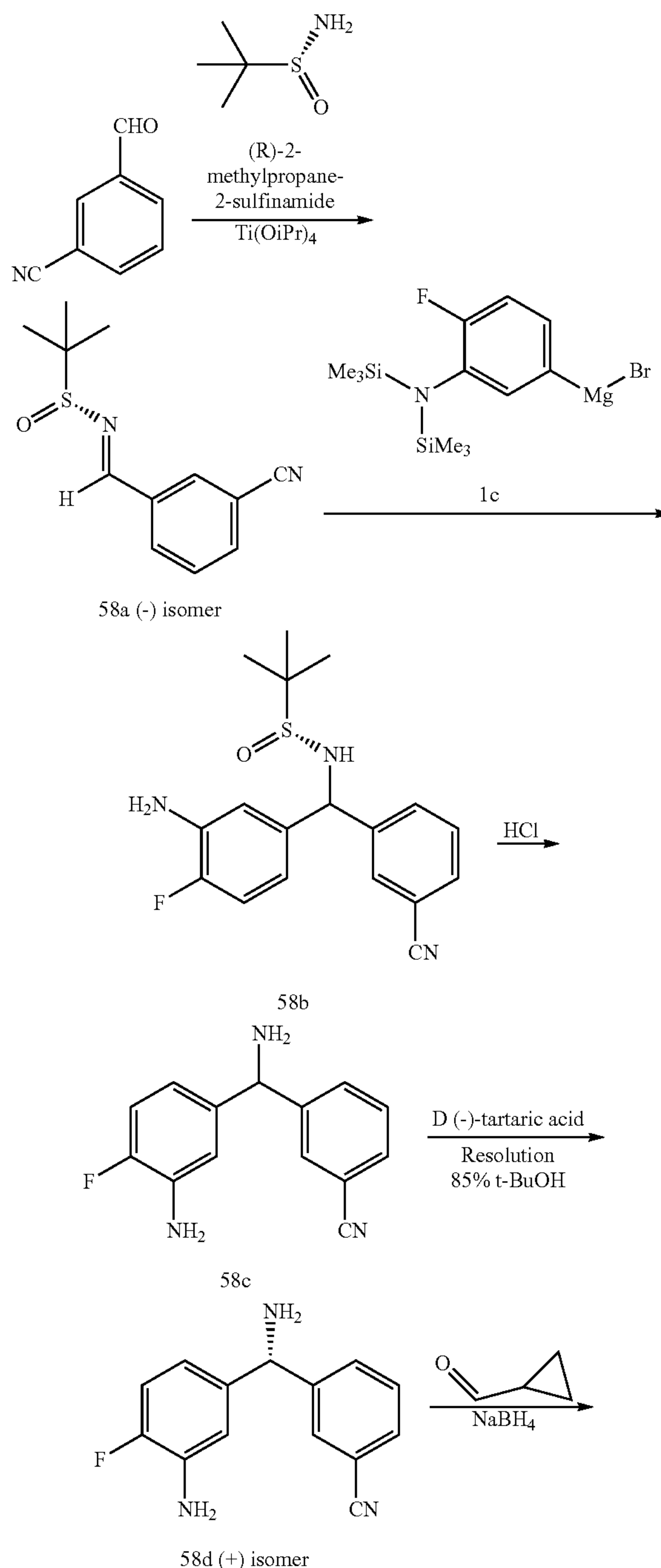
Scheme 58
