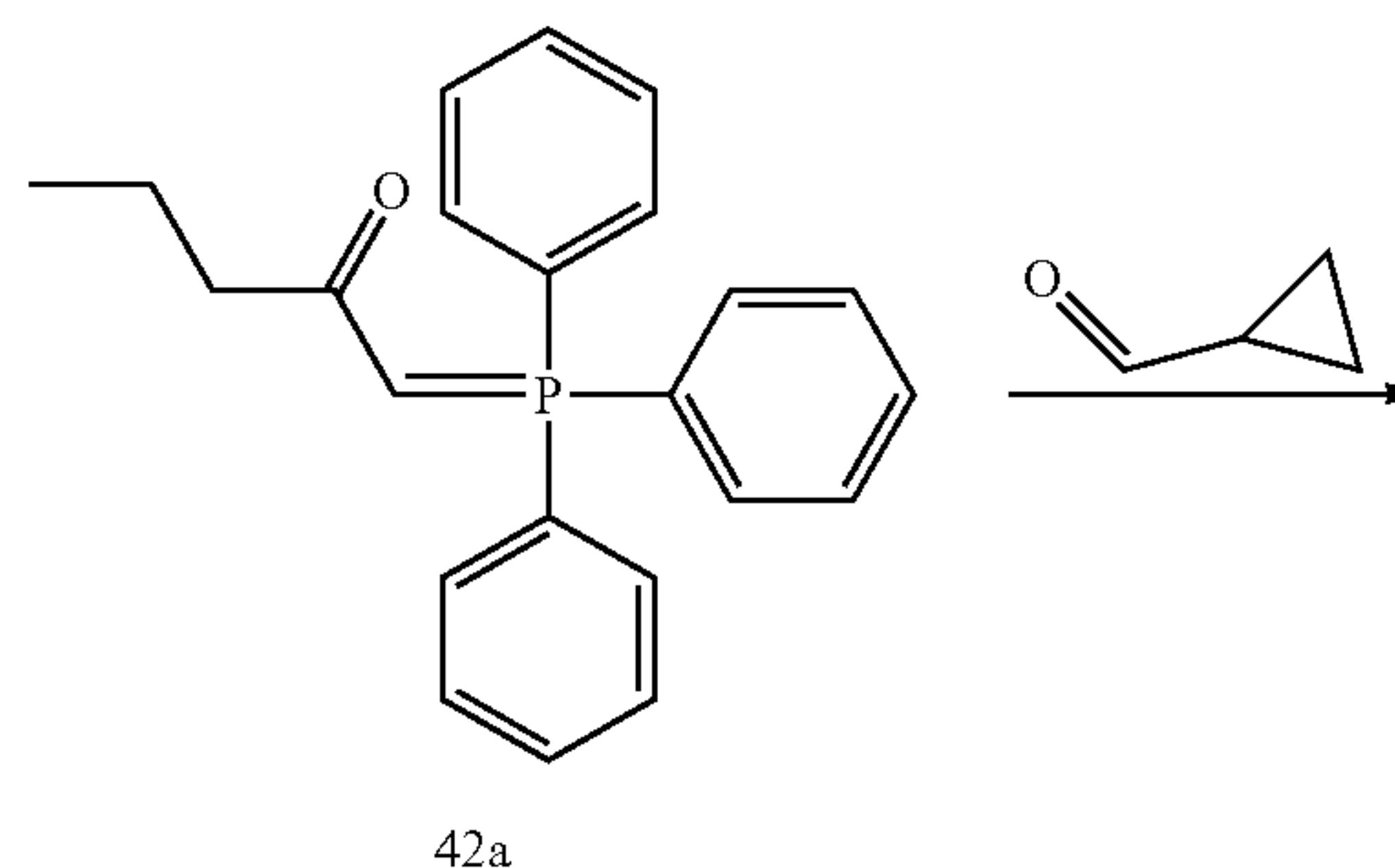
Scheme 42
