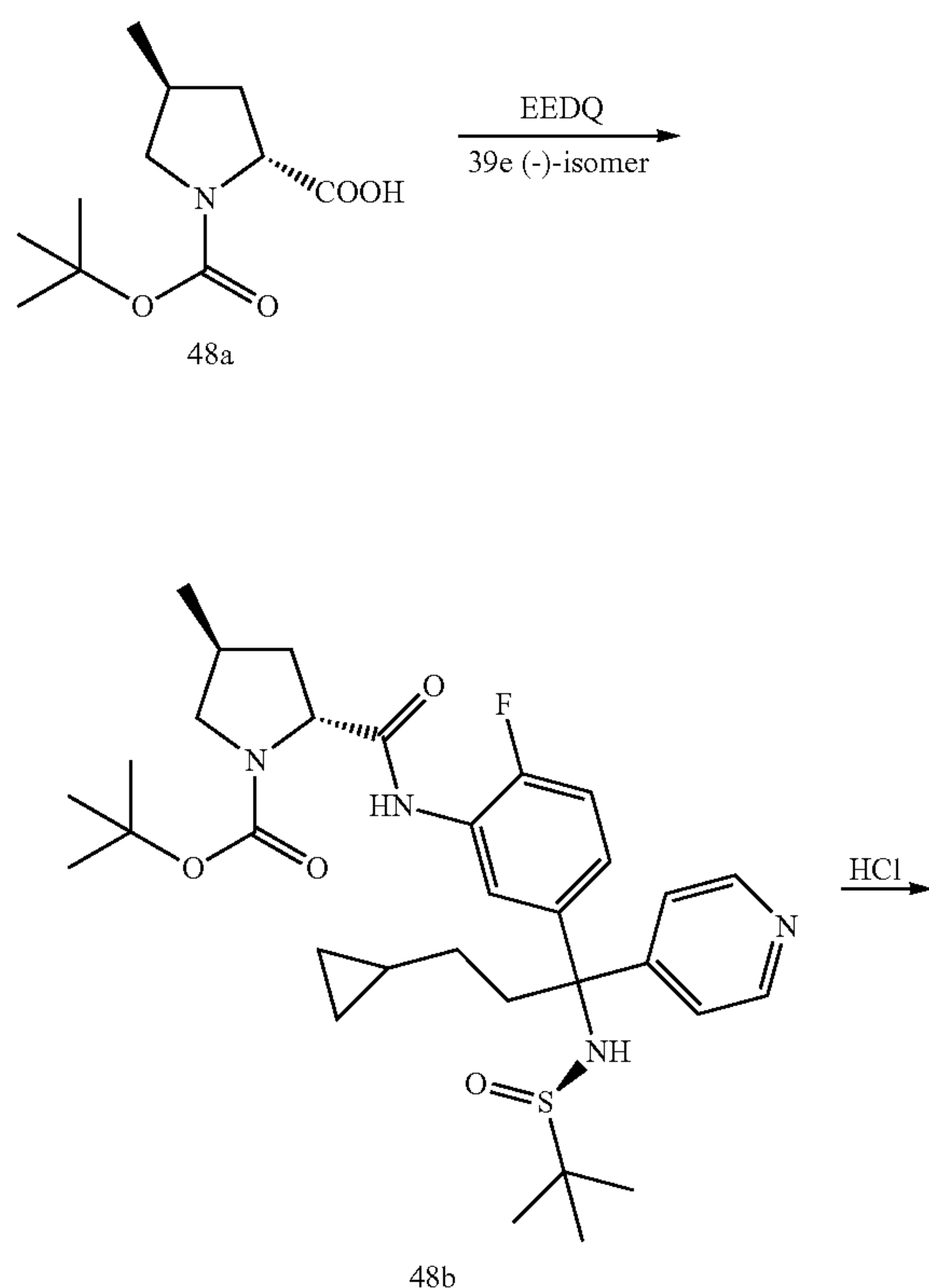
Scheme 48
