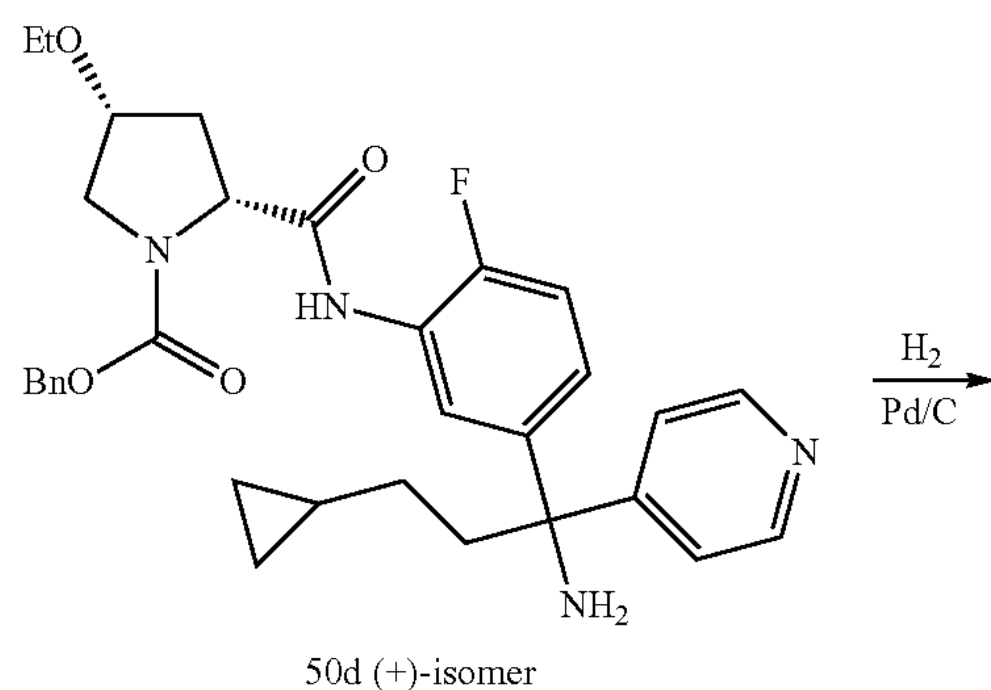
Scheme 51
