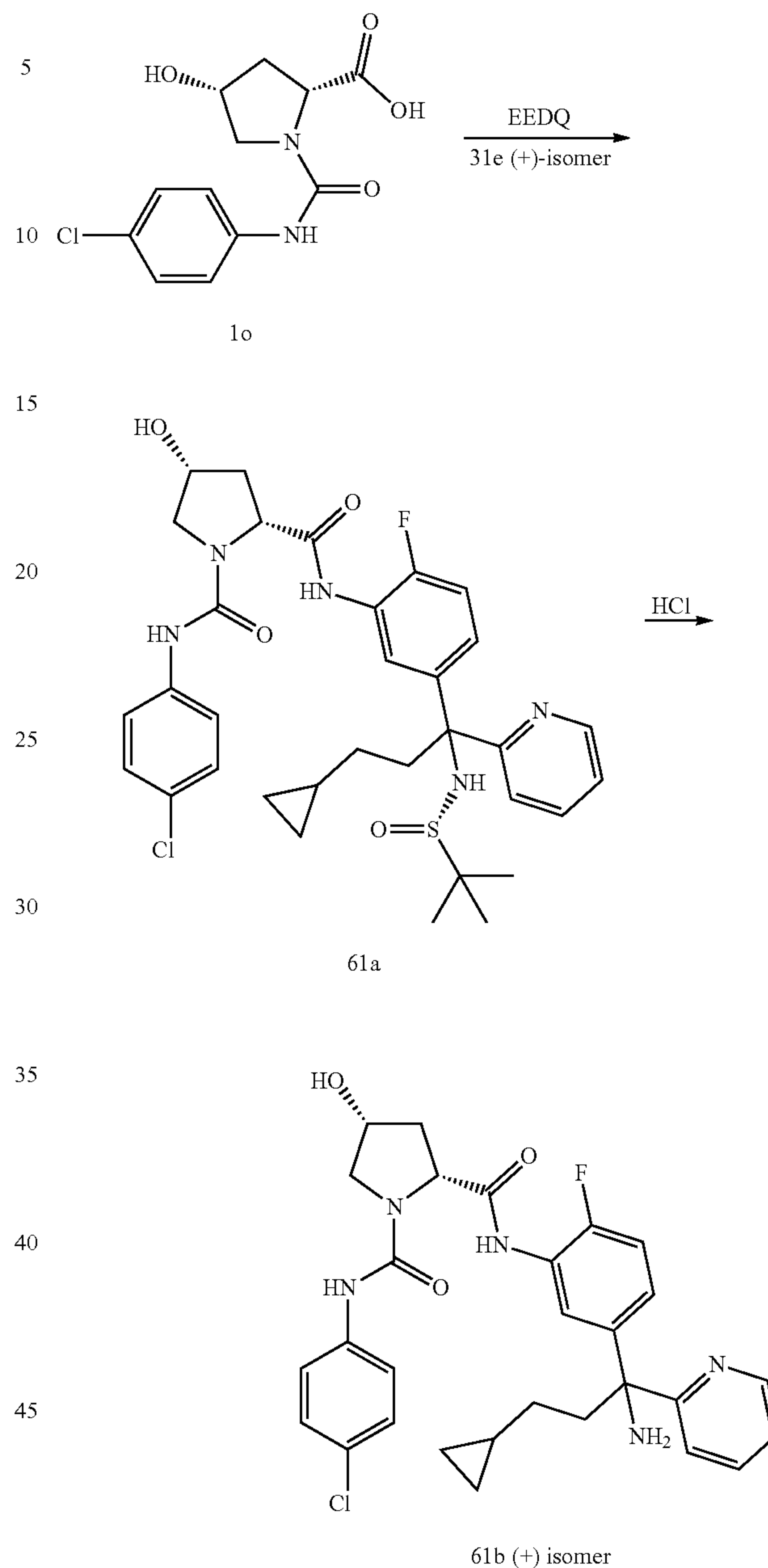
Scheme 61
