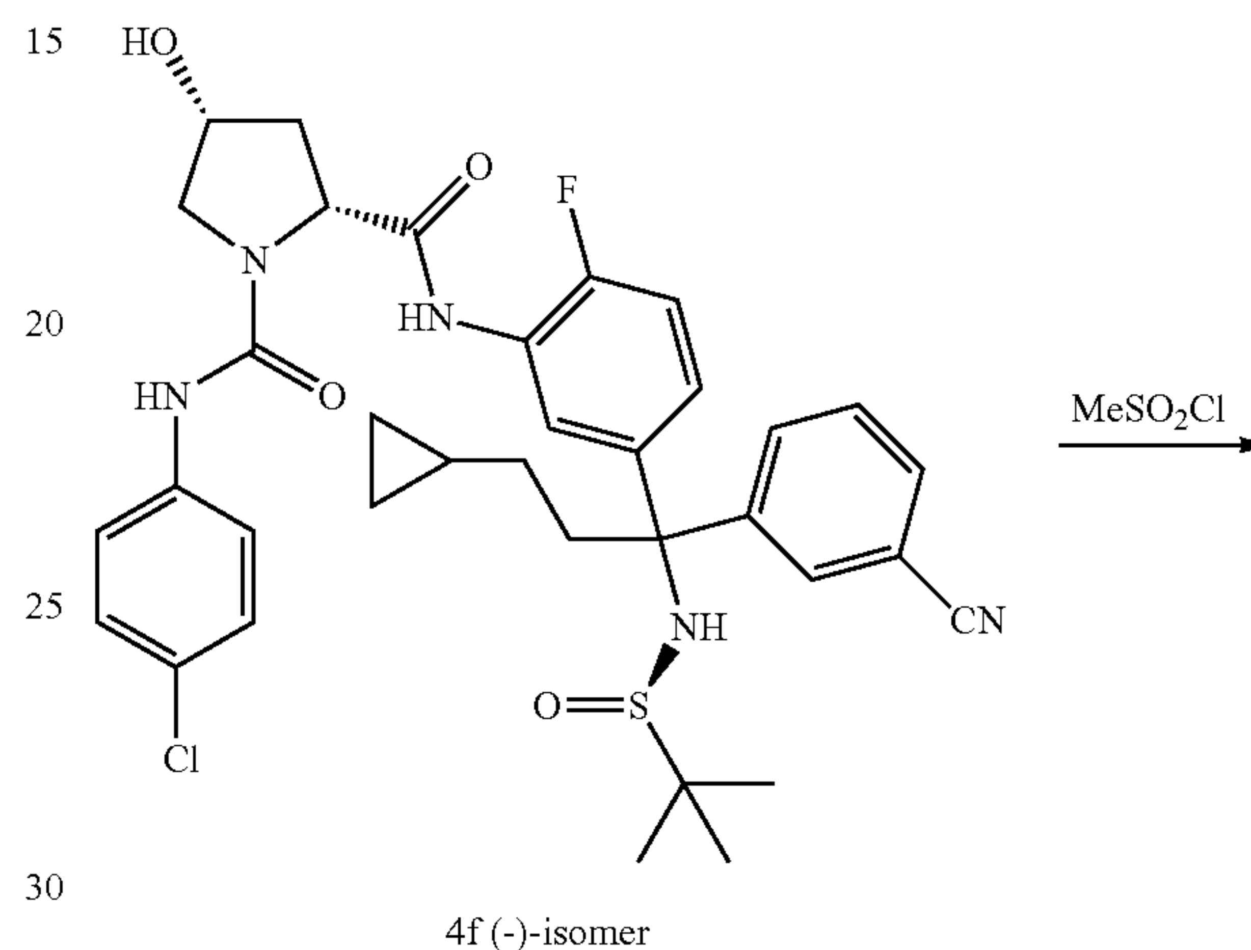
Scheme 33
