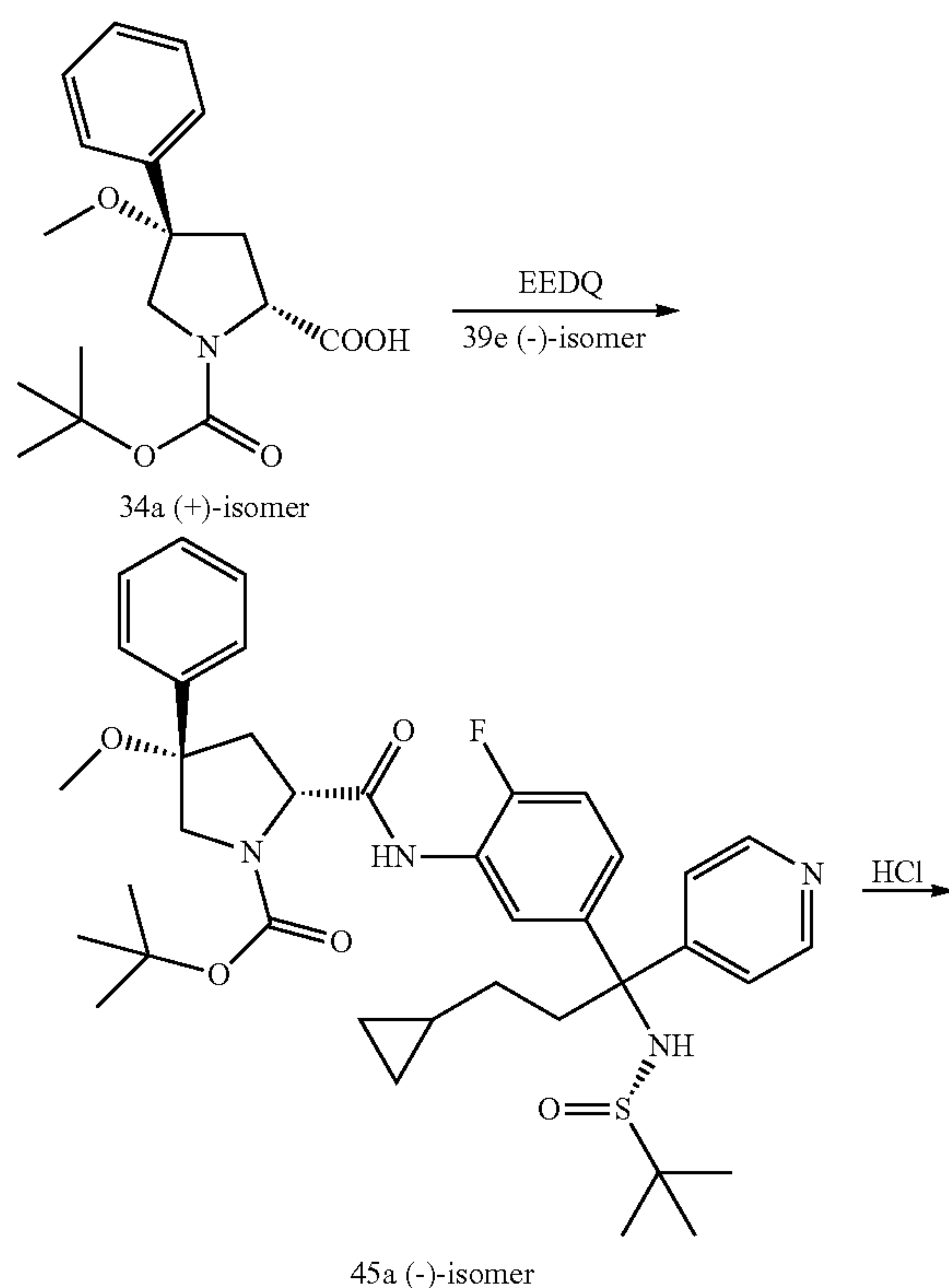
Scheme 45
