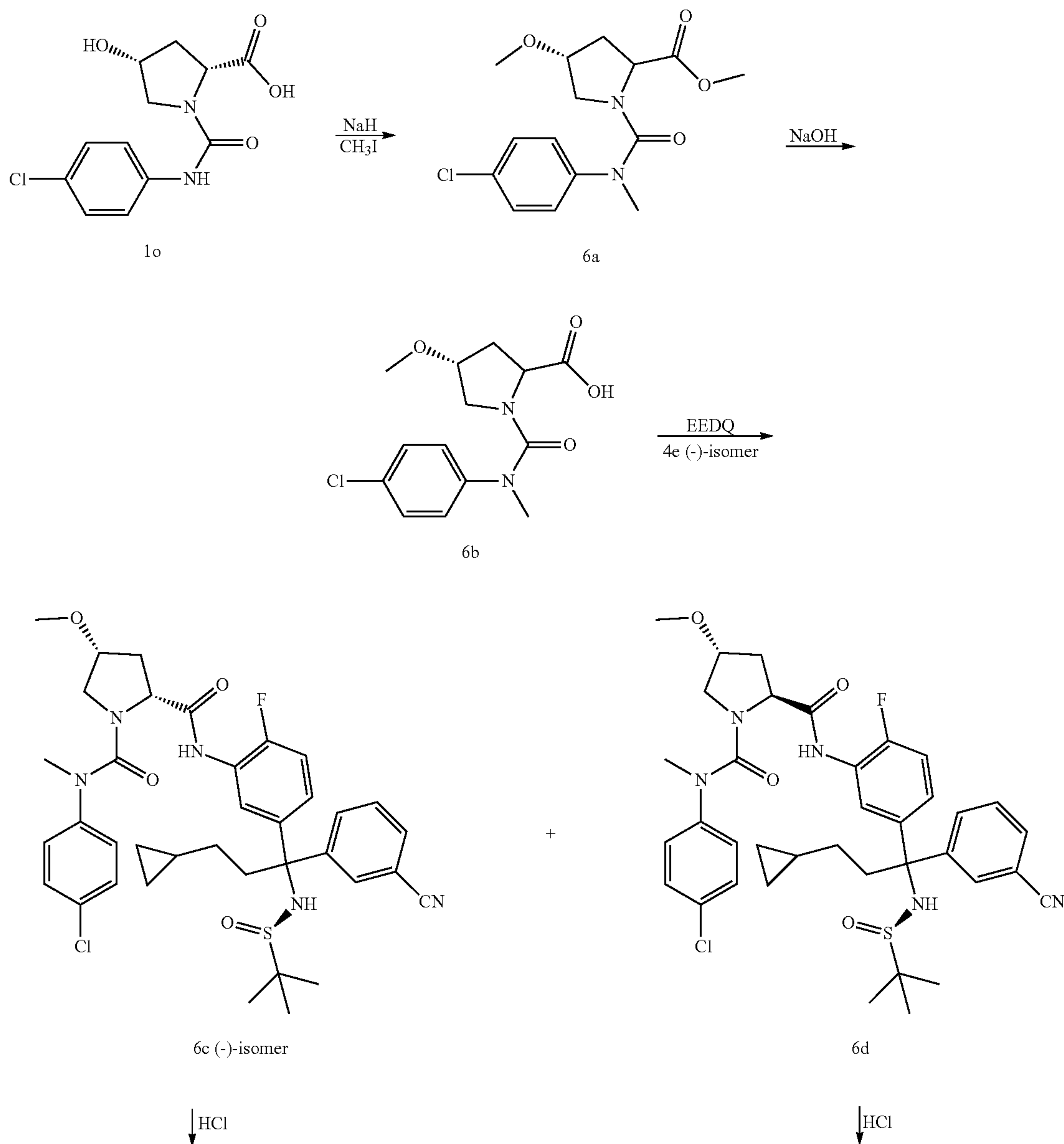
Scheme 6
