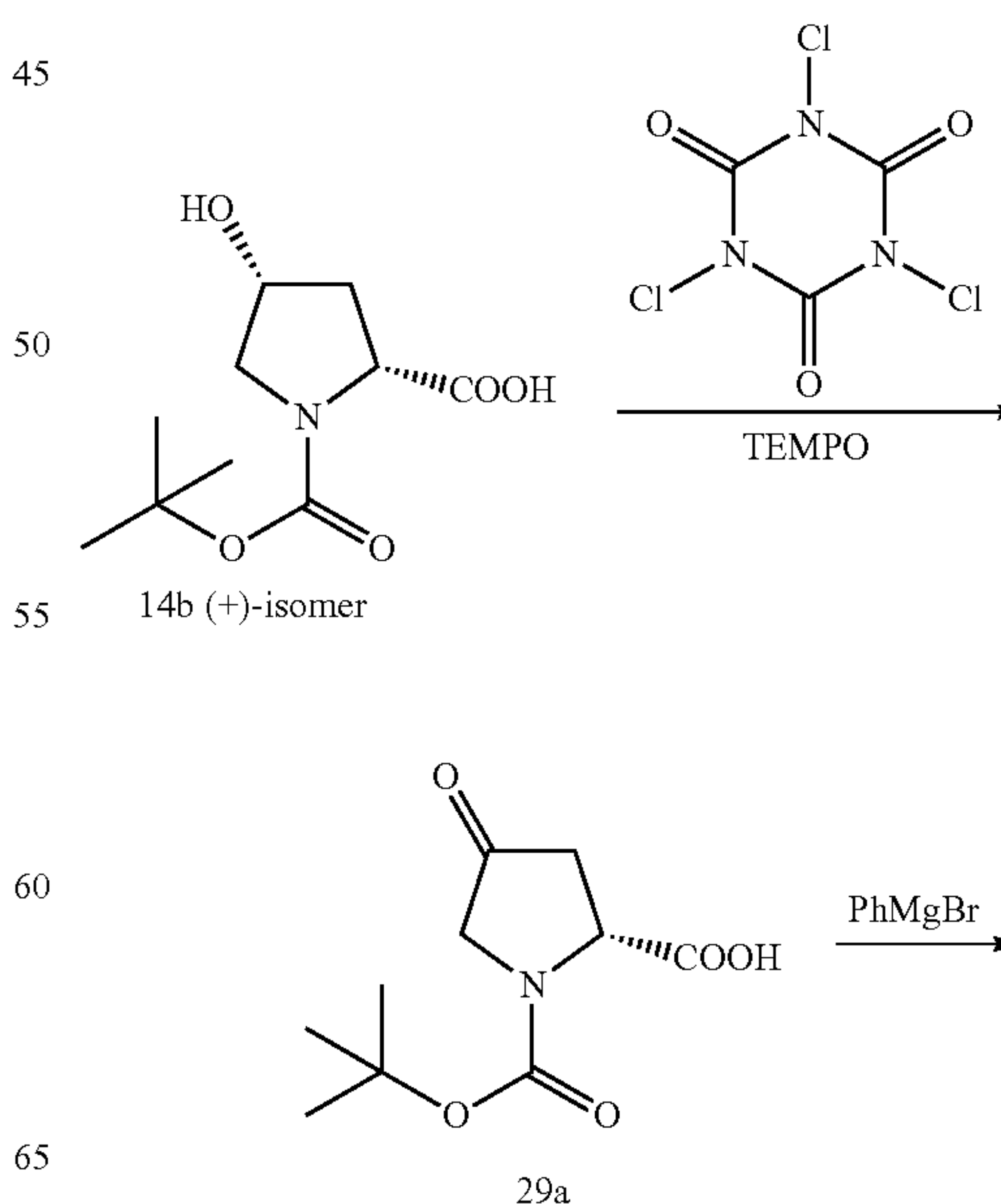
Scheme 29
