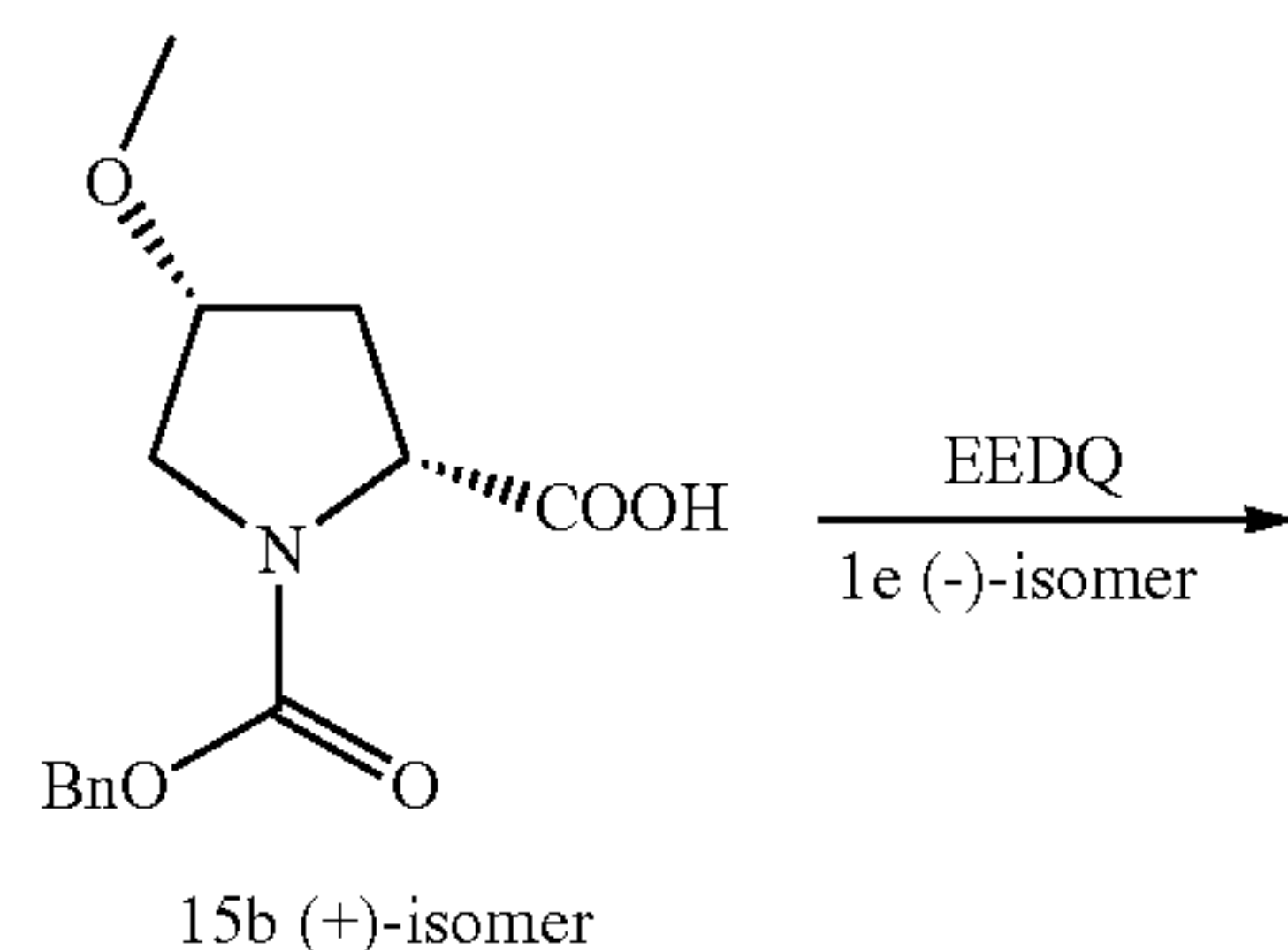
Scheme 66
