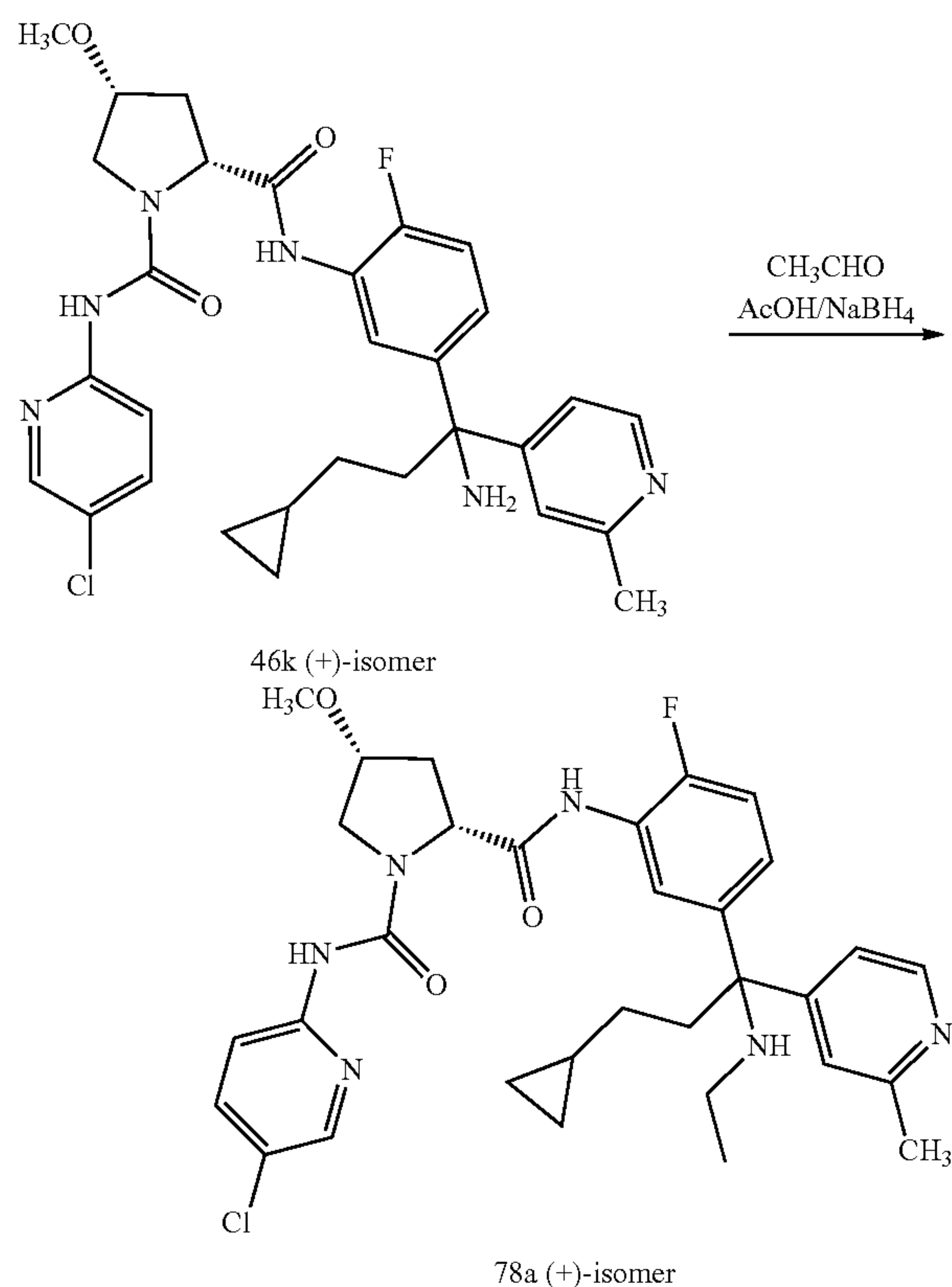
Scheme 78
