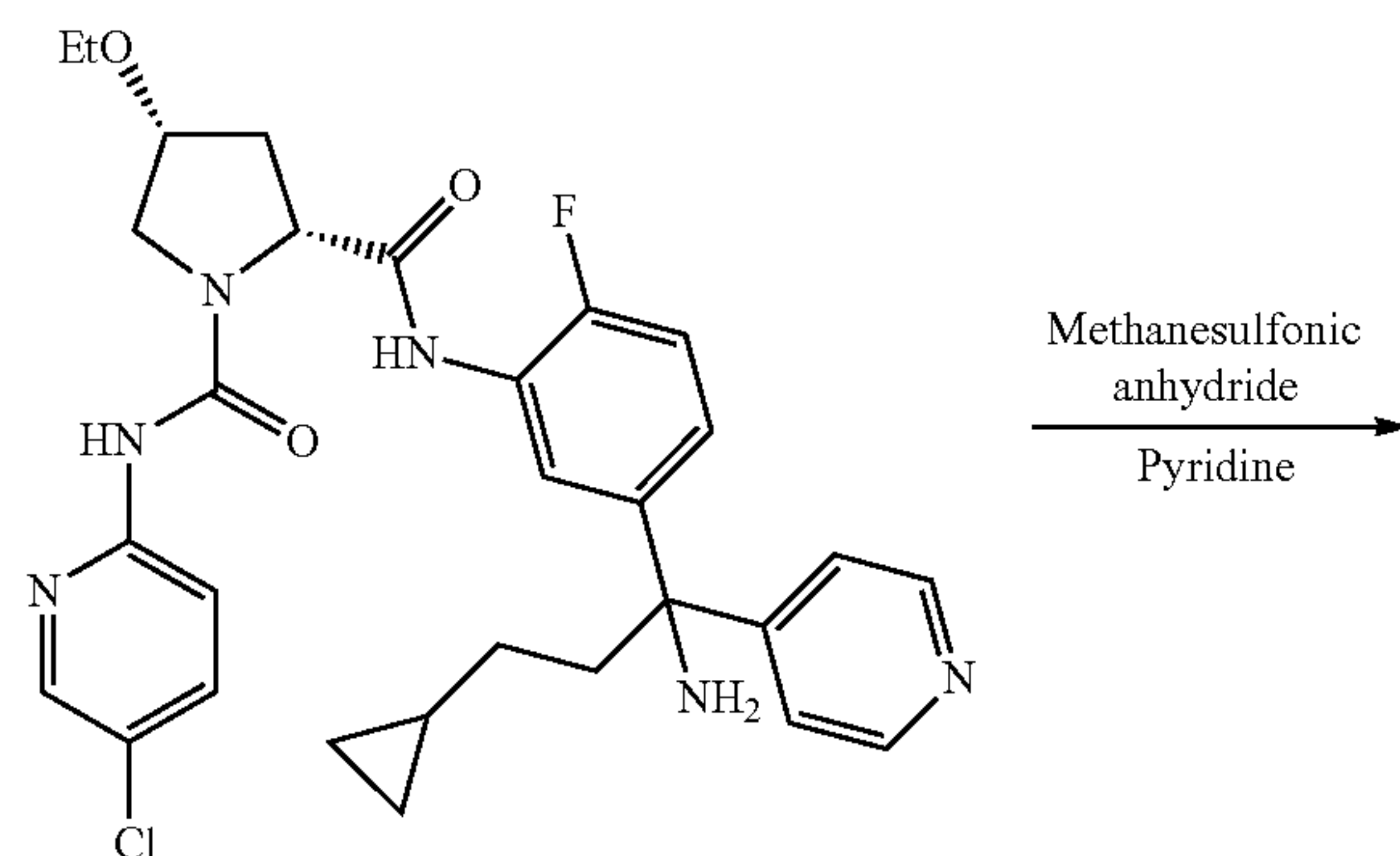
Scheme 55
