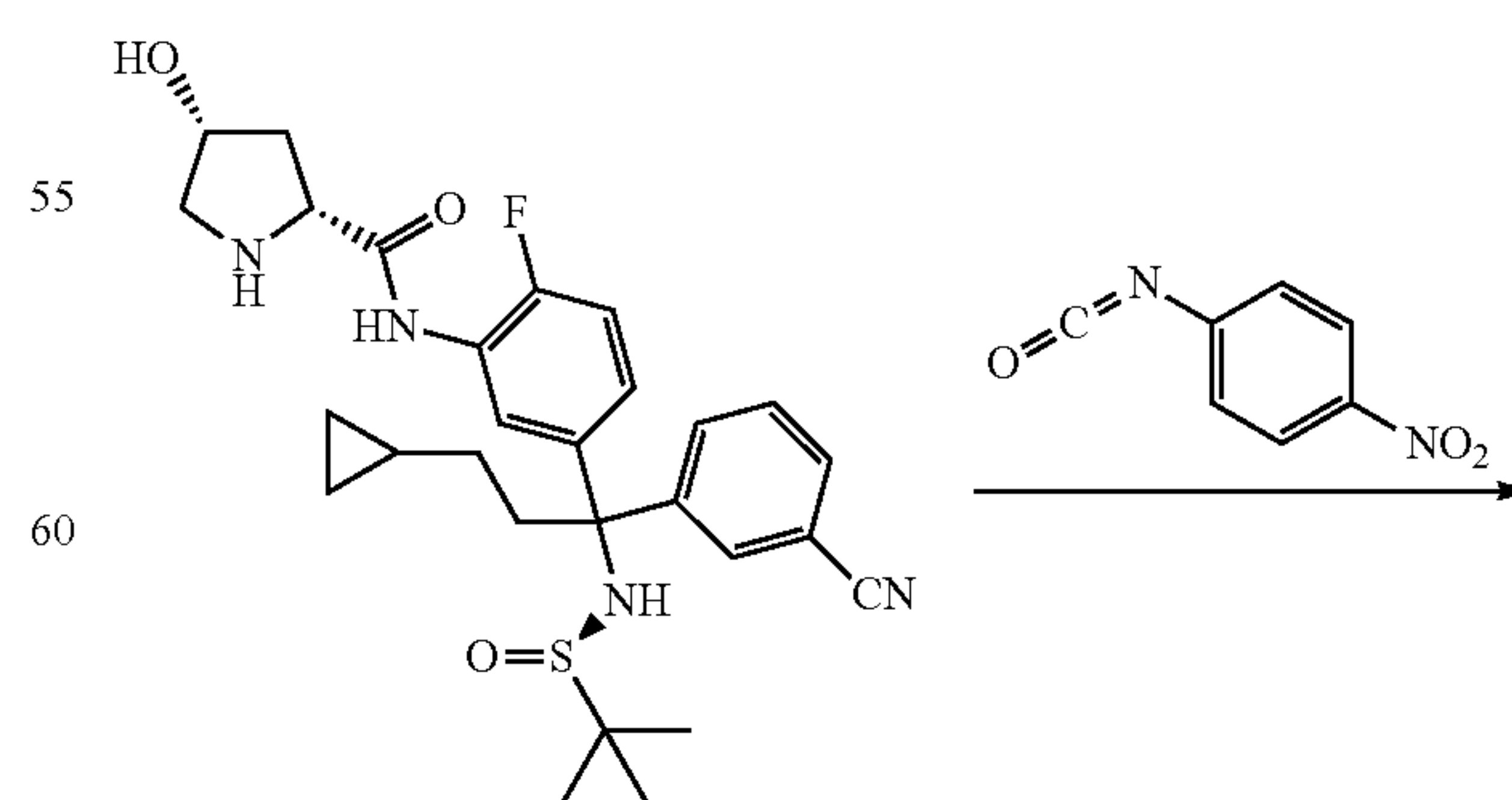
Scheme 25
