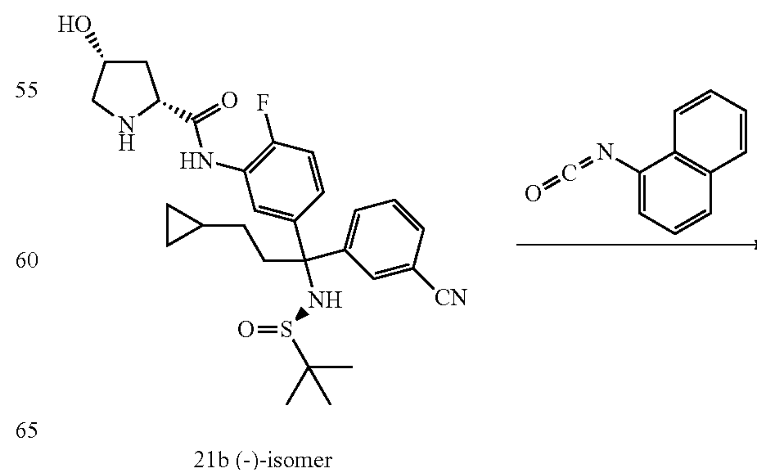
Scheme 26
