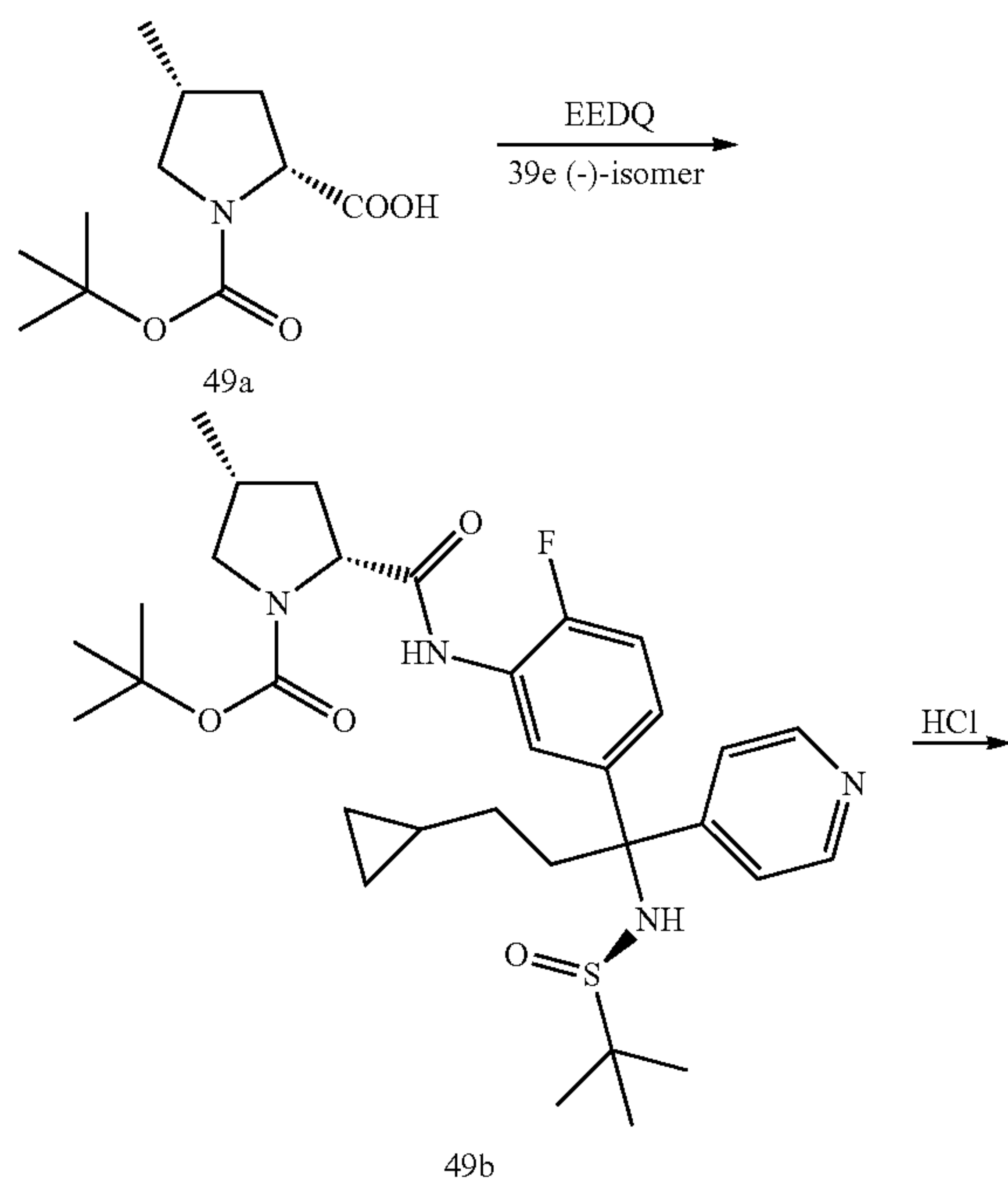
Scheme 49
