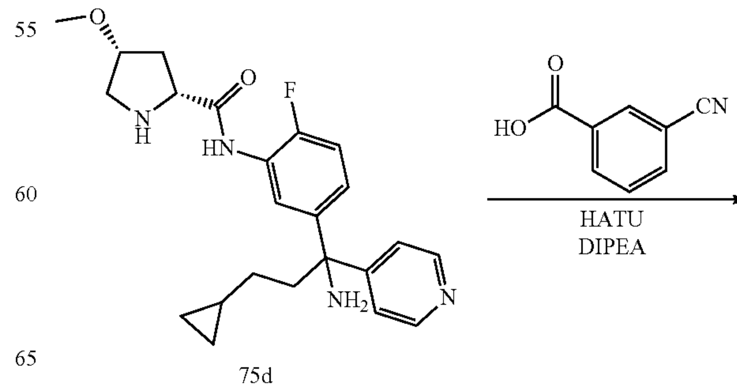
Scheme 86
