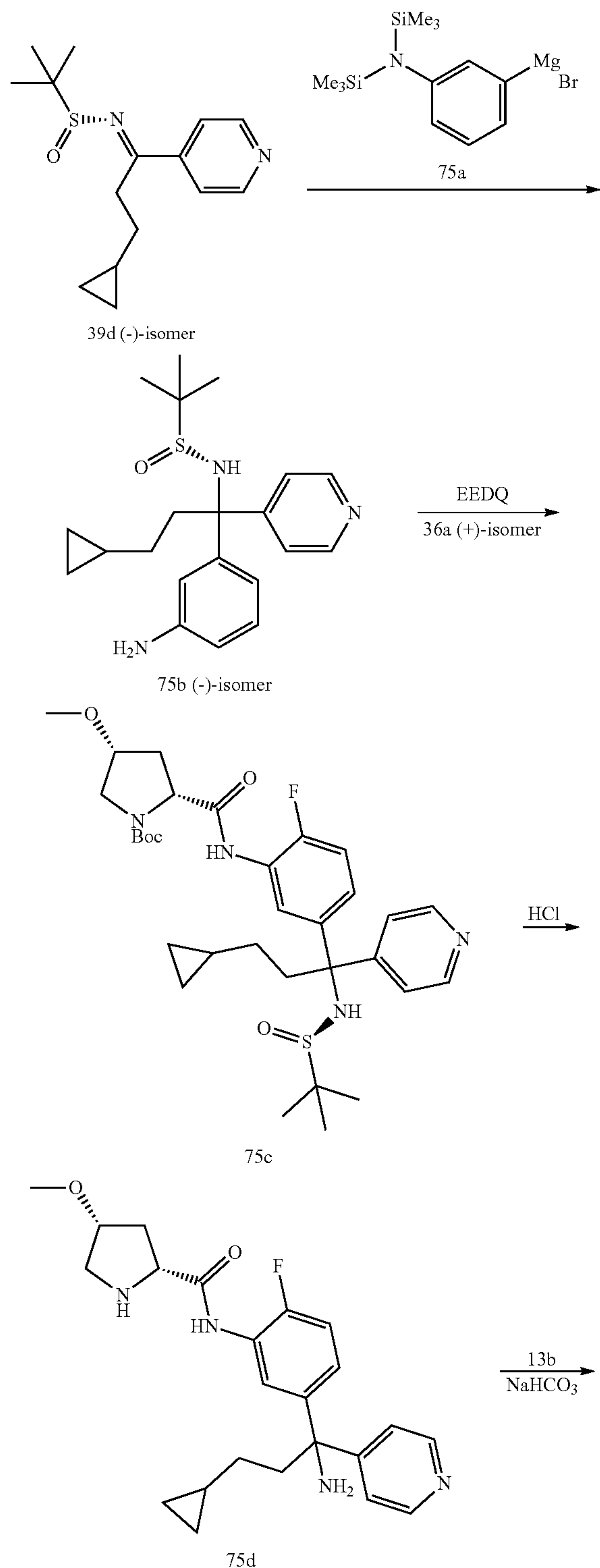
Scheme 75
