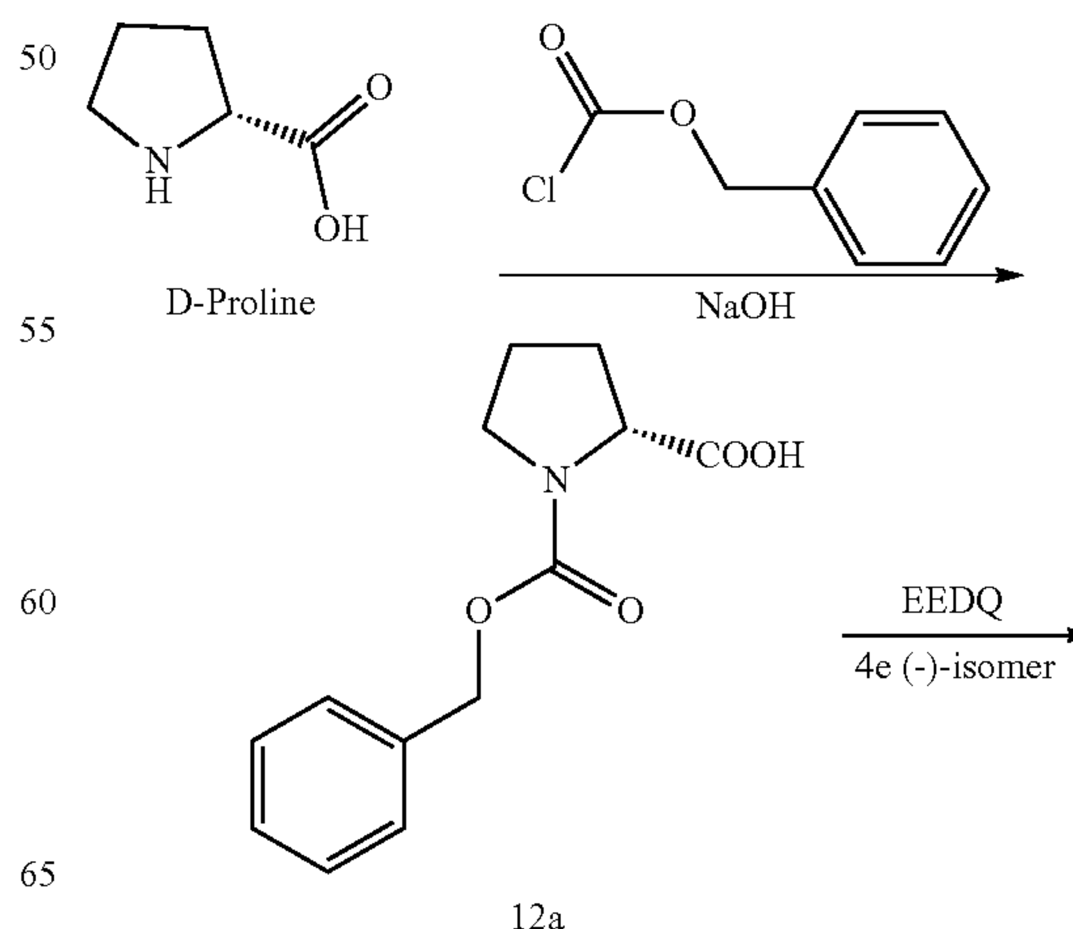
Scheme 12
