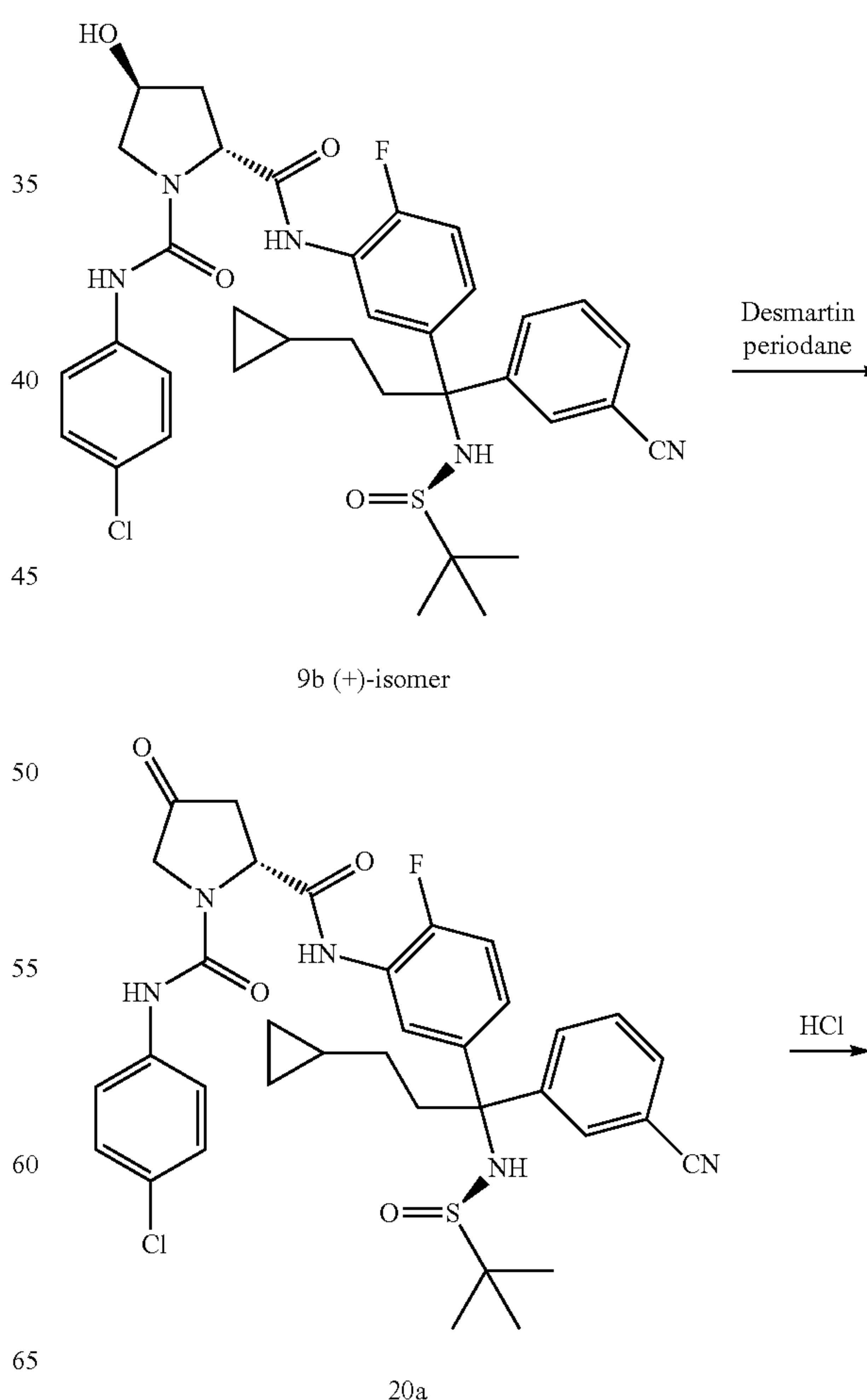
Scheme 20
