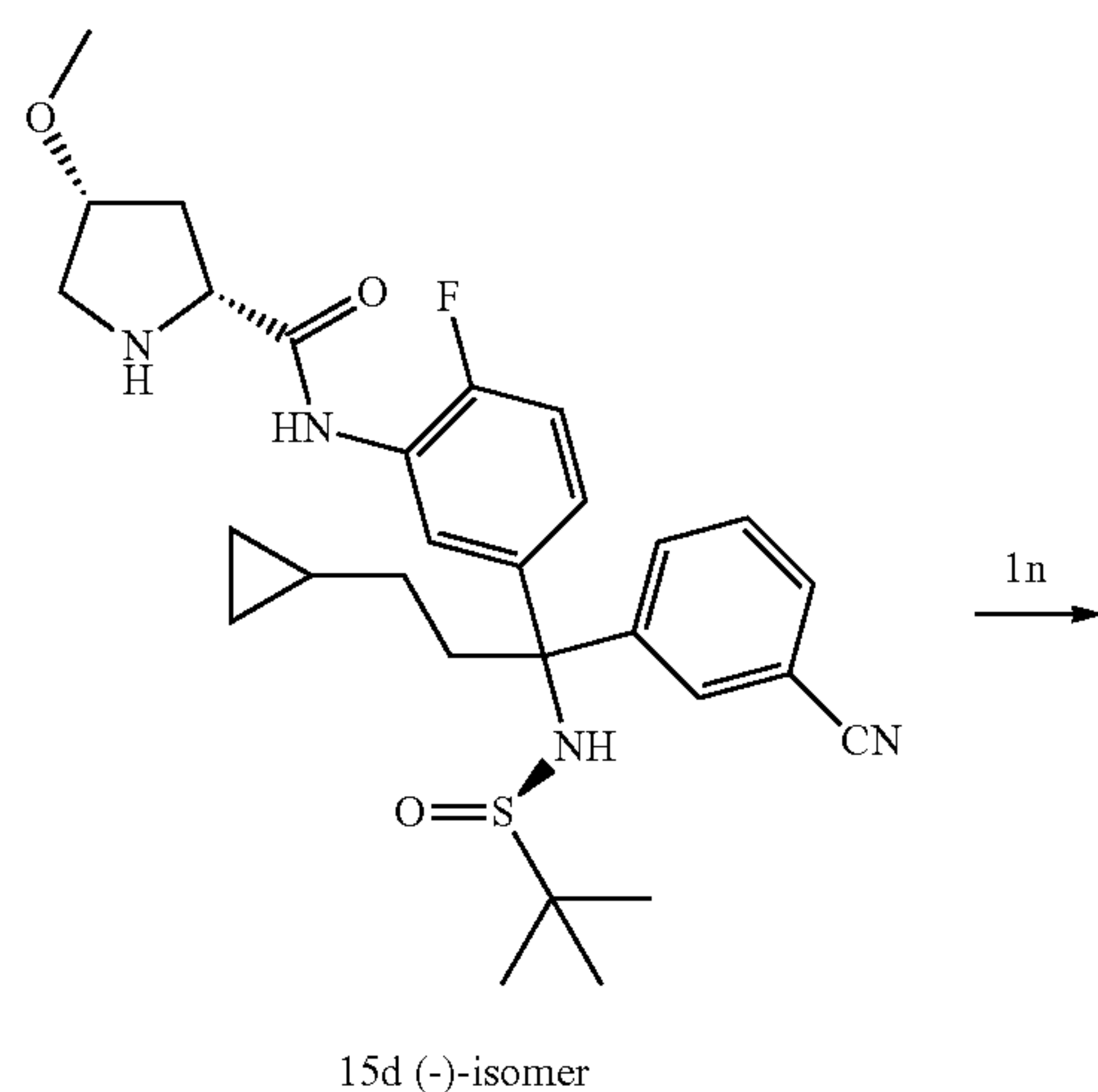
Scheme 17
