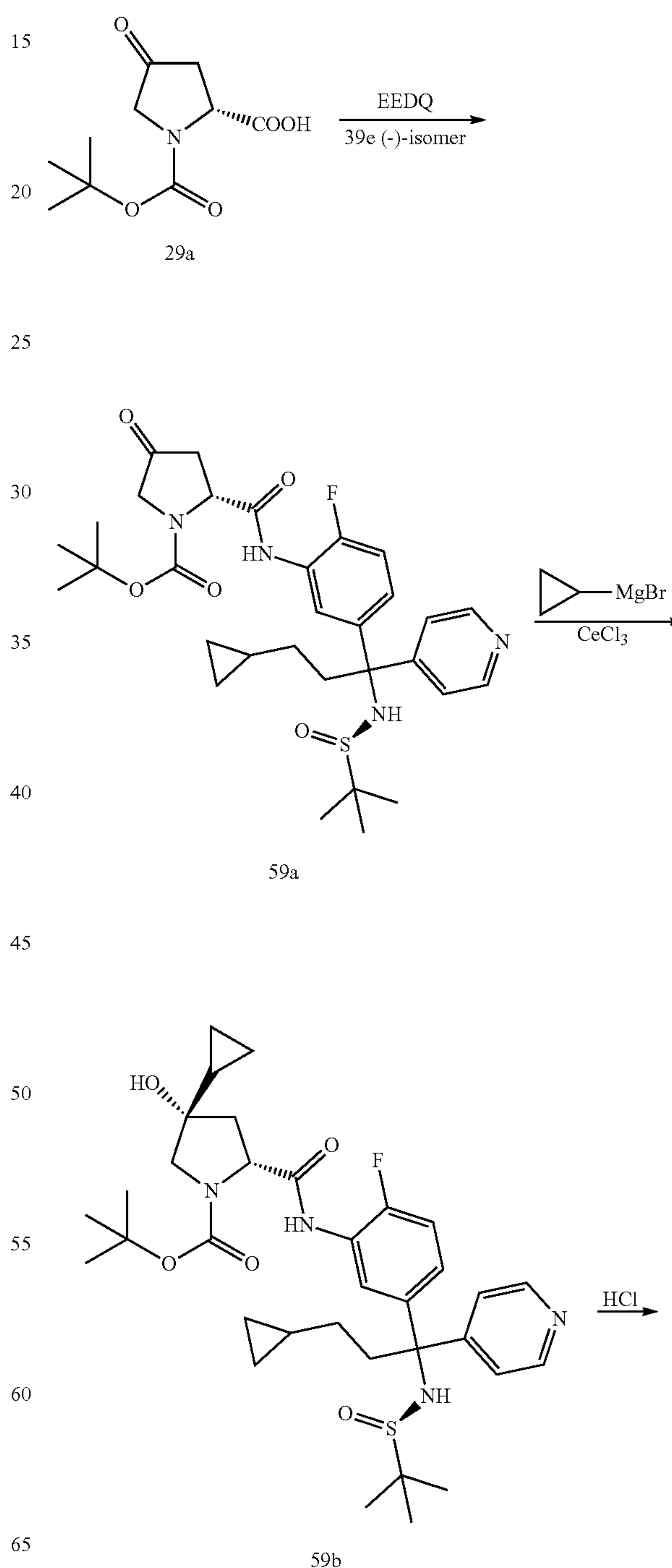
Scheme 59
