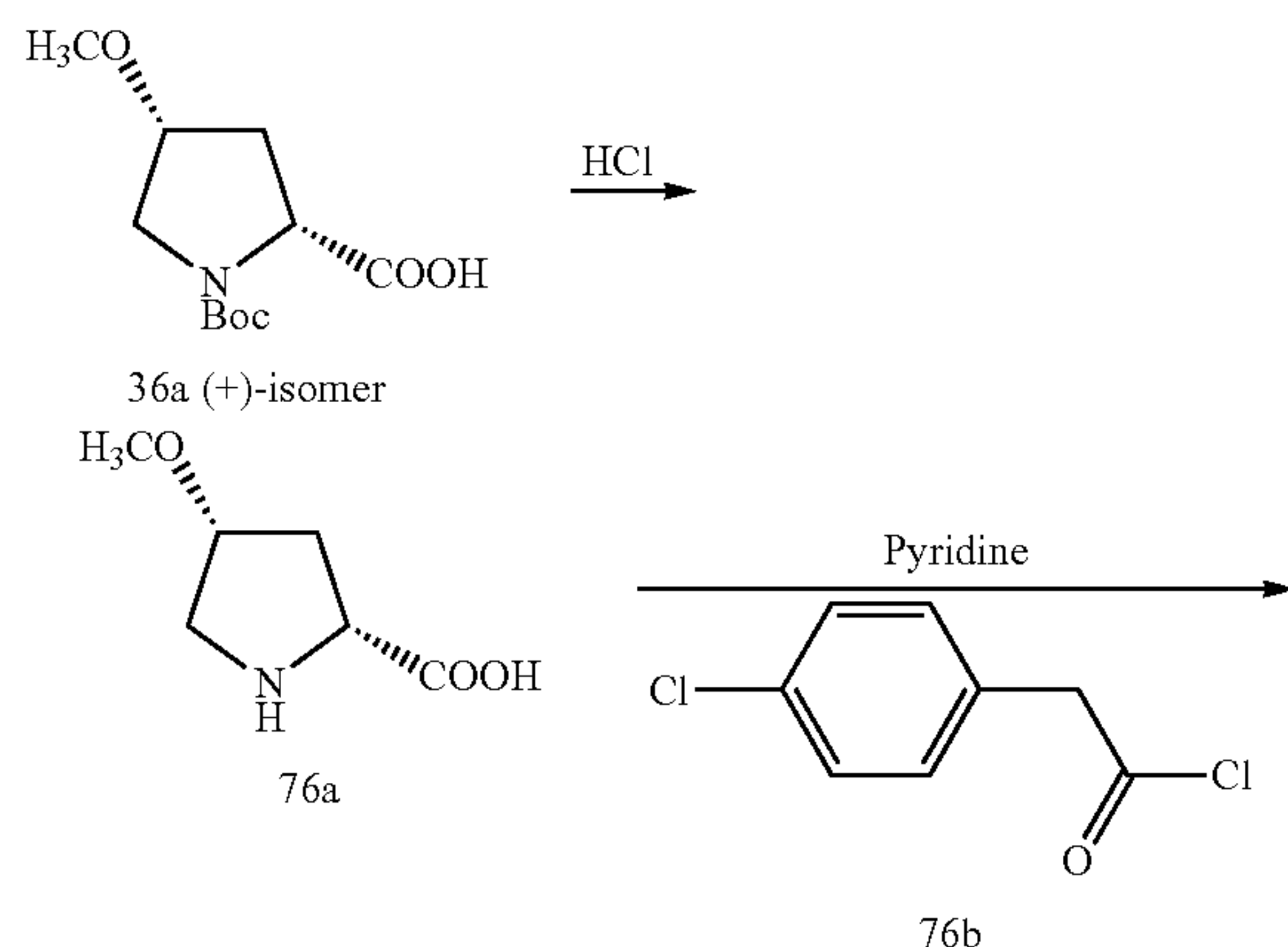
Scheme 76
