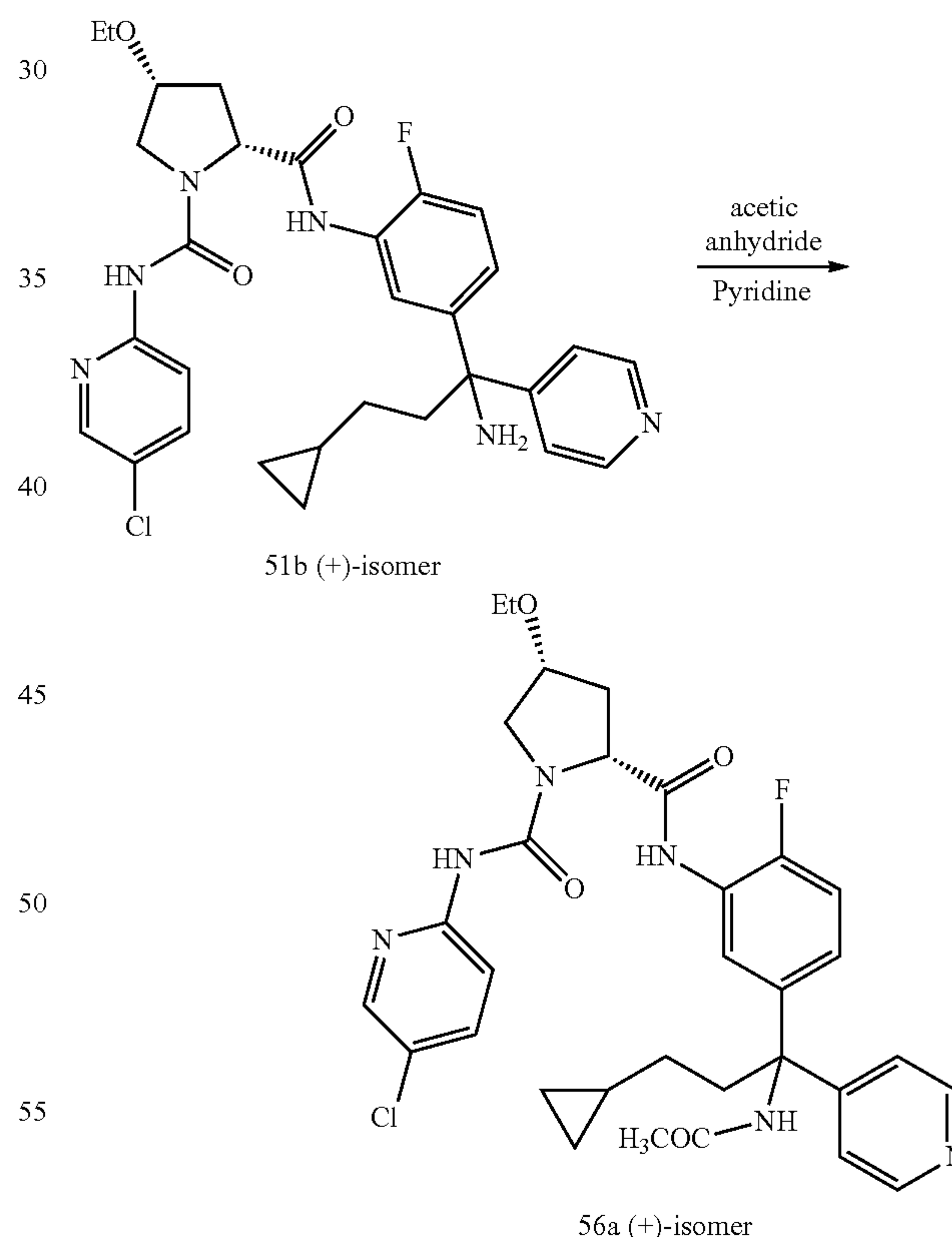
Scheme 56
