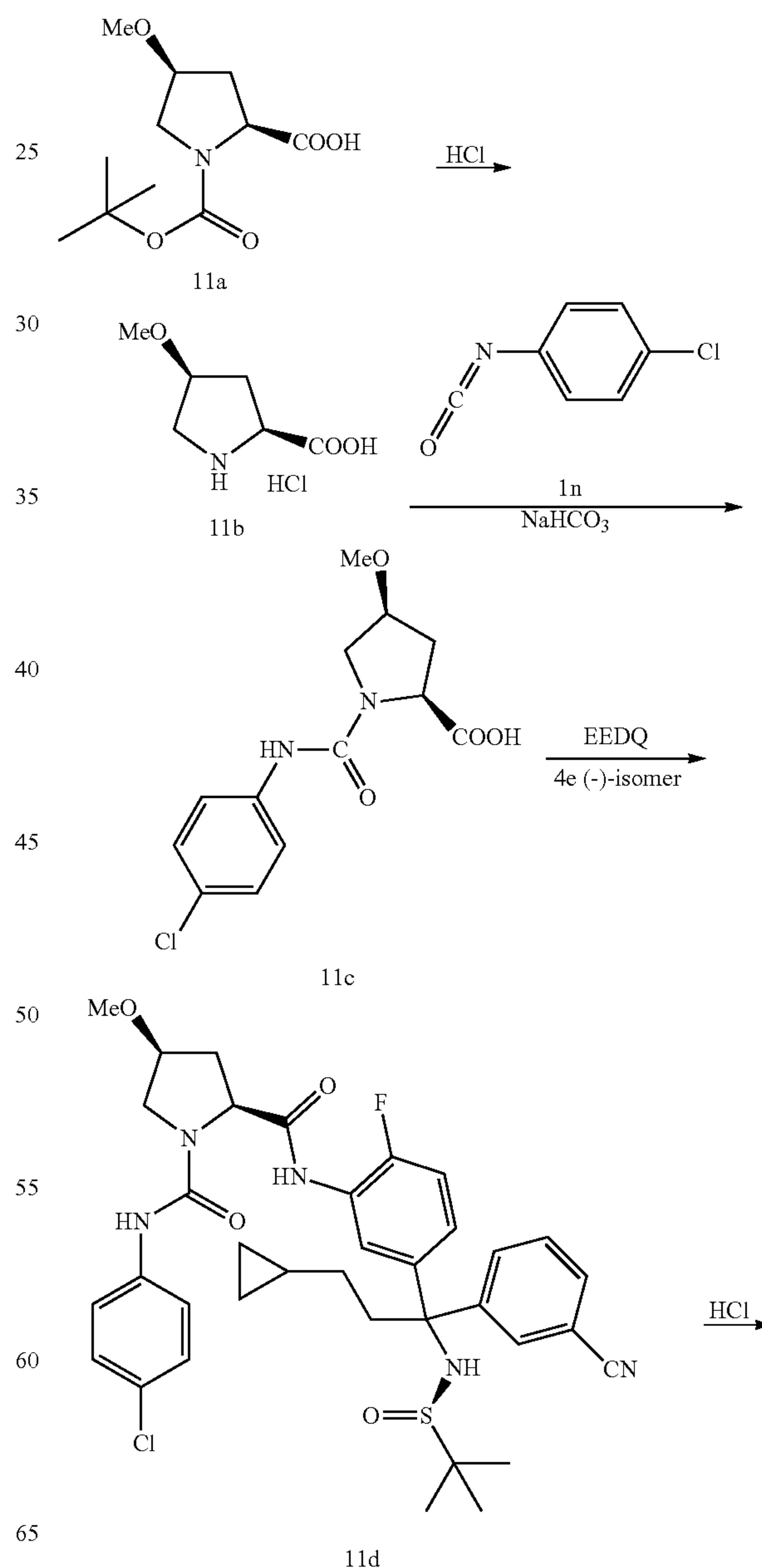
Scheme 11
