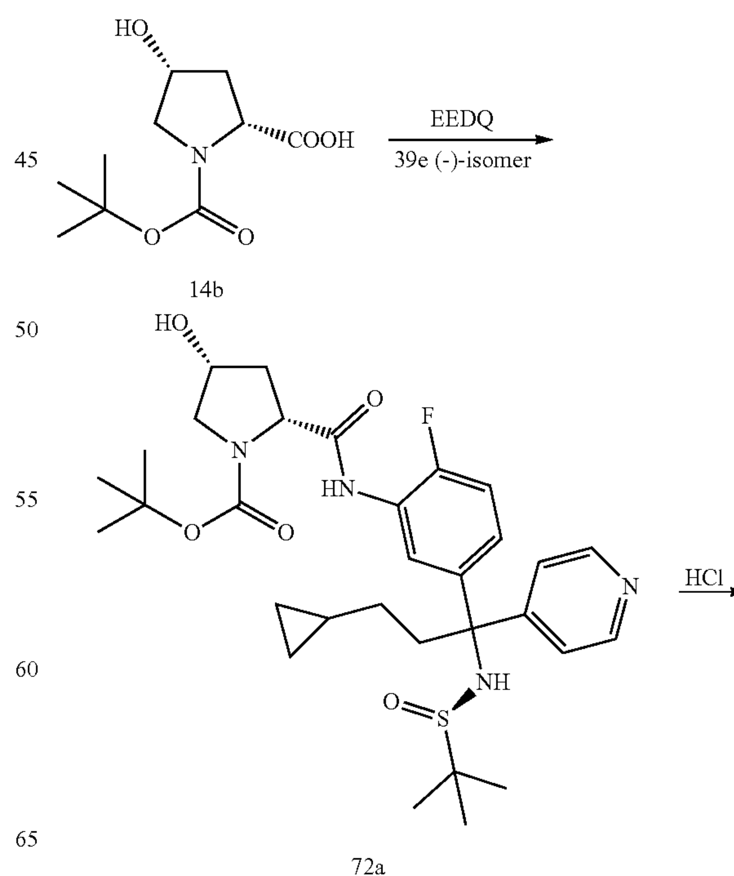
Scheme 72
