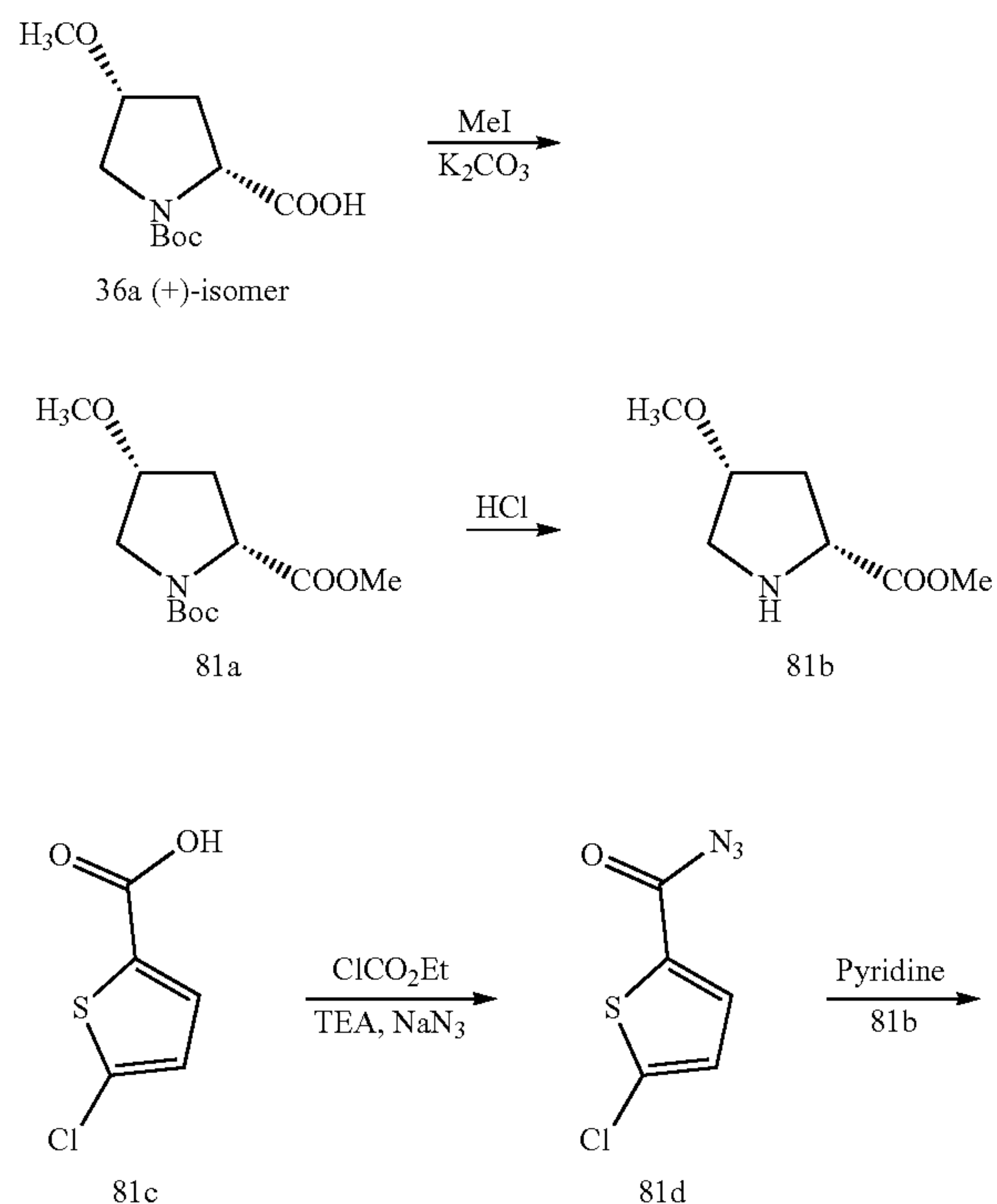
Scheme 81
