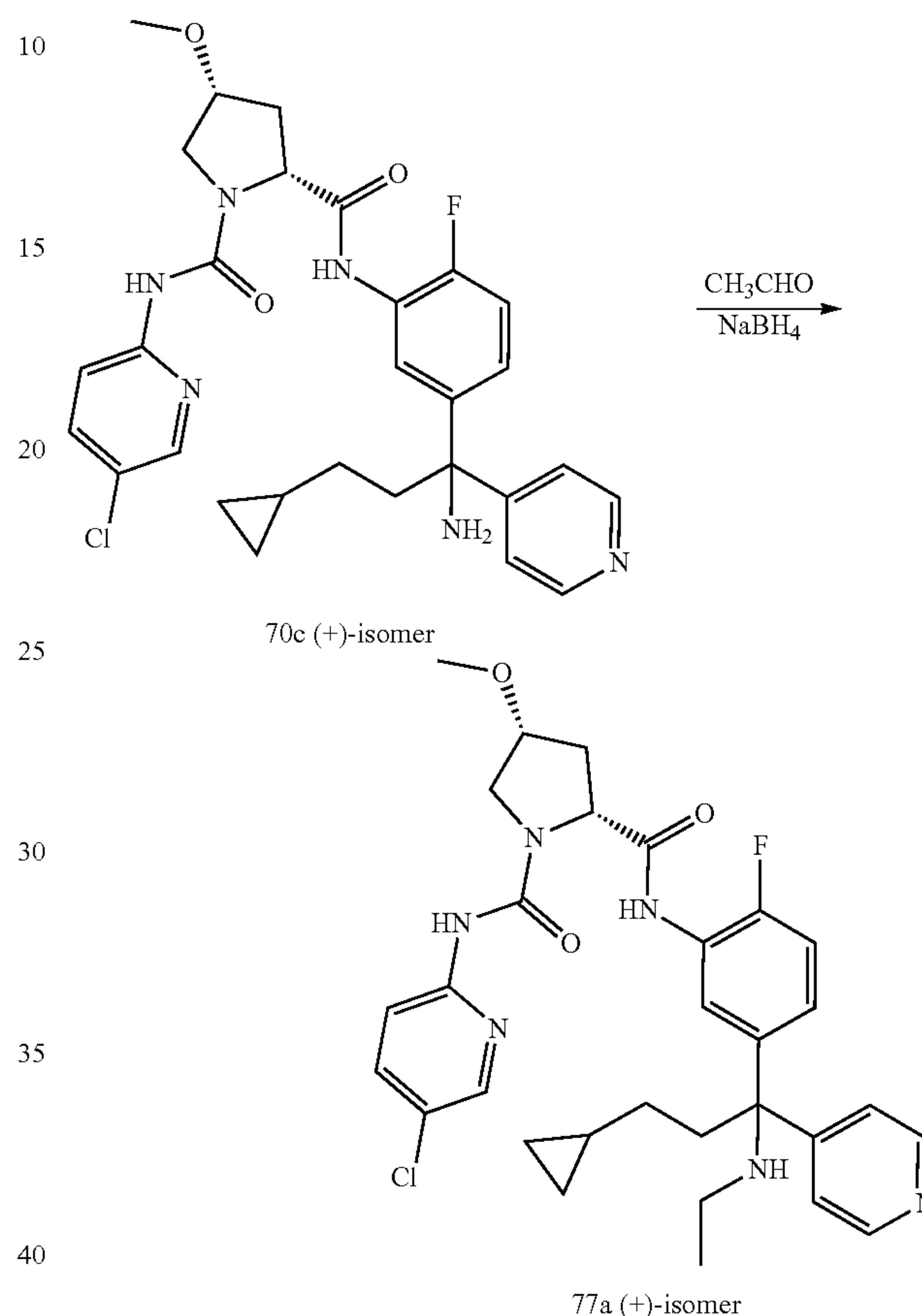
Scheme 77
