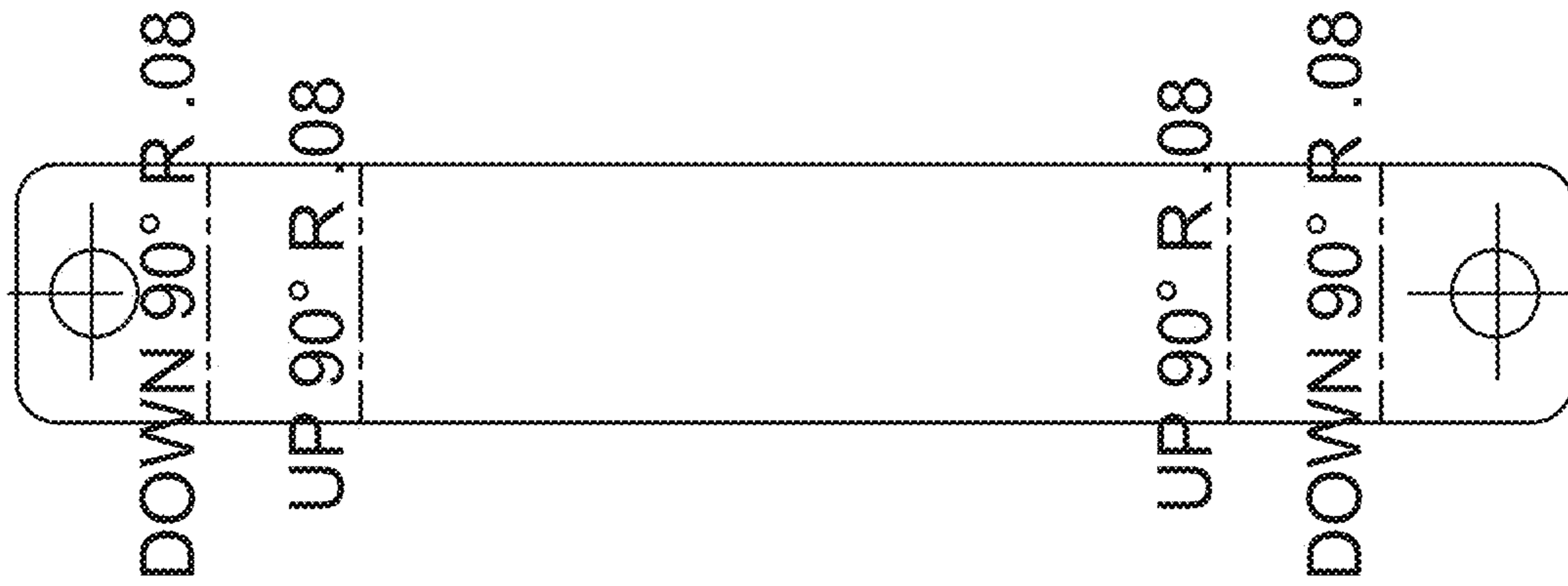
FLAT PATTERN
