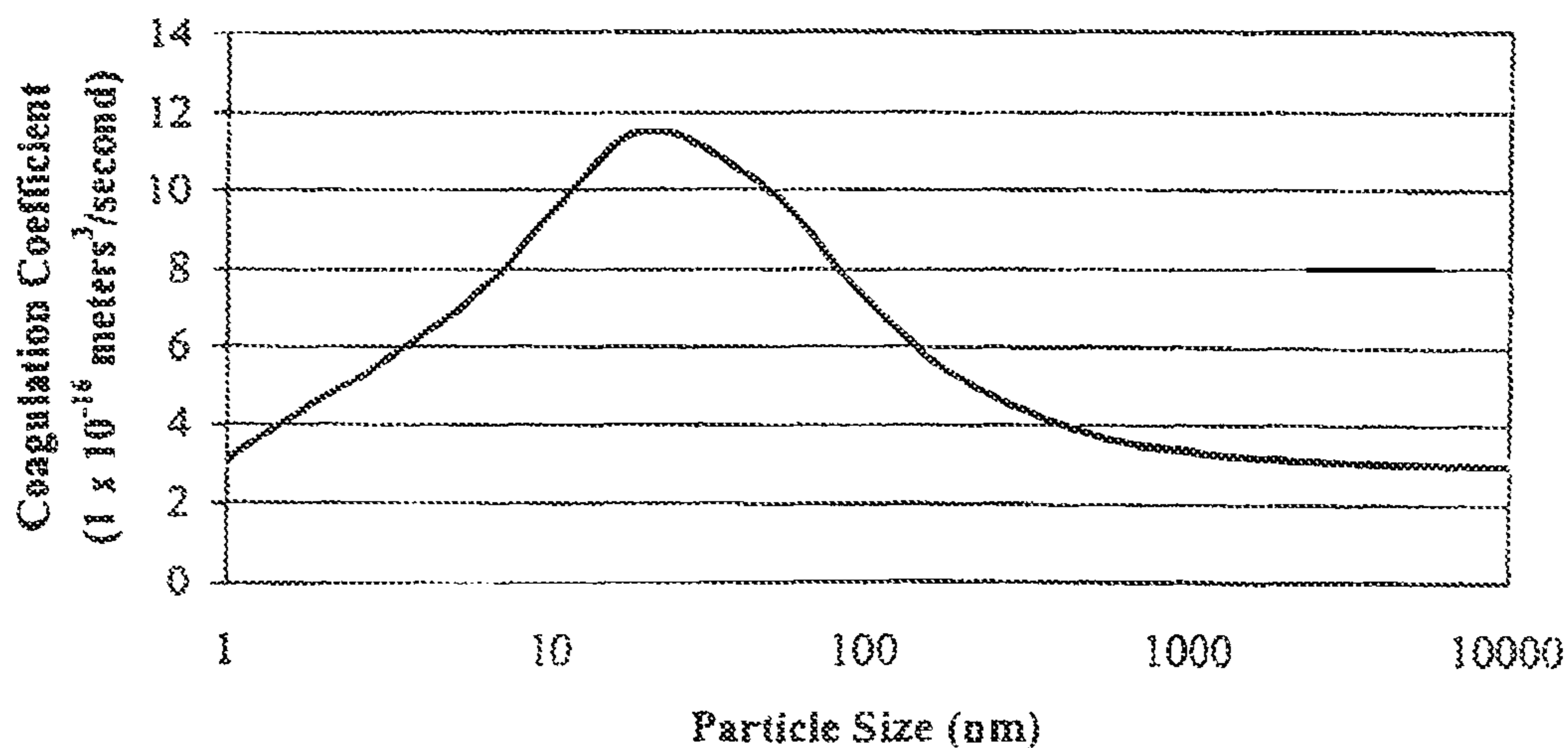
Coagulation Coefficient vs. Particle Size
