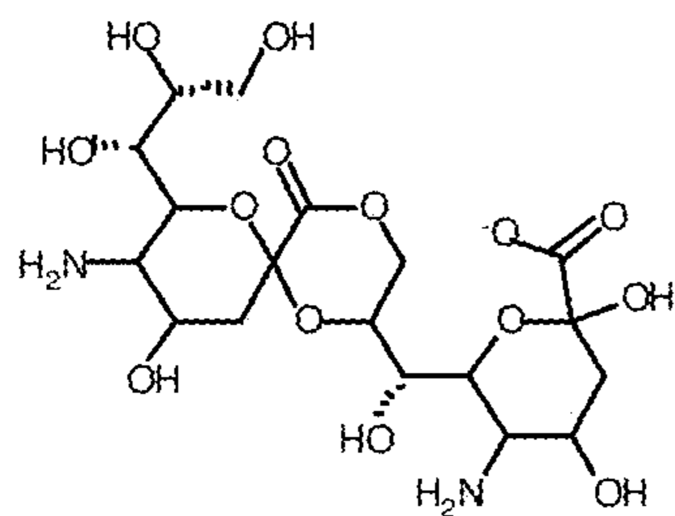
Structure VIII
