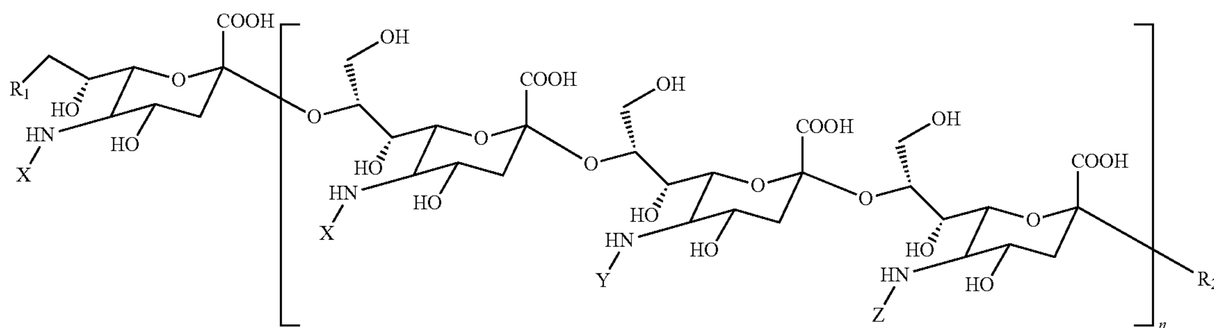
FORMULA IVb
