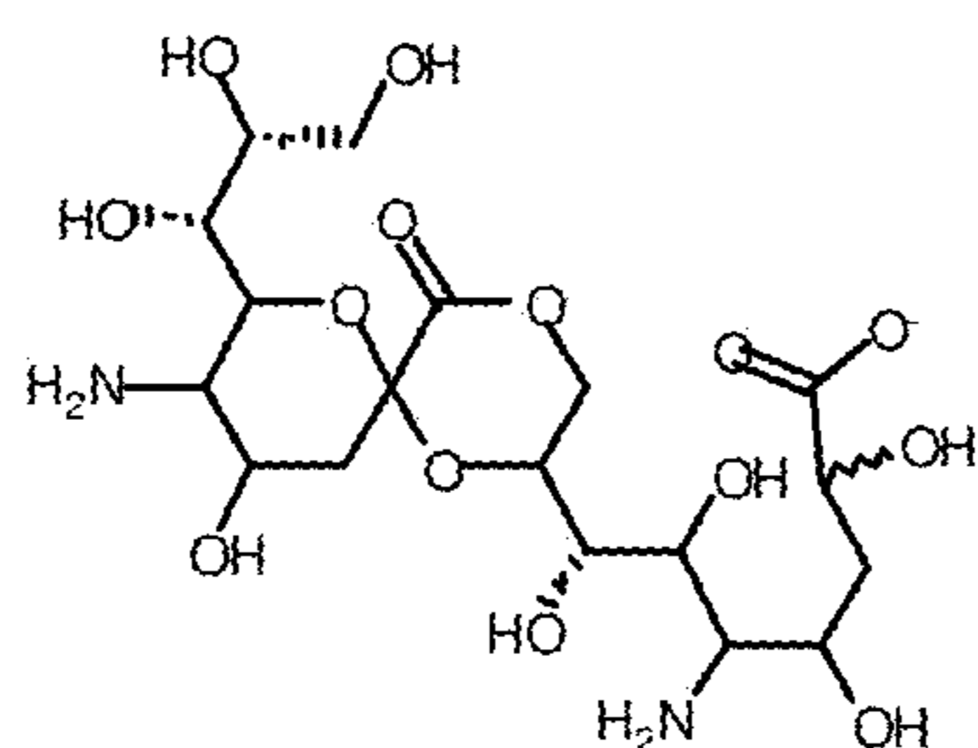
Structure VI
