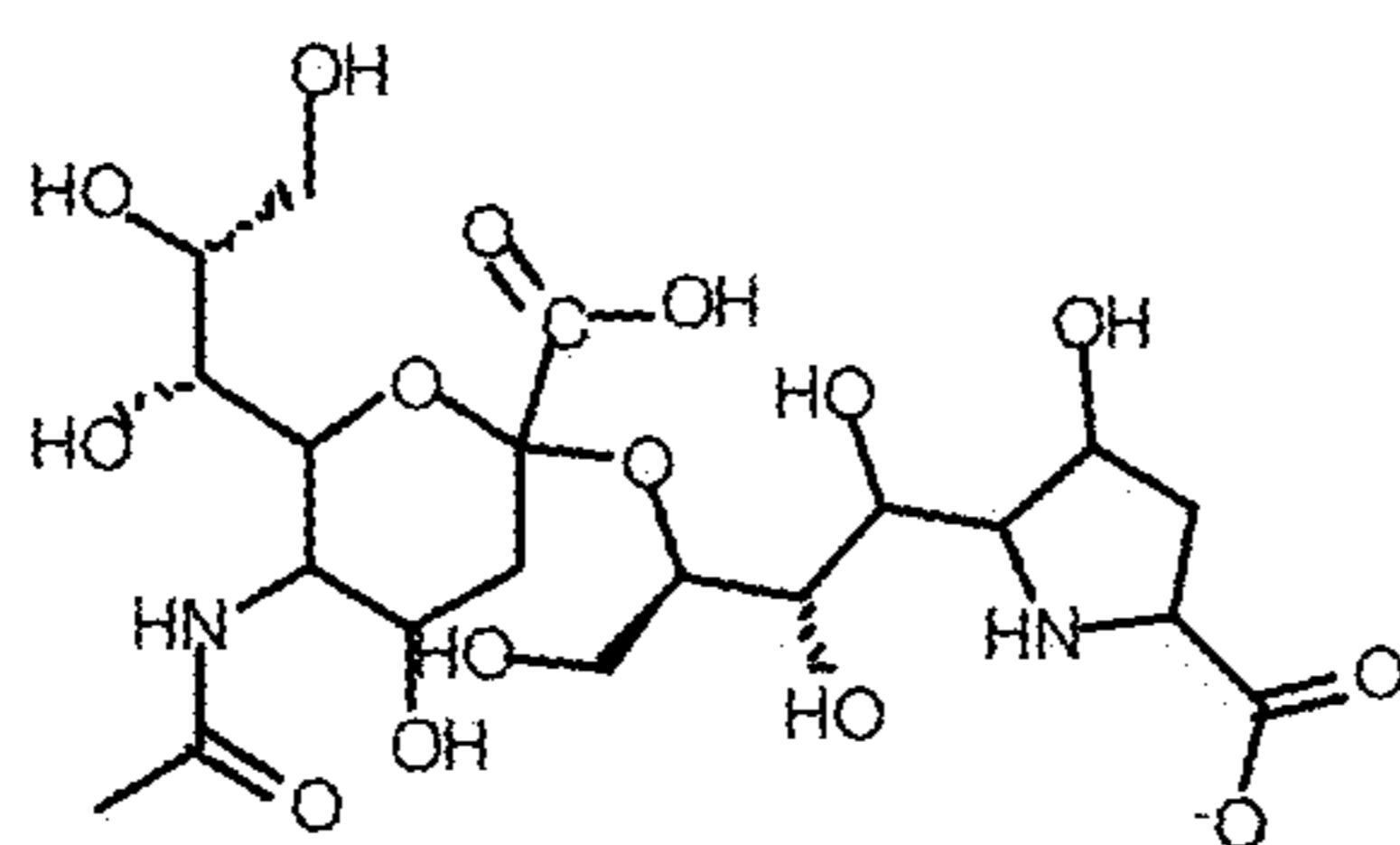
Structure IV
