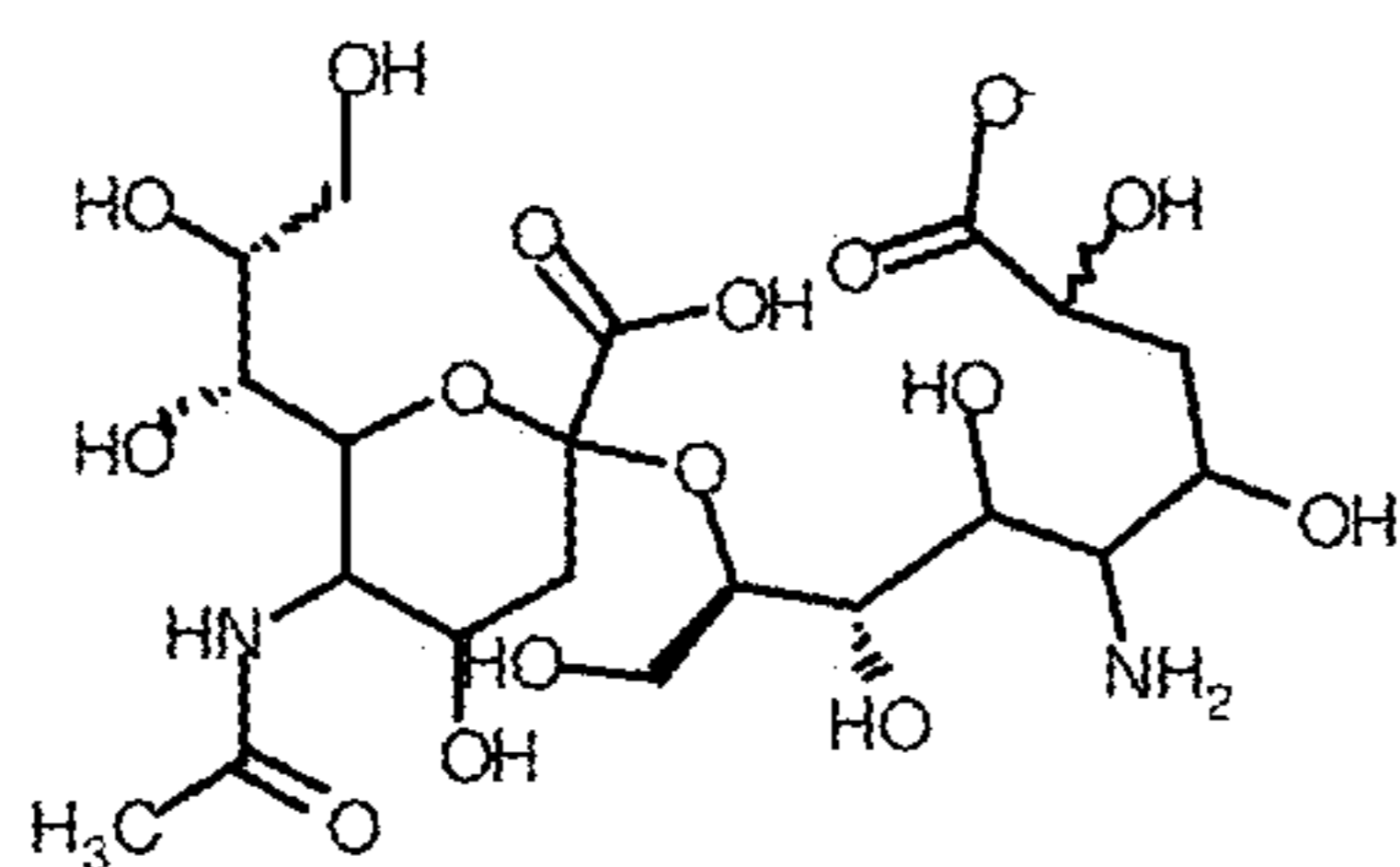
Structure I
