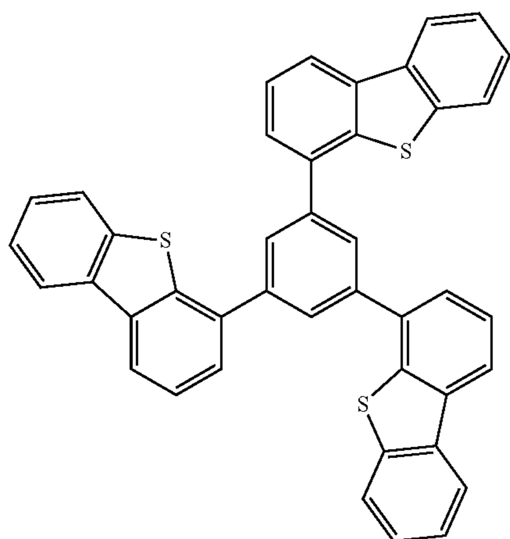
(i) DBT3P-II
