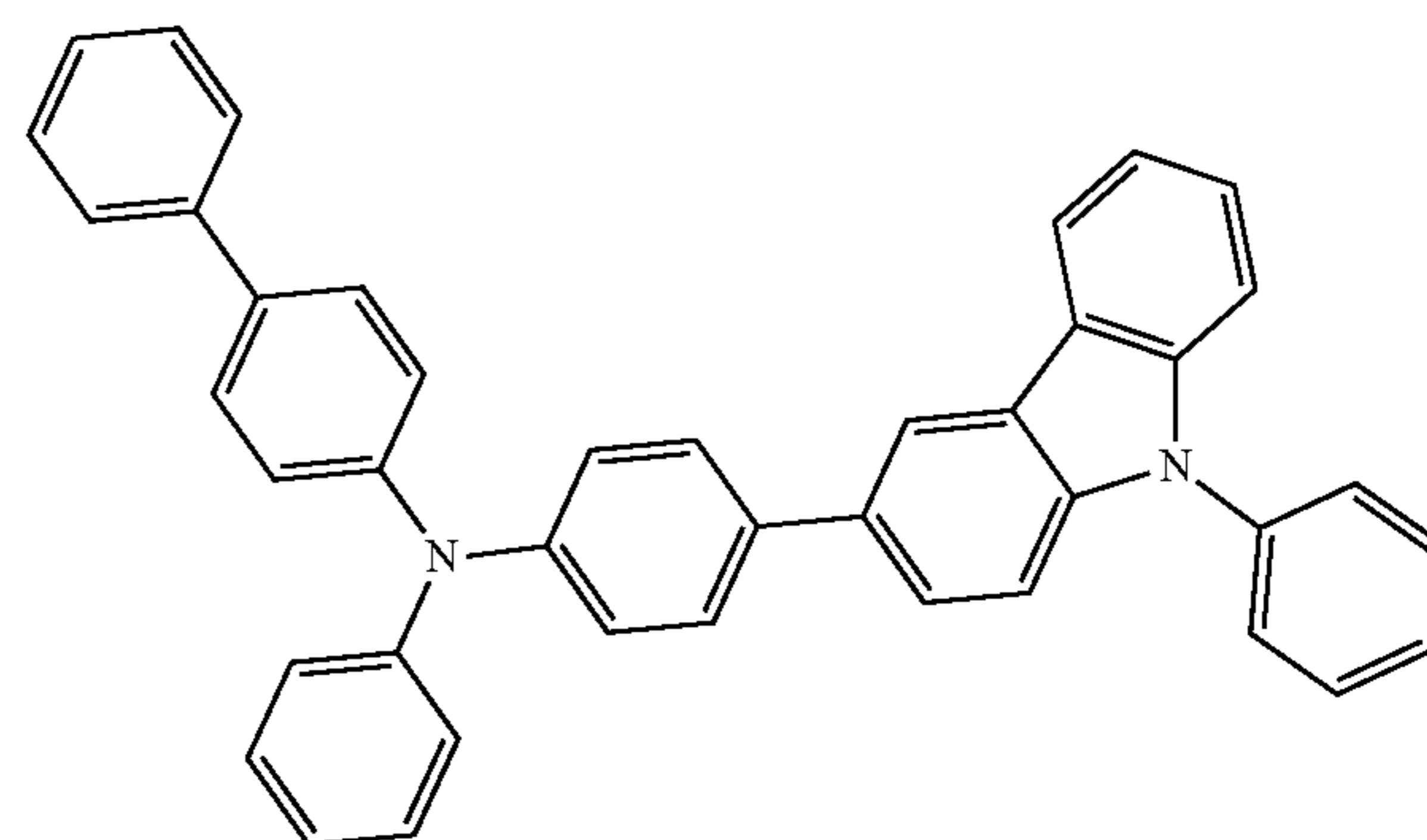
(iv) PCBA1BP
