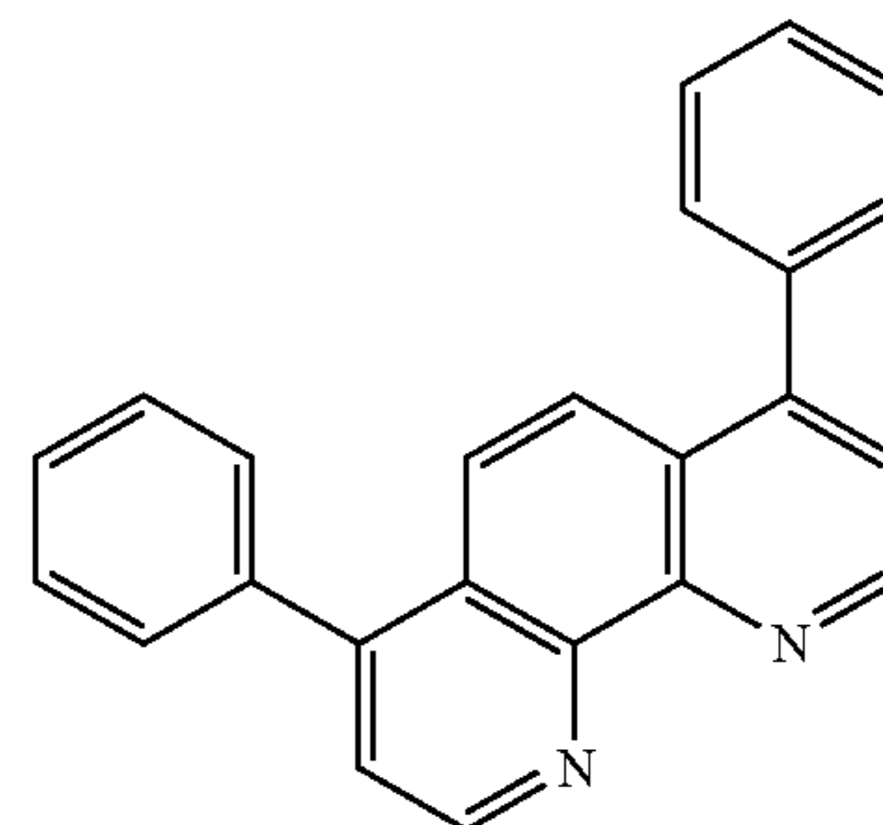
(xi) Bphen
