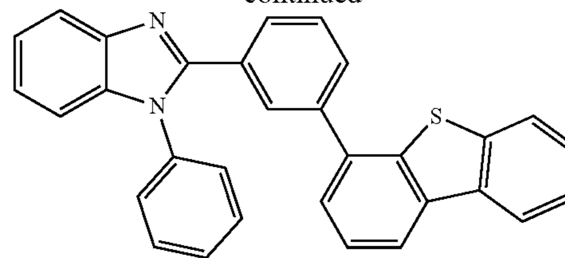
(x) mDBTBIIm-II
