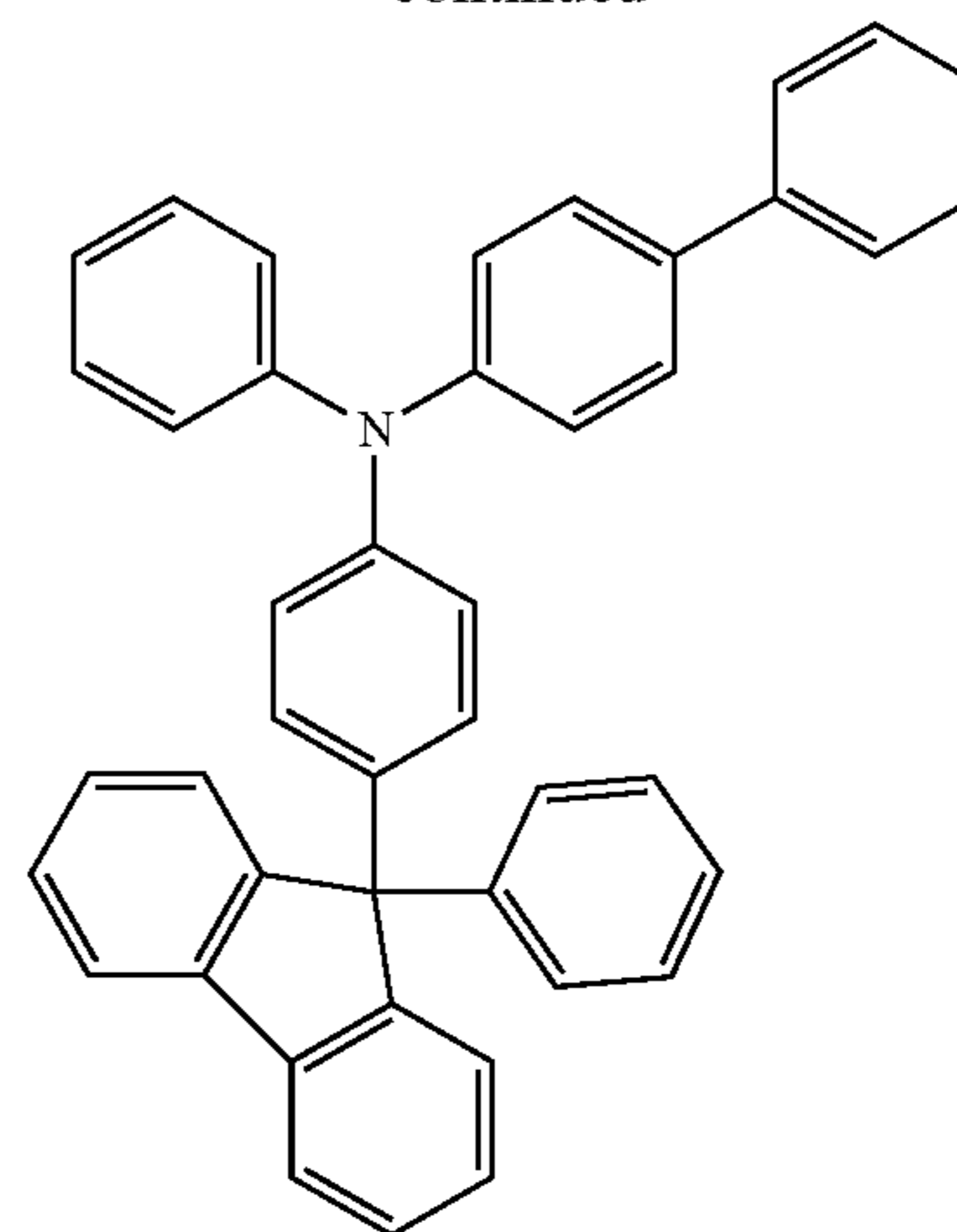
(ii) BPAFLP
