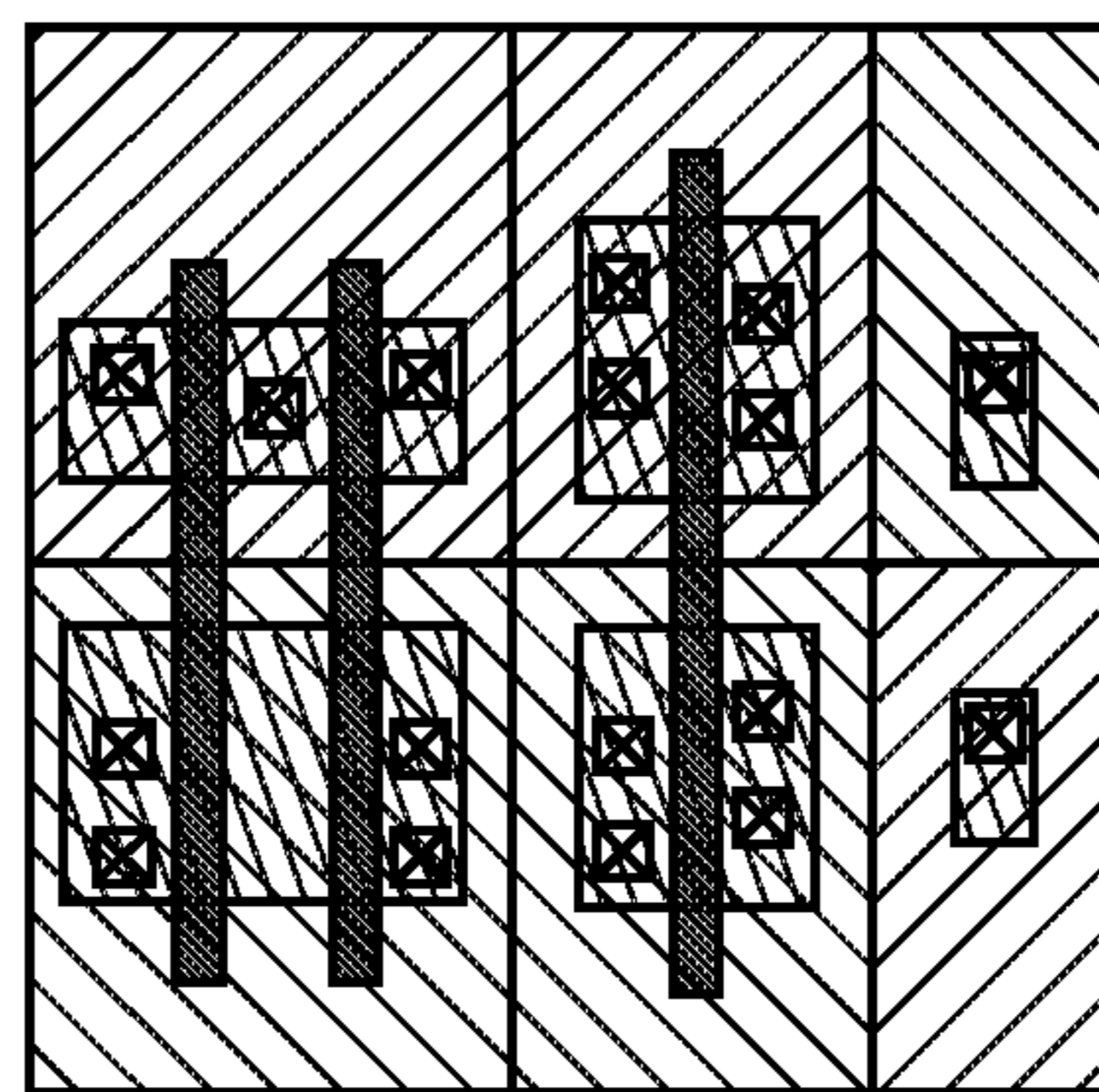
1.26 NAND2:INV:TAP
