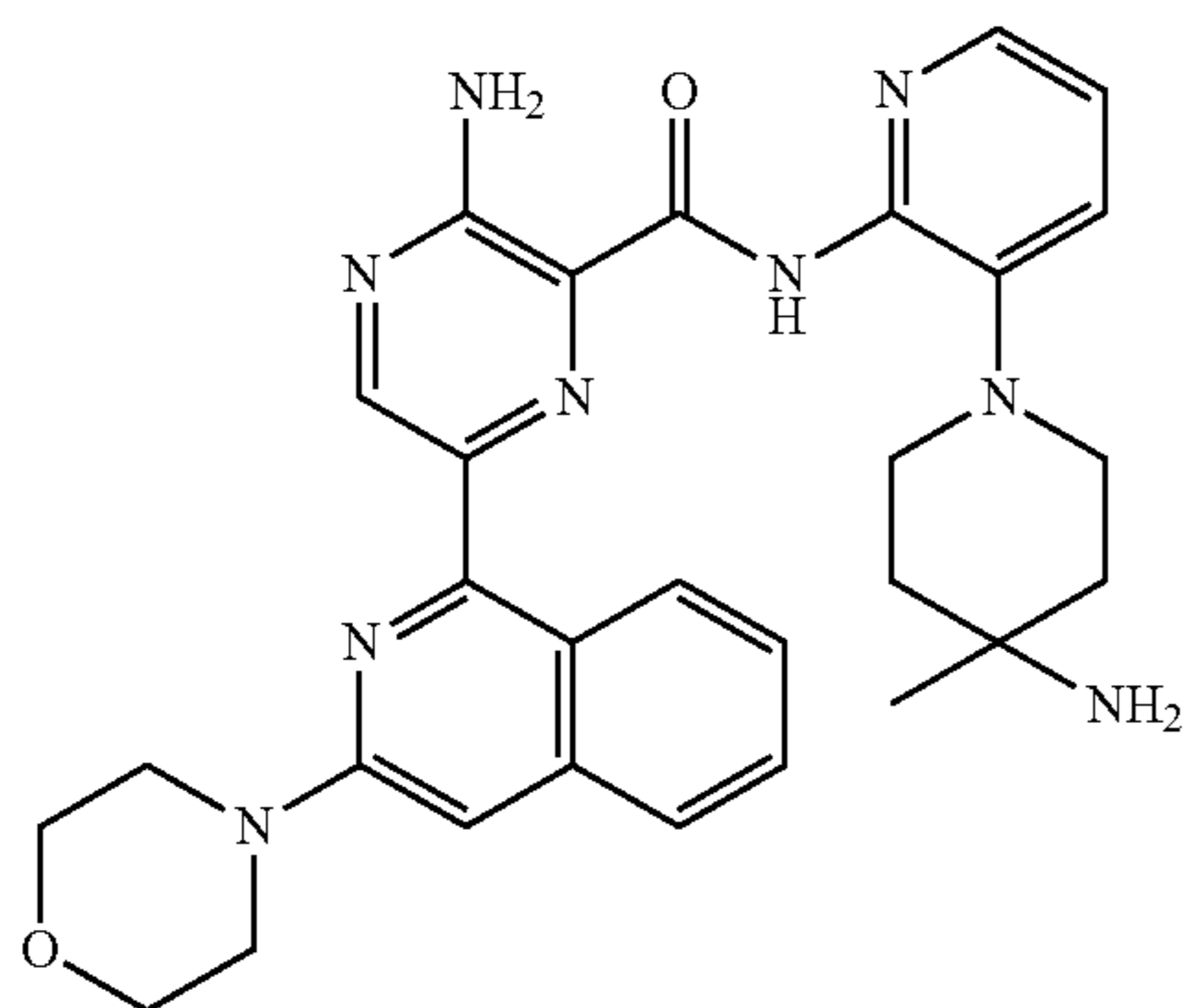
Synthesis of 3-amino-6-(3-morpholinoquinolin-1-yl)pyrazine-2-carboxylic acid
