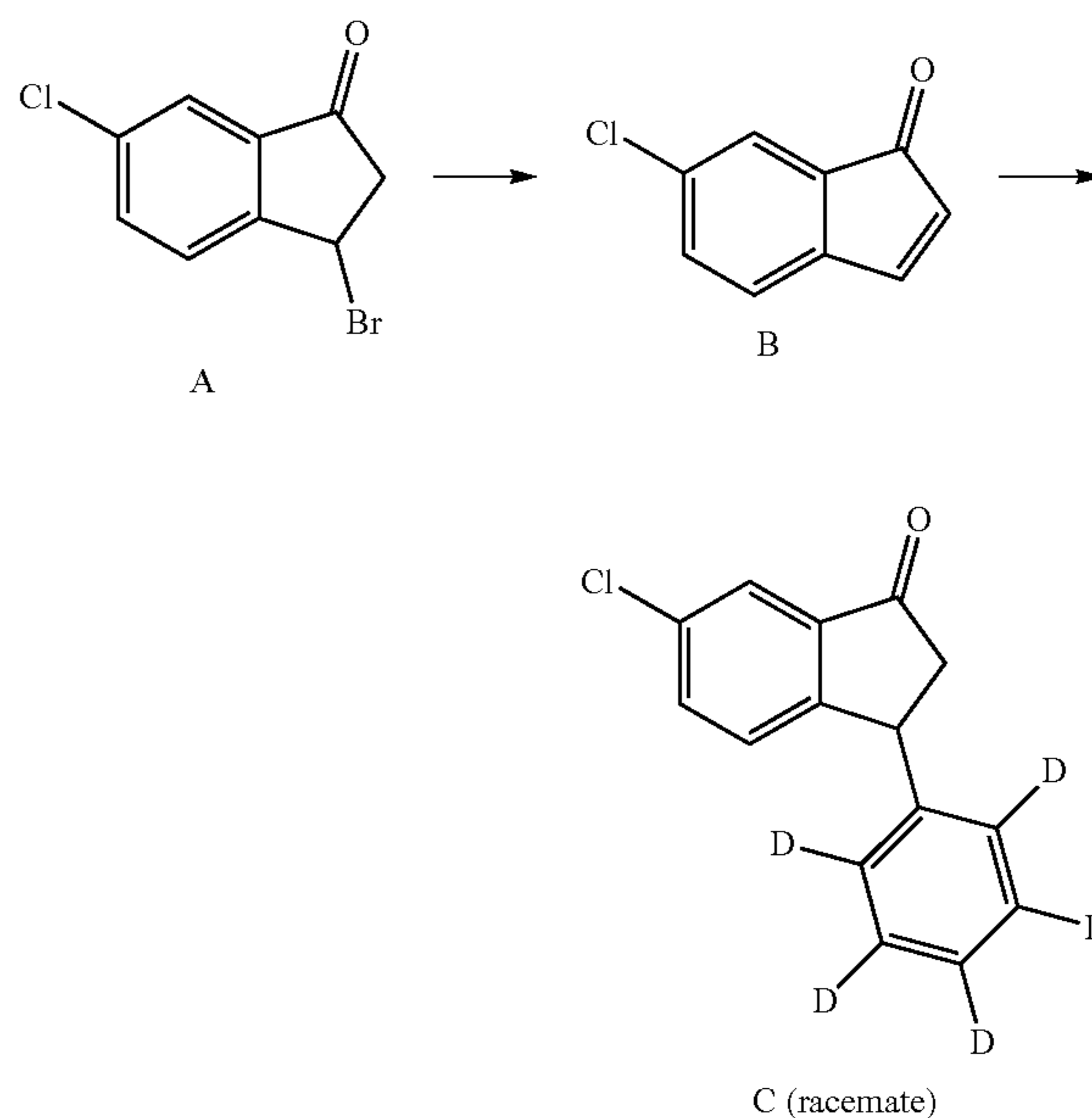
Scheme 1. Exemplary synthesis of intermediate C.
