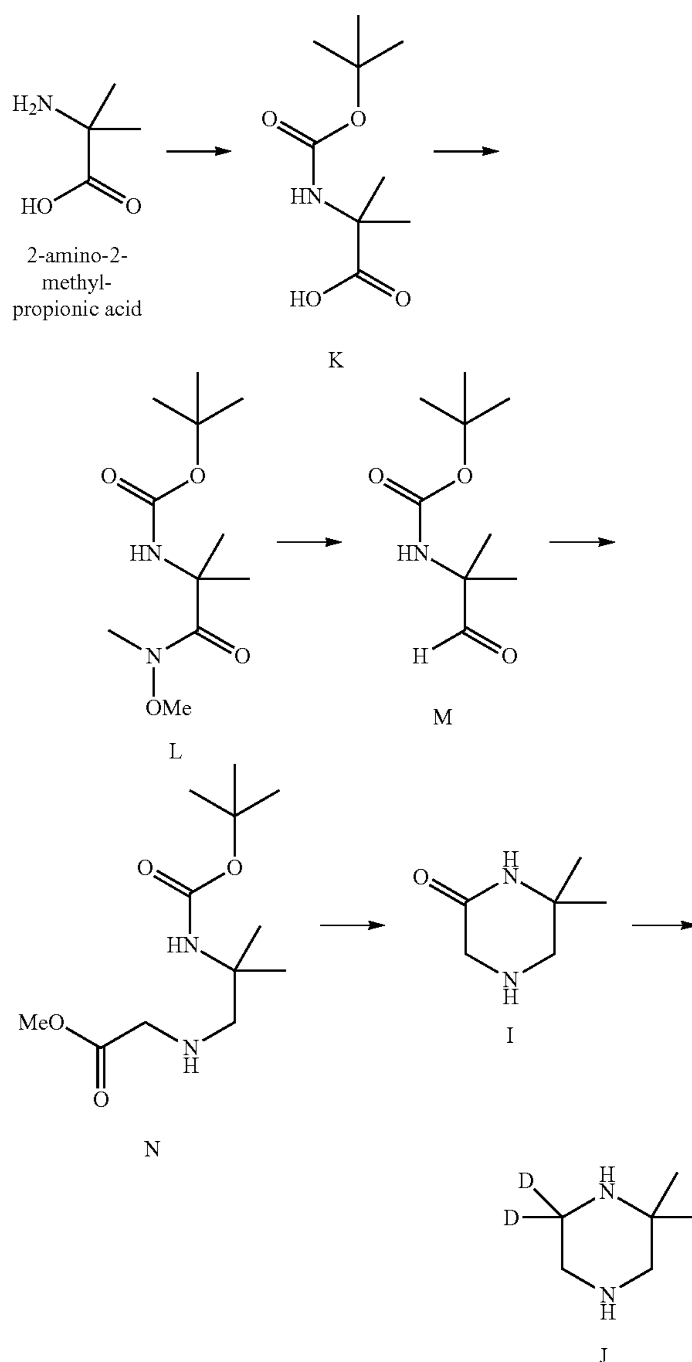
Scheme 11. Synthesis of intermediate J.
