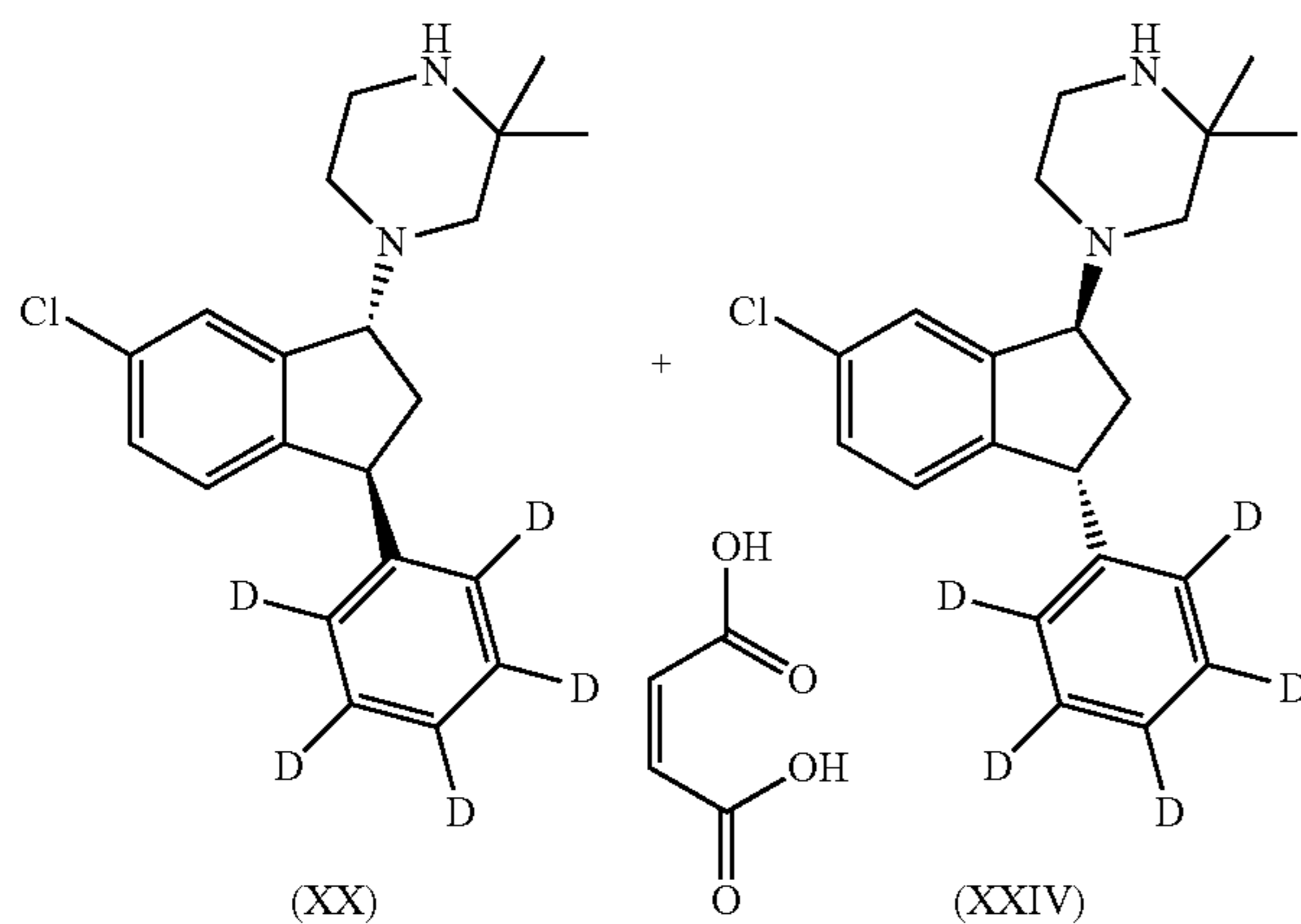
(XXV) maleate Mw 462.00 (345.93 + 116.07) trans racemate (+8% cis)
