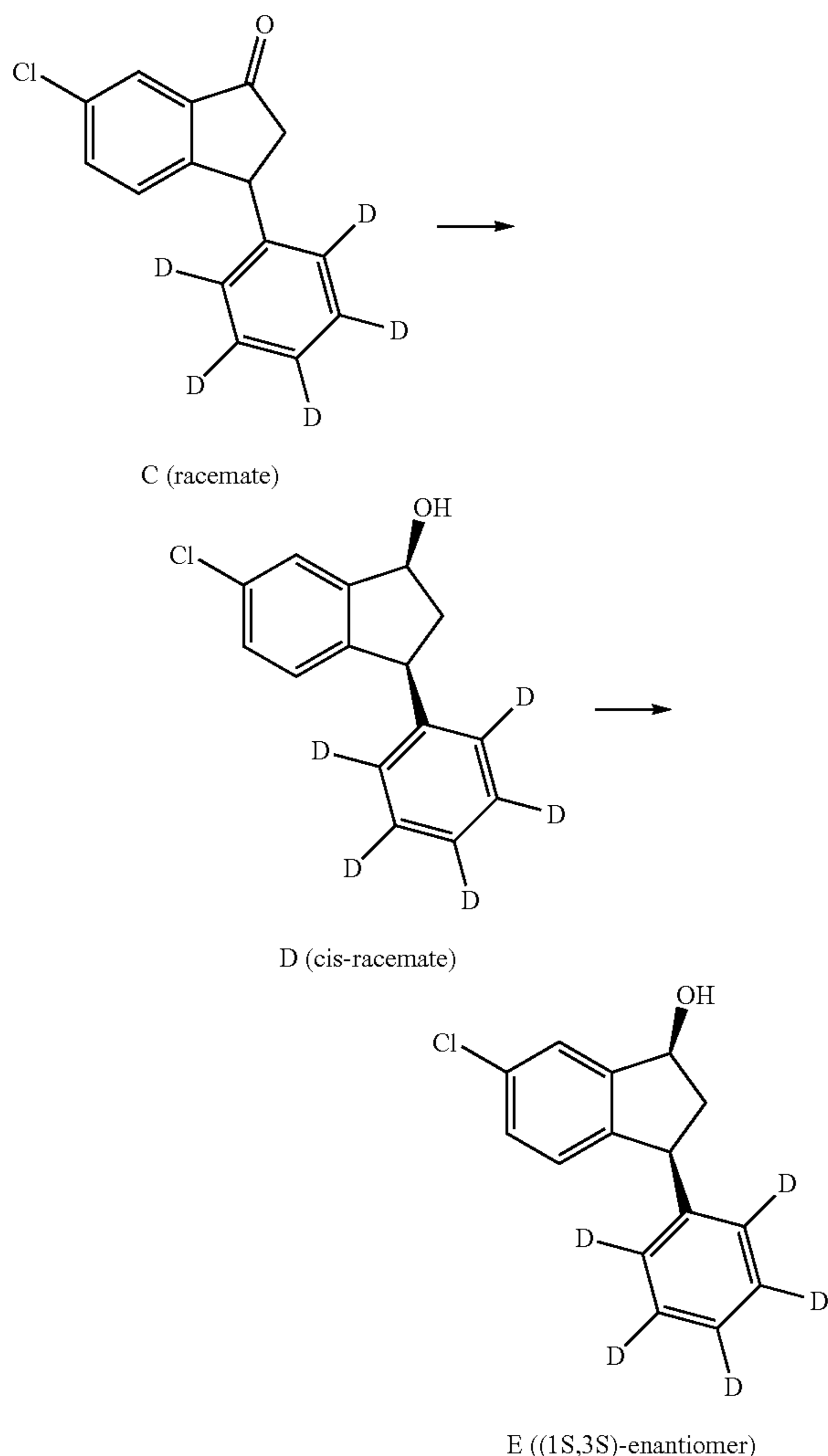
Scheme 2. Exemplary synthesis of intermediate E.
