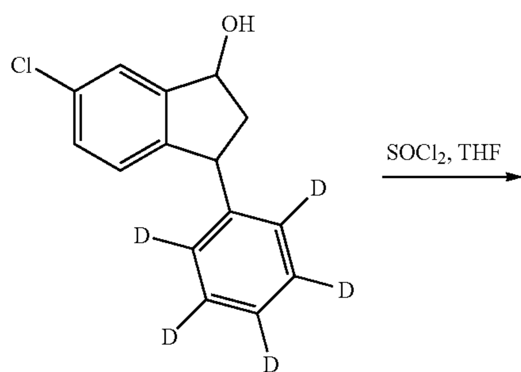
(XXII) cis racemate Mw 249.75 C_{15}H_8ClOD_5
