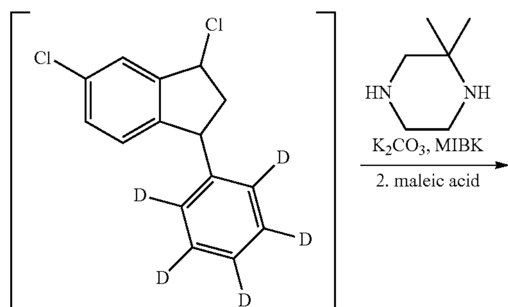
(XXIII) cis racemate (+15% trans) Mw 268.20 C_{15}H_7Cl_2D_5
