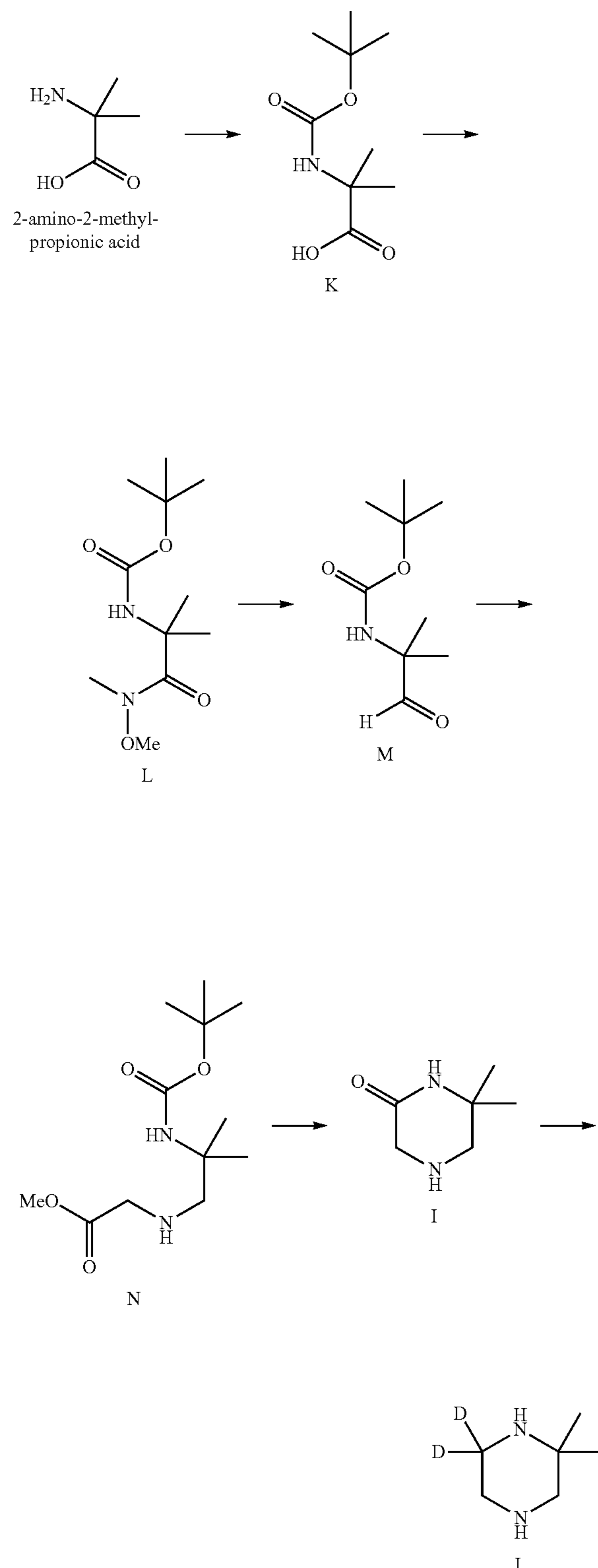
Scheme 7. Alternative exemplary synthesis of intermediate J.
