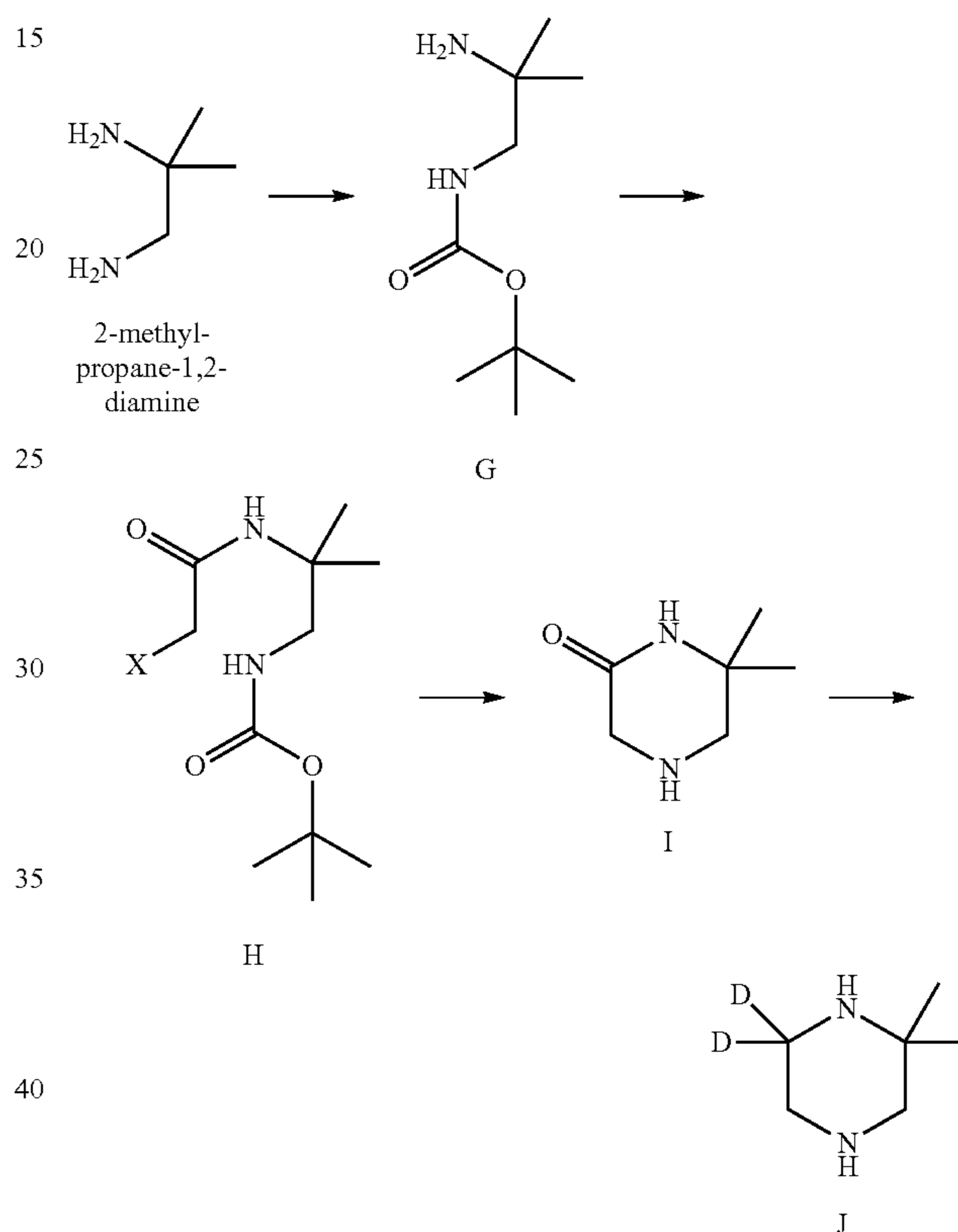
Scheme 6. Exemplary synthesis of intermediate J.
