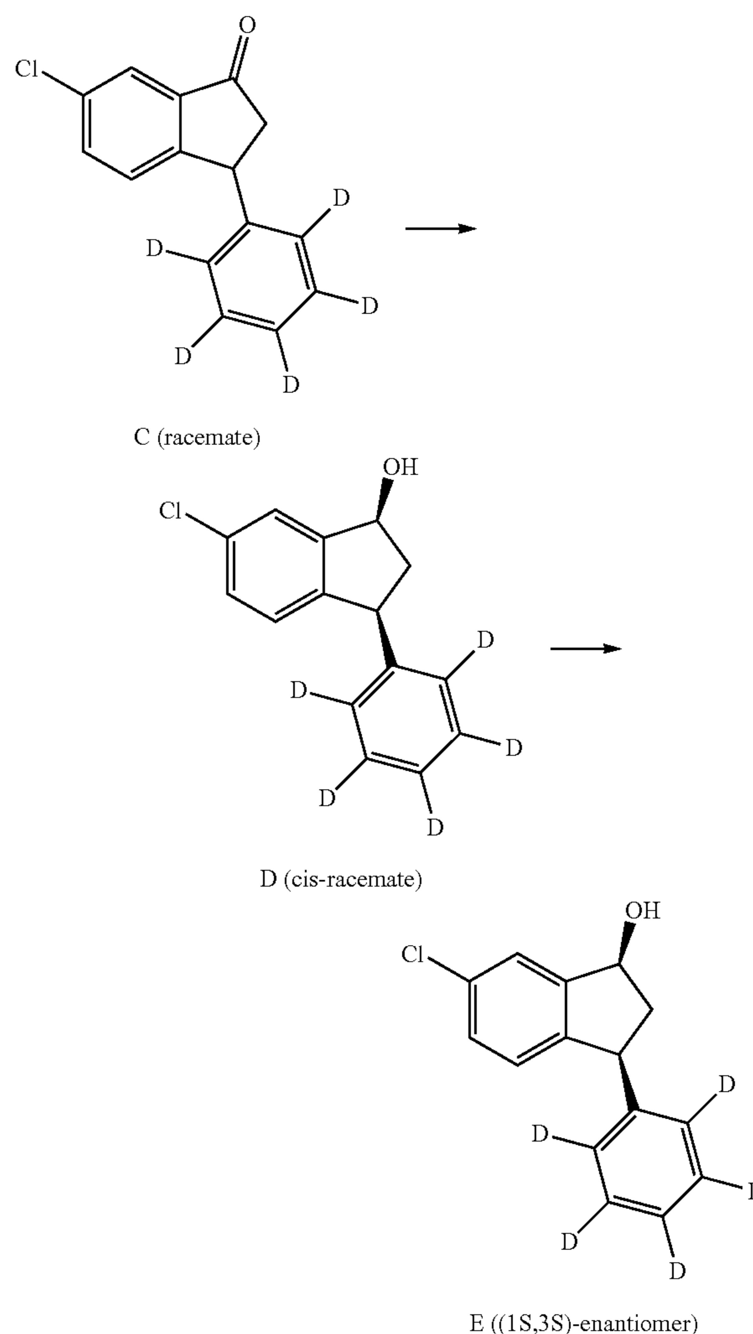
Scheme 10. Synthesis and resolution of Compound E.
