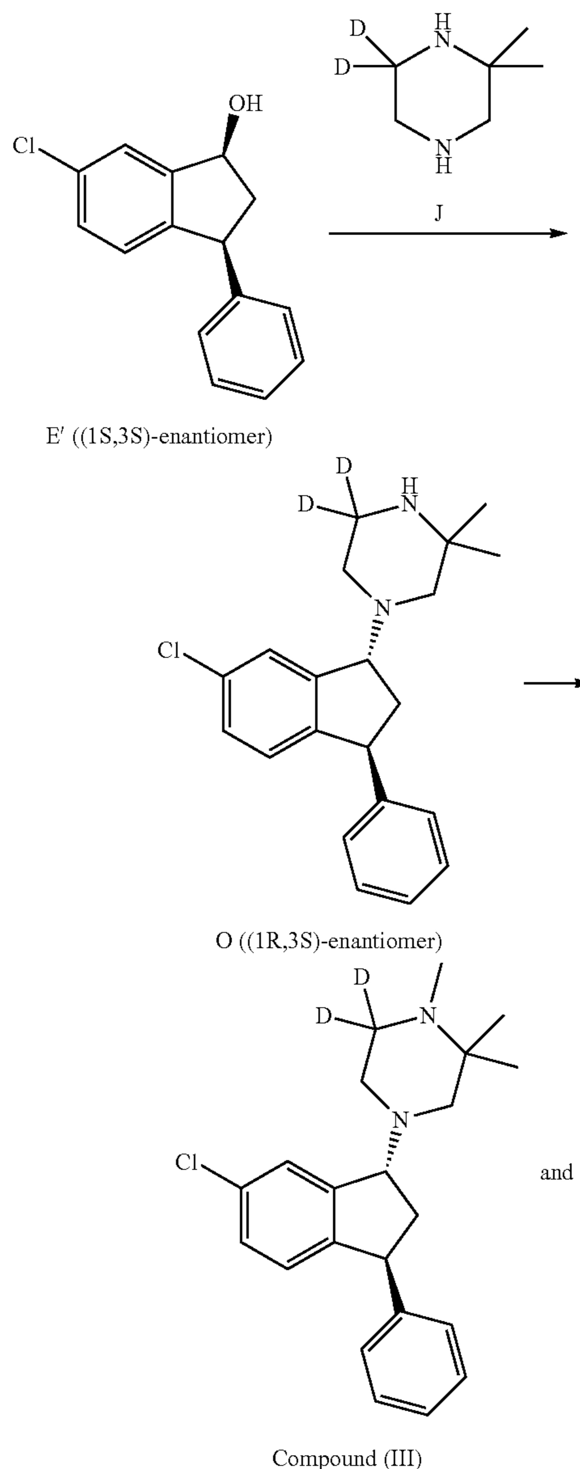
Scheme 12. Synthesis of Compound (III) and Compound (V).
