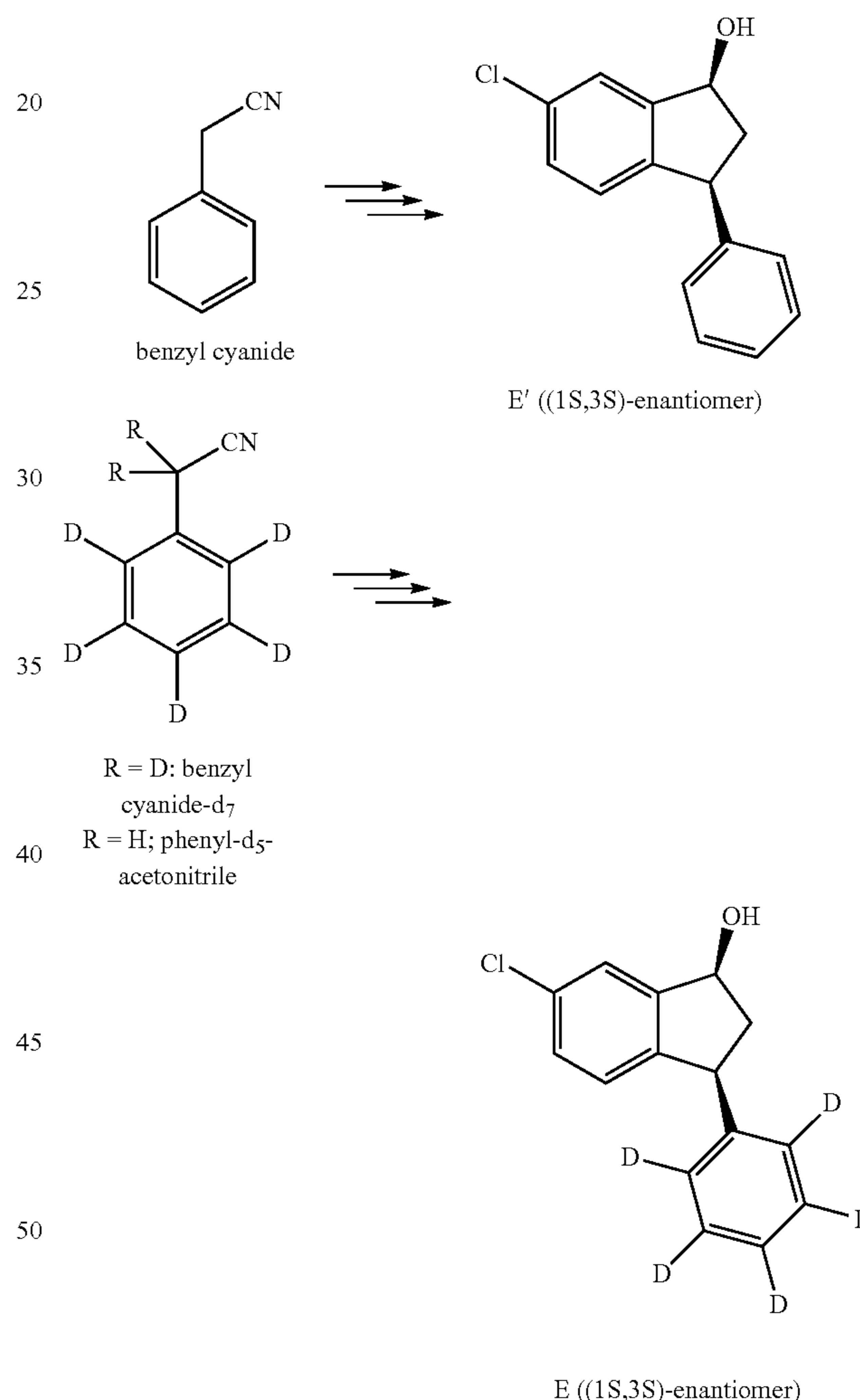
Scheme 4. Exemplary synthesis of intermediates E and E'.
