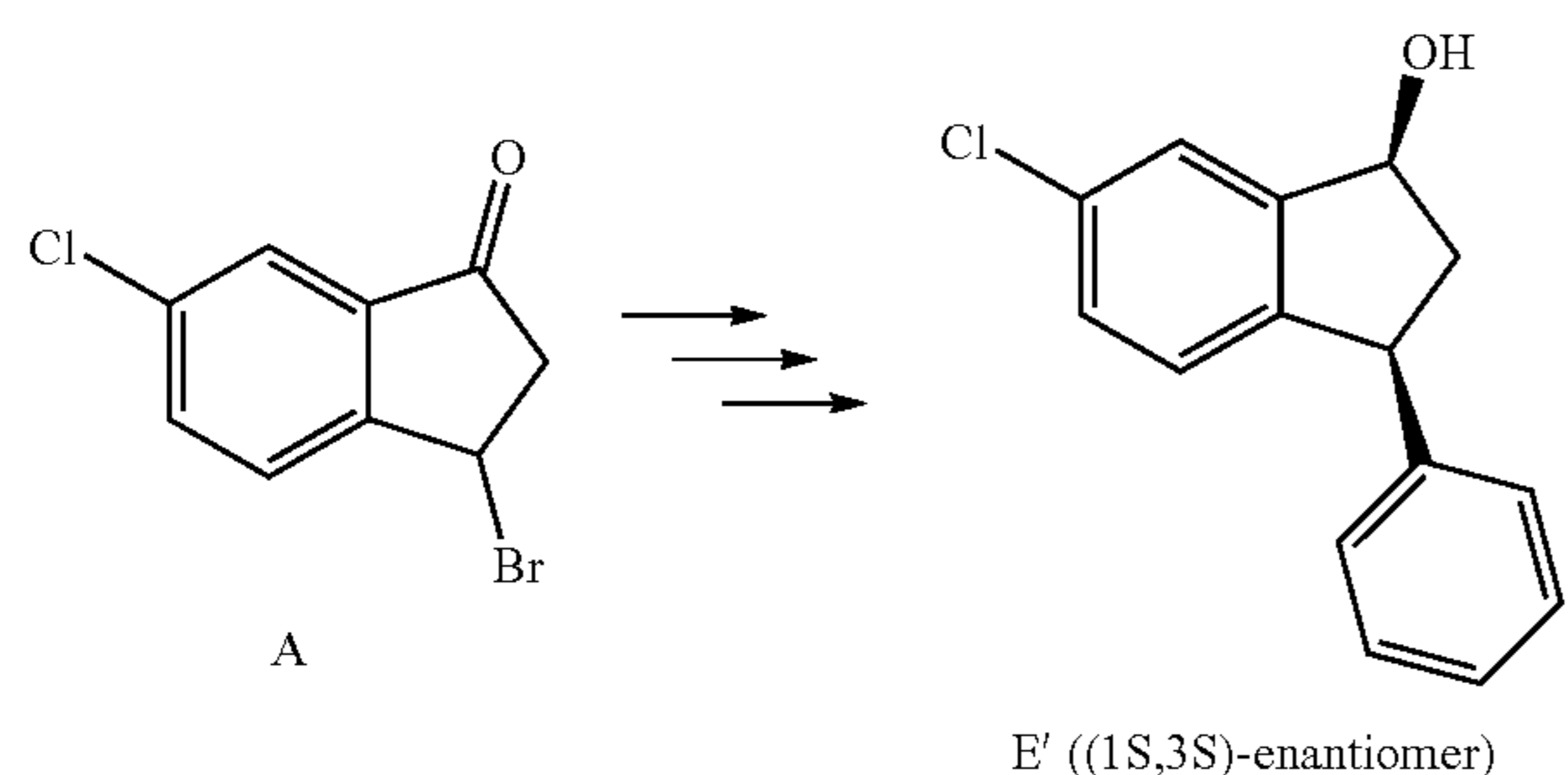
Scheme 3. Exemplary synthesis of intermediate E'.
