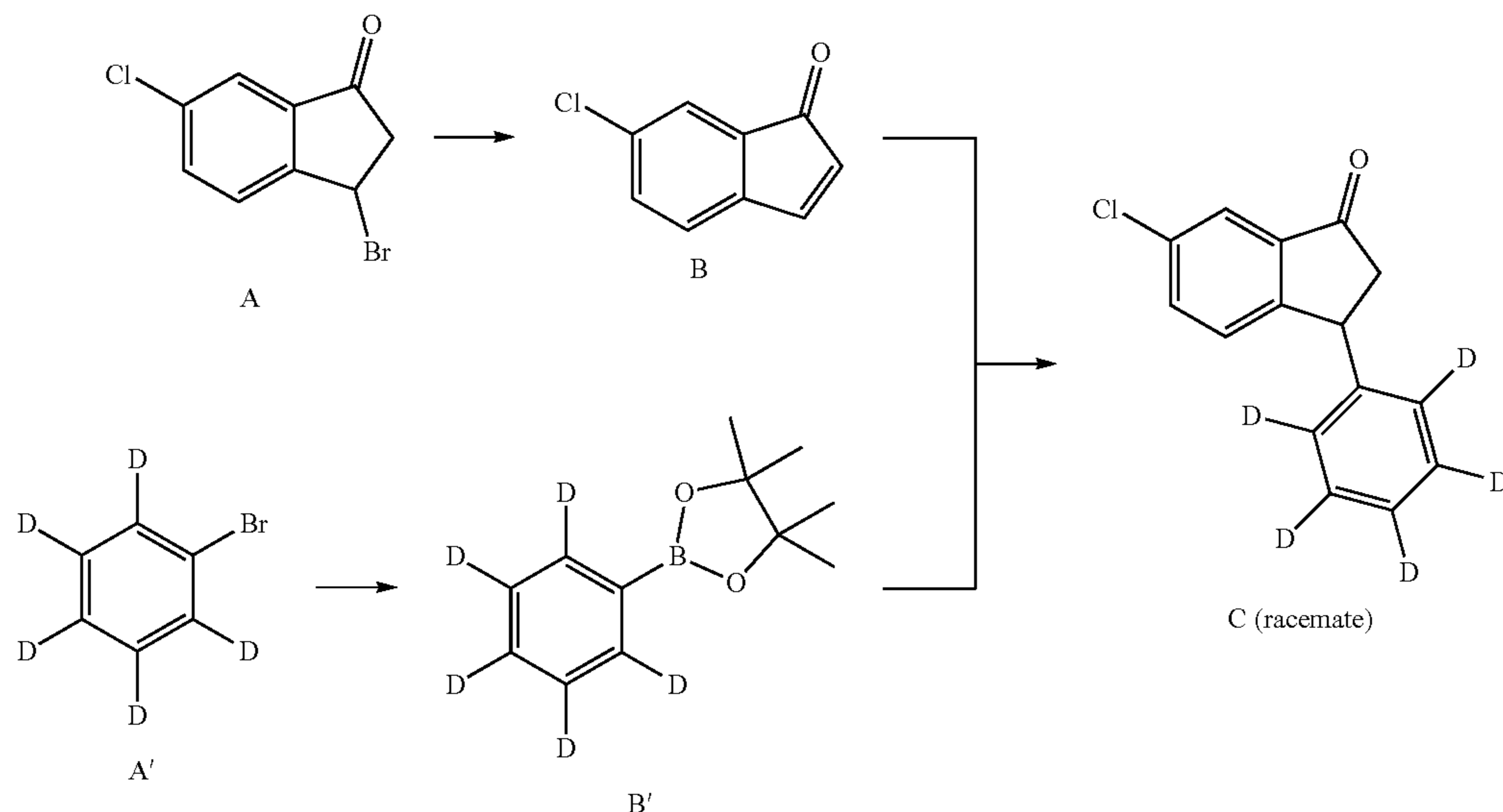
Scheme 9. Synthesis of Compound C.
