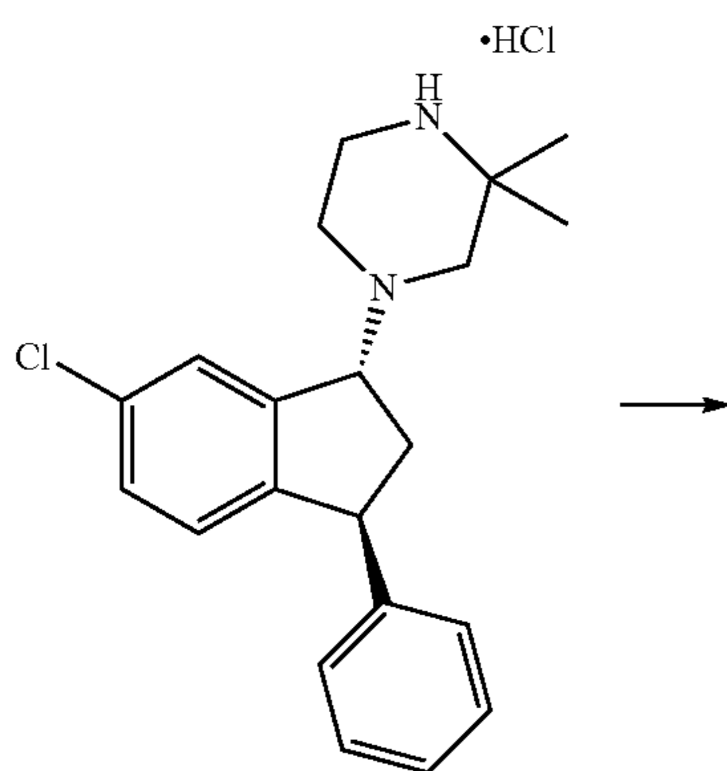
1-((1R,3S)-6-Chloro-3-phenyl-indan-1-yl)-3,3-dimethyl-piperazine hydrochloride (Compound (XI) hydrochloride)
