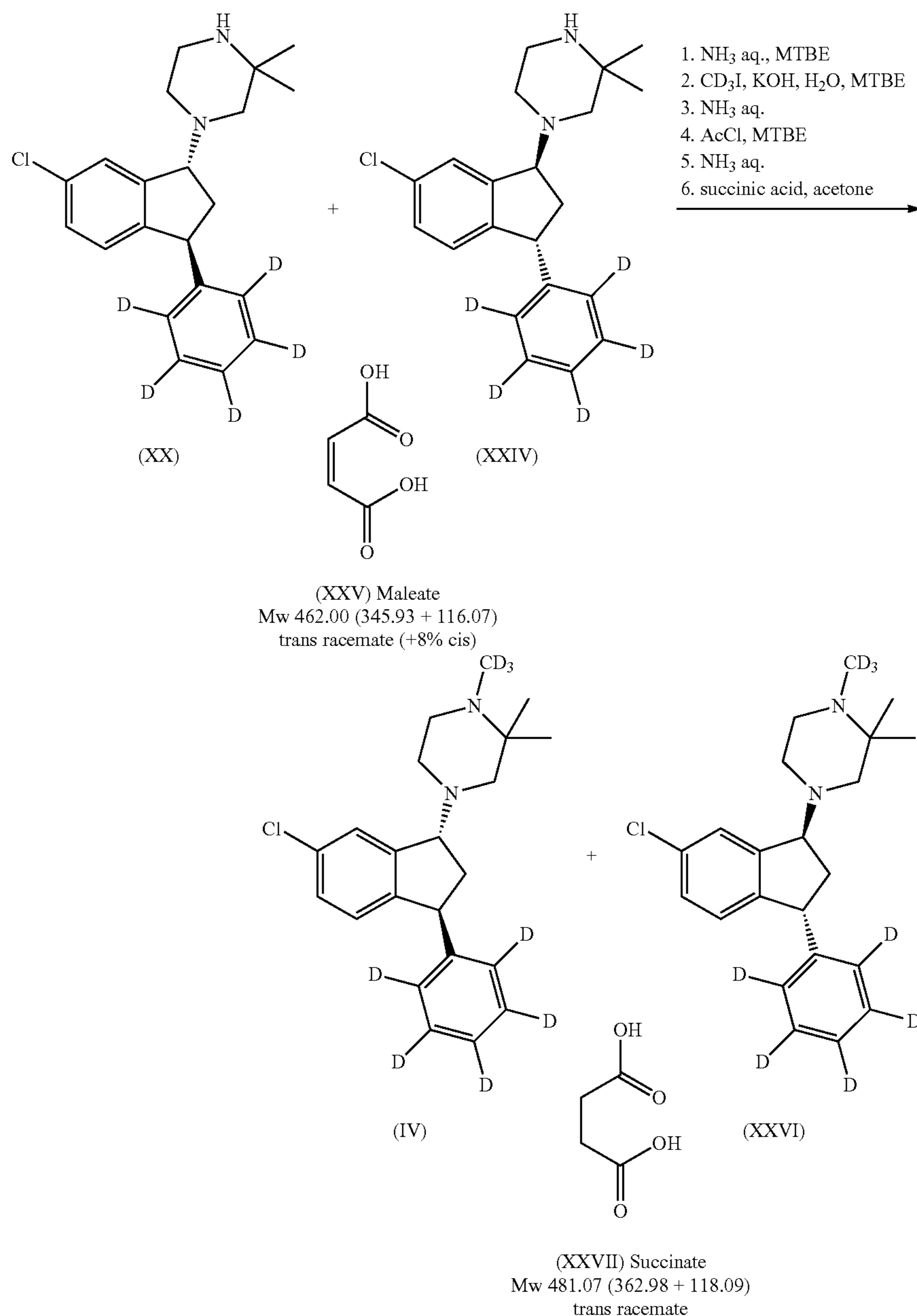
Scheme 17: Synthesis of rac-trans-1-(6-chloro-3-phenyl(d 5 )-indan-1-yl)-1-(d 3 ), 2,2-trimethyl-piperazine succinate.
