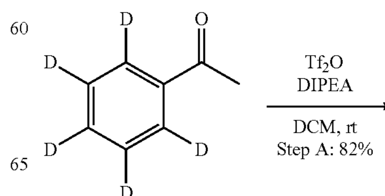
Scheme 14. Synthesis of Compound (XV)
