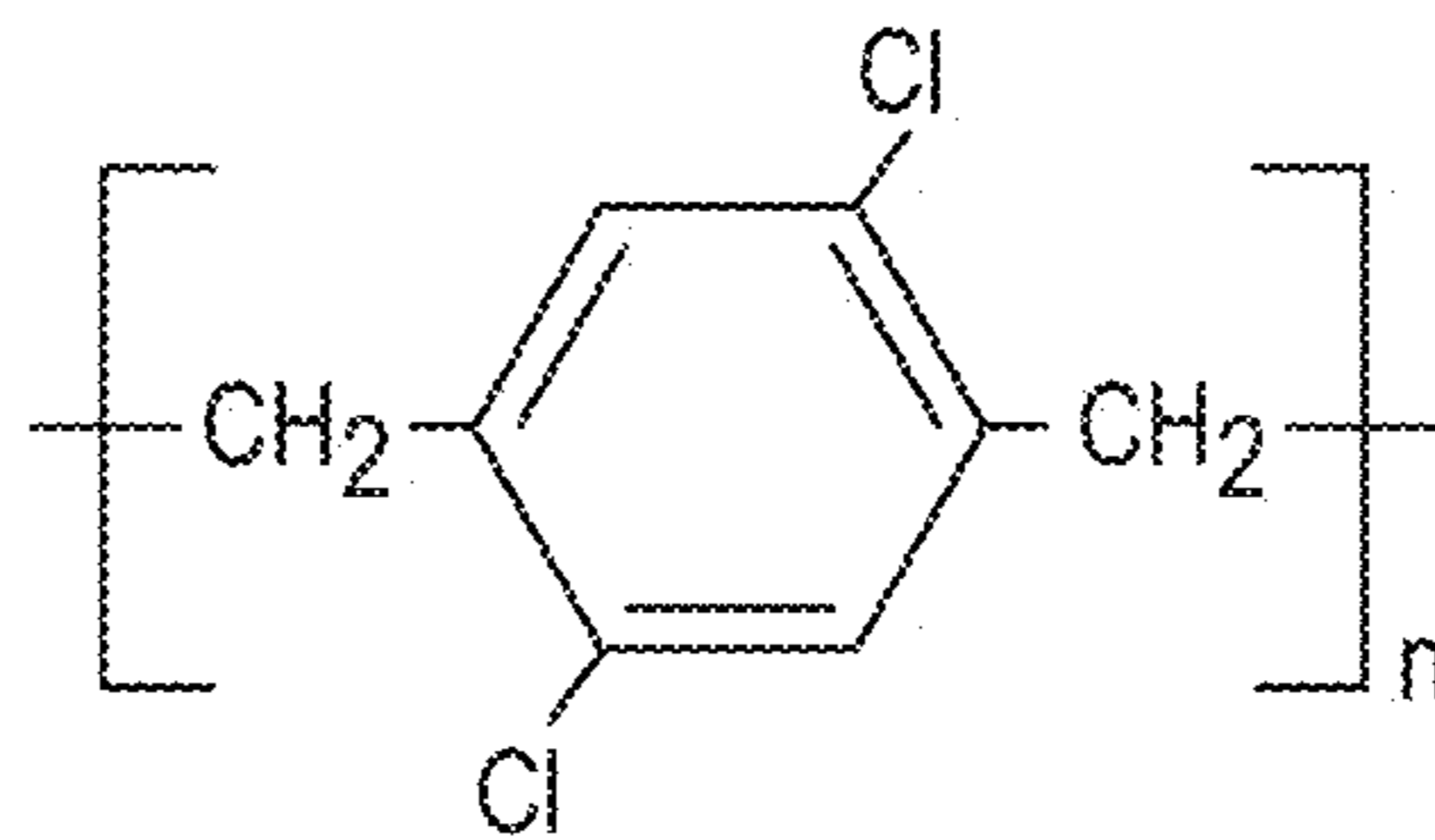
Parylene D
