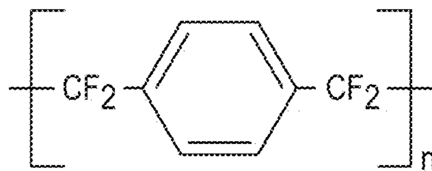
Parylene HT
