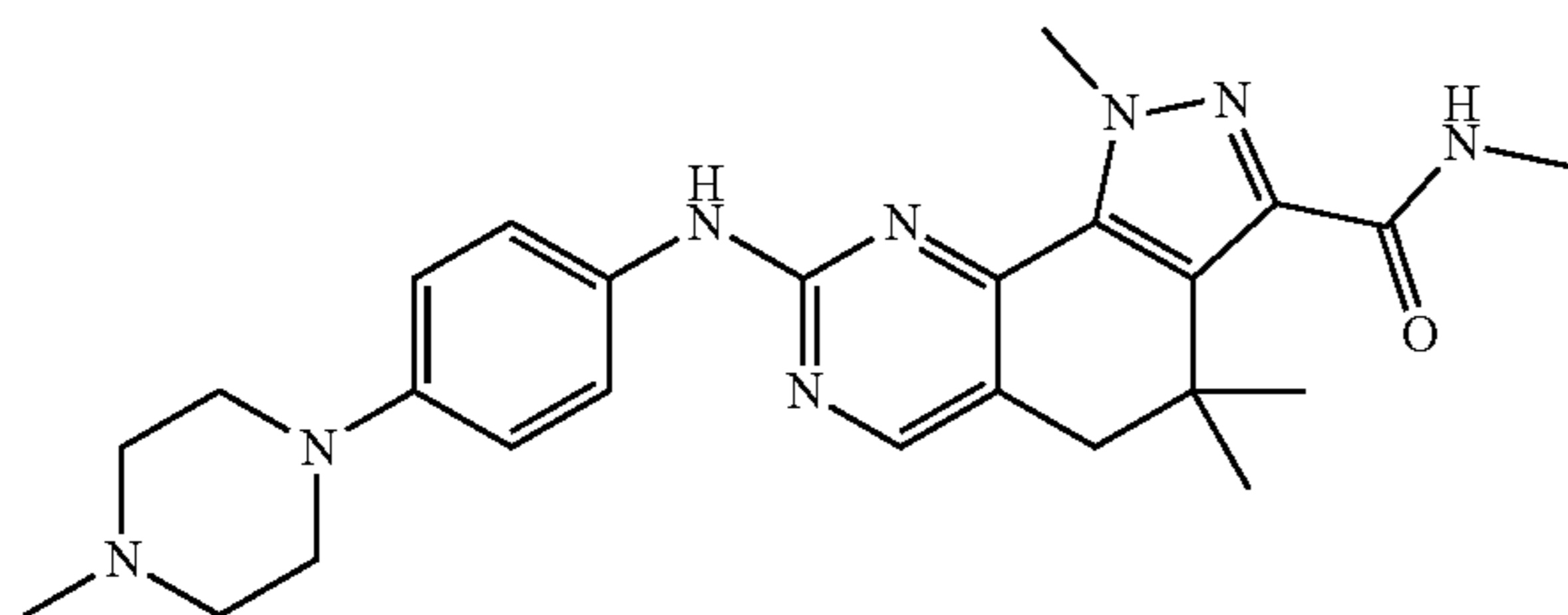
Miliciclib Chemical Structure Molecular Weight: 460.57
