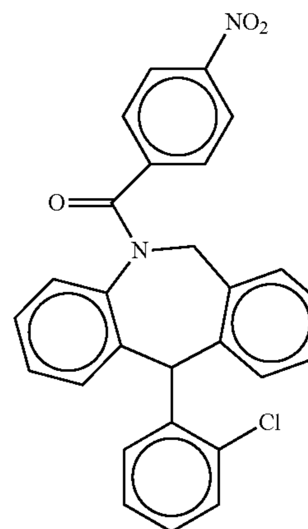
NC381 Chemical Structure Molecular Weight: 454
