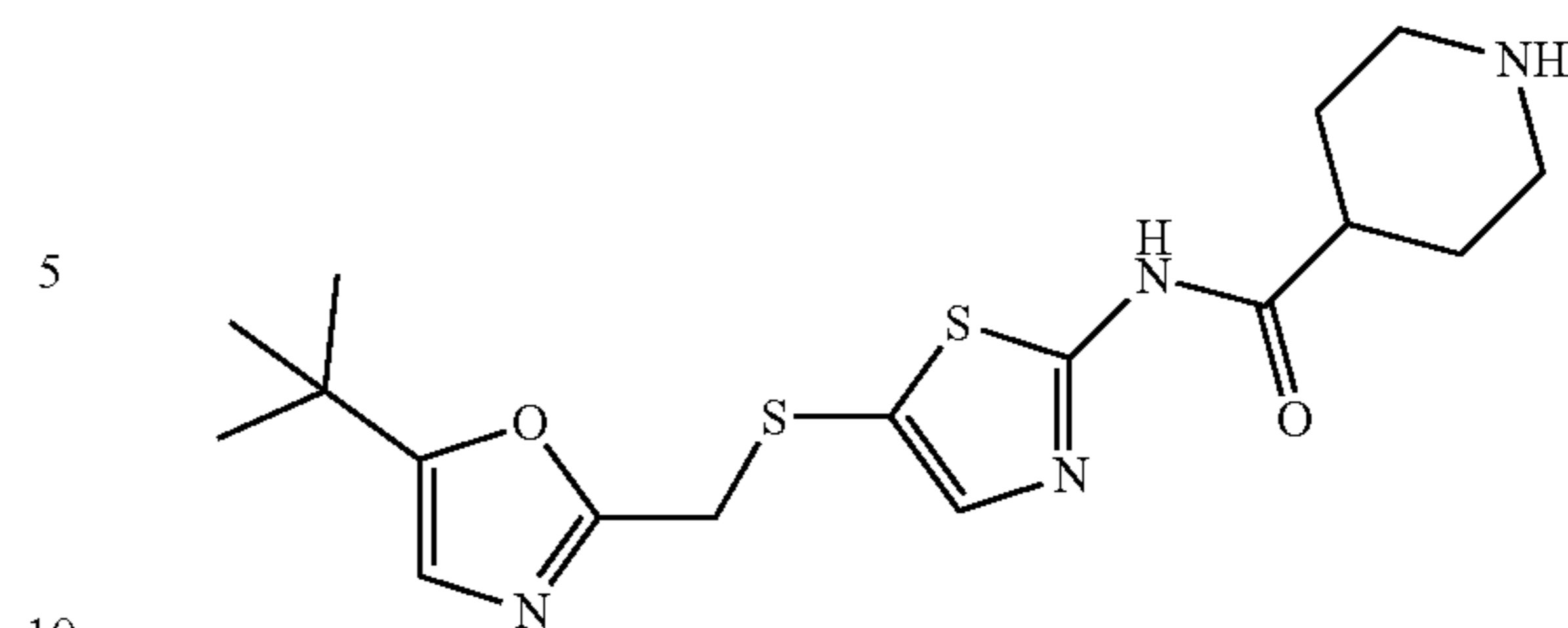
SNS032 Chemical Structure Molecular Weight: 380.53
