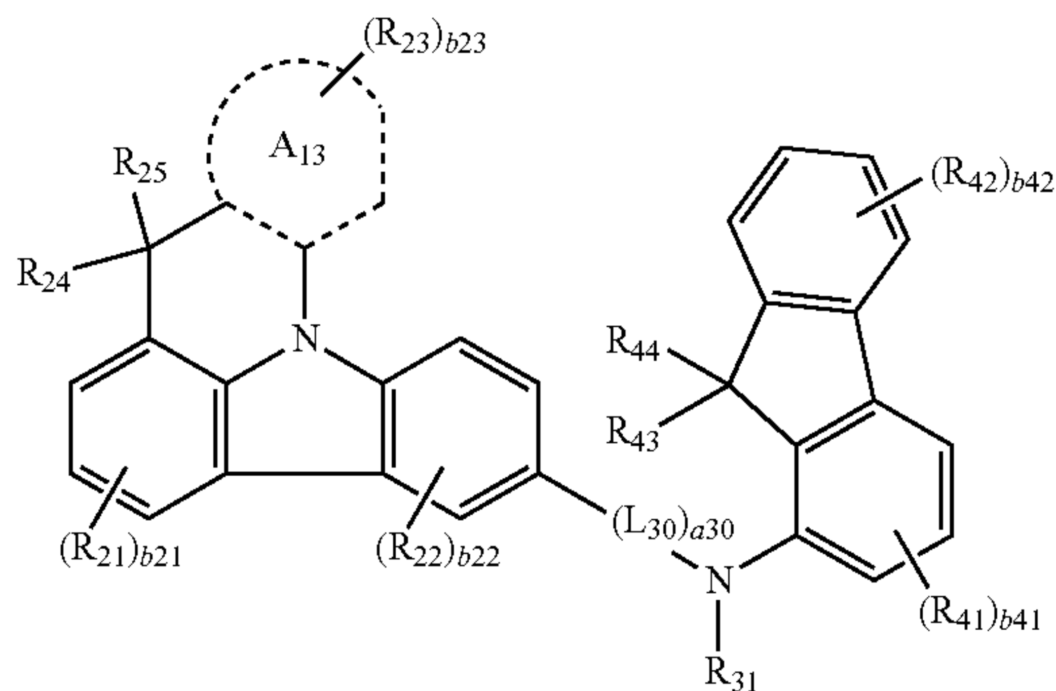
Formula 2B(12)
