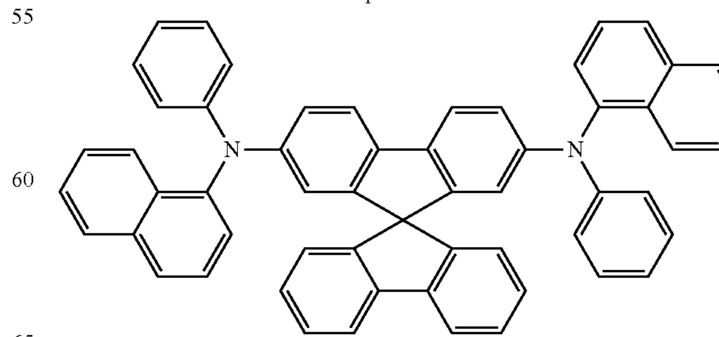
Spiro-NPB
