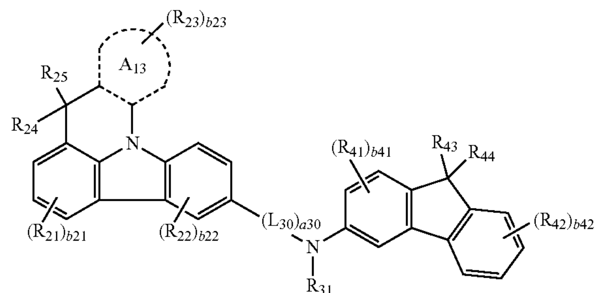
Formula 2B(10)
