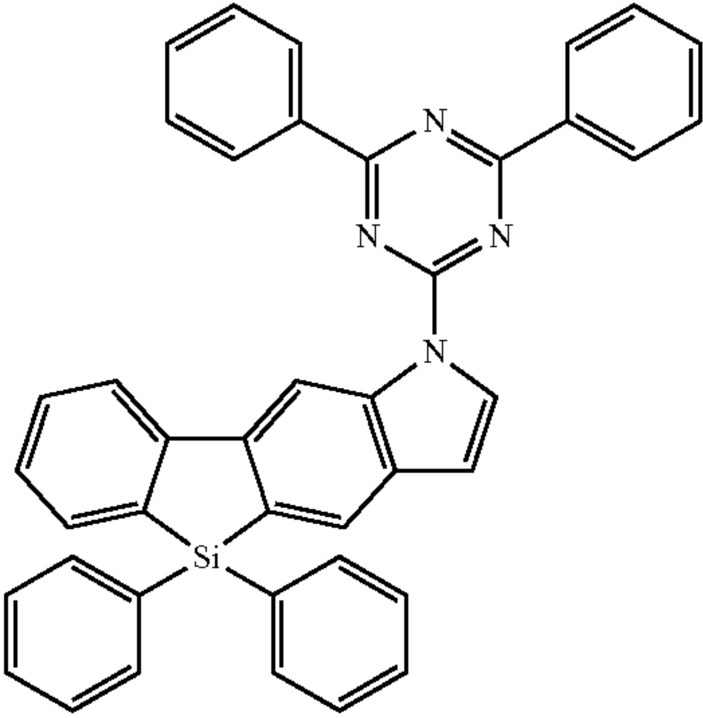
1-7
