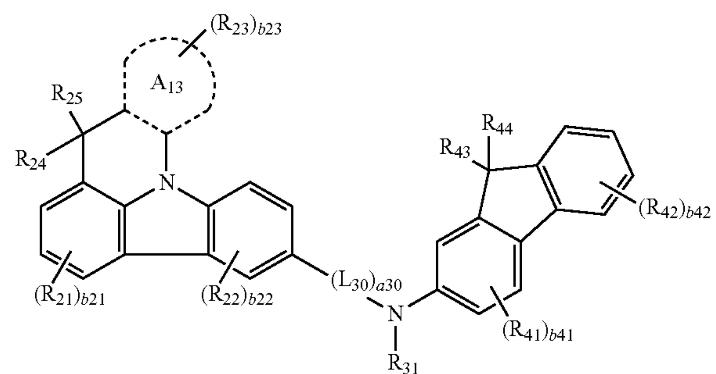
Formula 2B(11)
