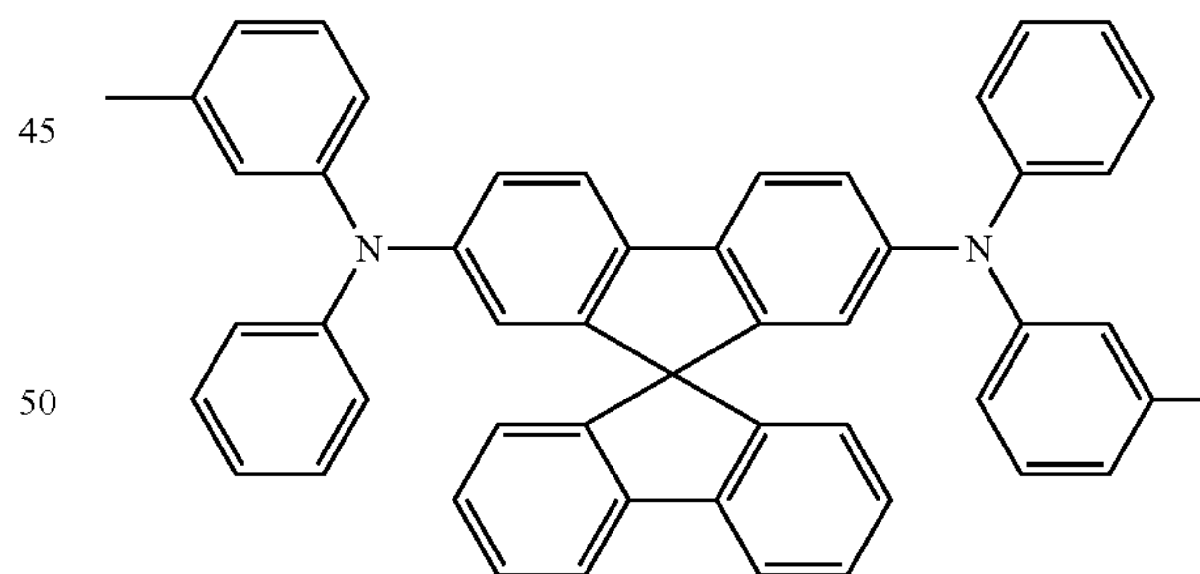
Spiro-TPD
