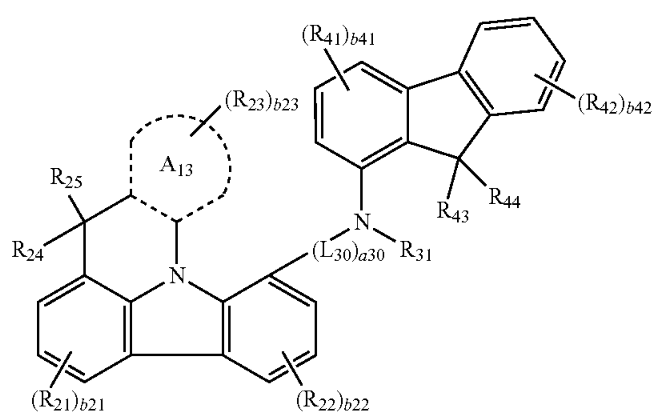
Formula 2B(5)
