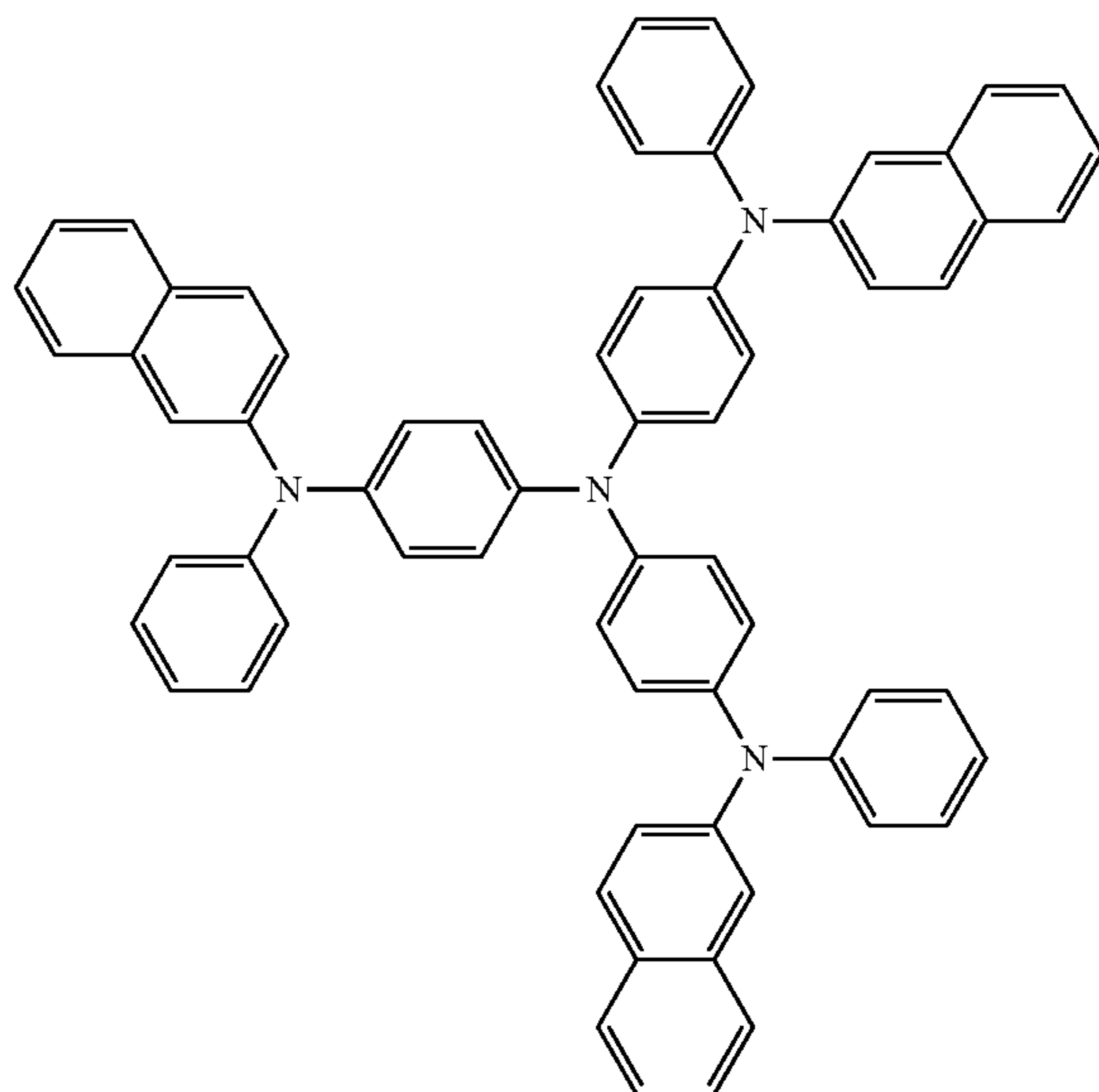
2-TNATA
