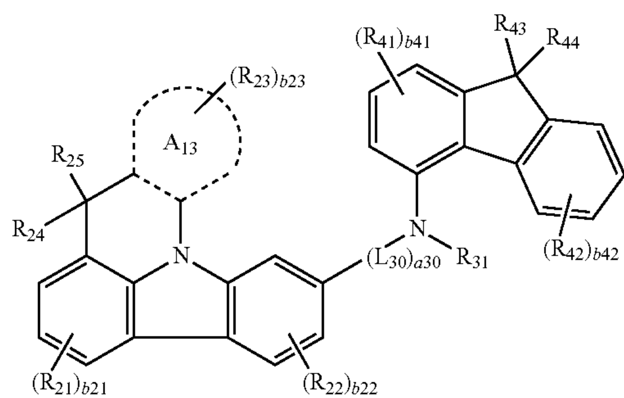
Formula 2B(5)
