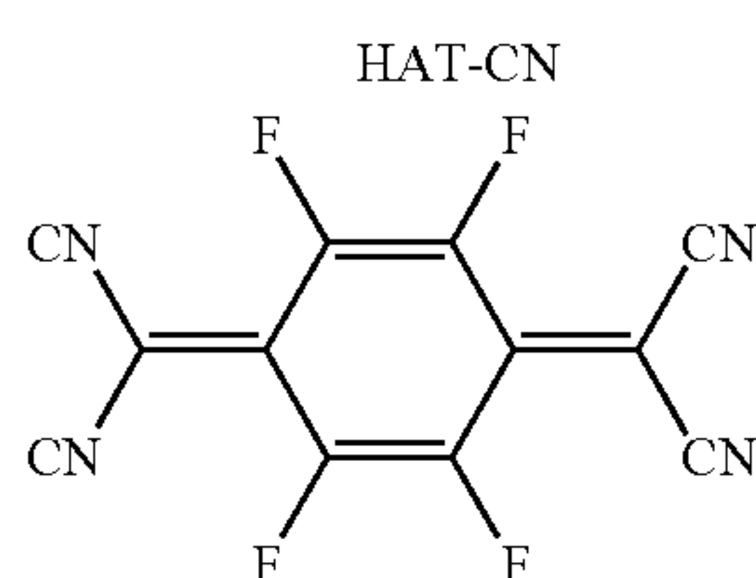
F4-TCNQ
