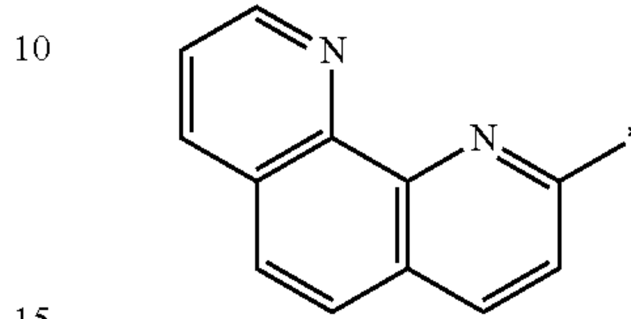
Formula 10-112
