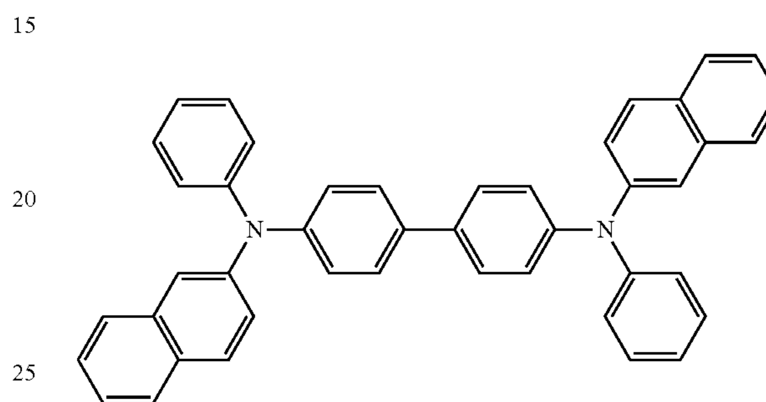
\beta -NPB
