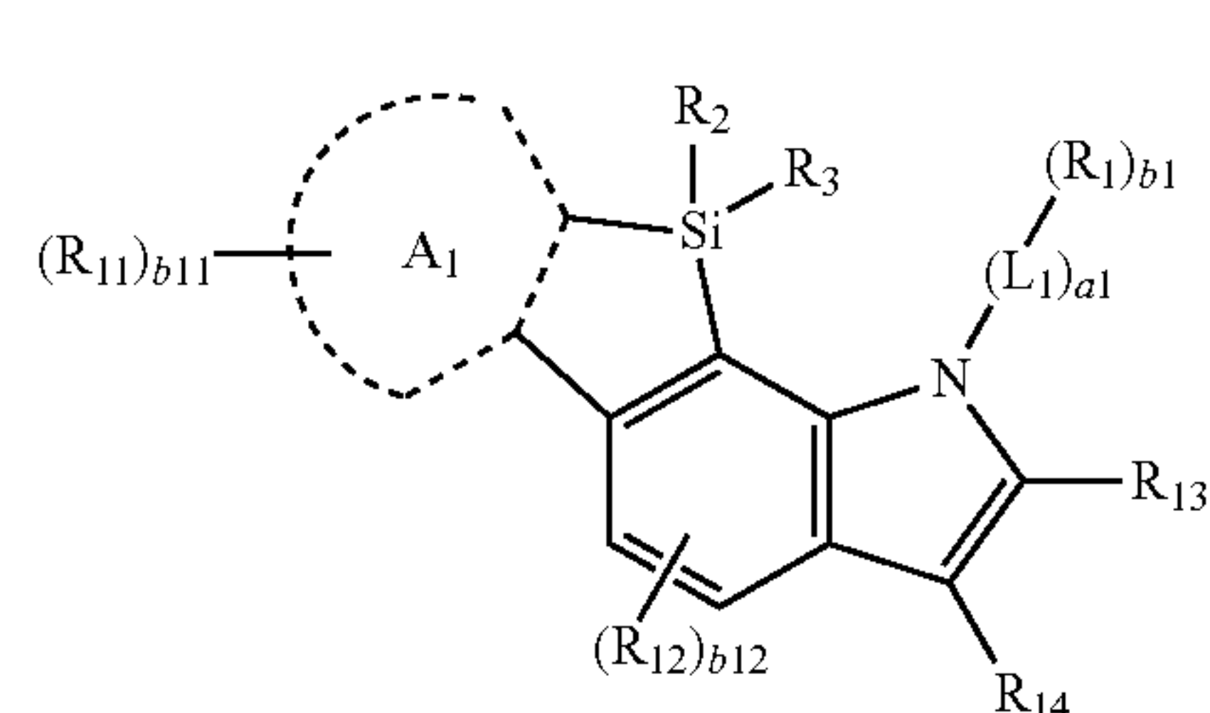
Formula 1A
