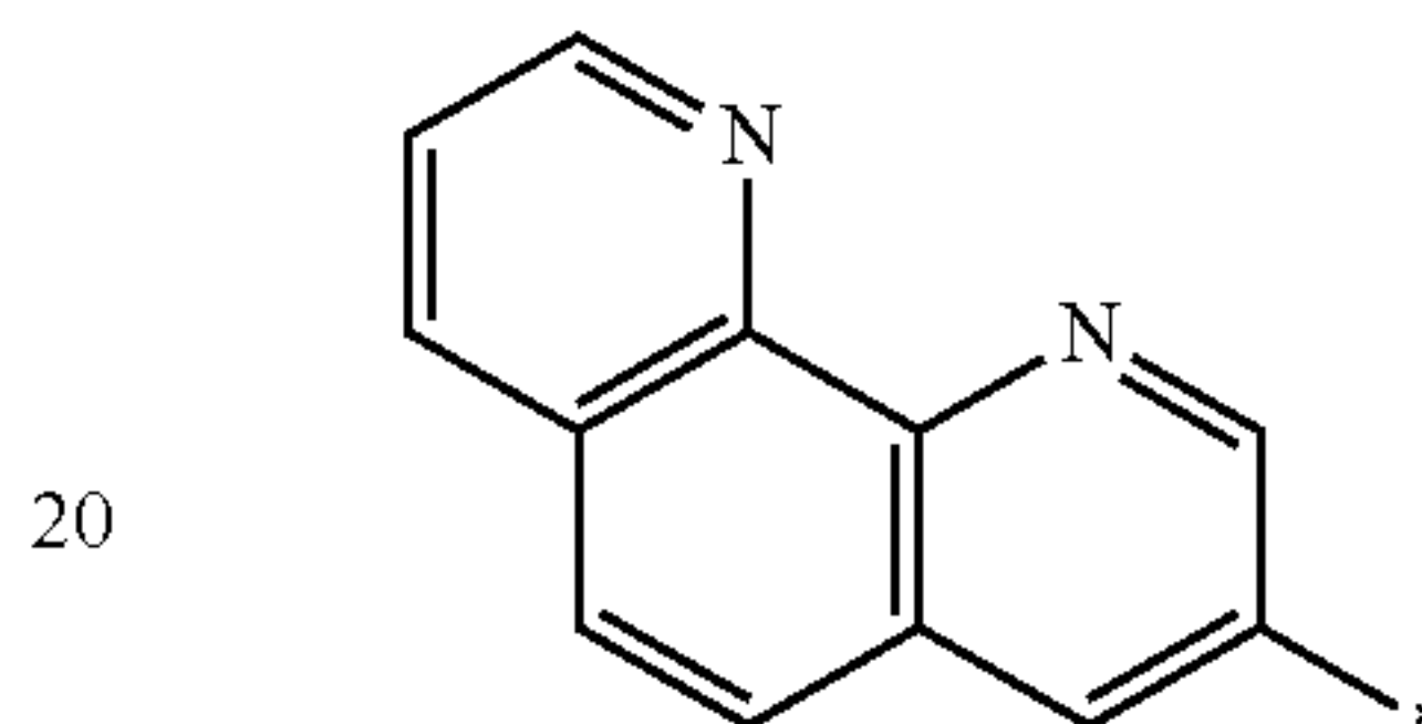
Formula 10-113
