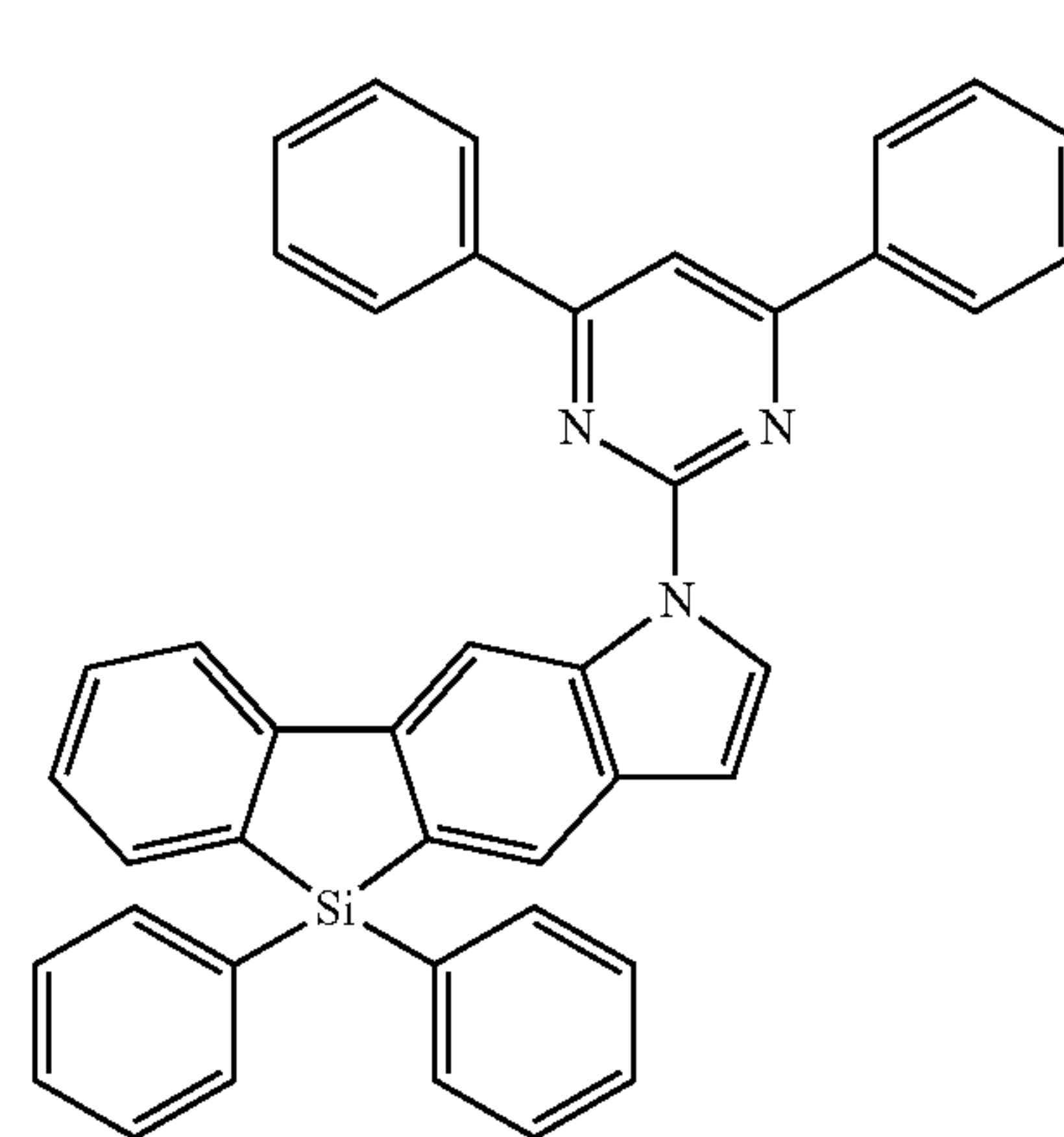
Compound 1-9
