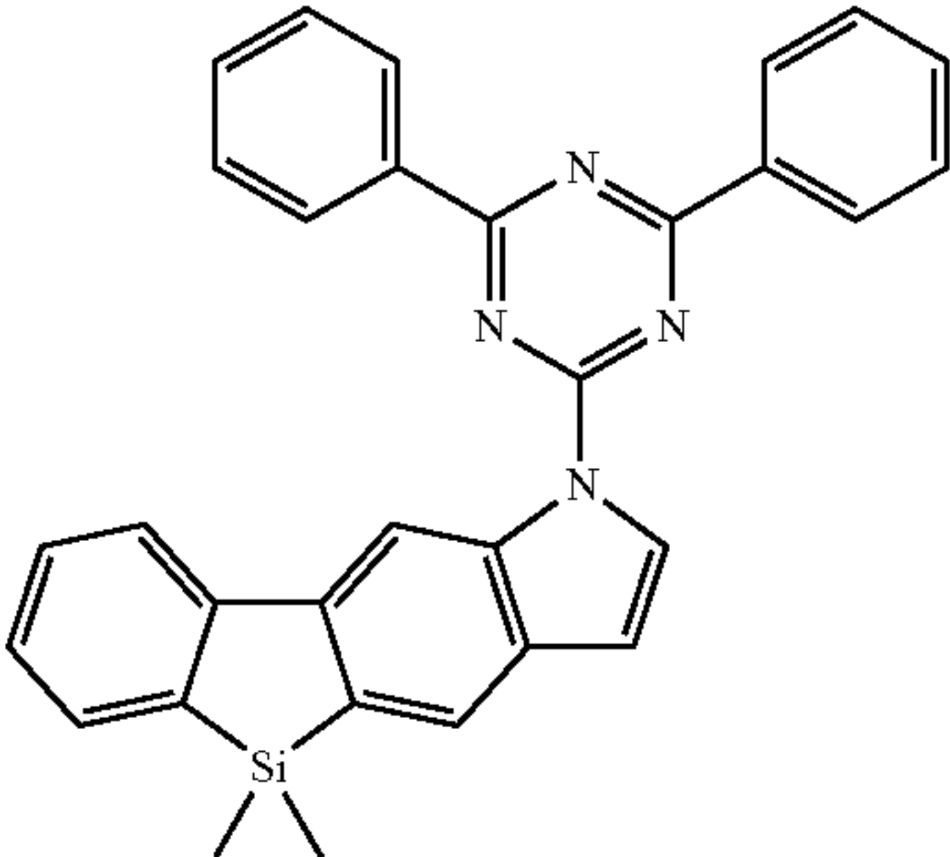
1-4
