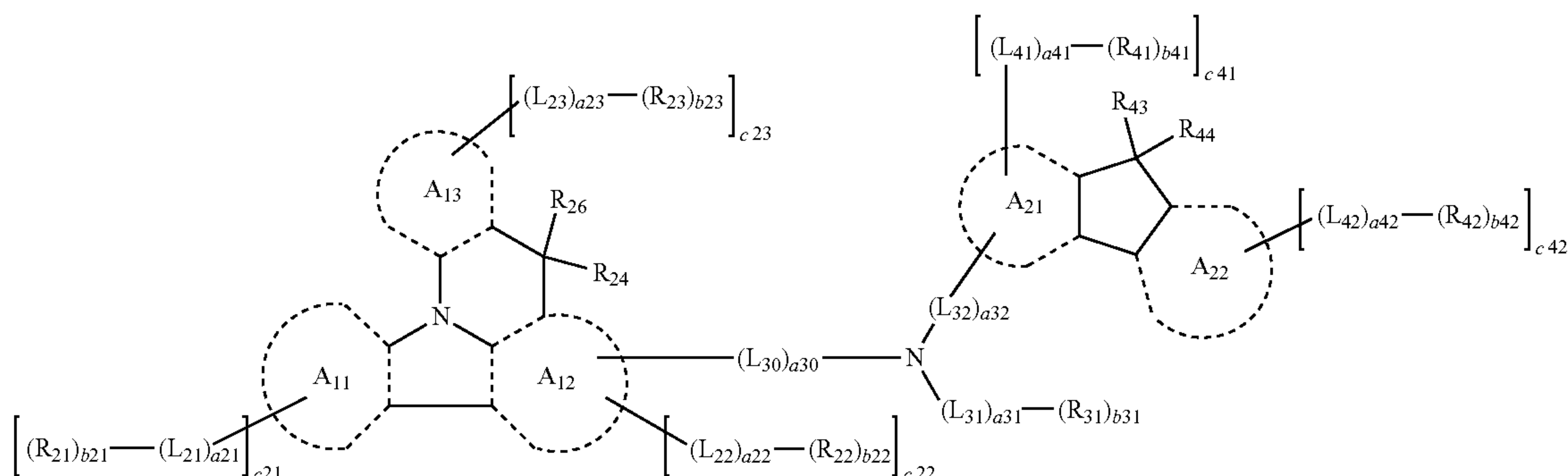
Formula 2A
