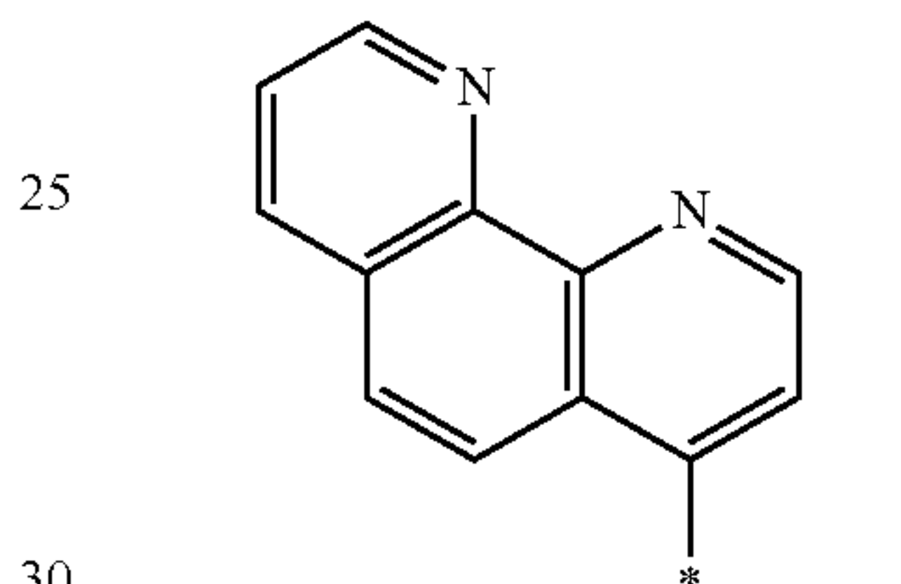
Formula 10-114
