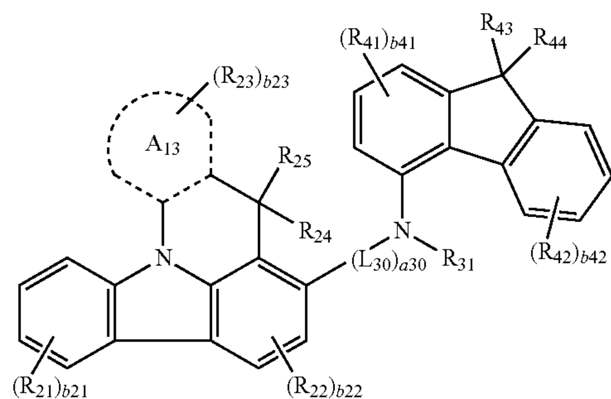
Formula 2A(2)
