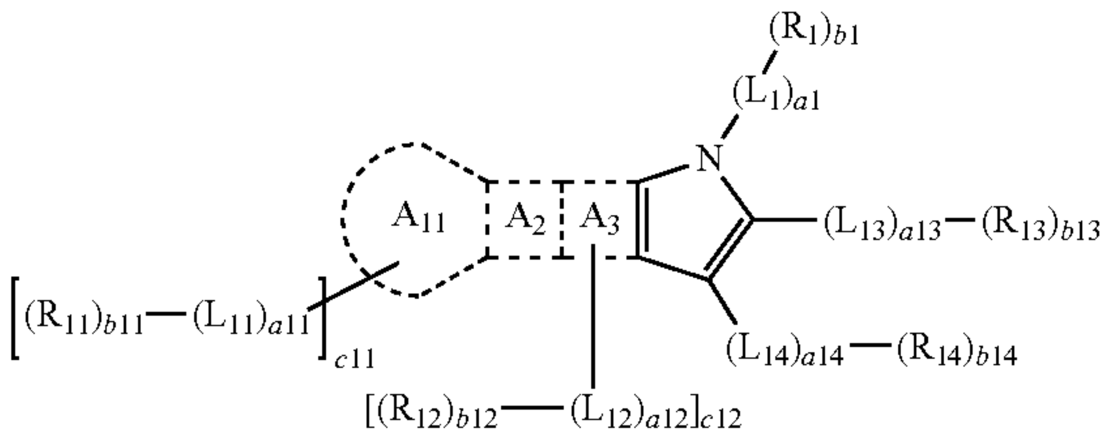
Formula 1
