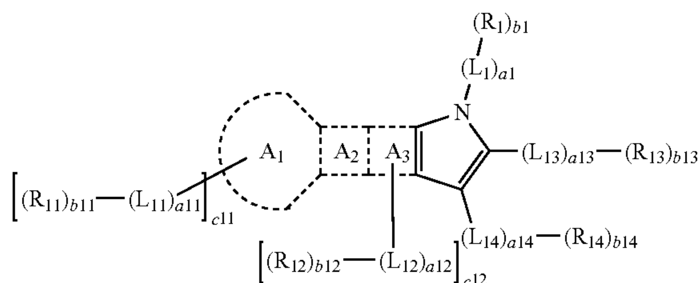
Formula 1
