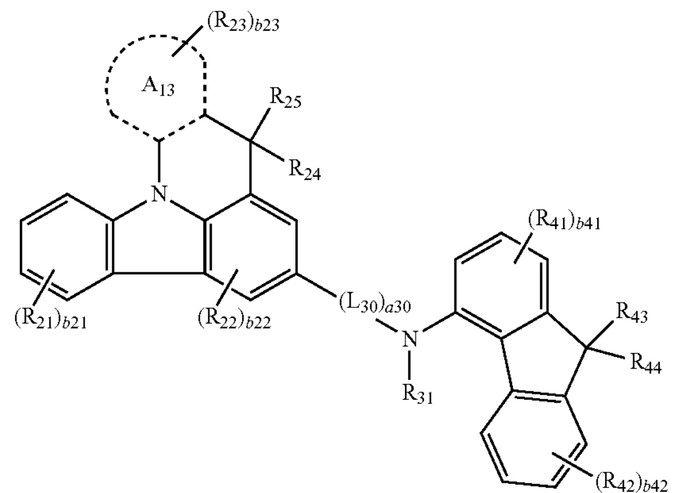
Formula 2A(5)
