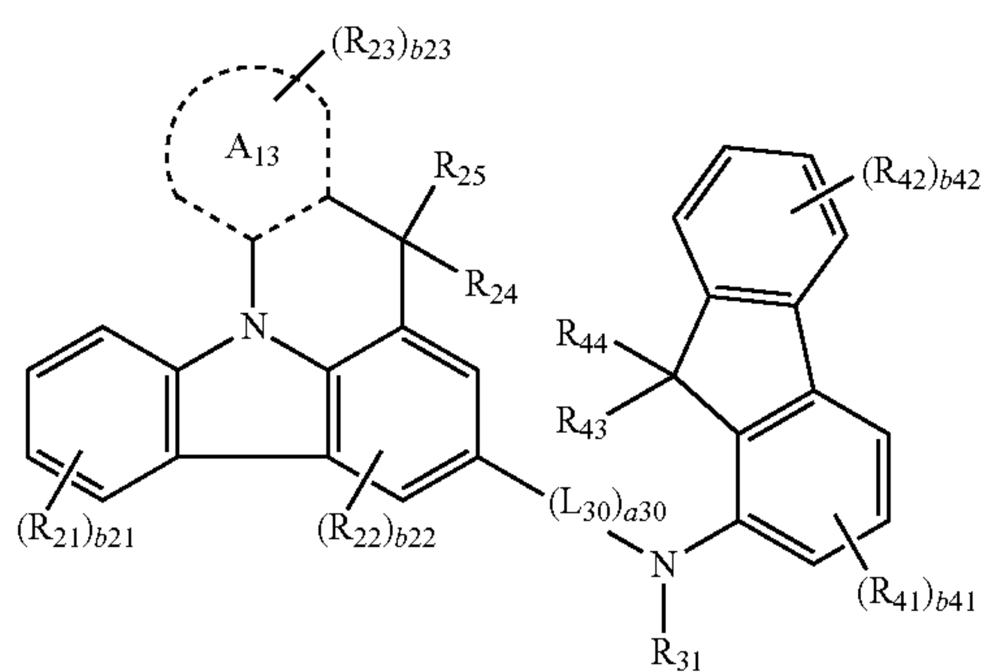
Formula 2A(9)
