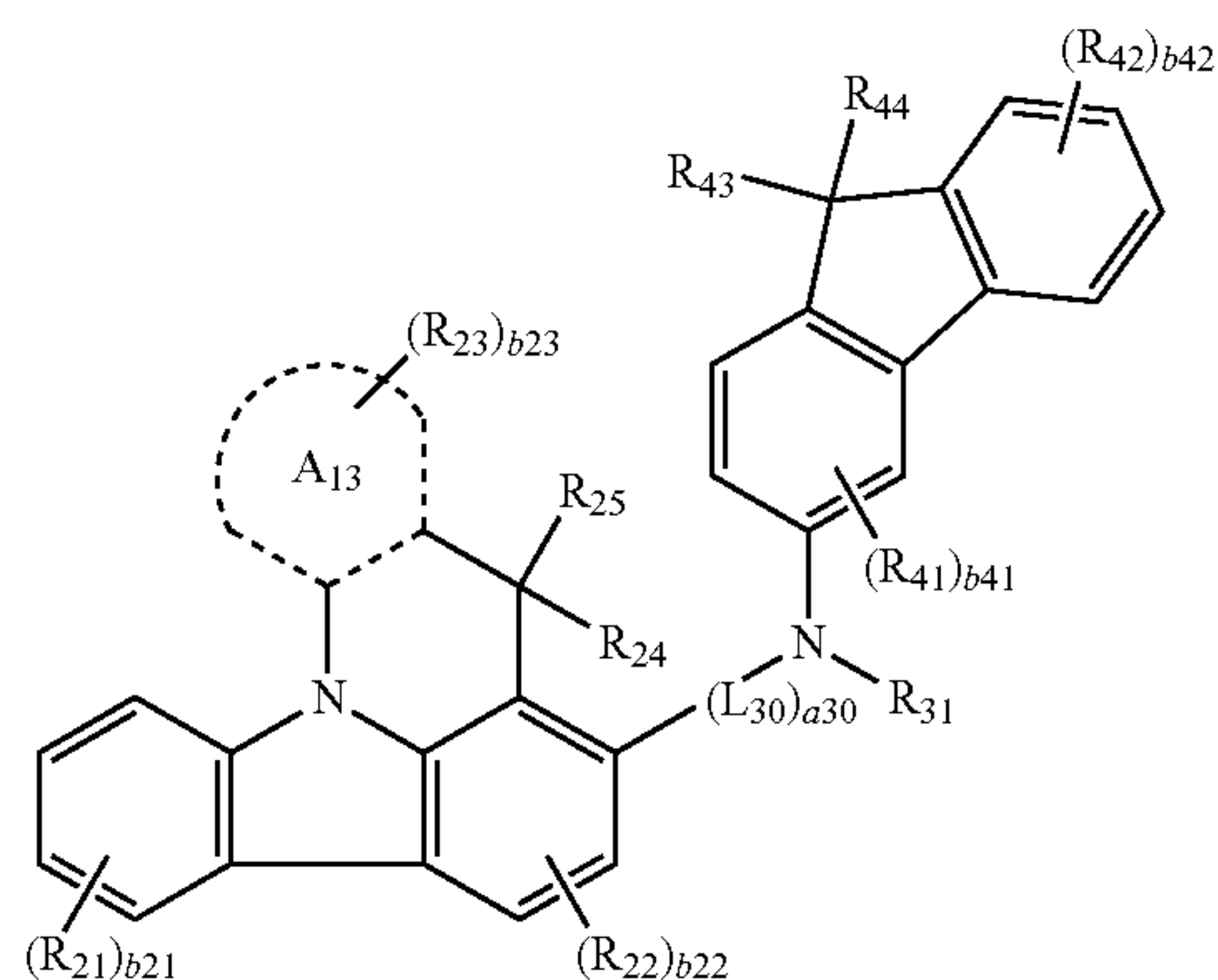
Formula 2A(2)
