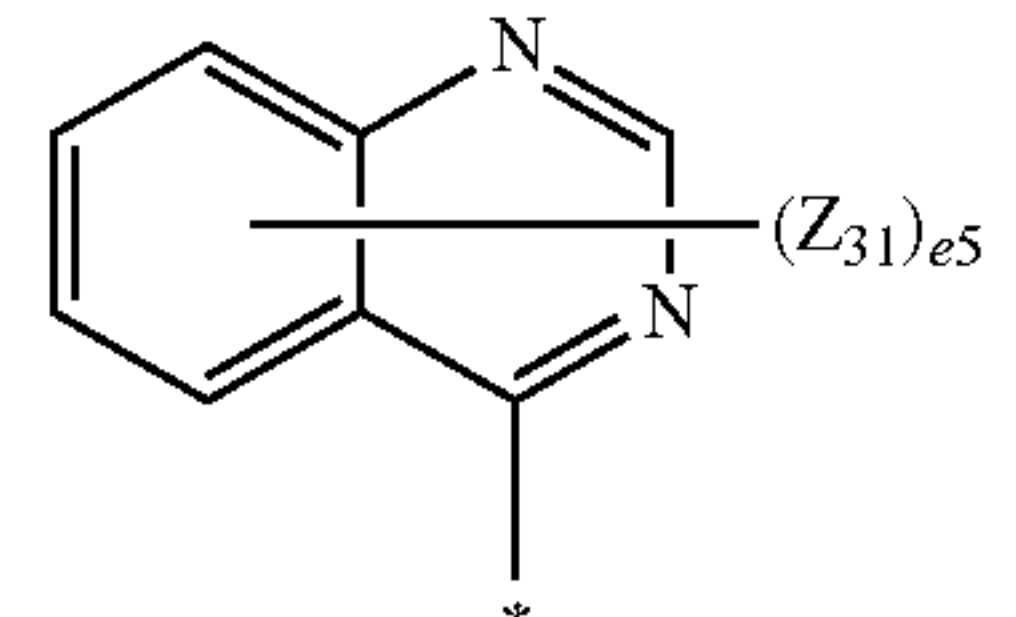
Formula 6-25
