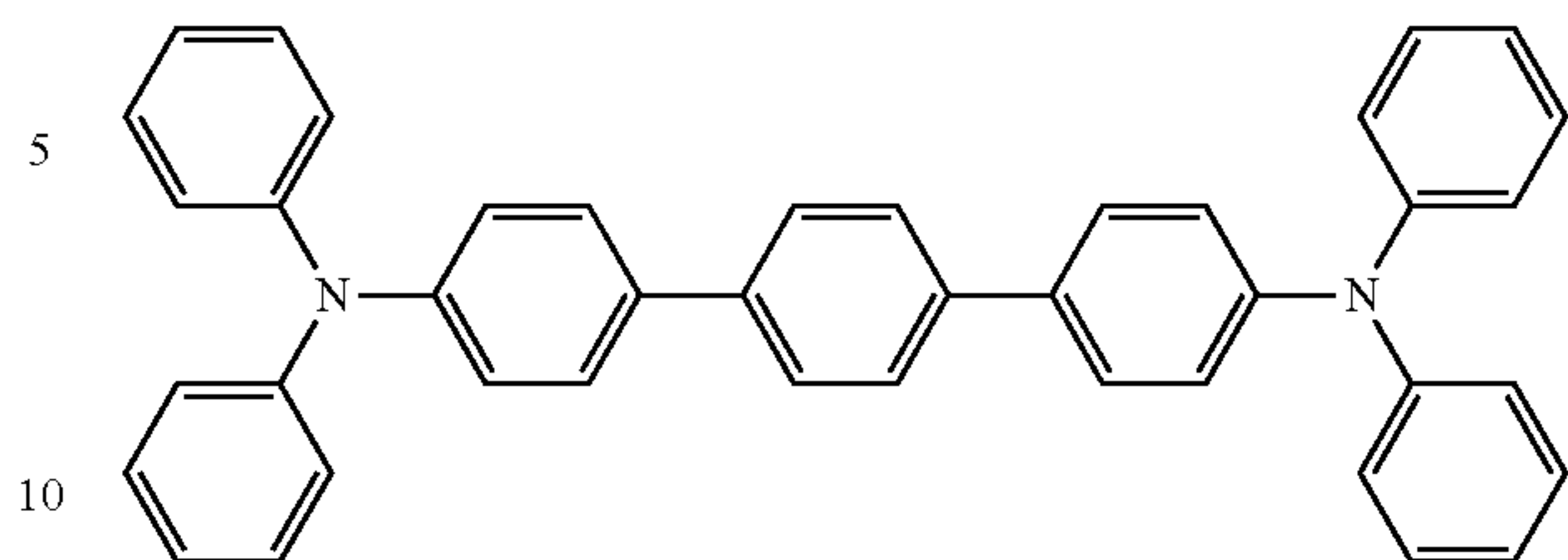
CP3
