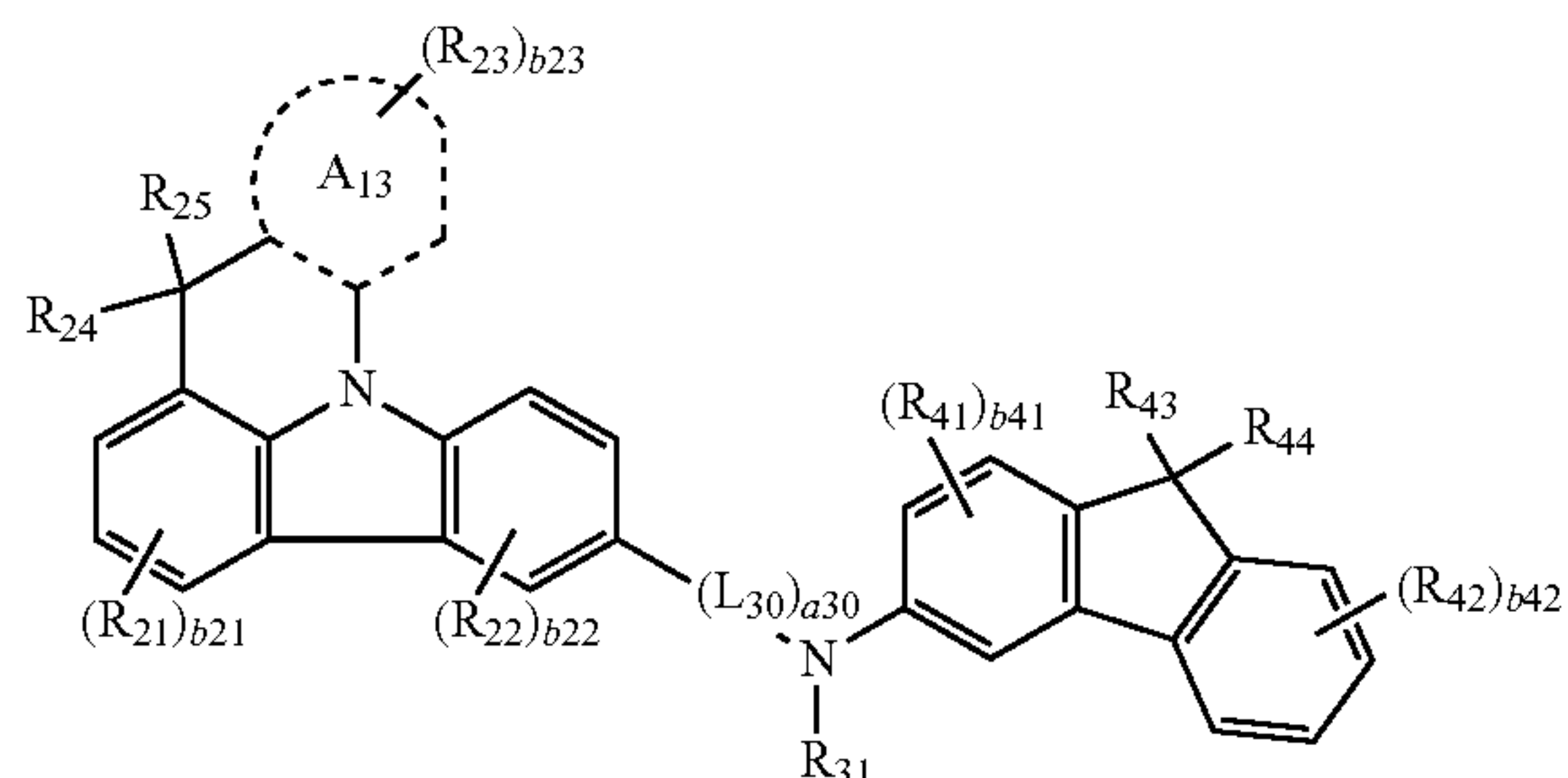
Formula 2B(10)
