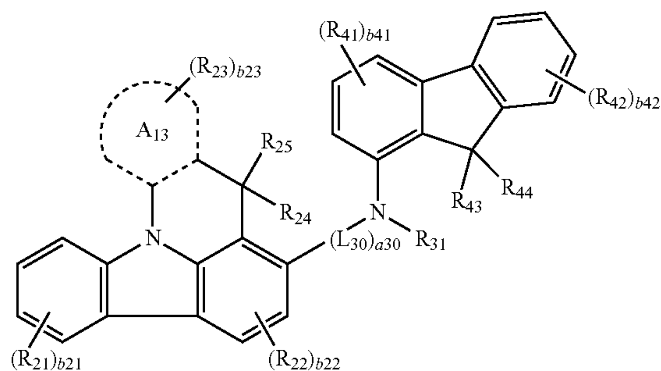
Formula 2A(4)
