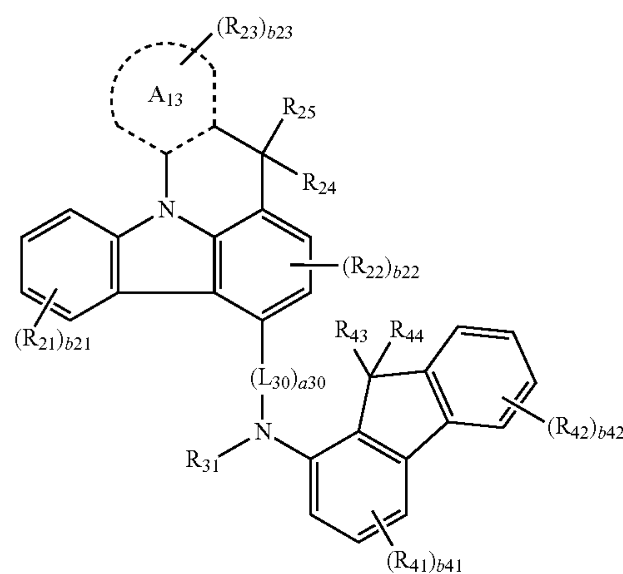
Formula 2A(12)
