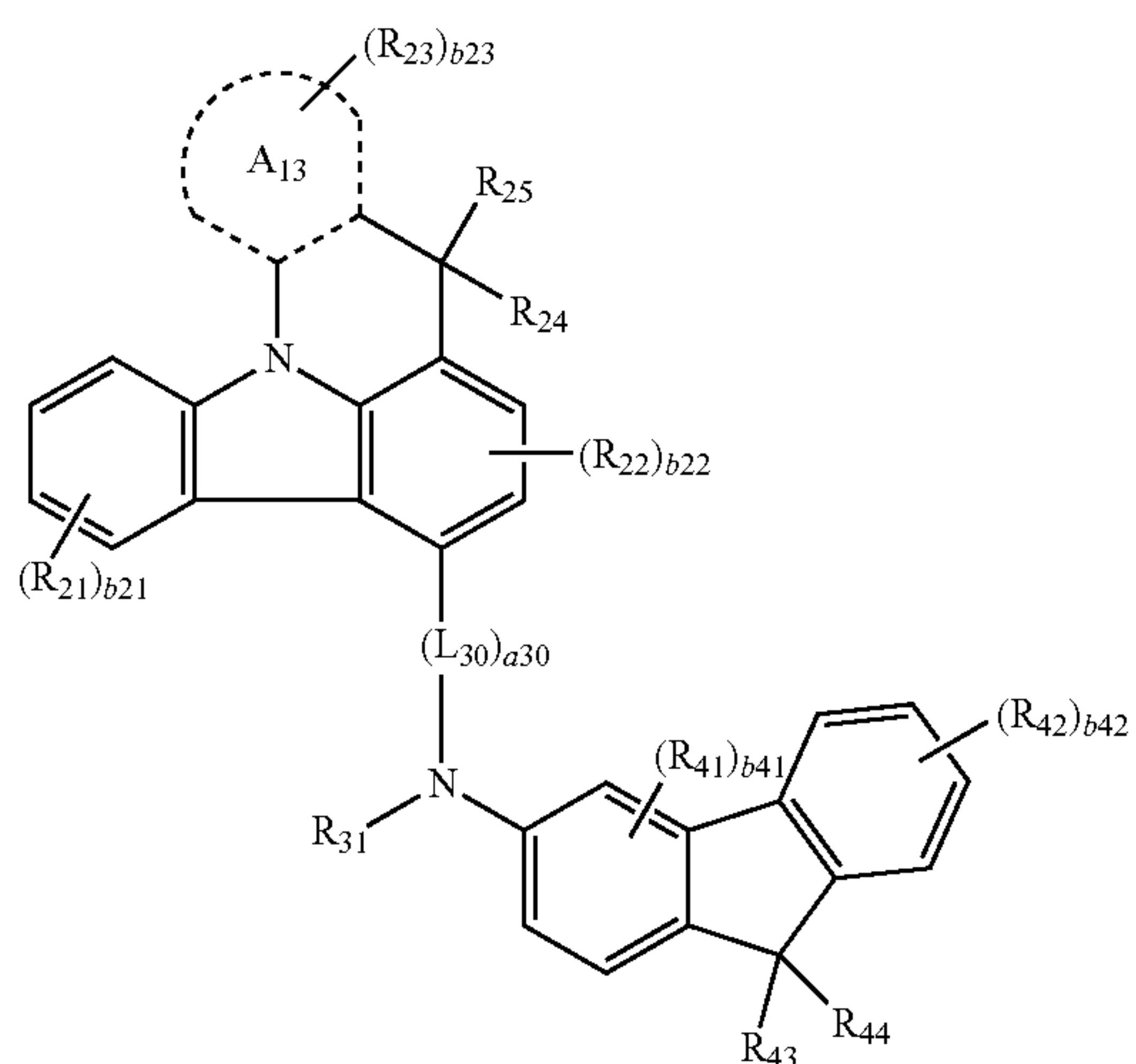
Formula 2A(10)
