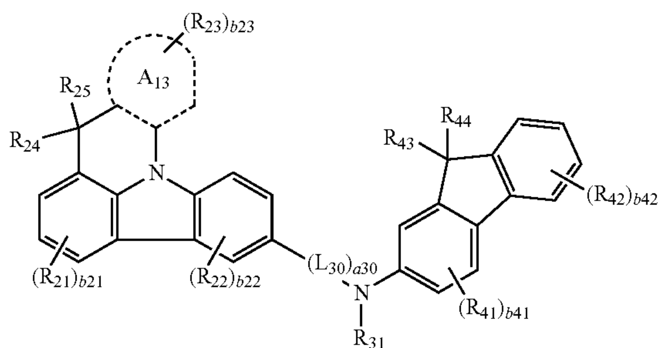
Formula 2B(11)
