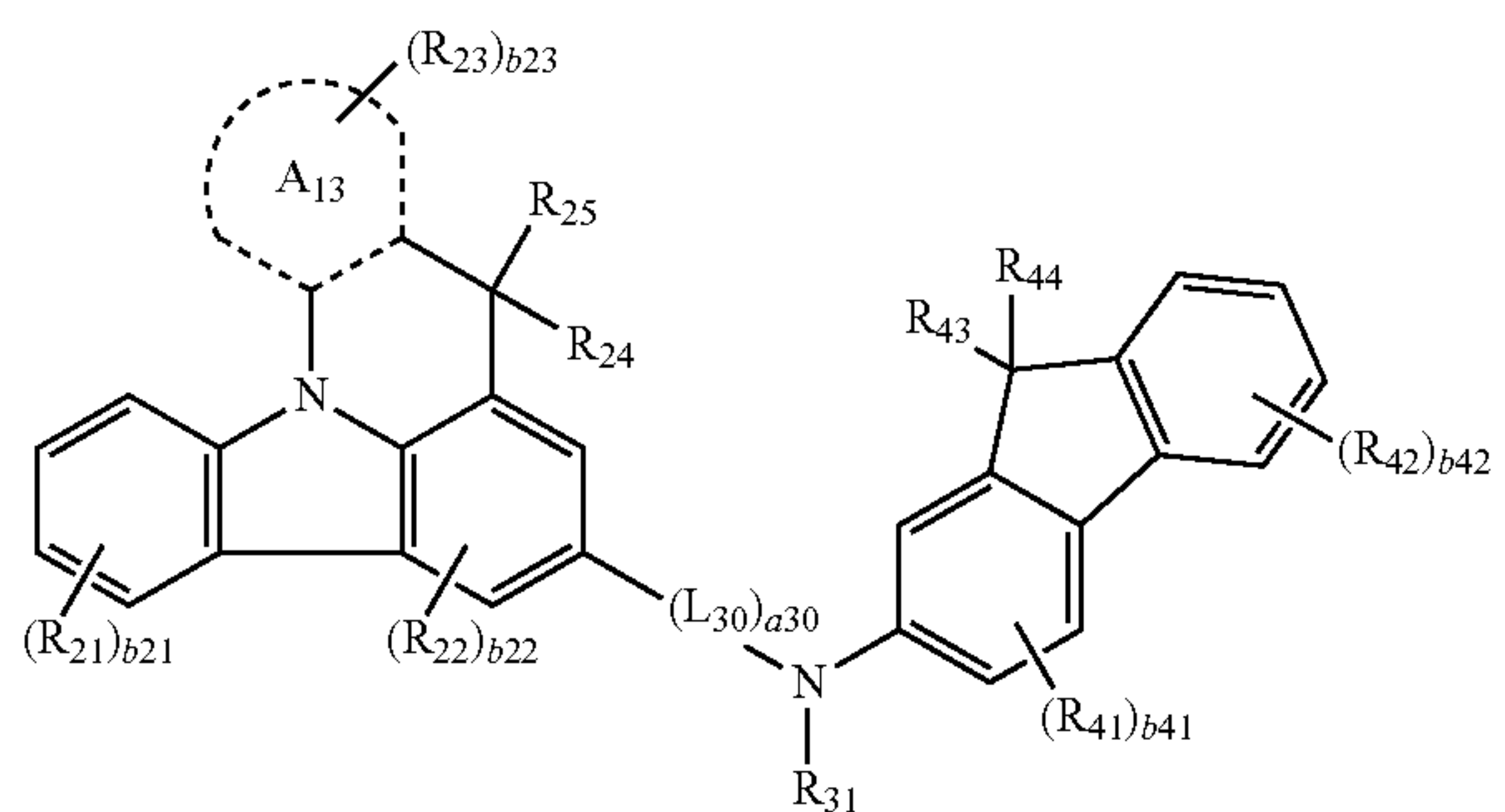
Formula 2A(8)
