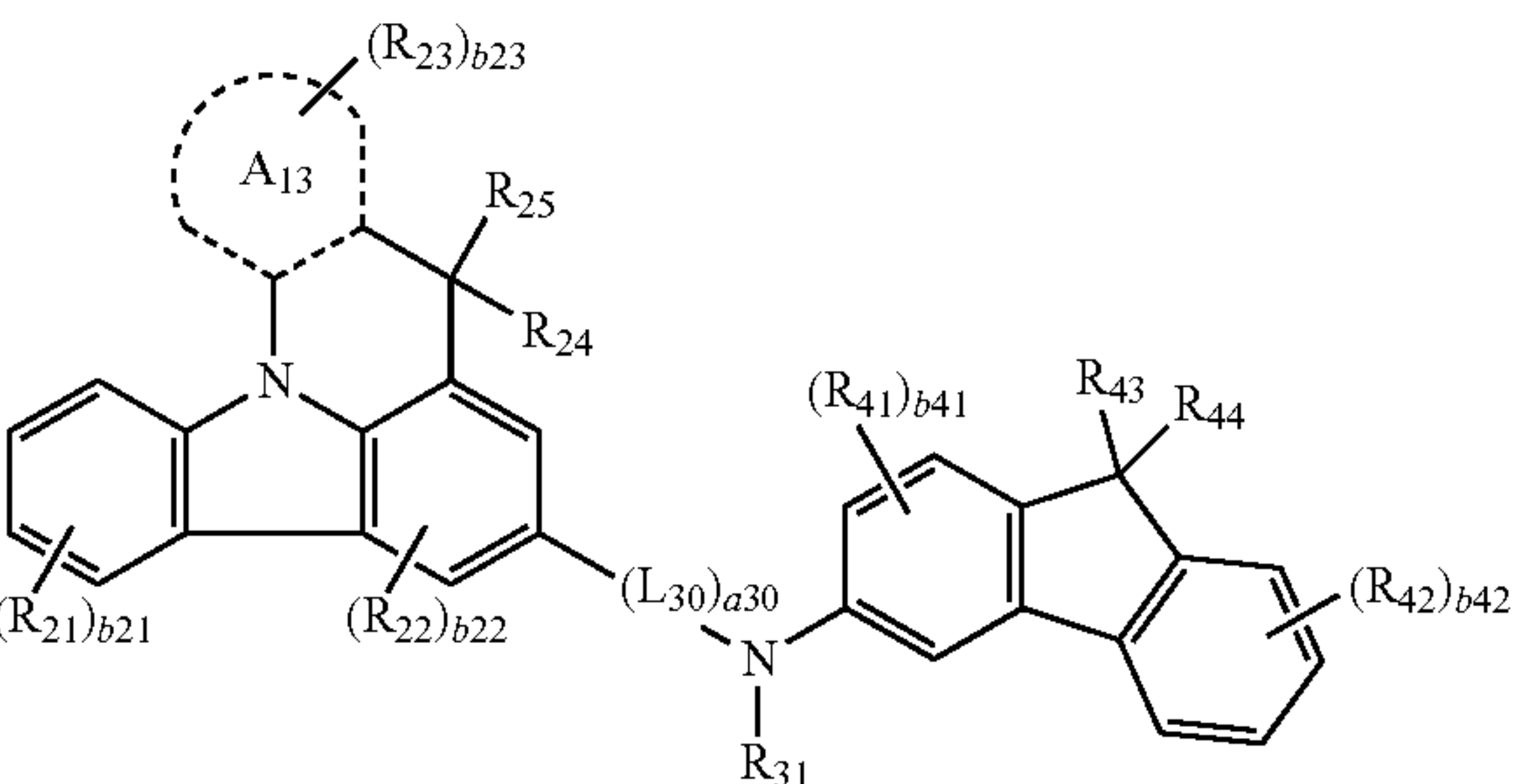
Formula 2A(6)
