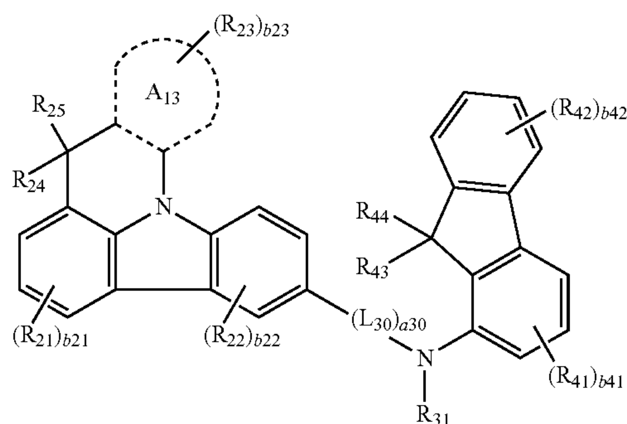
Formula 2B(12)
