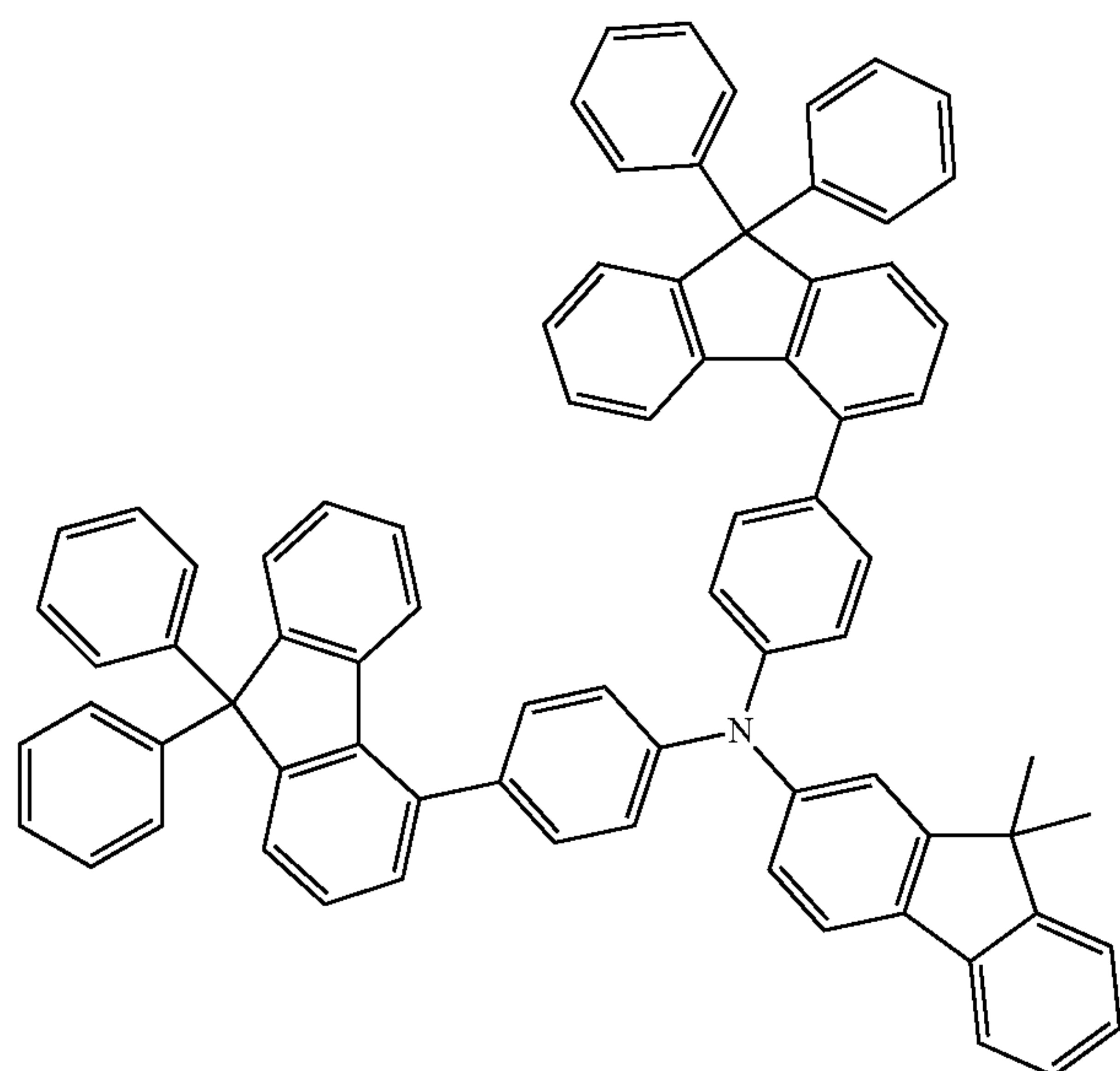
formula (A-70)
