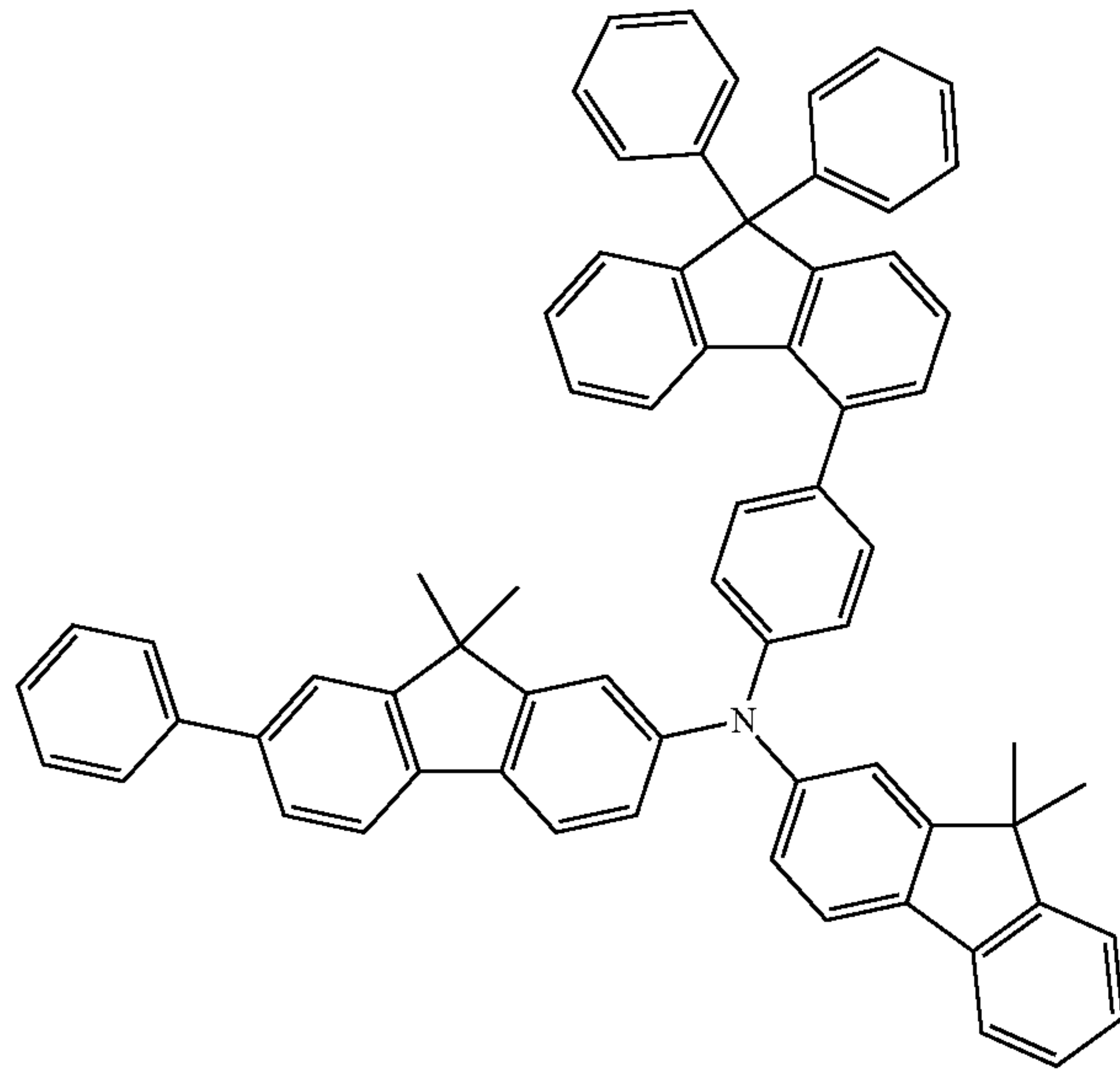
formula (A-66)
