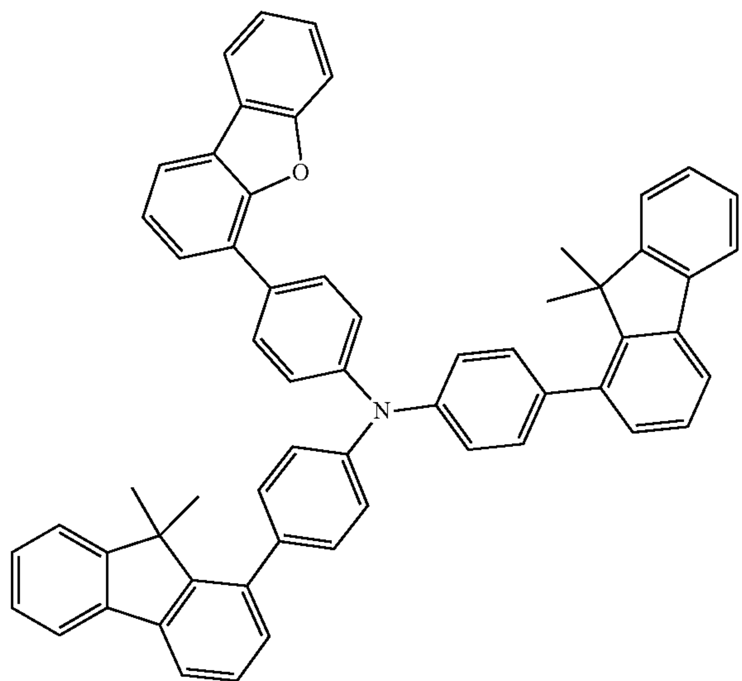
formula (A-51)
