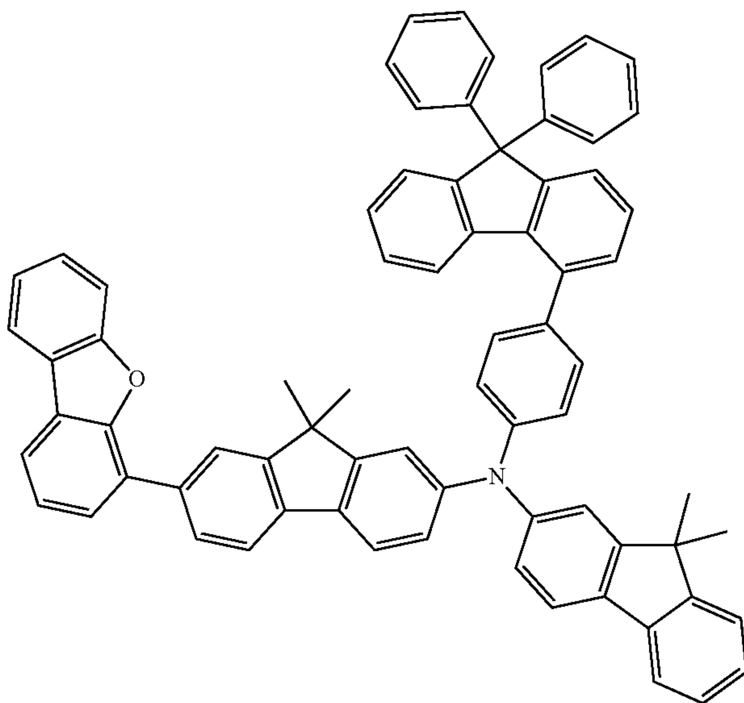
formula (A-68)
