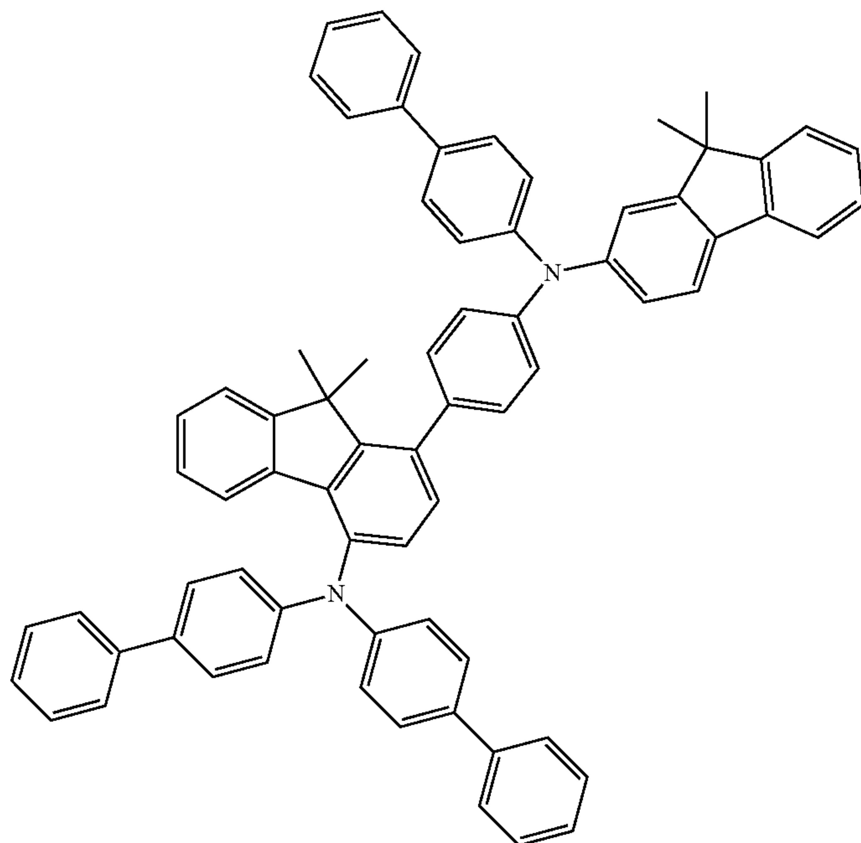
formula (A-49)
