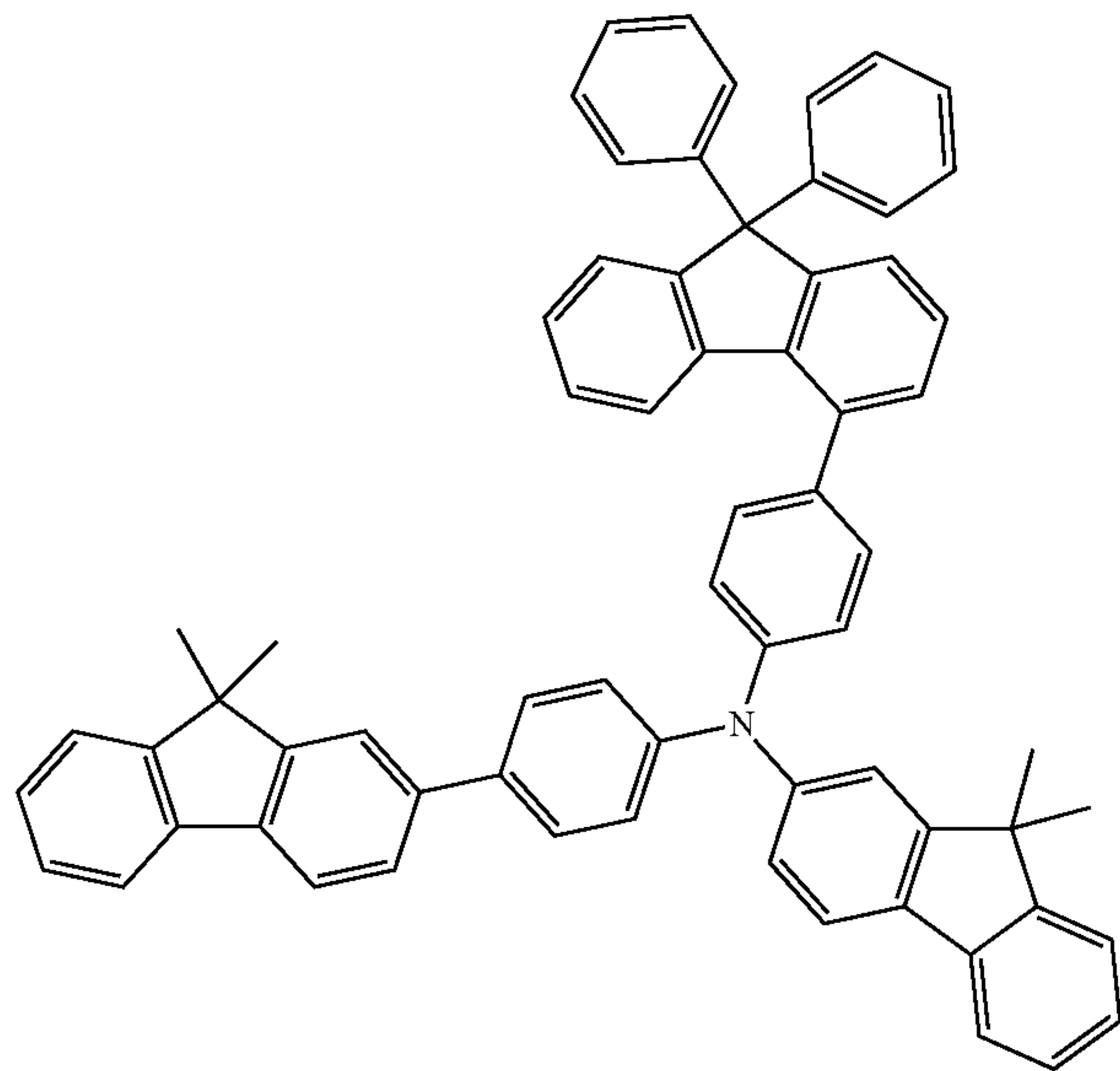
formula (A-69)
