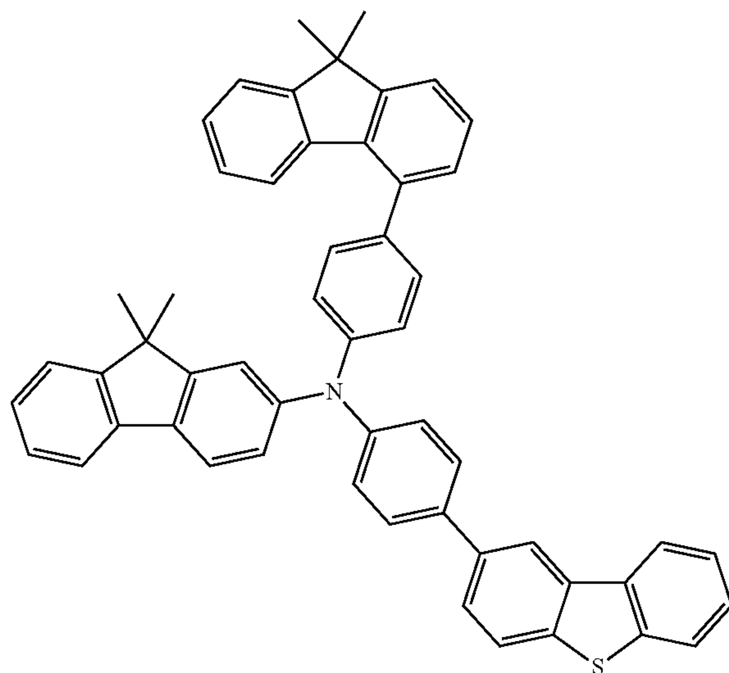
formula (A-10)
