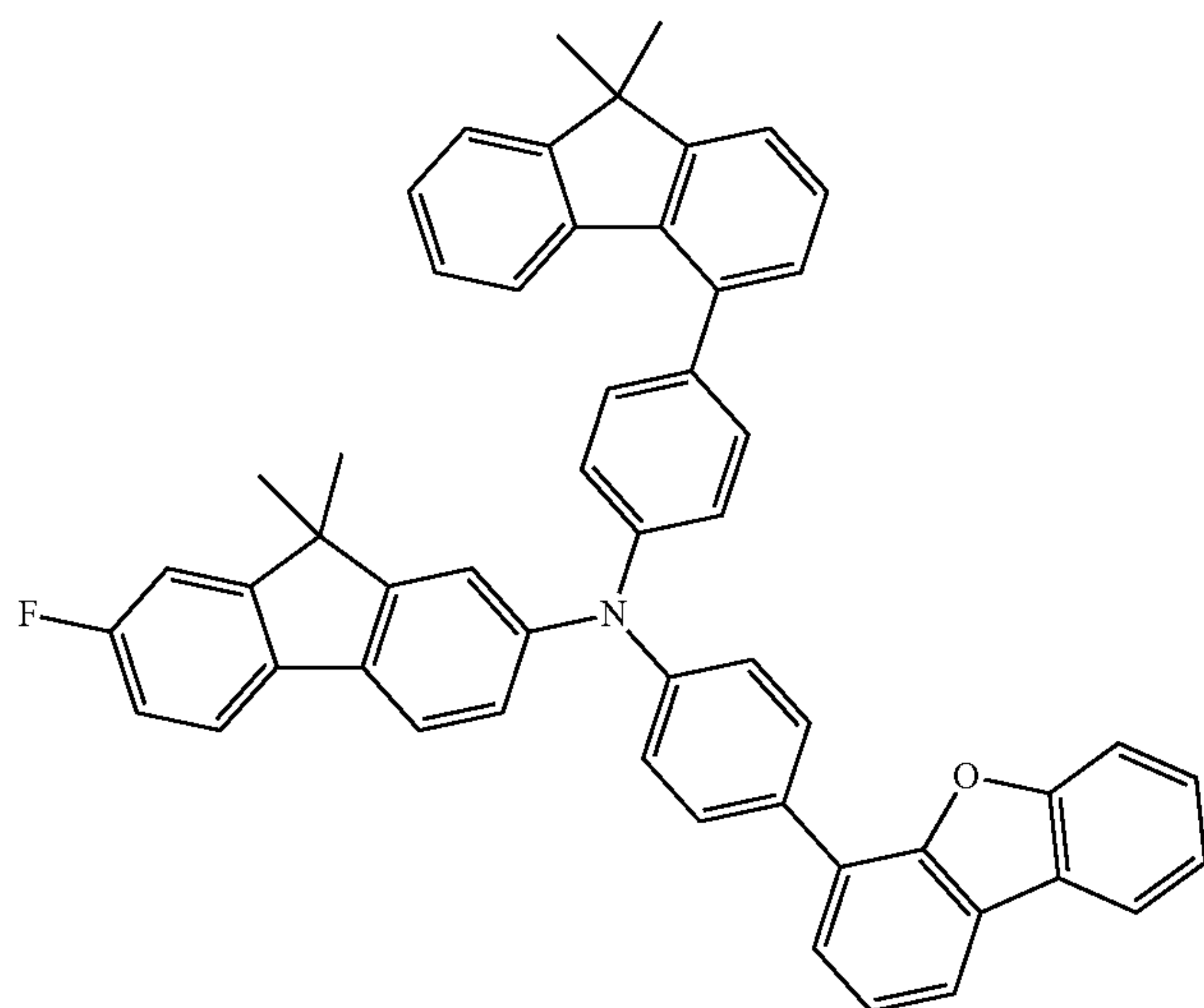
formula (A-30)
