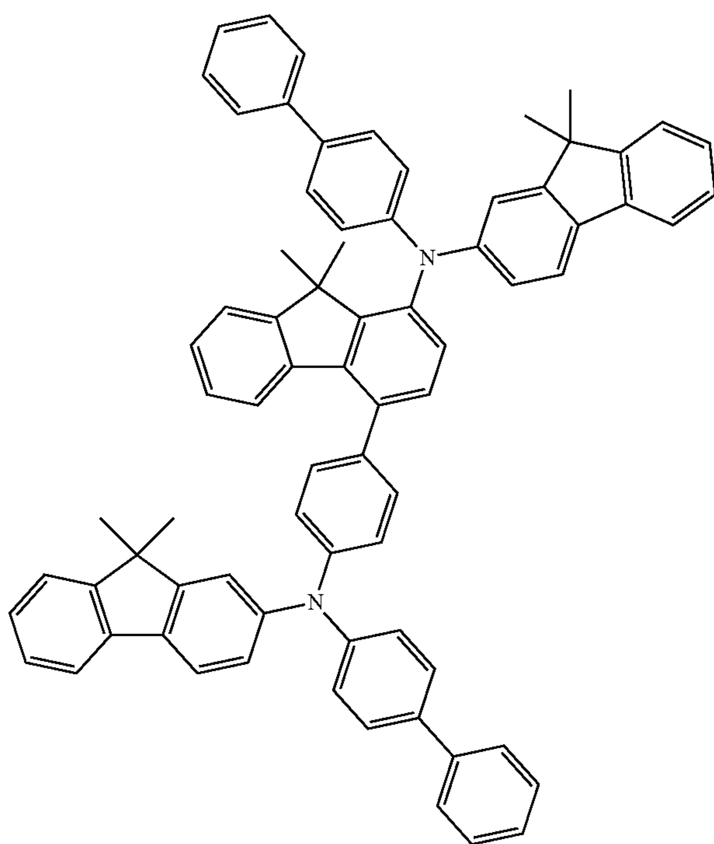
formula (A-48)
