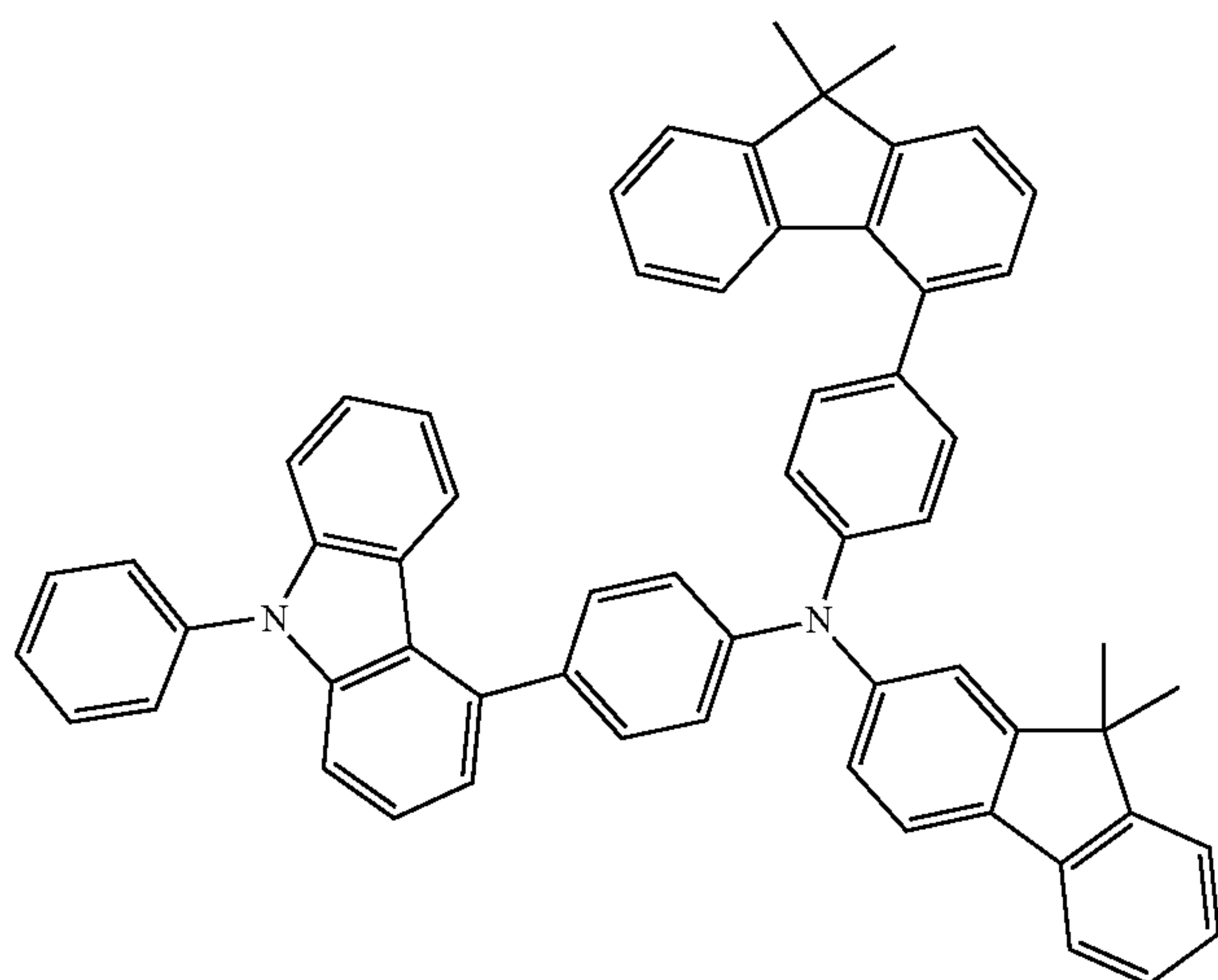
formula (A-65)
