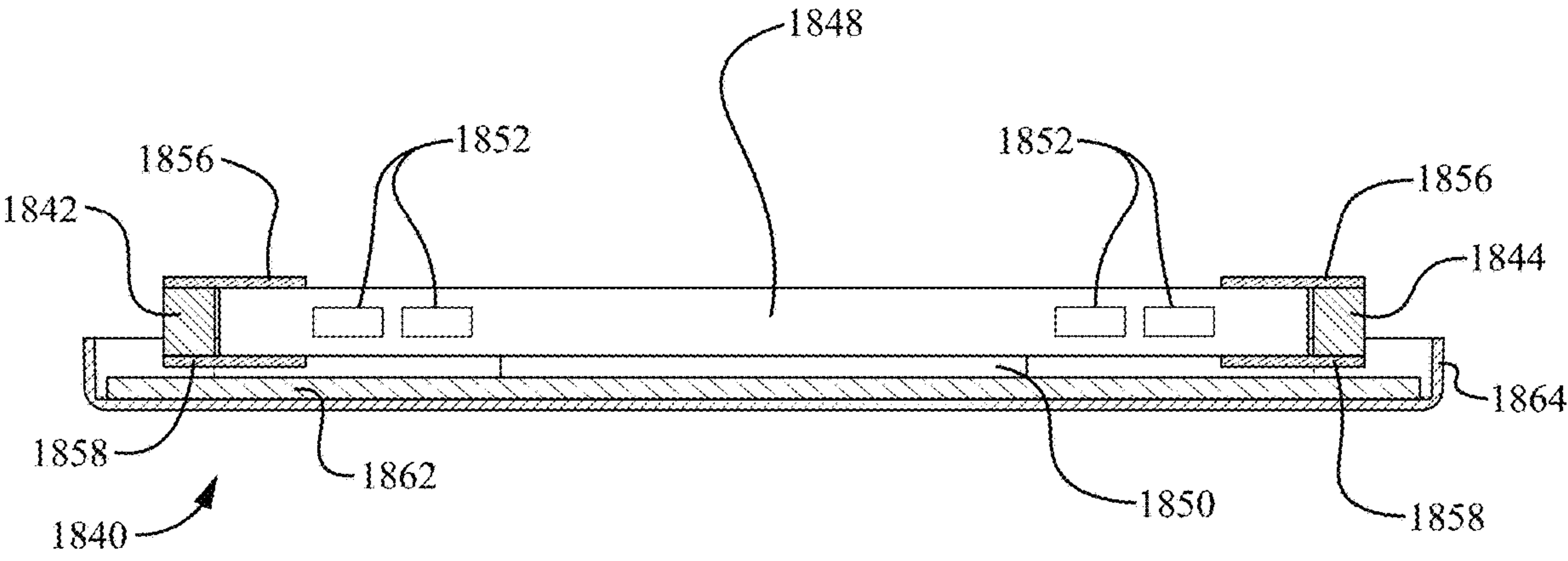
Section E-E FIG. 89
