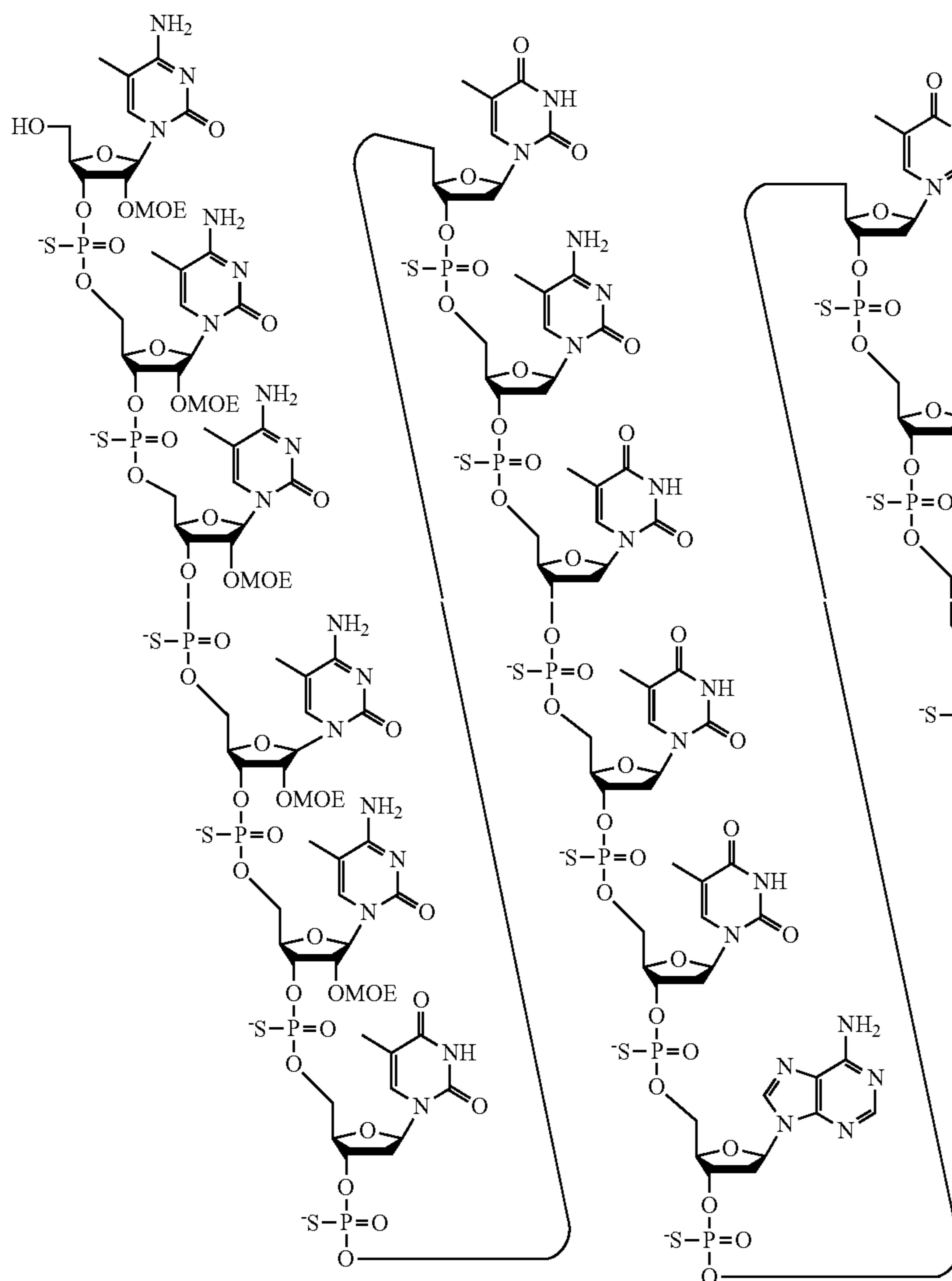
Structure 2. ISIS 546343
