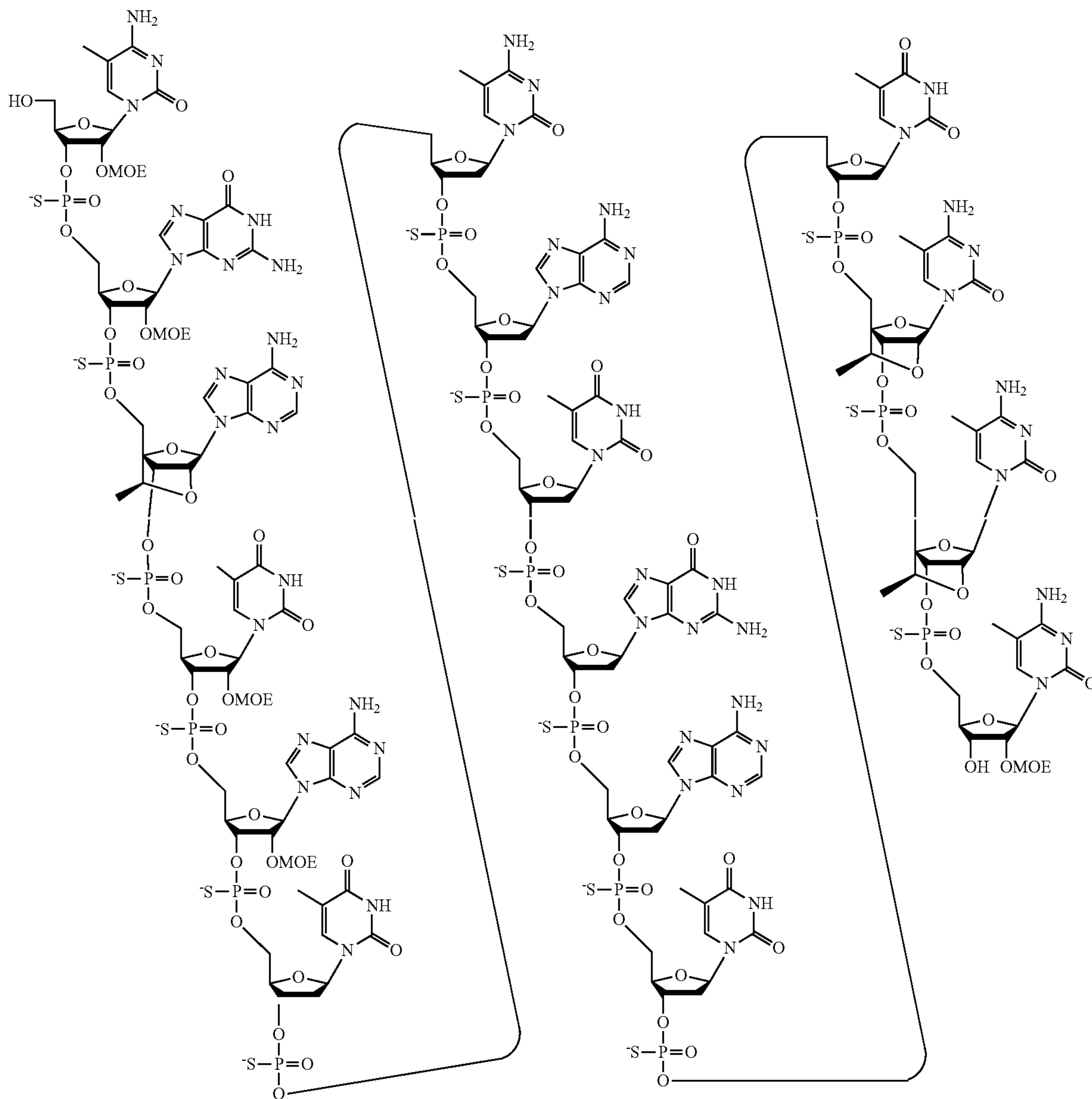
Structure 3. ISIS 548048
