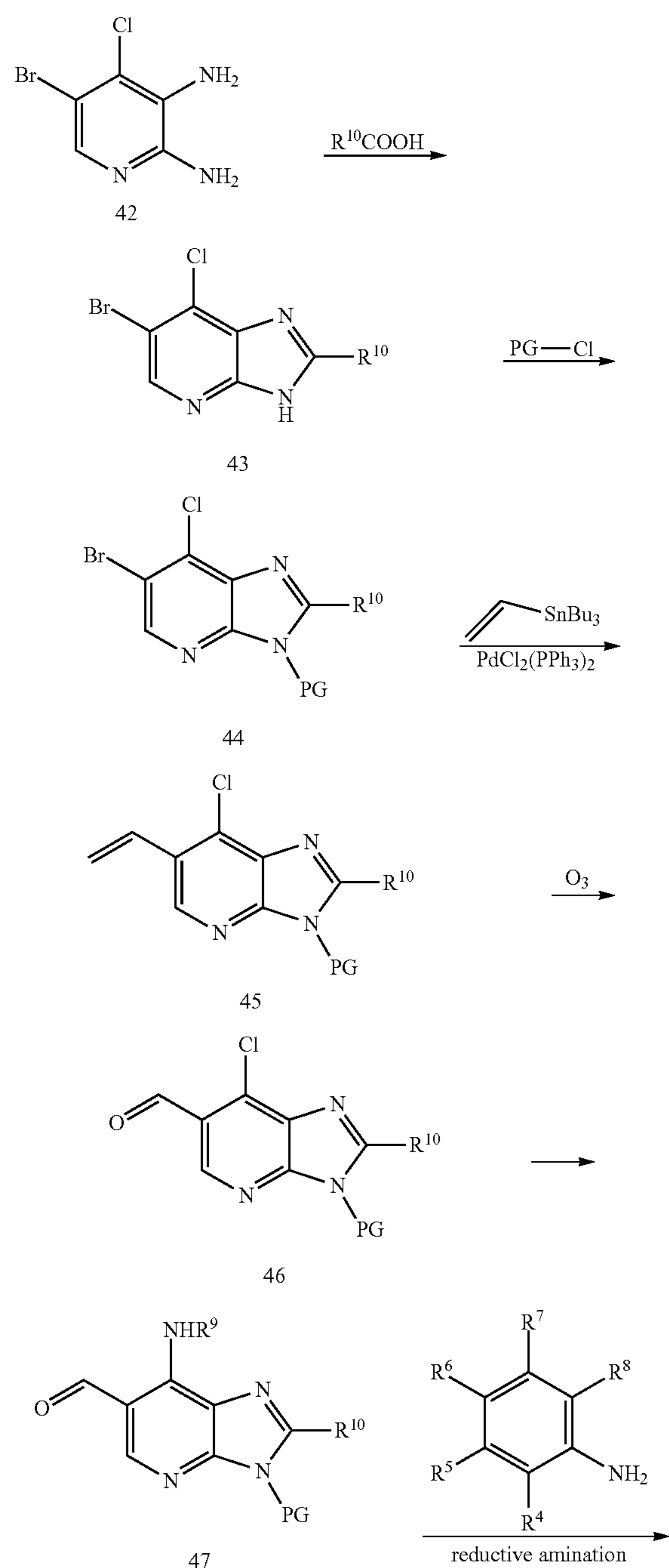
Scheme 11
