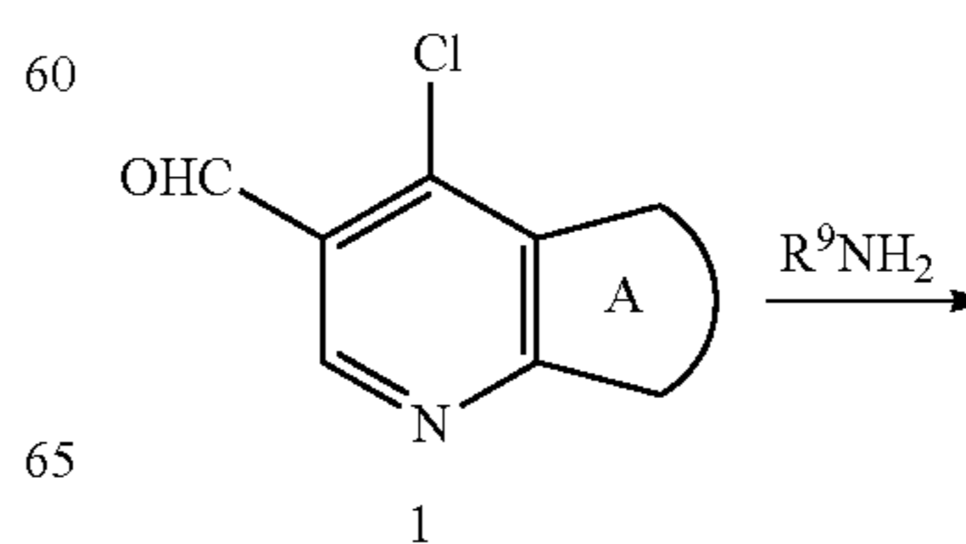
Scheme 1
