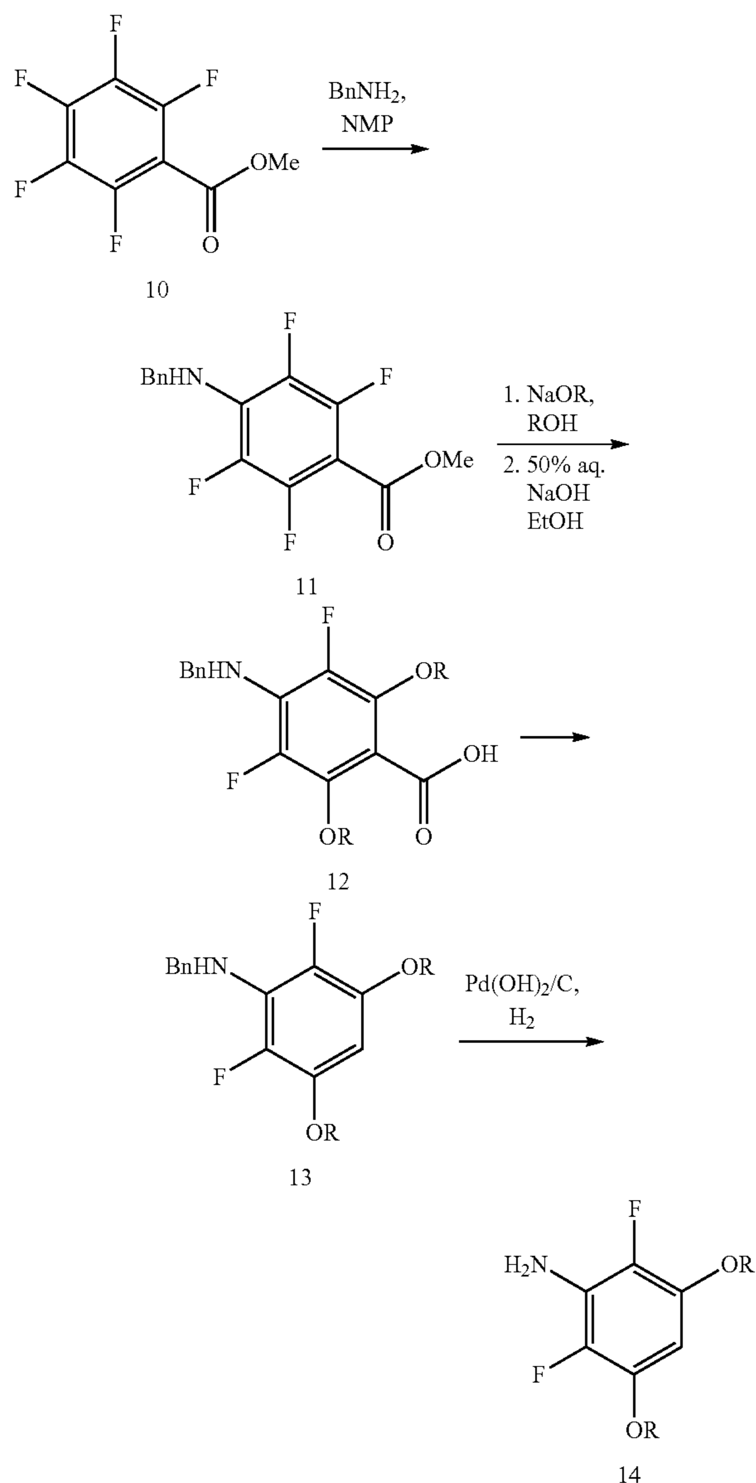
Scheme 3
