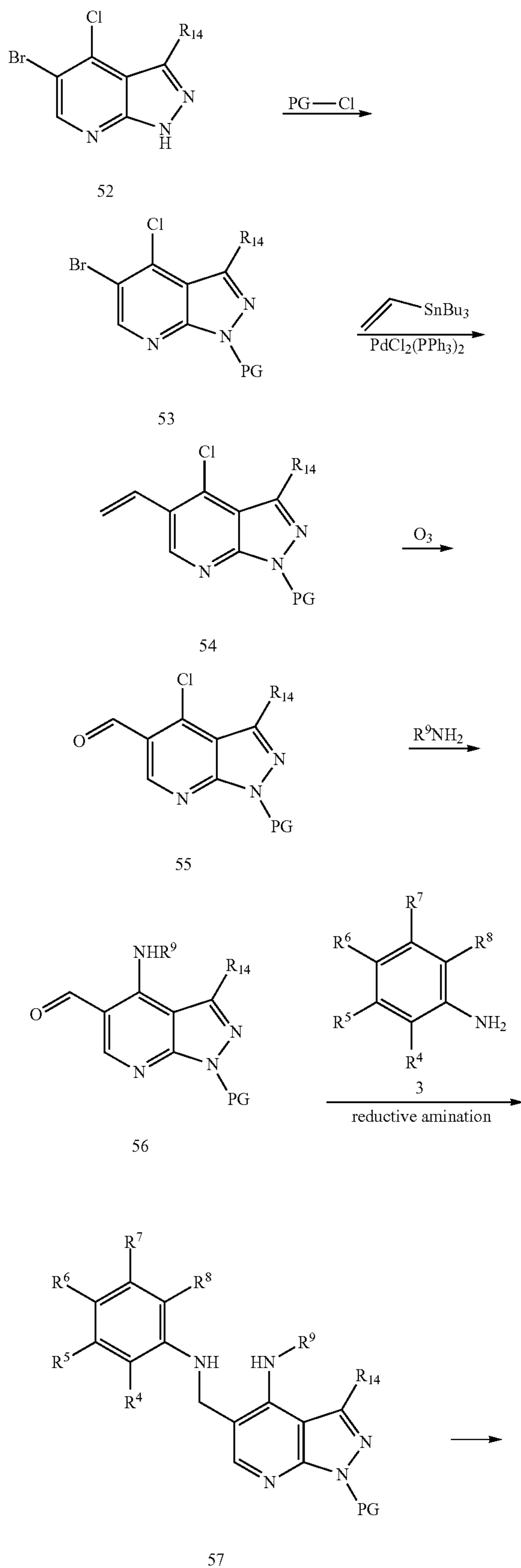
Scheme 12
