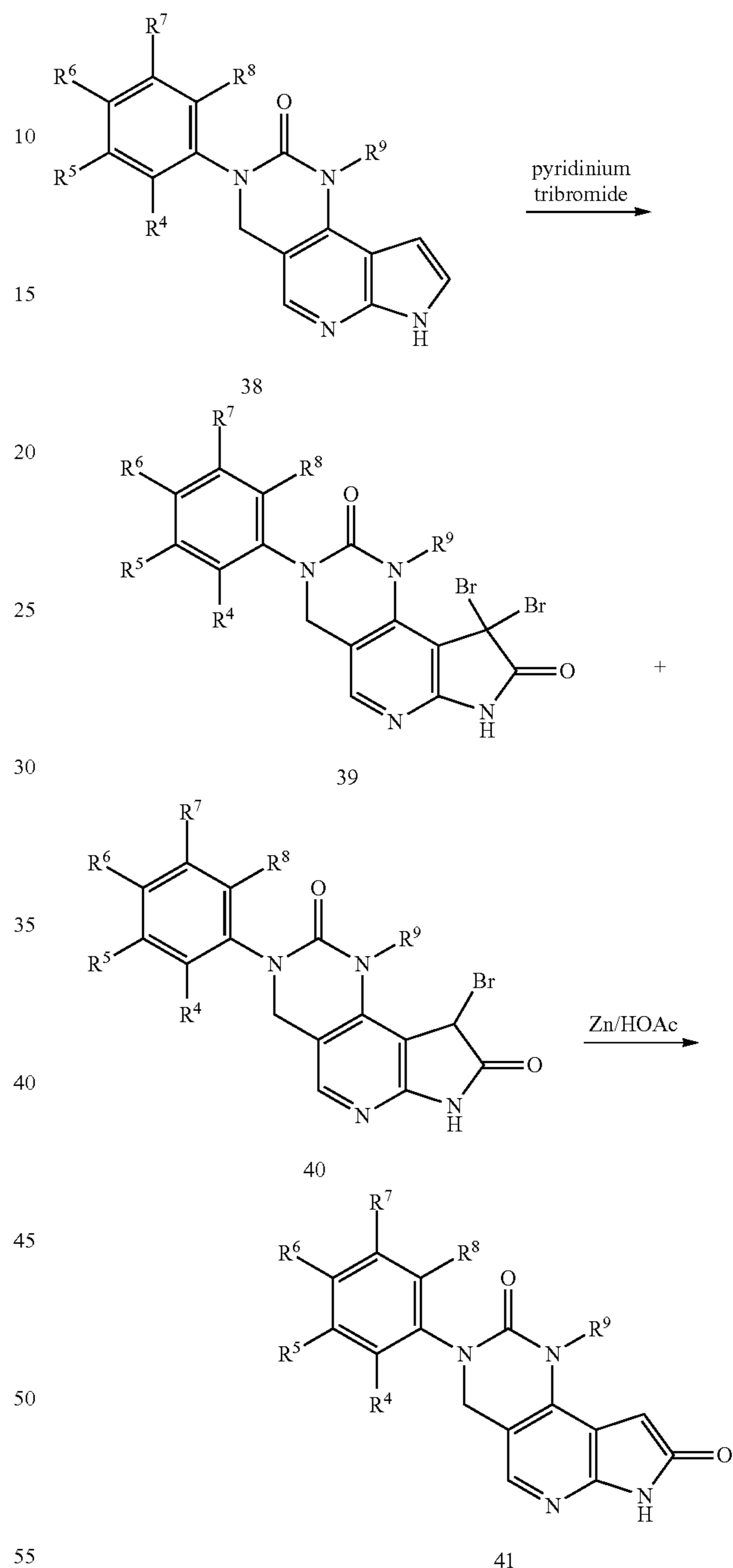
Scheme 10
