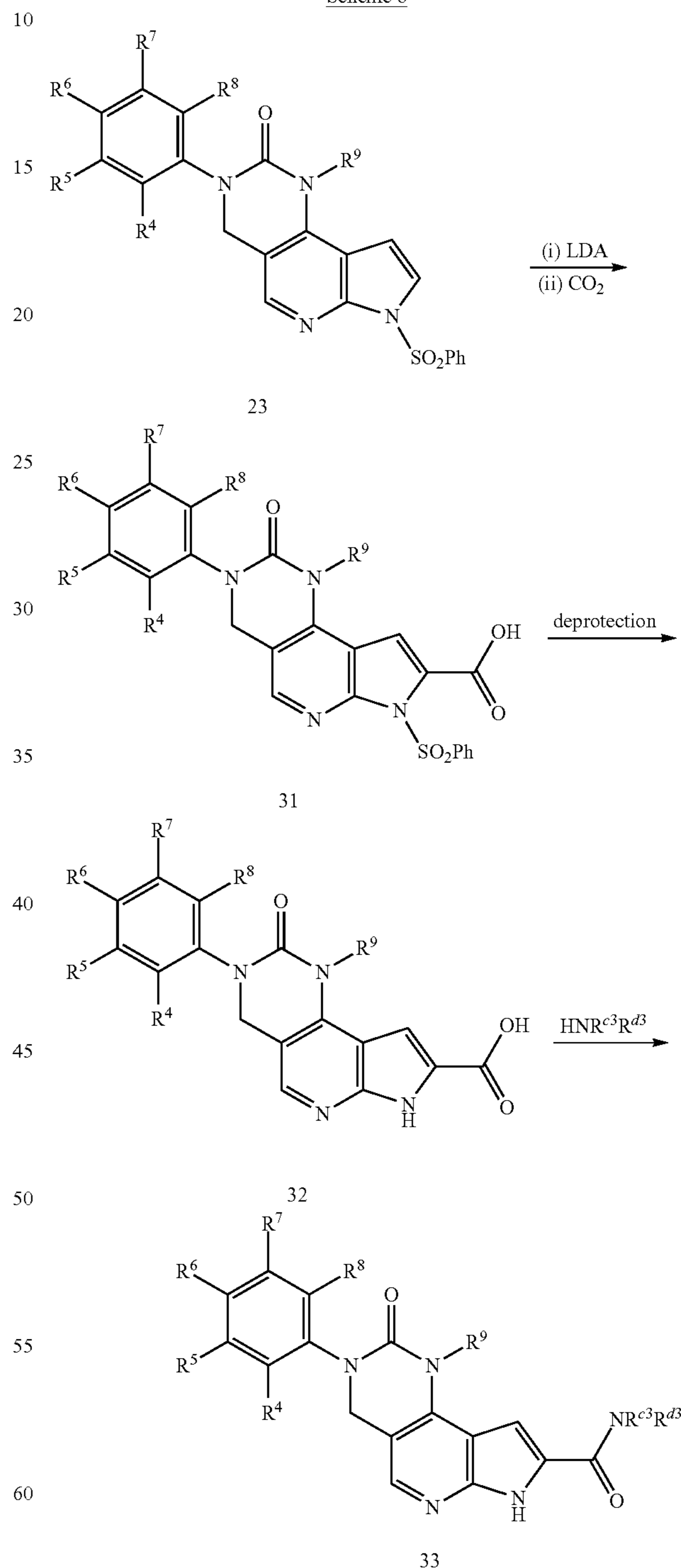
Scheme 8
