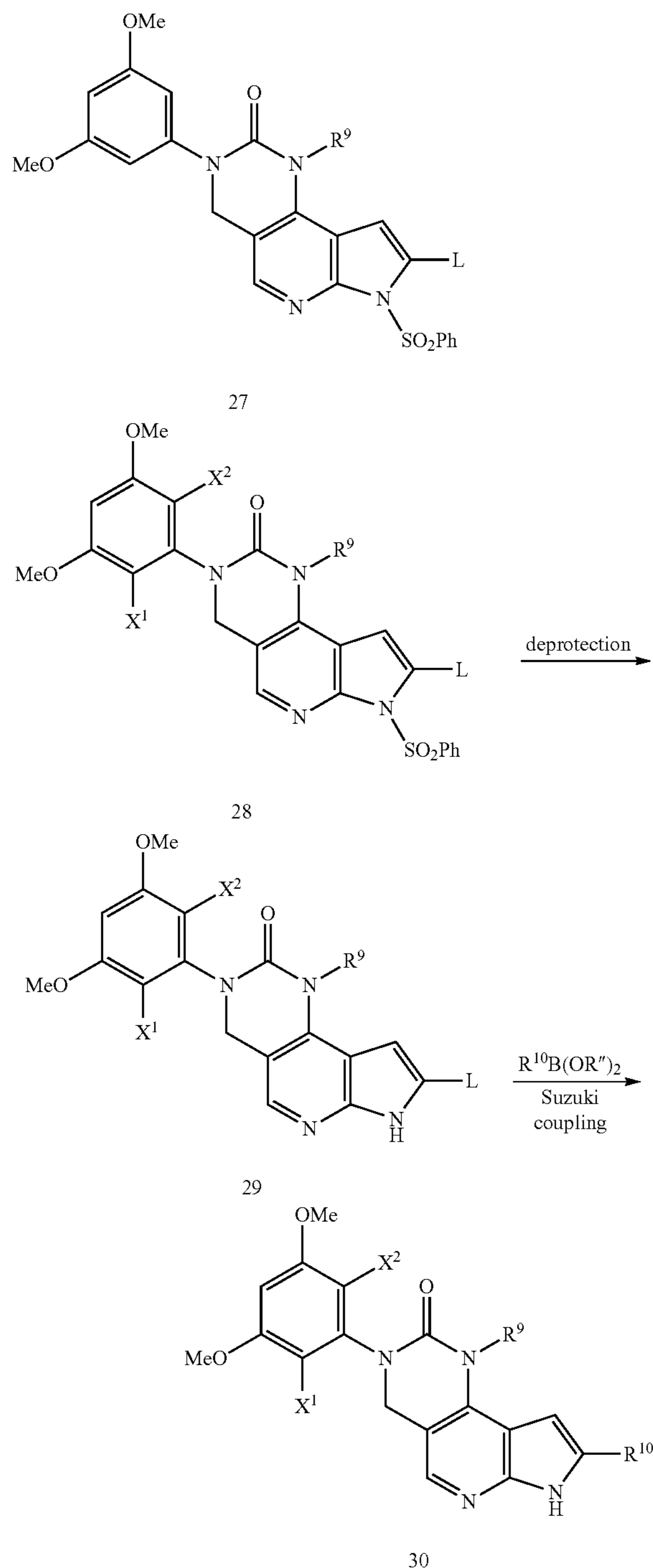
Scheme 7
