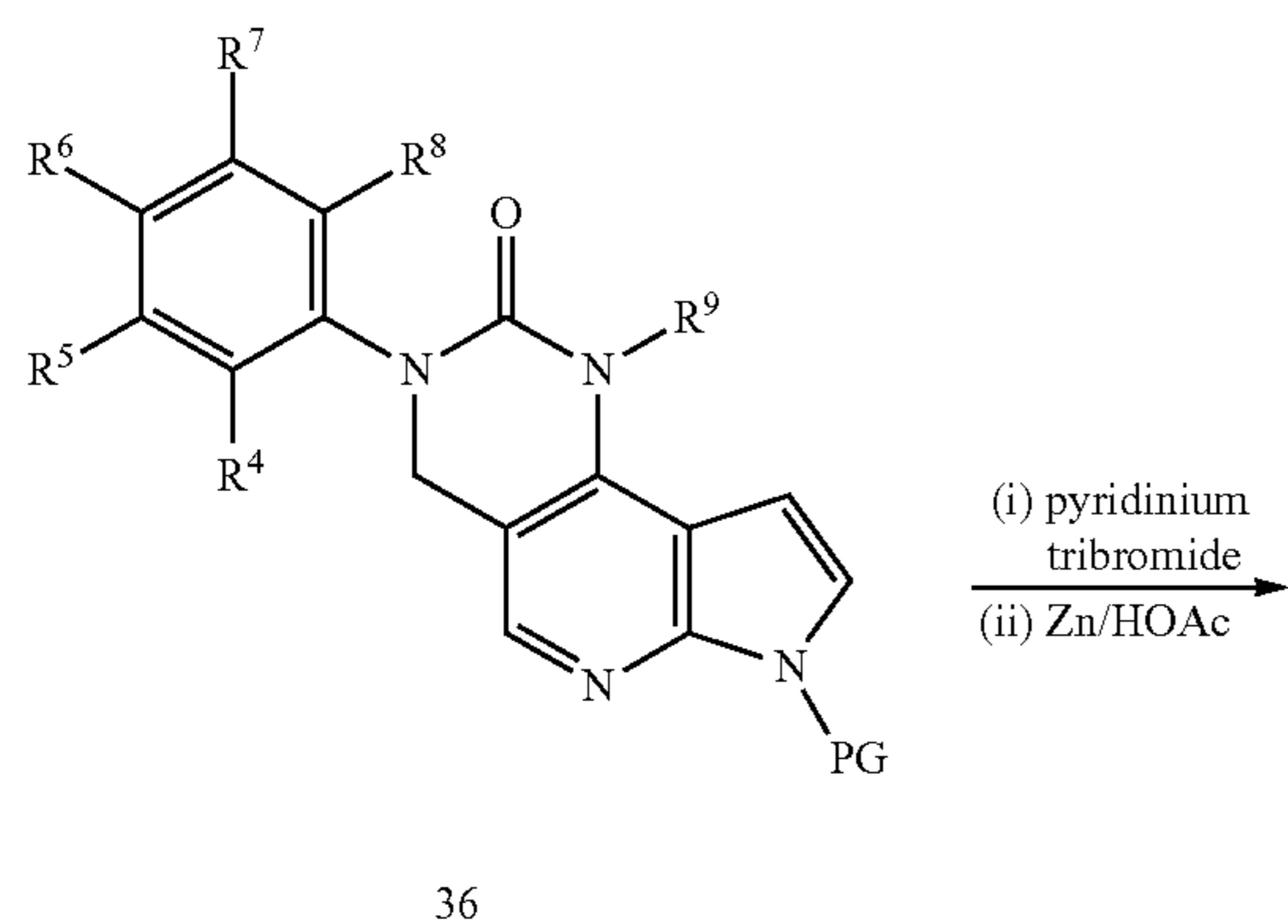
Scheme 14
