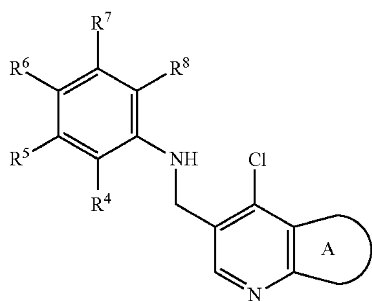
Scheme 16
