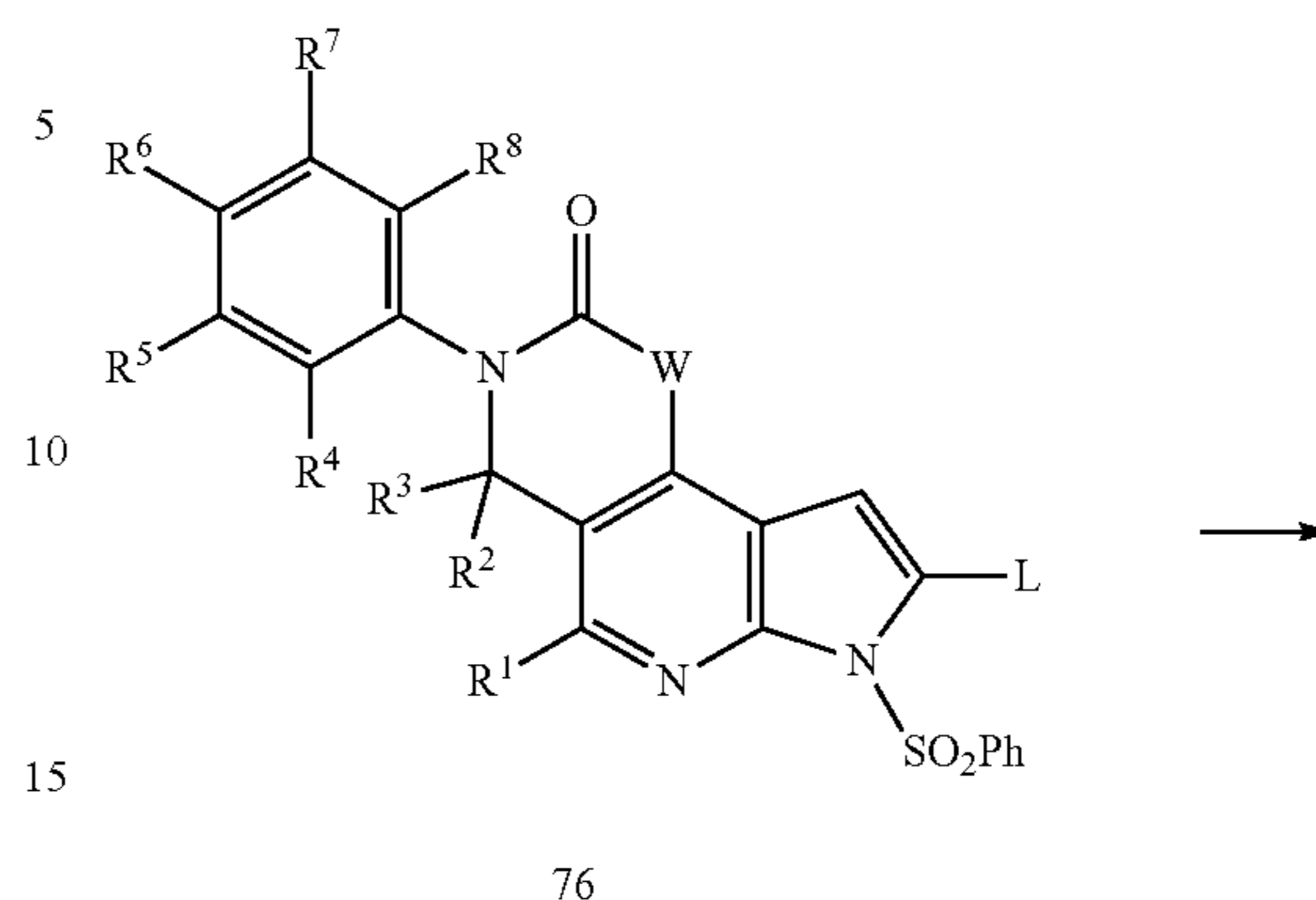
Scheme 20
