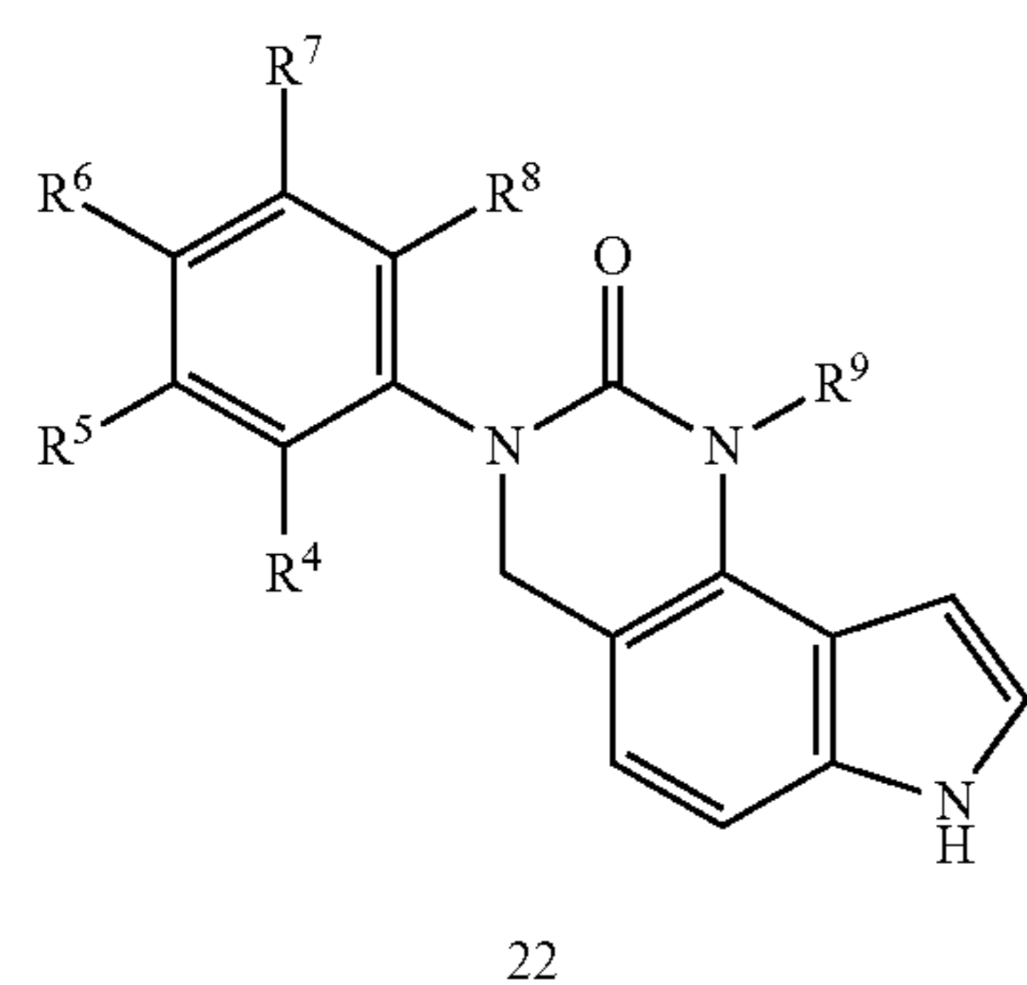
Scheme 6
