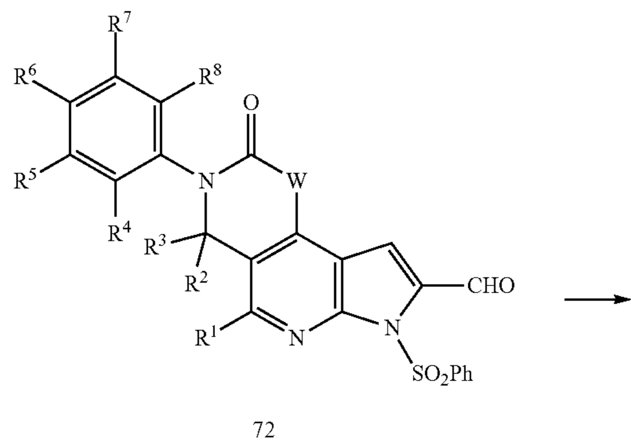
Scheme 19
