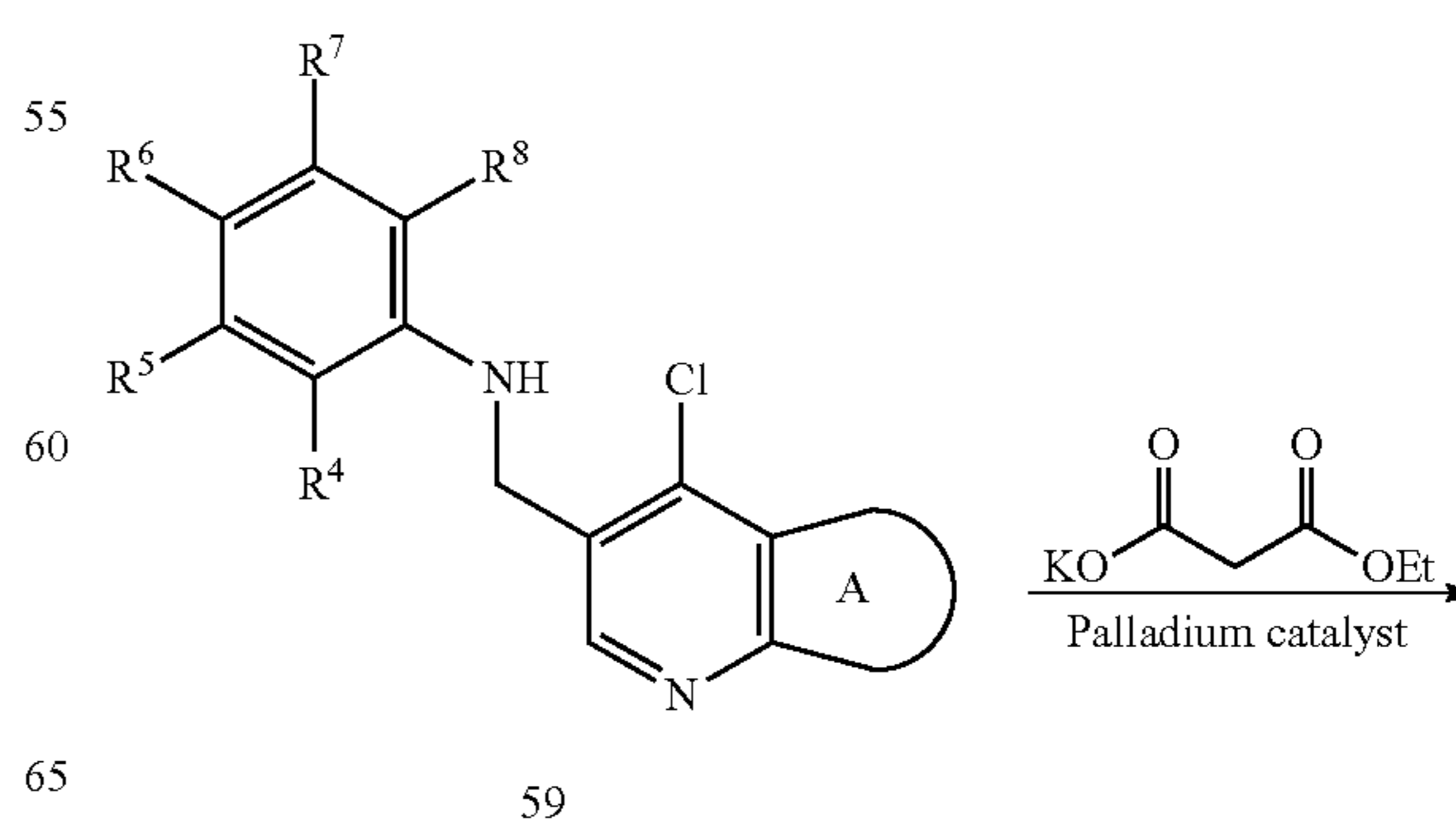
Scheme 15
