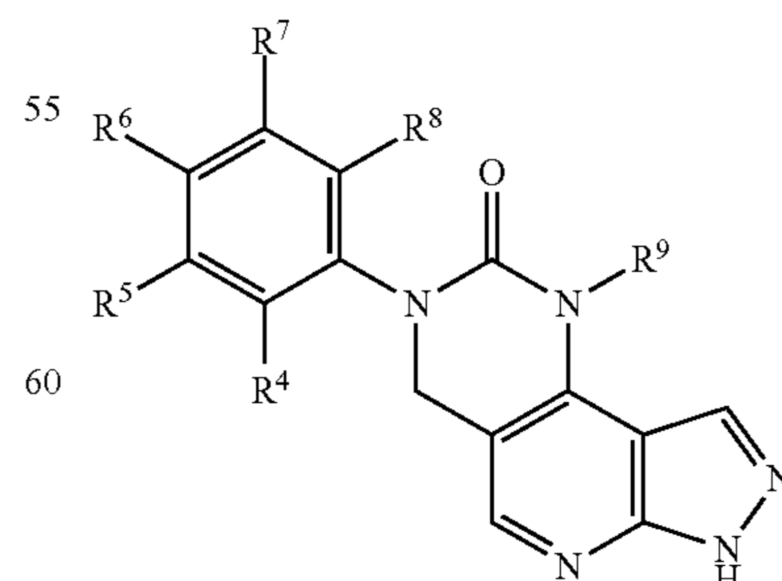
Scheme 17
