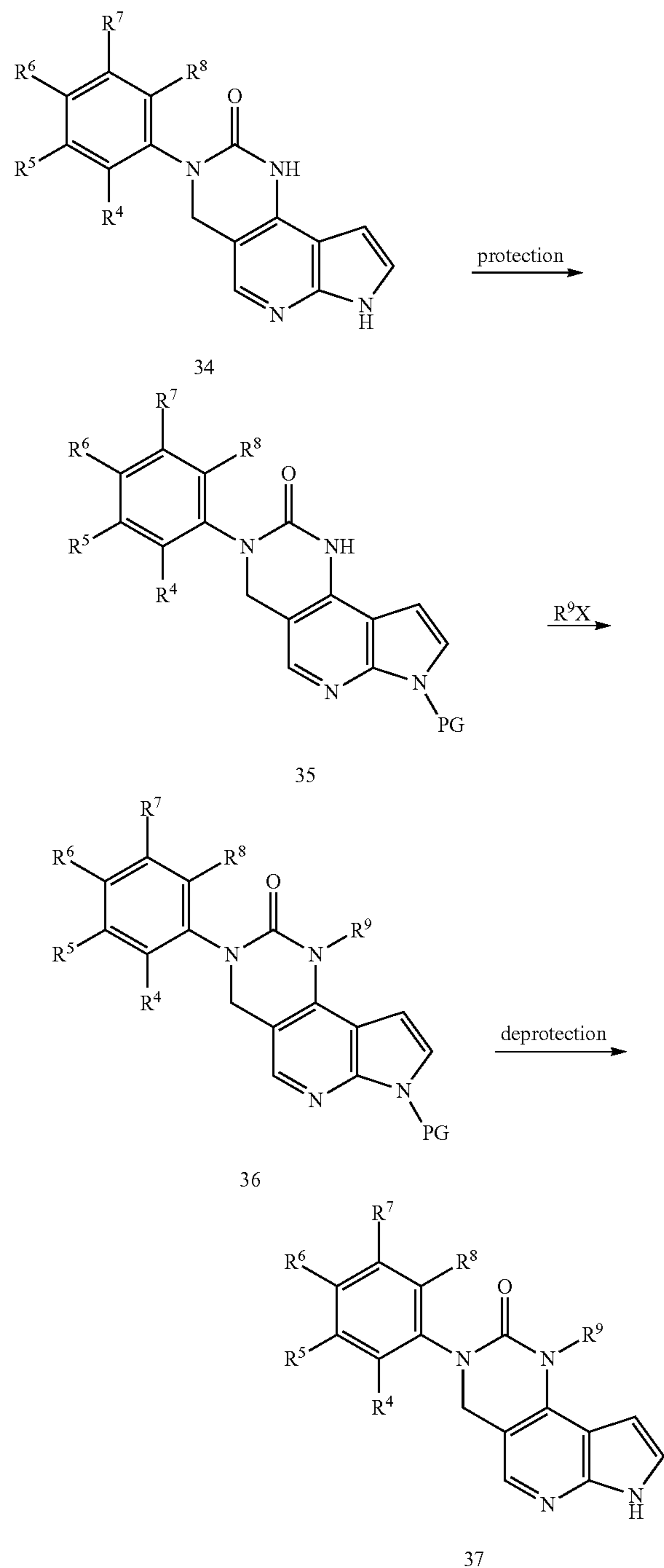
Scheme 9
