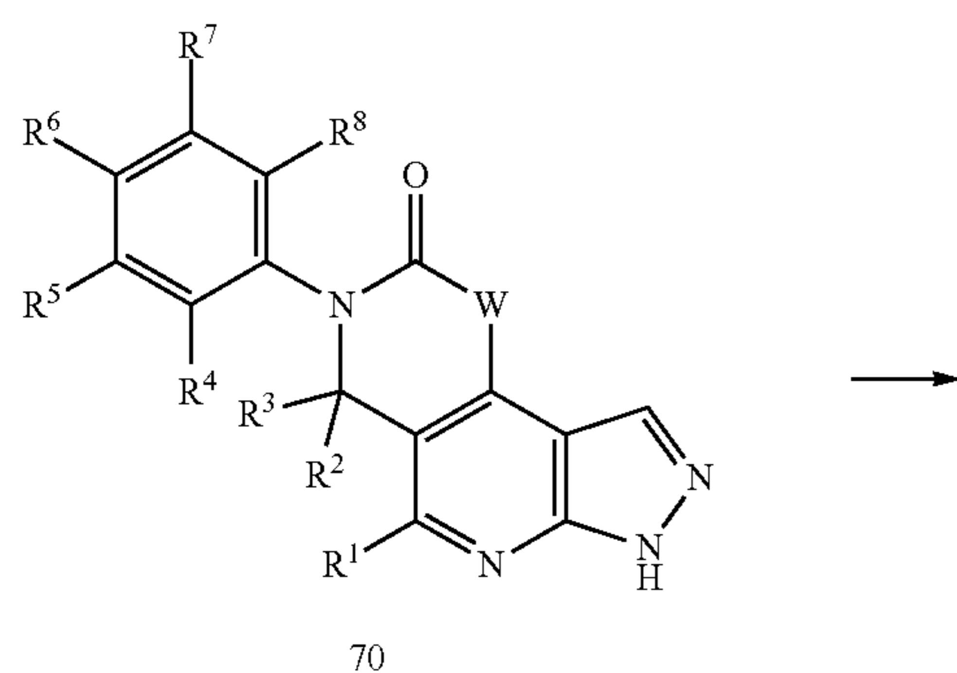
Scheme 18
