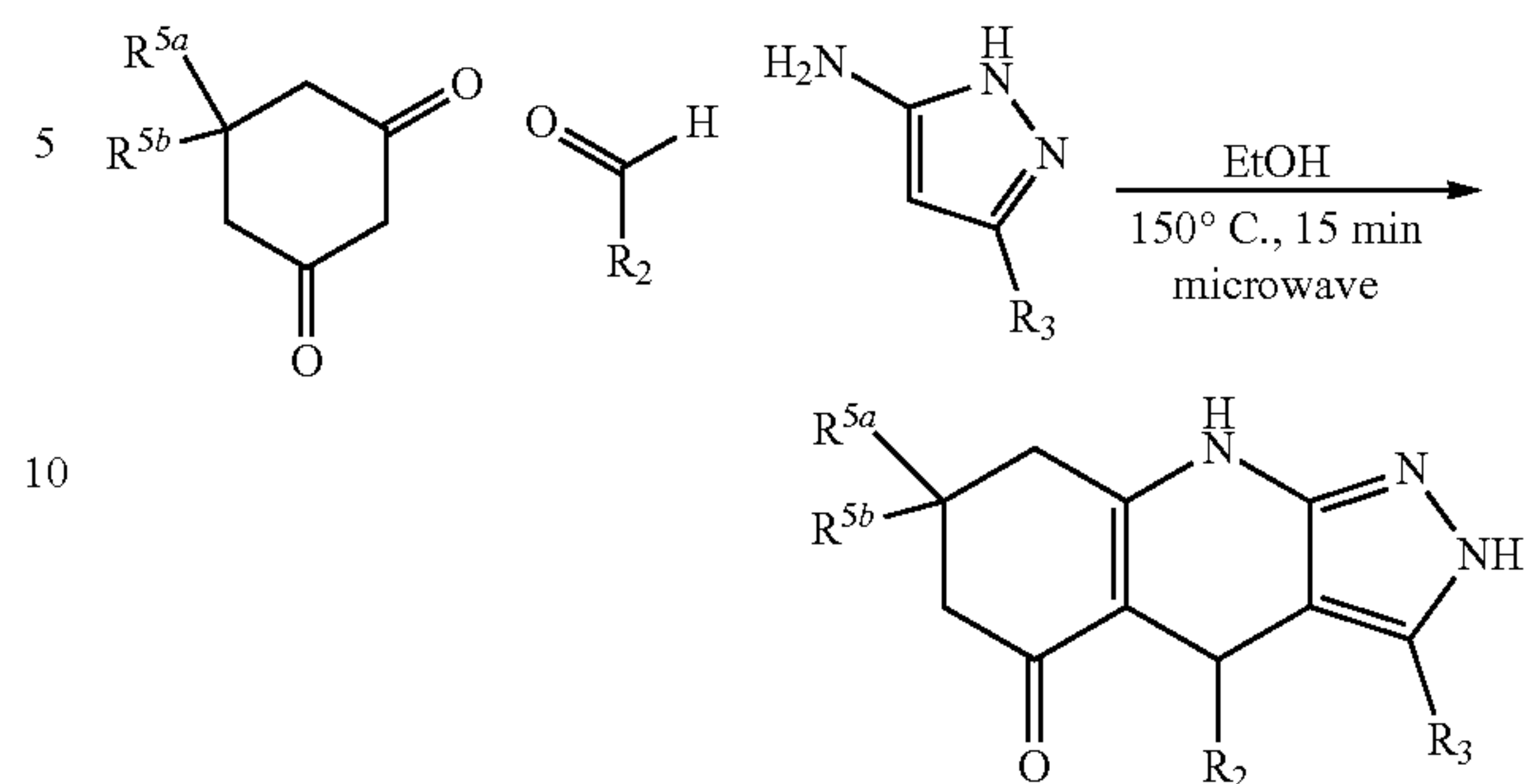
Scheme 1a. Synthesis of Protocol A
