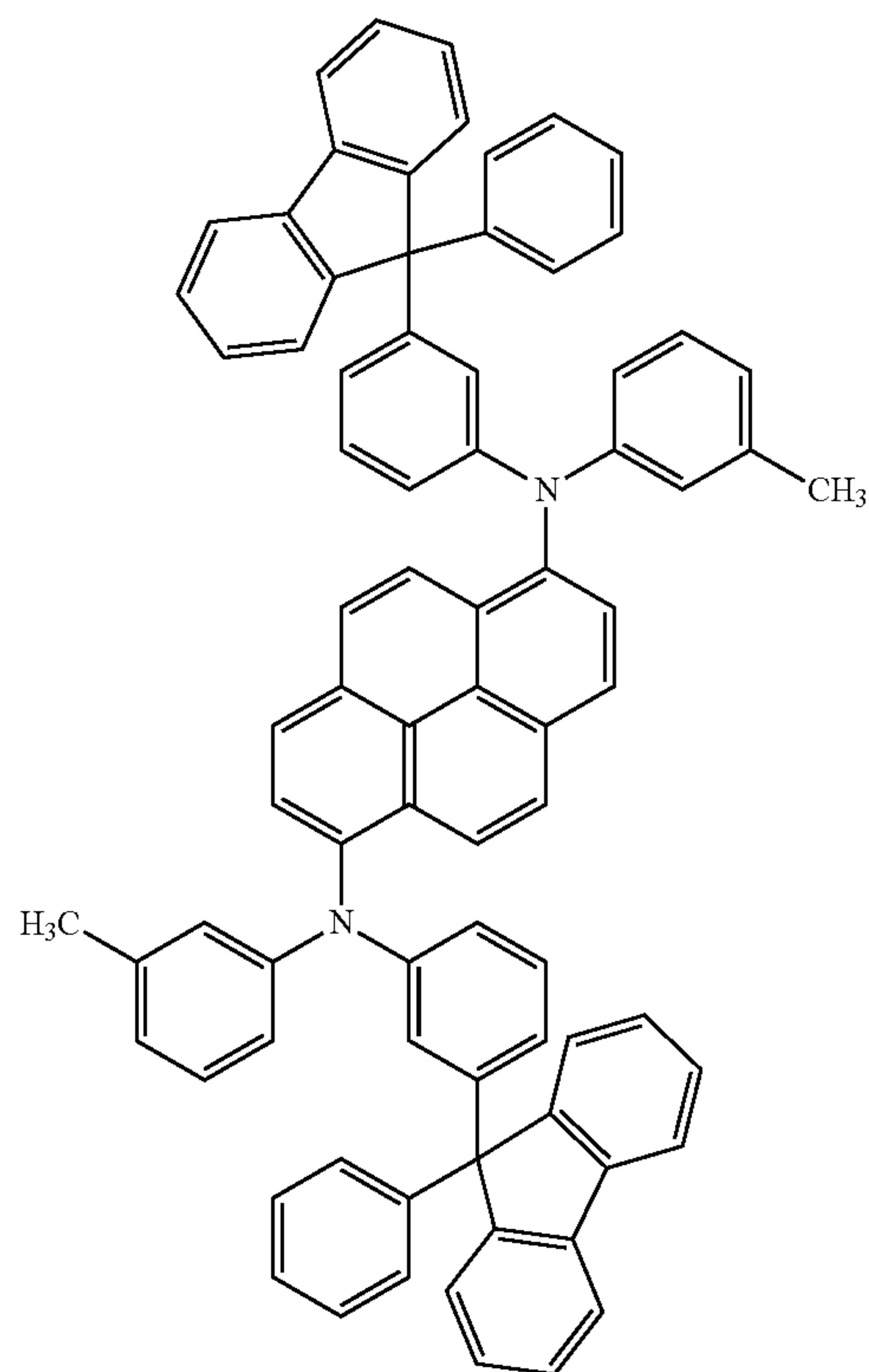
1,6mMemFLAPrn
