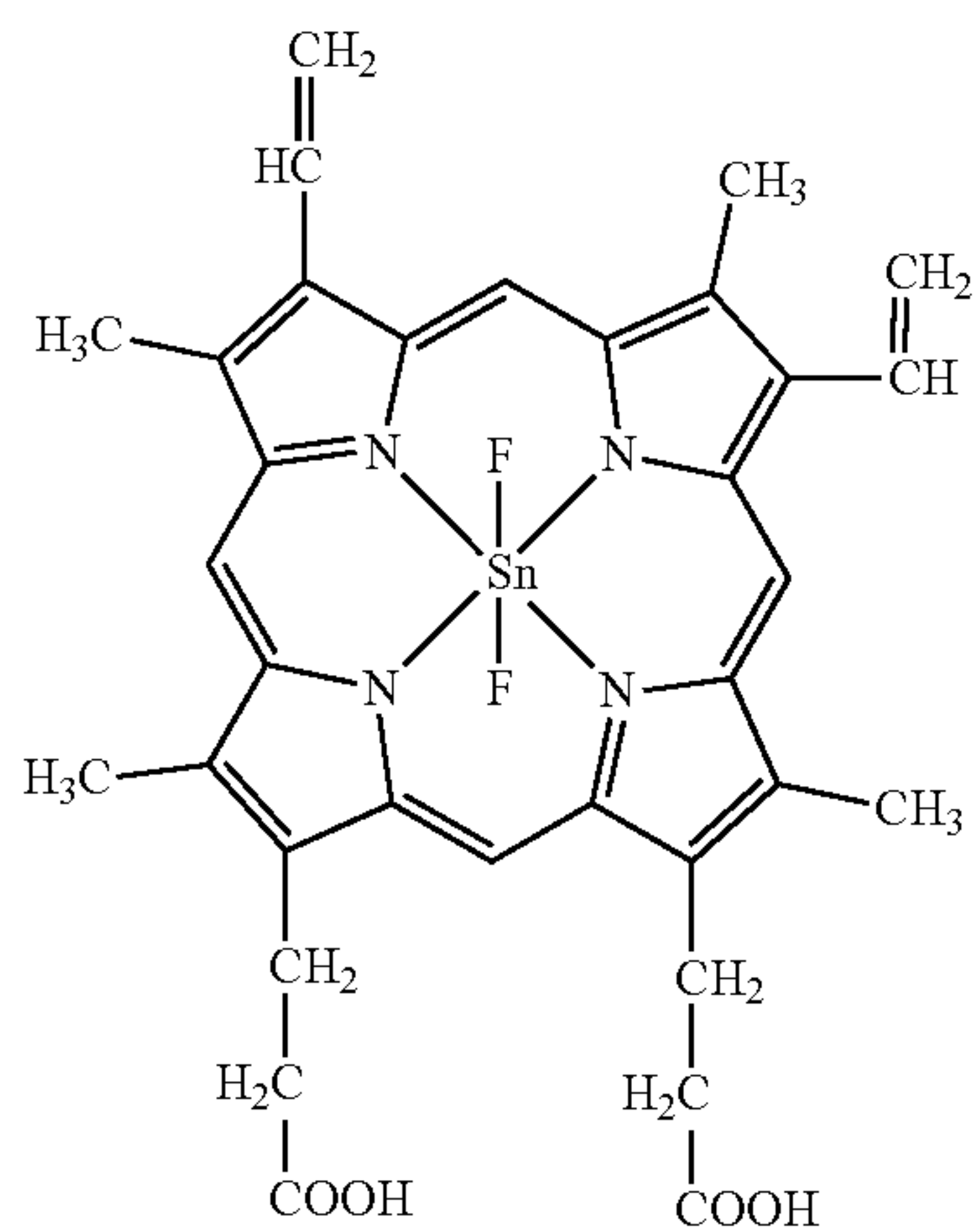
\text{SnF}_2(\text{Proto IX})
