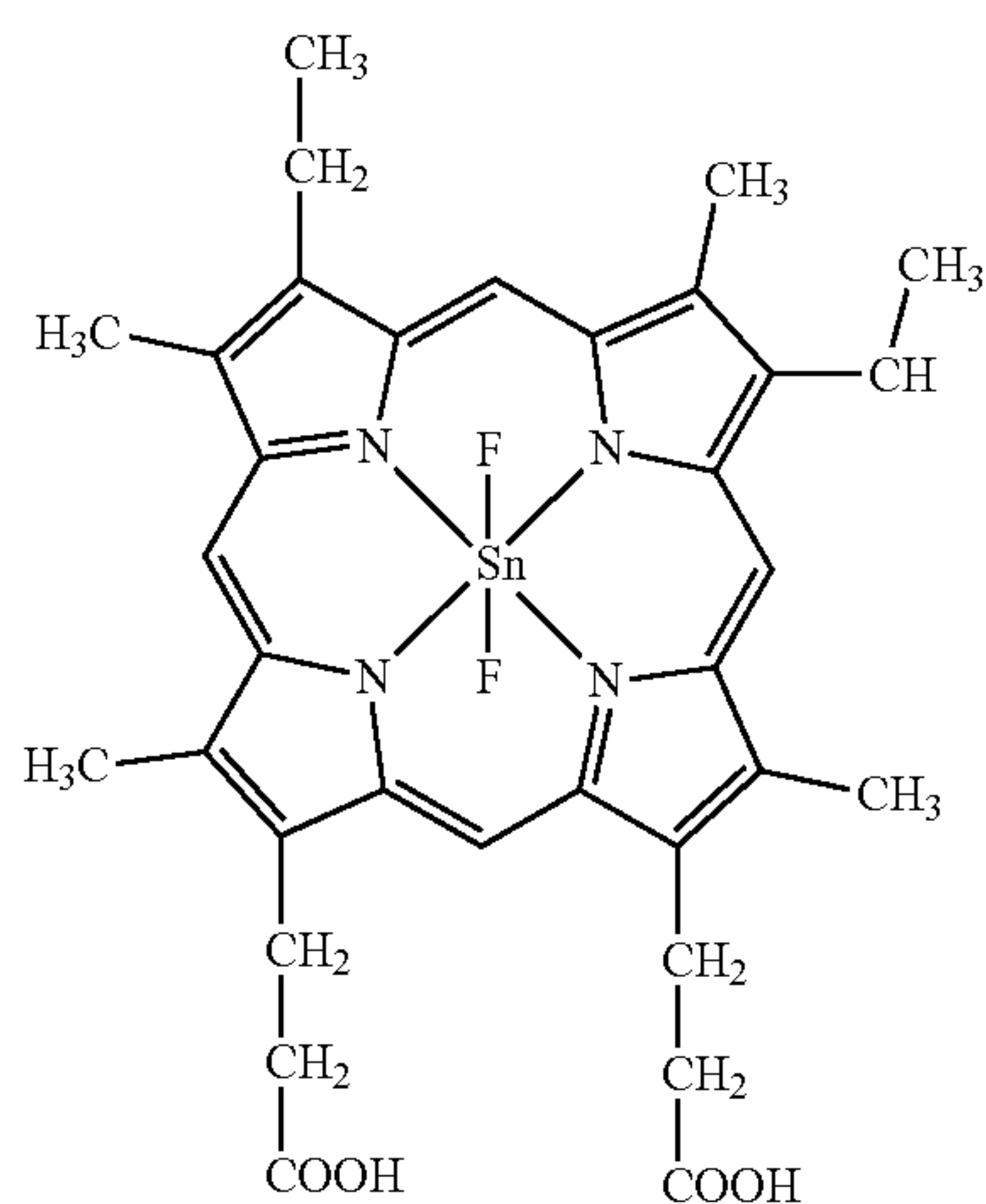
\text{SnF}_2(\text{Meso IX})
