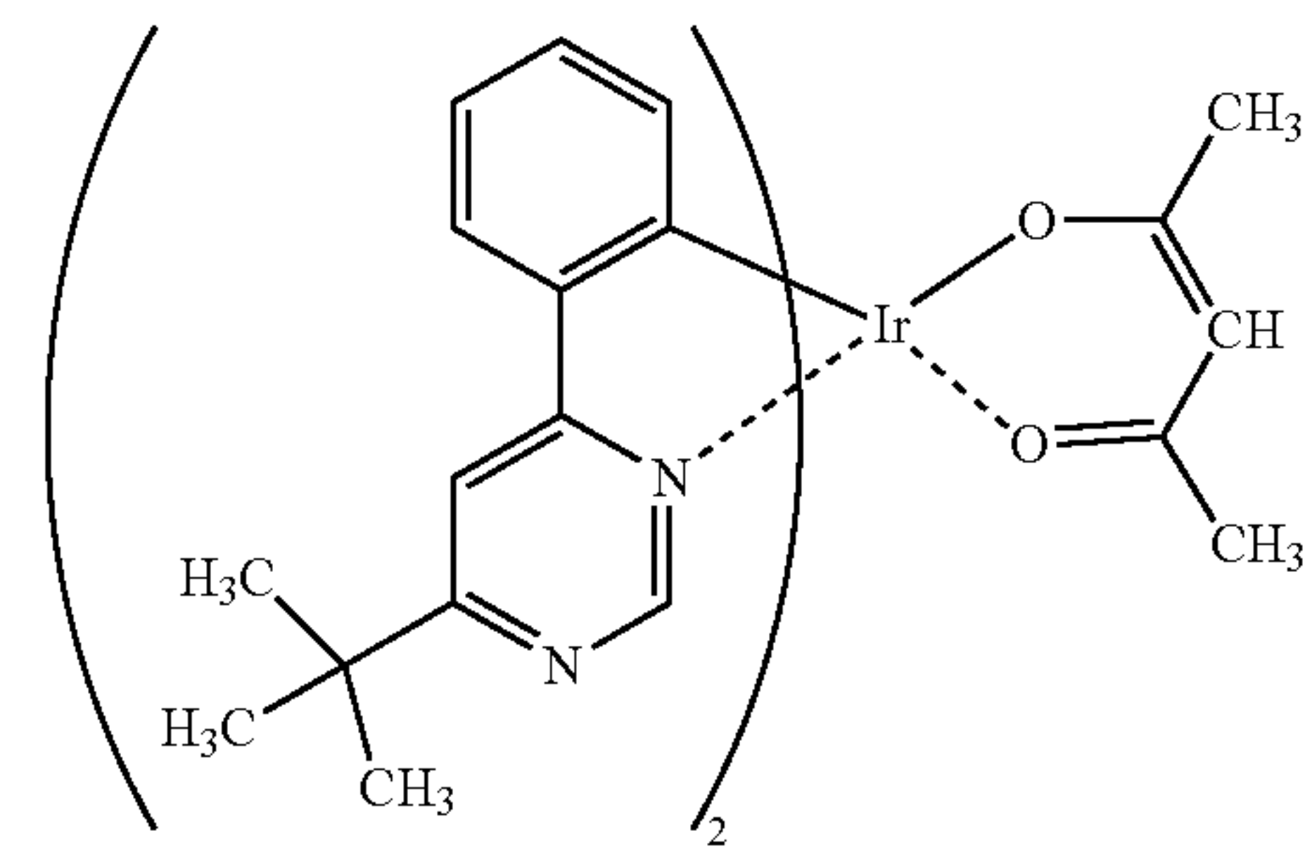
[Ir(tBuppm) 2 (acac)]
