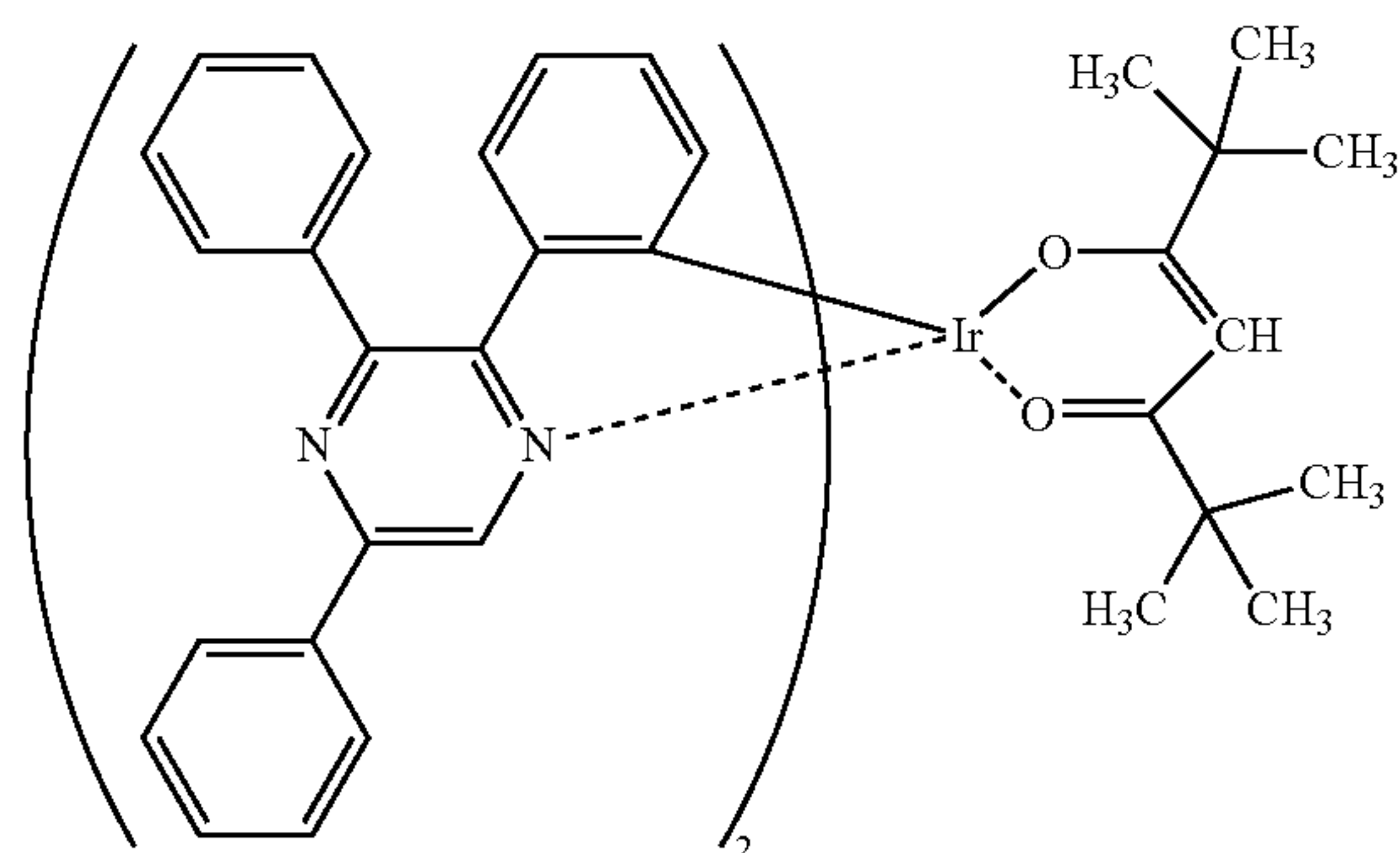
[Ir(tppr) 2 (dpm)]
