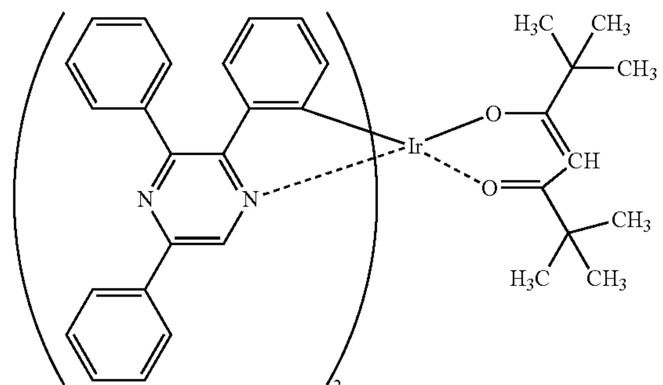
[Ir(tppr) 2 (dpm)]
