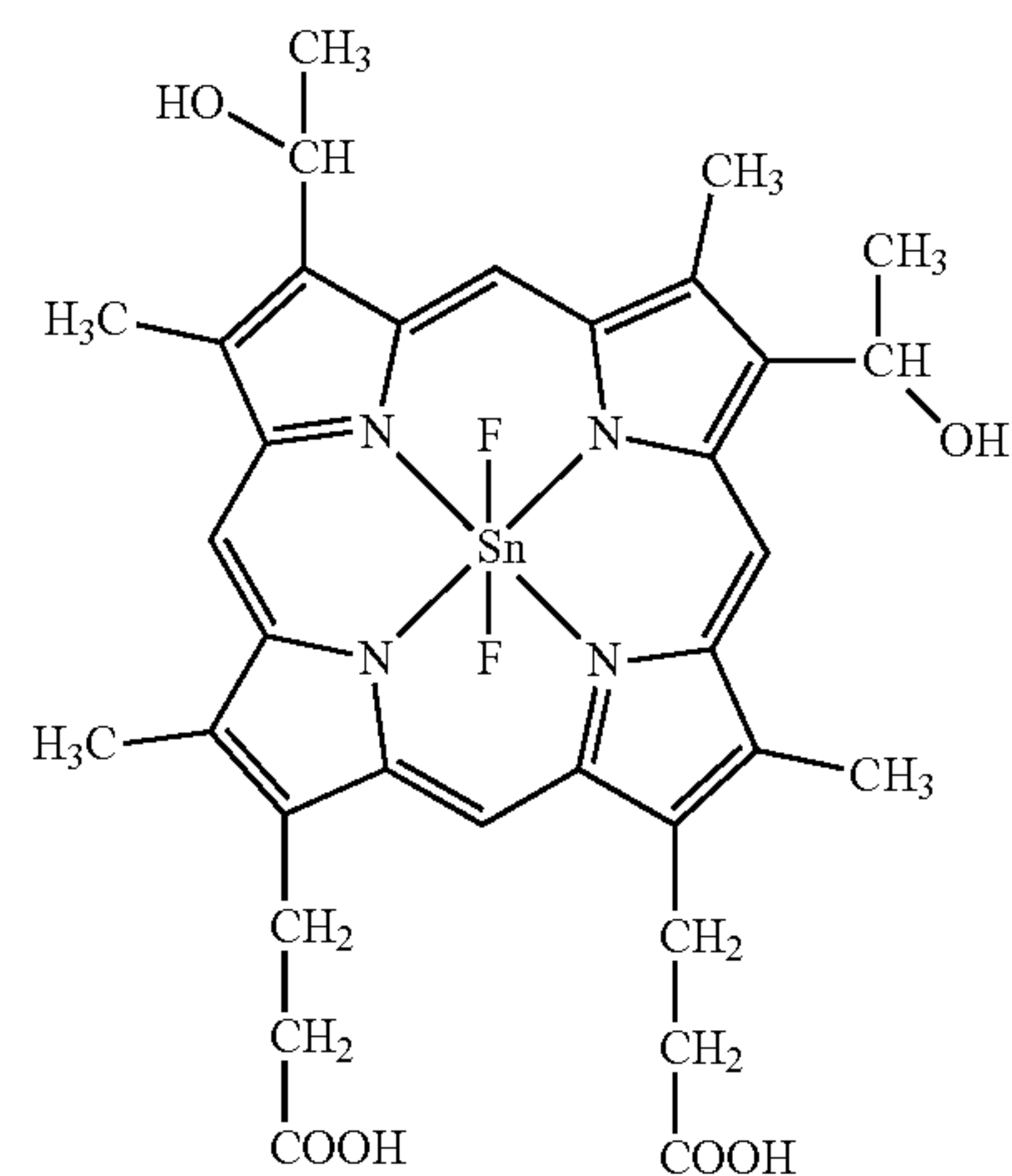
\text{SnF}_2(\text{Hemato IX})
