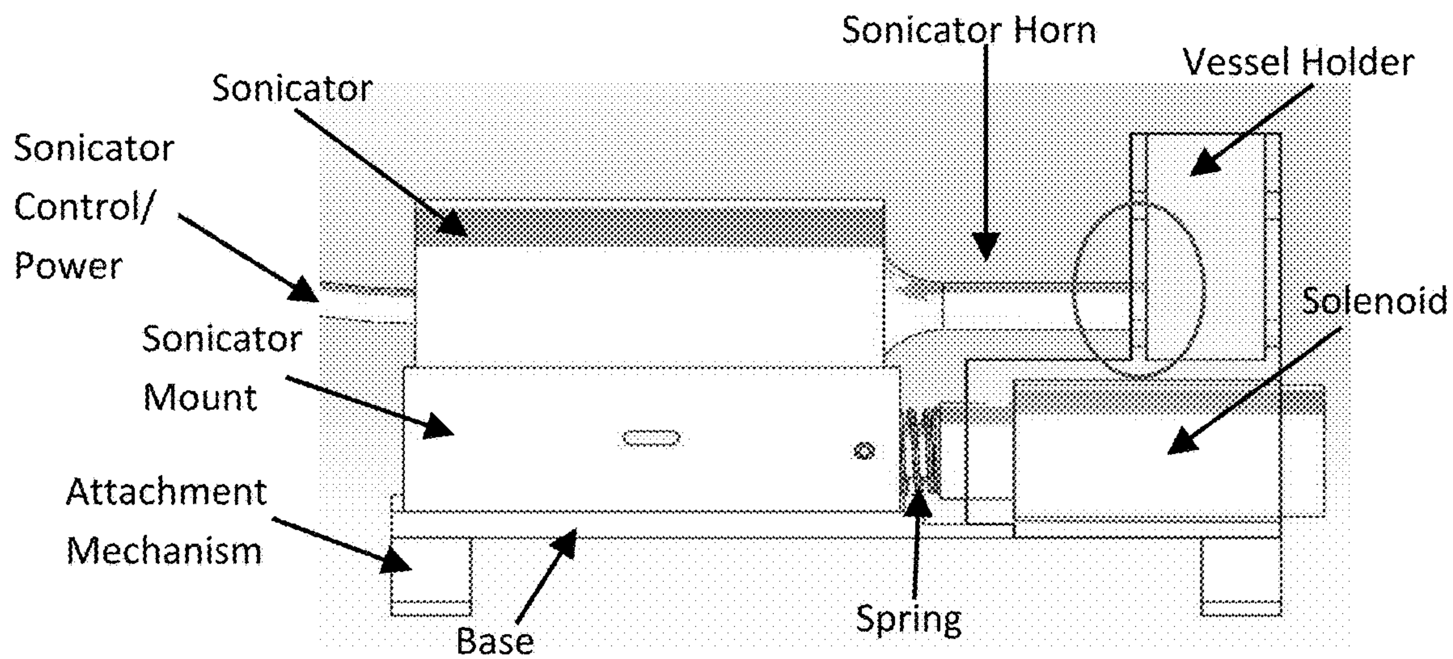
Solenoid On
