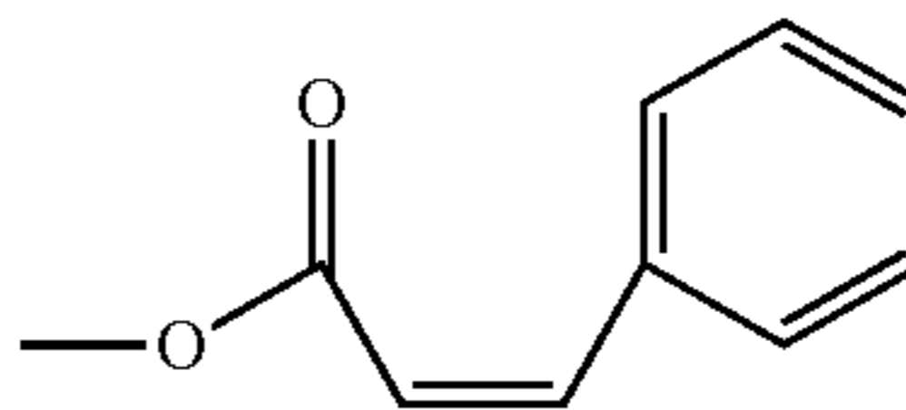
(Z)—O(C=O)CH=CH—C 6 H 5 is an example of [O-C3 alkenoyl substituted with phenyl]
