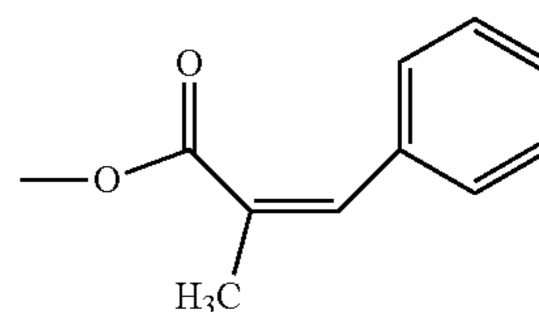
(Z)—O(C=O)C(CH 3 )=CH—C 6 H 5 is an example of [O-C4 alkenoyl substituted with phenyl]
