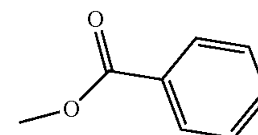
O(C=O)C 6 H 5 , Benzoyl is an example of [O-C1 alkanoyl substituted with phenyl]
