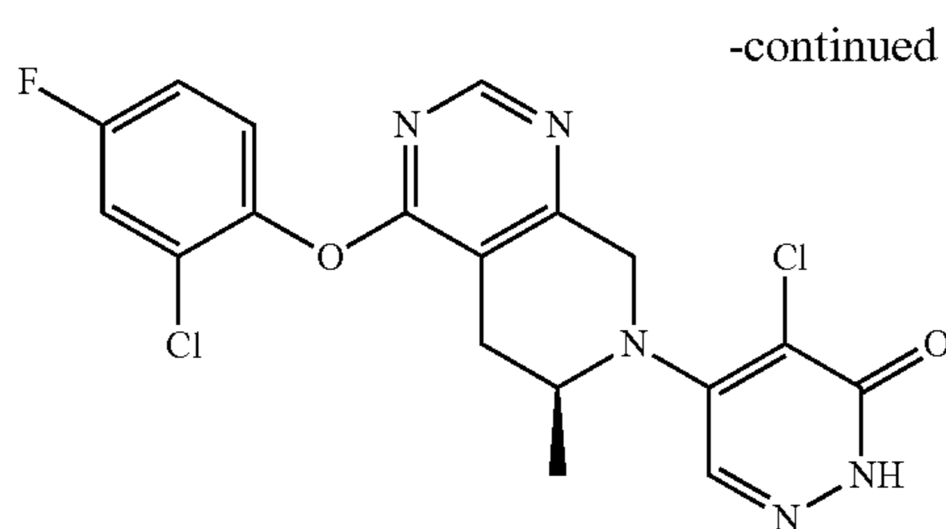
Compound 117a
