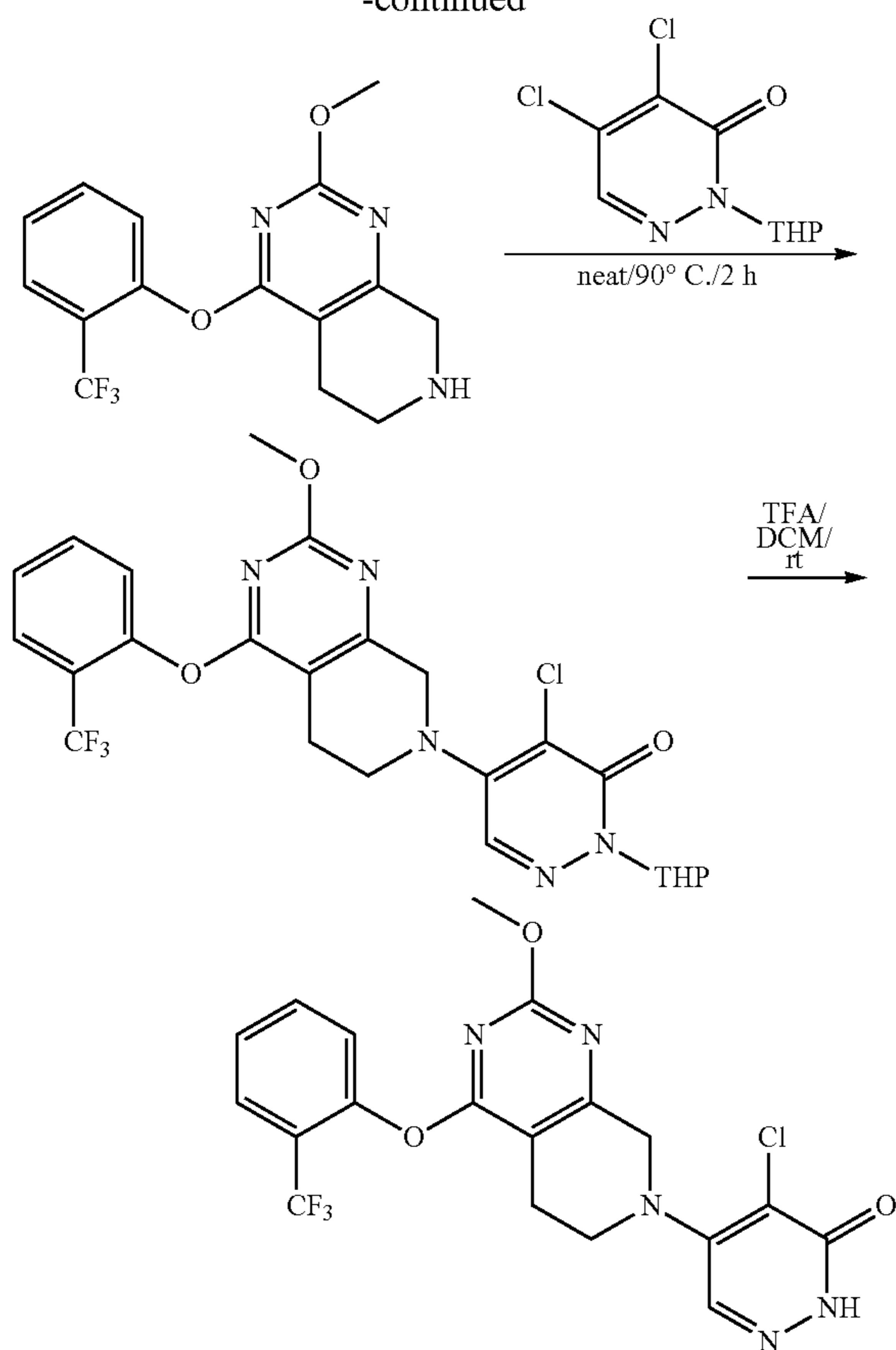
Compound 110
