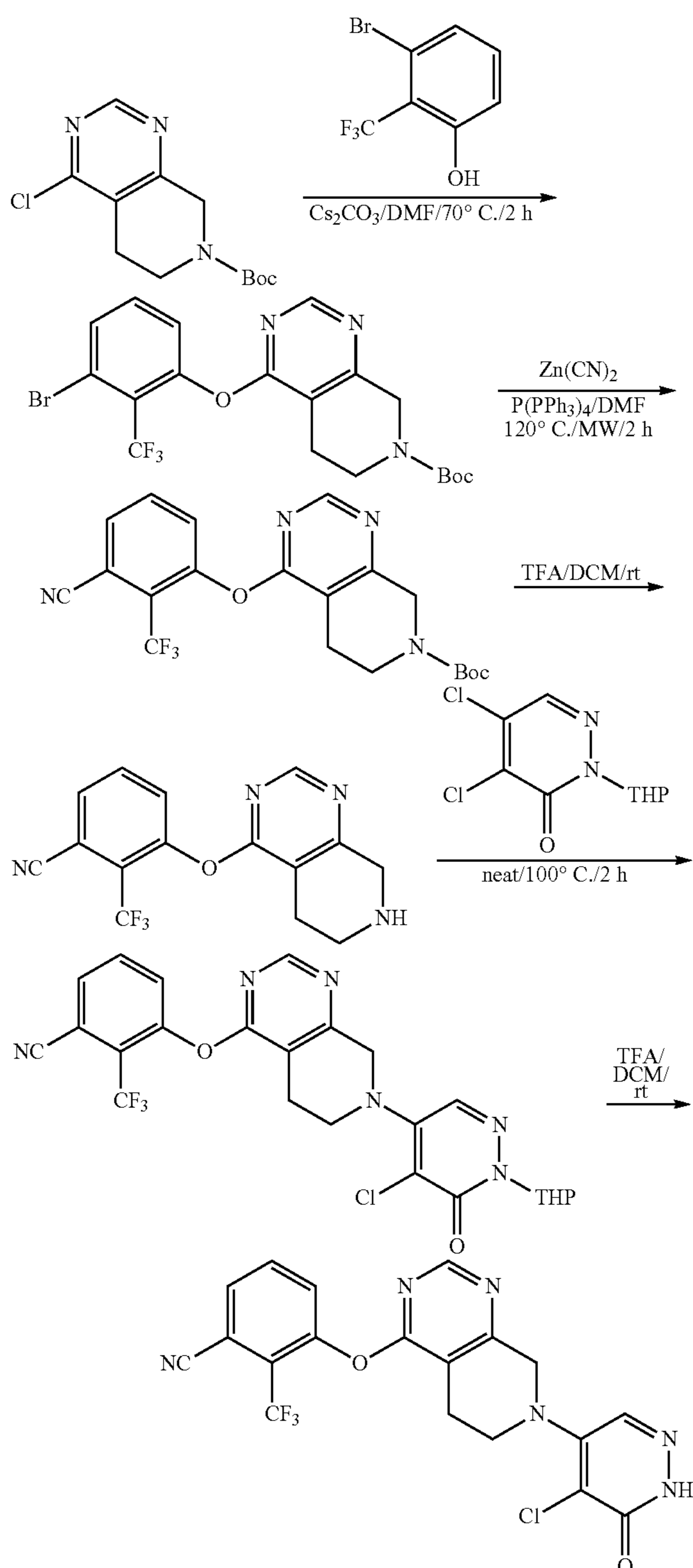
Compound 111
