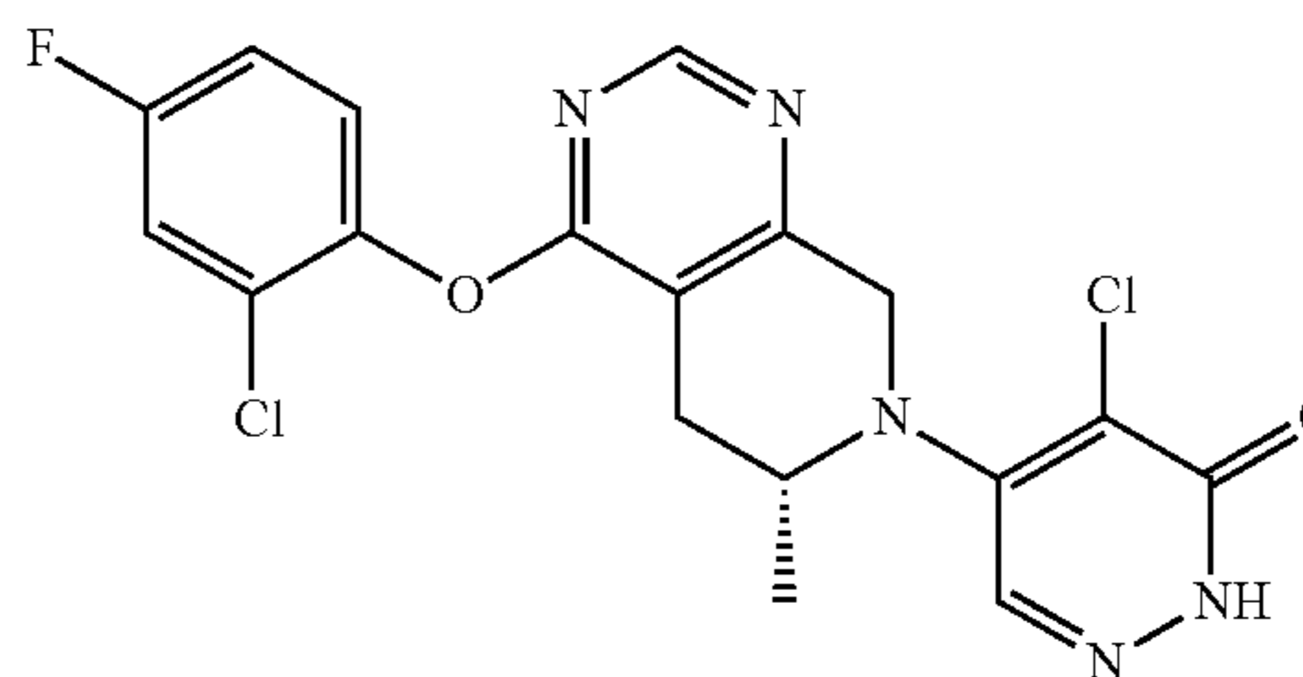
Compound 117
