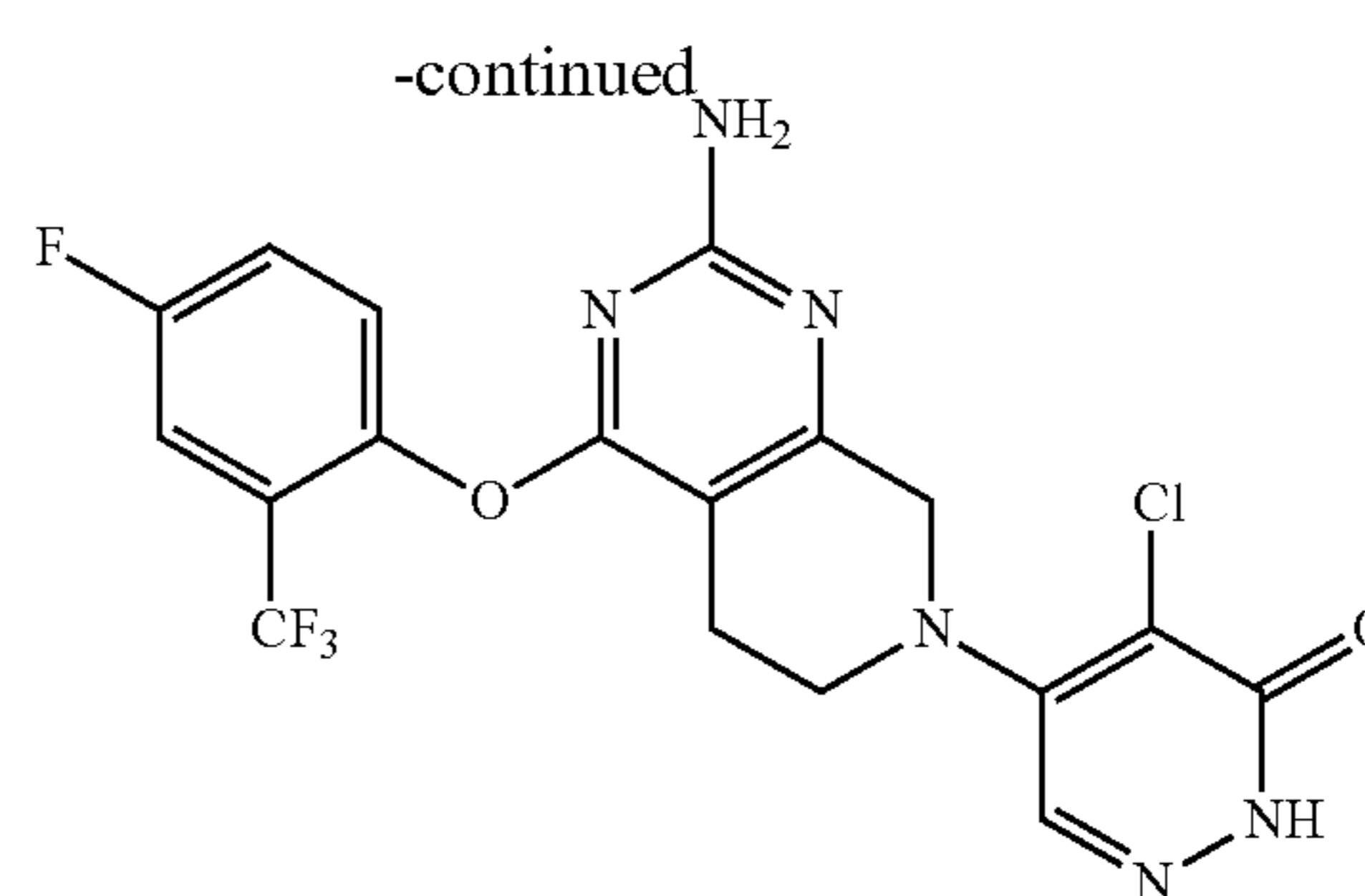
Compound 112
