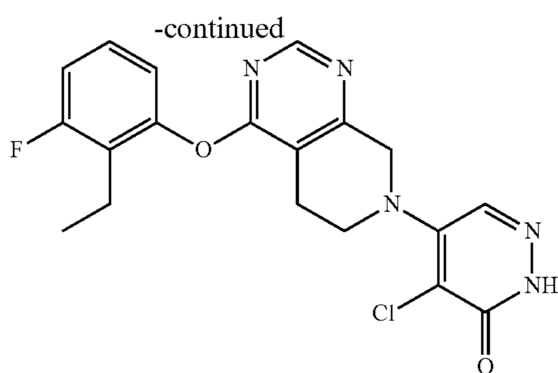
Compound 109
