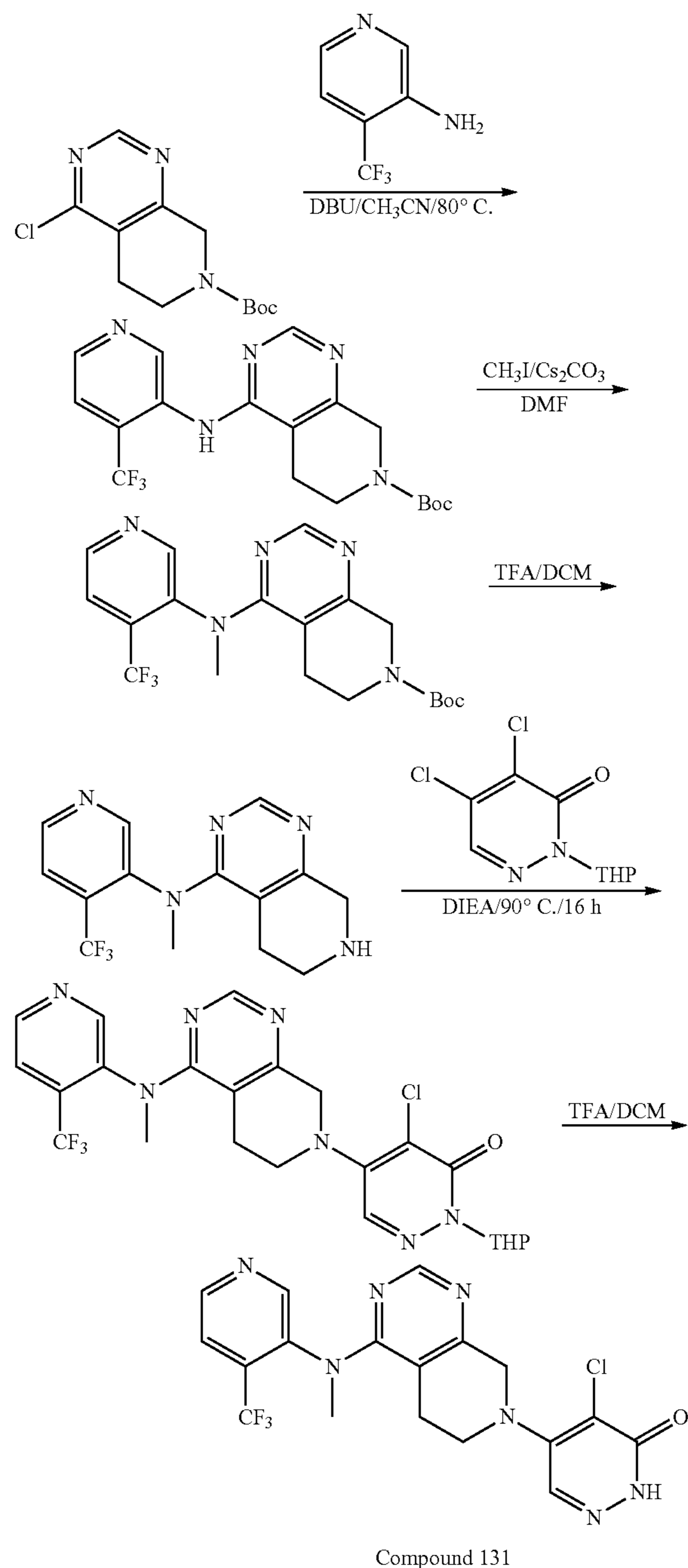
Tert-Butyl 4-[[4-(trifluoromethyl)pyridin-3-yl]amino]-5H,6H,7H,8H-pyrido[3,4-d]pyrimidine-7-carboxylate
