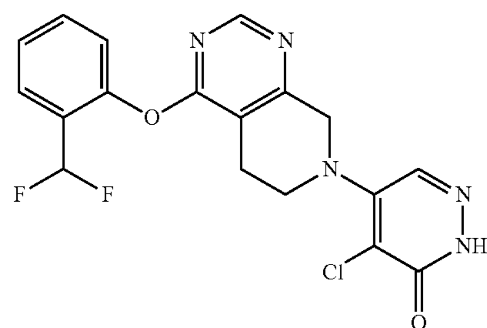
Compound 103
