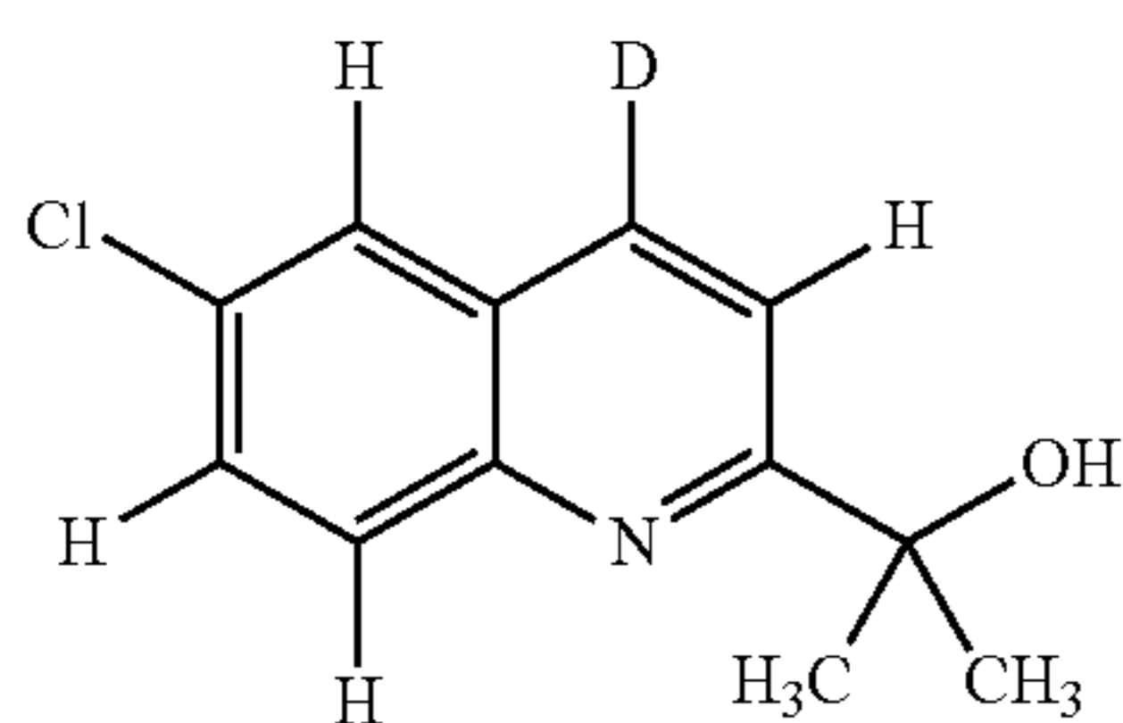
2-(6-chloroquinolin-2-yl-4-d)propan-2-ol
