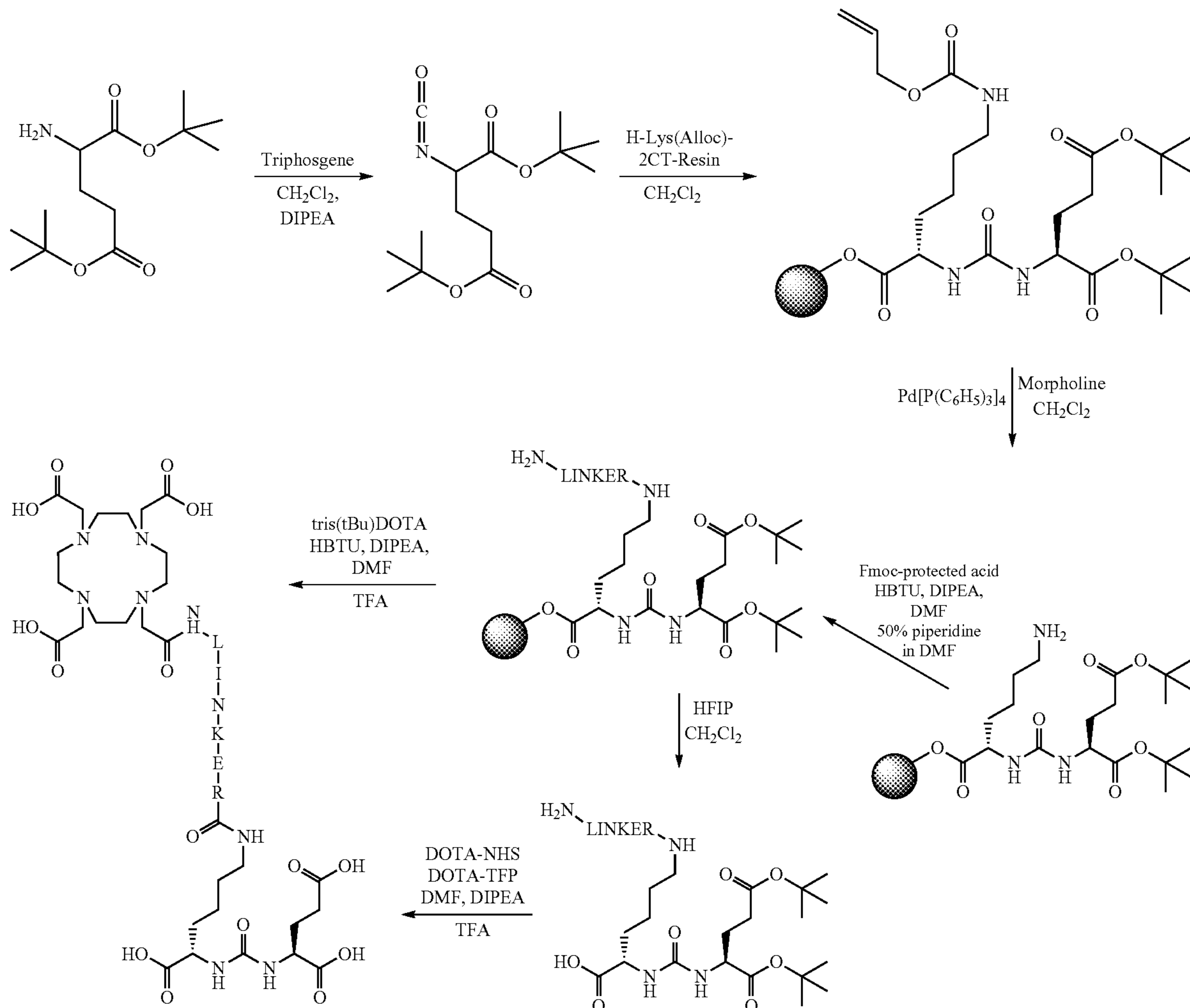
Scheme 2
