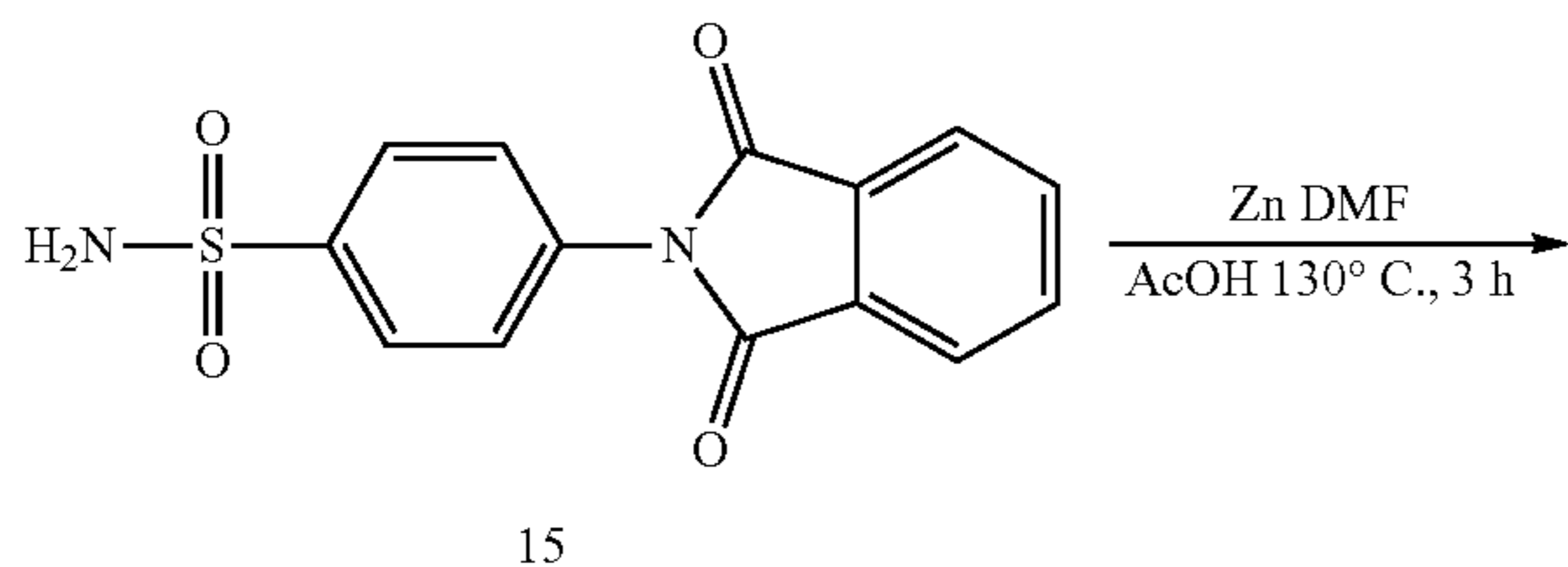
Synthetic Scheme B-2: Sample Experimental for compound #26
