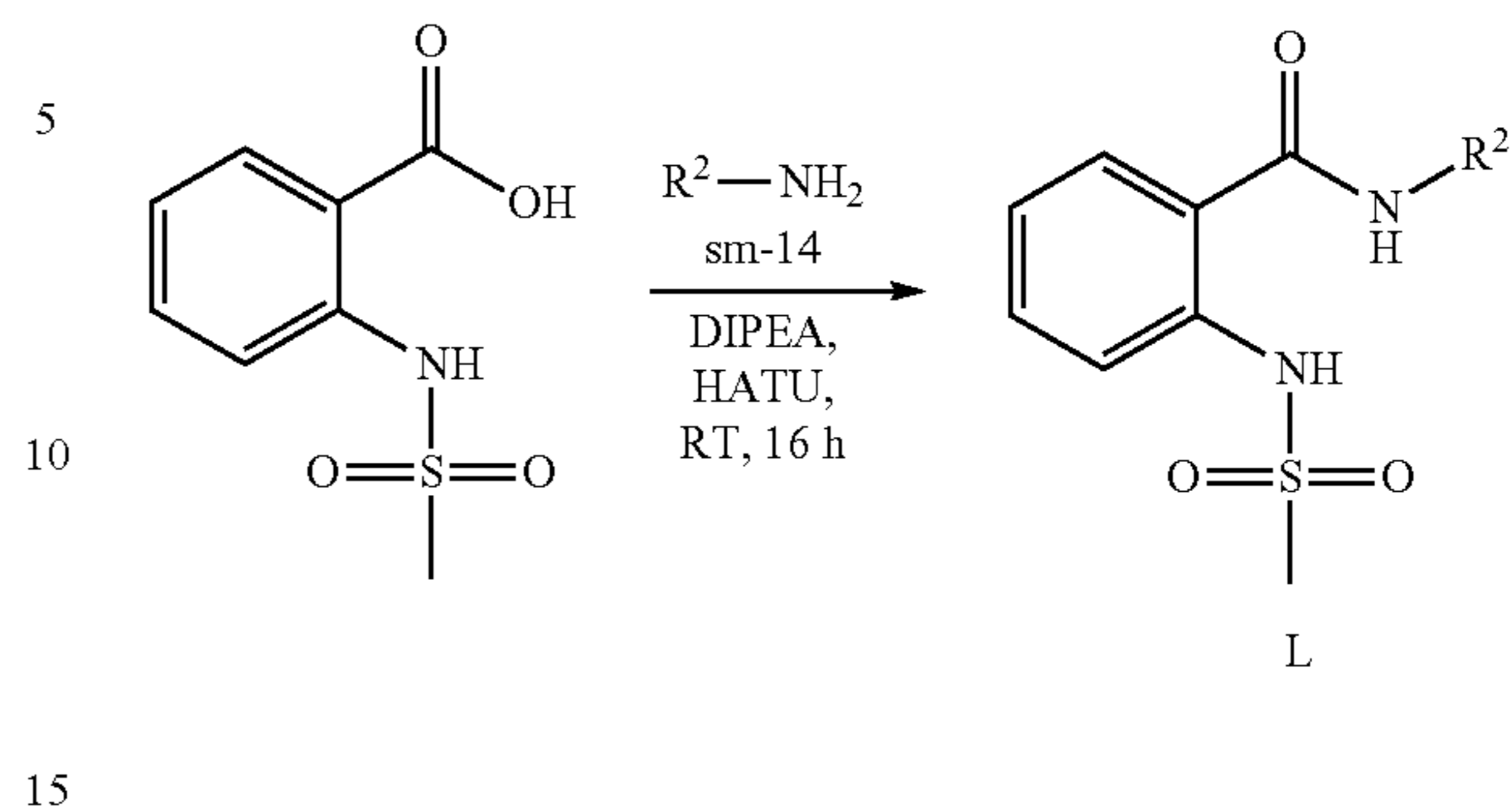
Synthetic Scheme L: General procedure for compounds L
