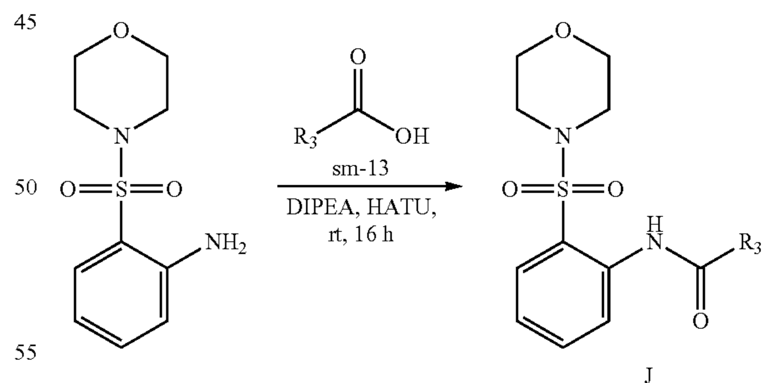
Synthetic Scheme J: General procedure for compounds J
