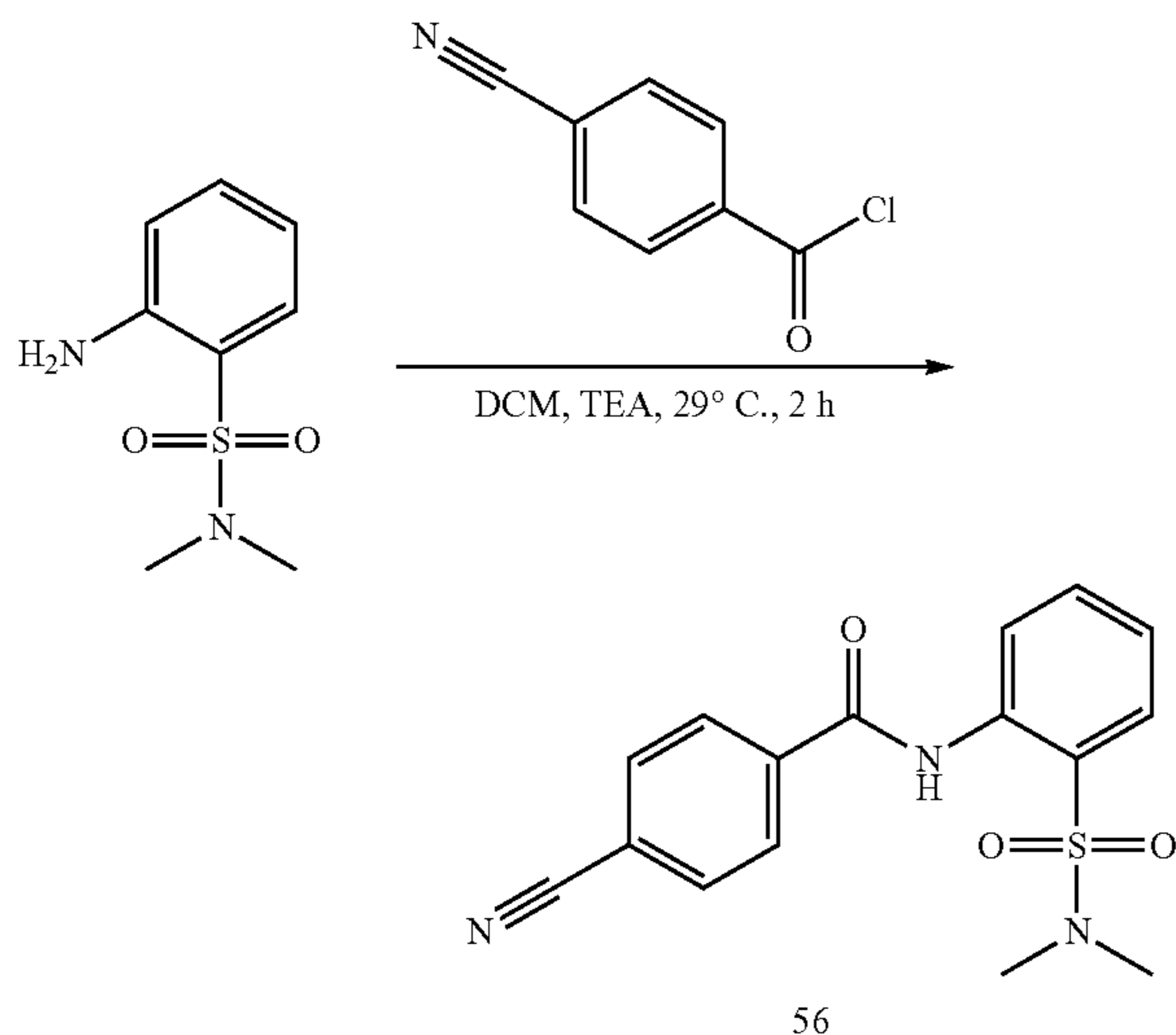
Synthetic Scheme G: Sample Experimental for compound #56
