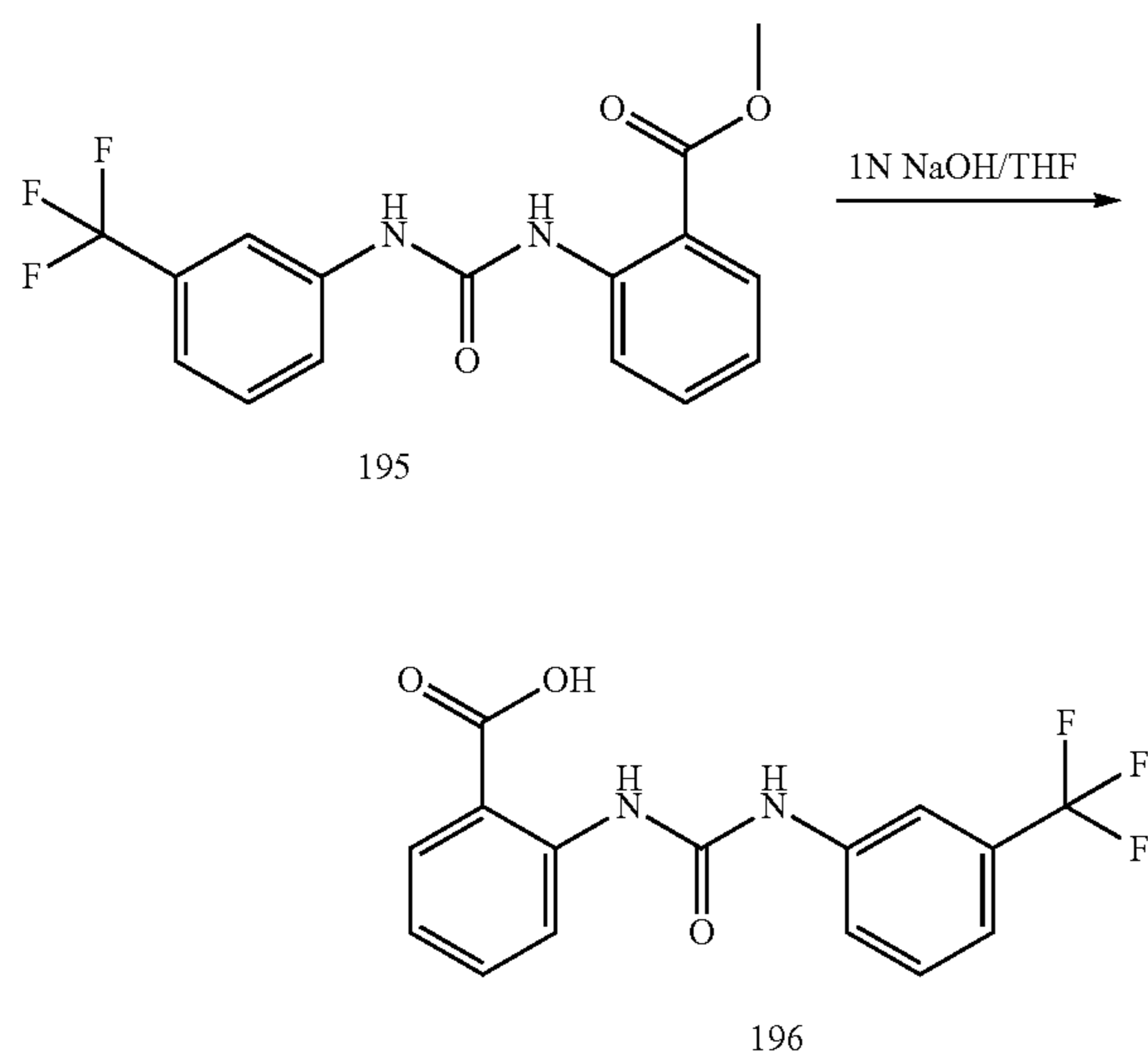
Synthetic Scheme K-2: Sample Experimental compound #196
