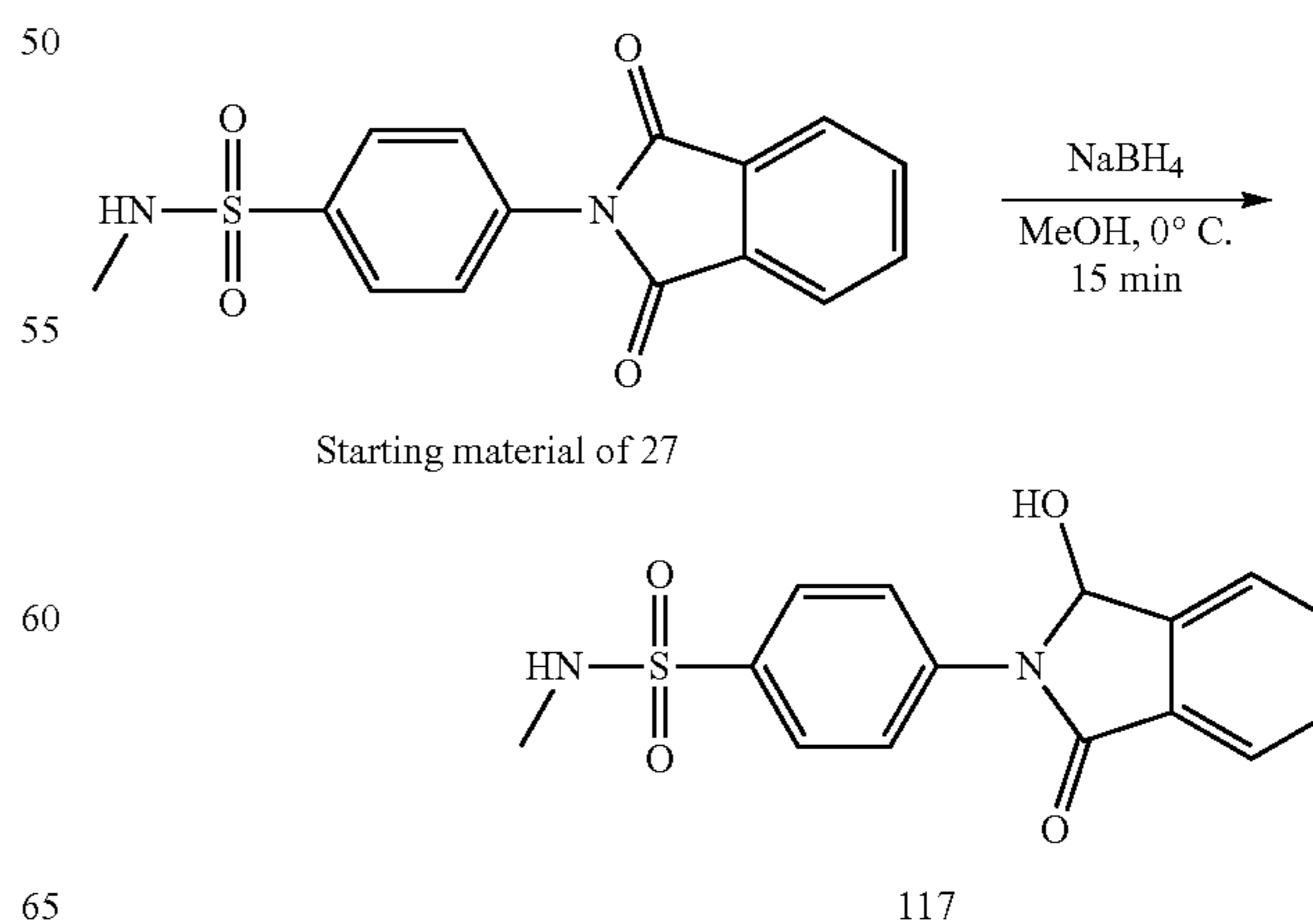
Synthetic Scheme B-3: Sample Experimental for compound #117
