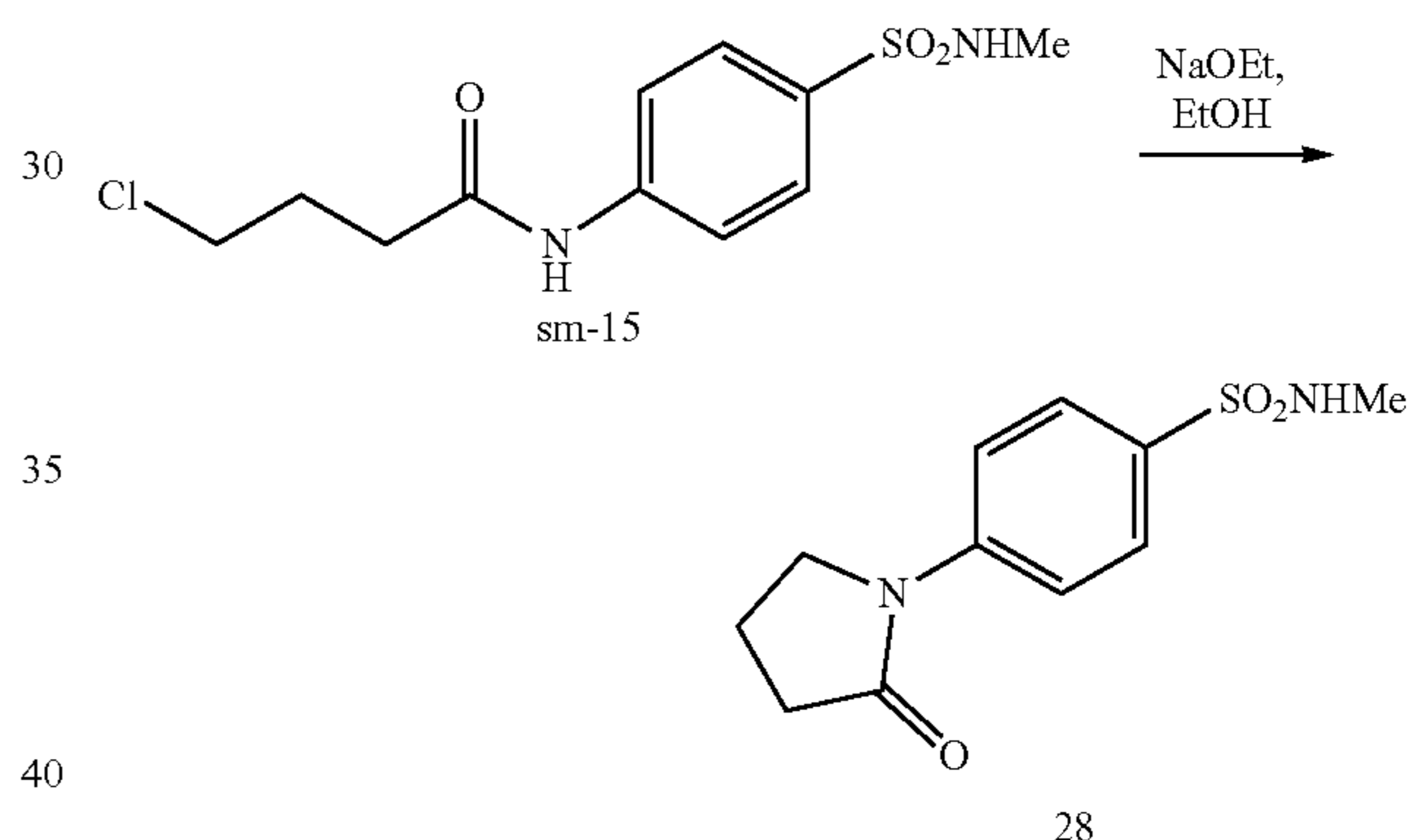
Synthetic Scheme for Compound 28
