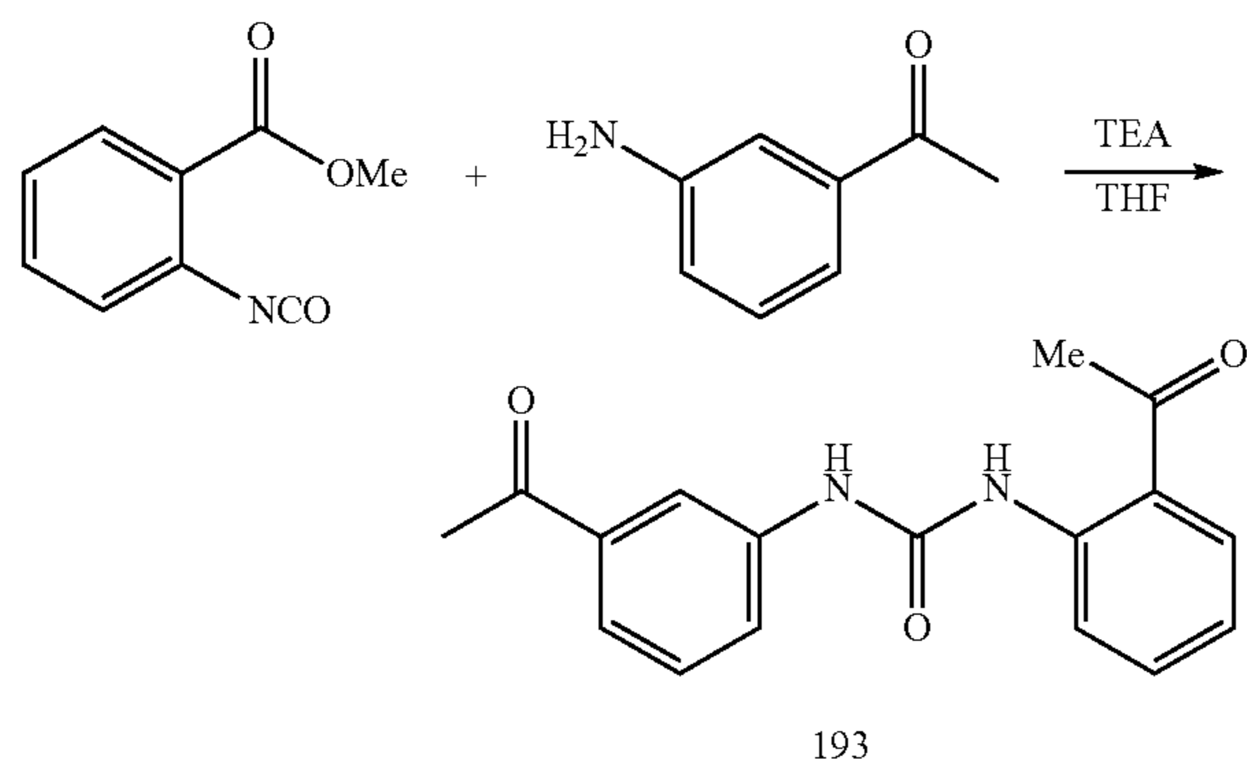
Synthetic Scheme K-1: Sample Experimental for compound #193
