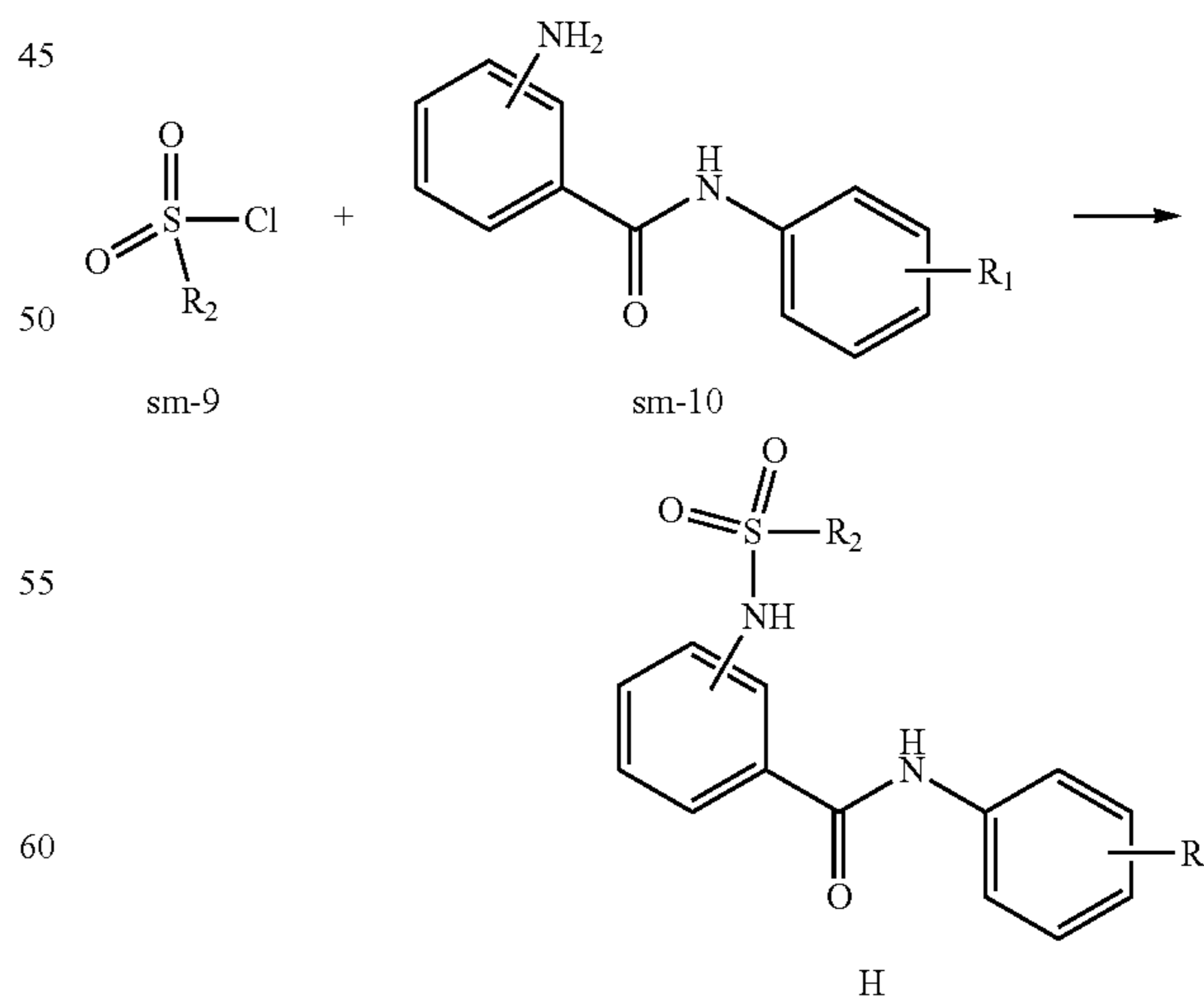
Synthetic Scheme H: General procedure for compounds H
