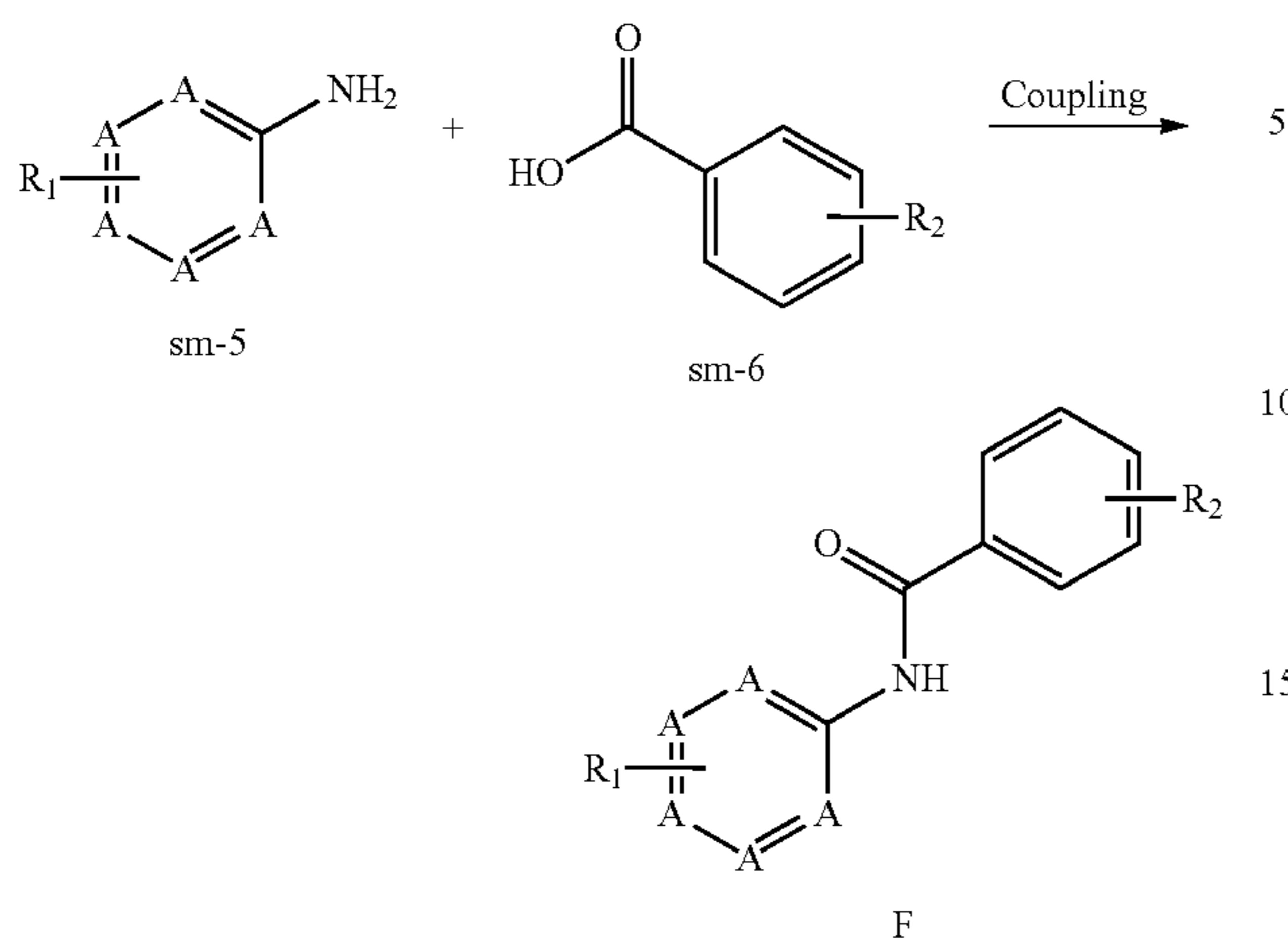
Synthetic Scheme F: General procedure for compounds F
