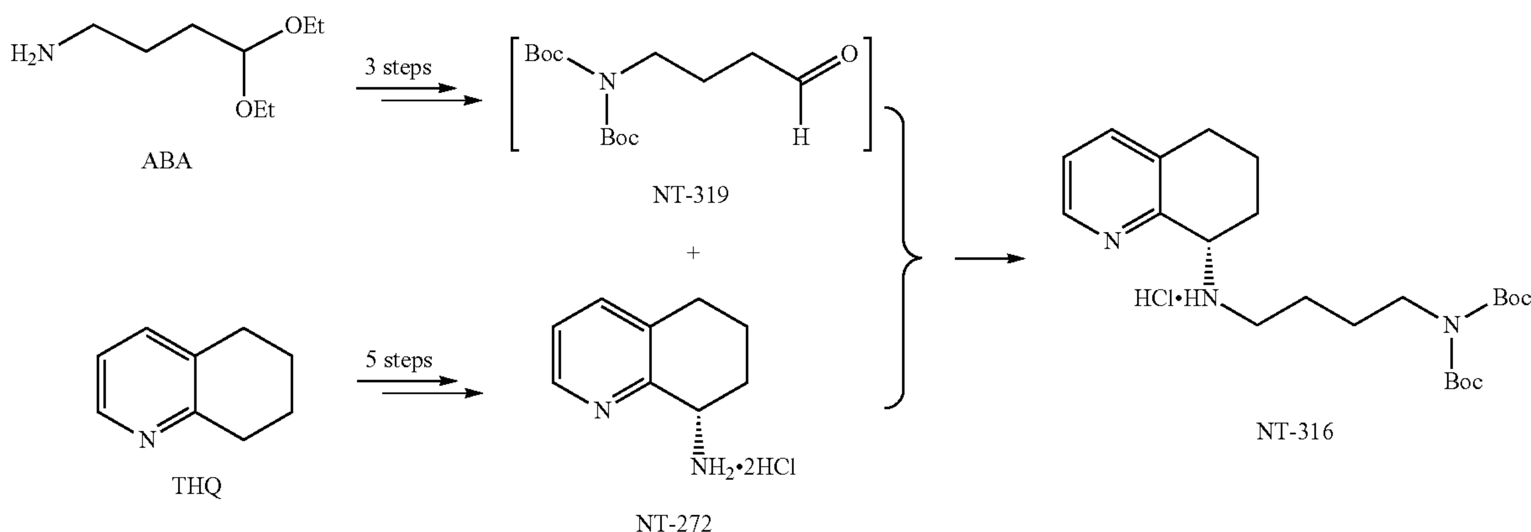
Scheme 7: Early steps in the synthesis of X4P-001.
