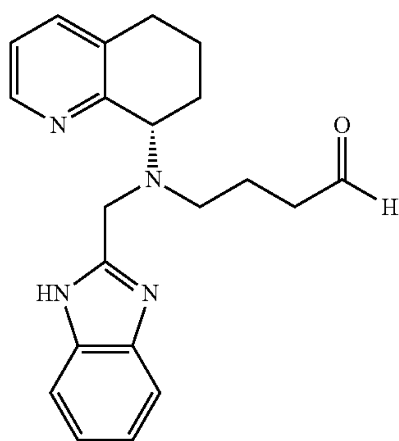
aldehyde D
