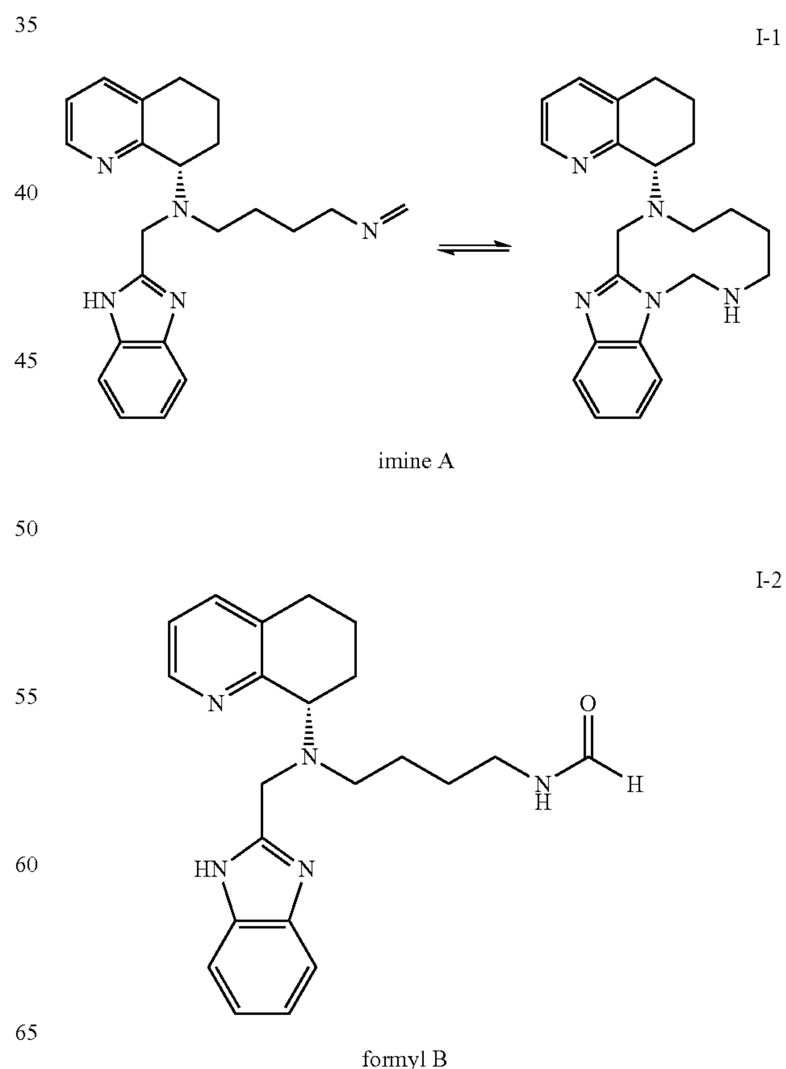
Scheme 9: Impurities Discovered in the Bulk Drug Substance
