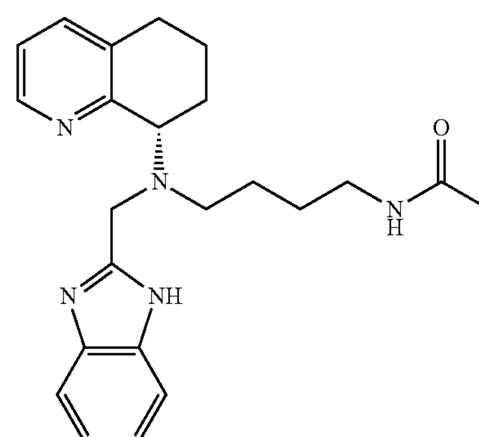
(S)-N-(4-(((1H-benzo[d]imidazol-2-yl)methyl)(5,6,7,8-tetrahydroquinolin-8-yl)amino)butyl)acetamide
