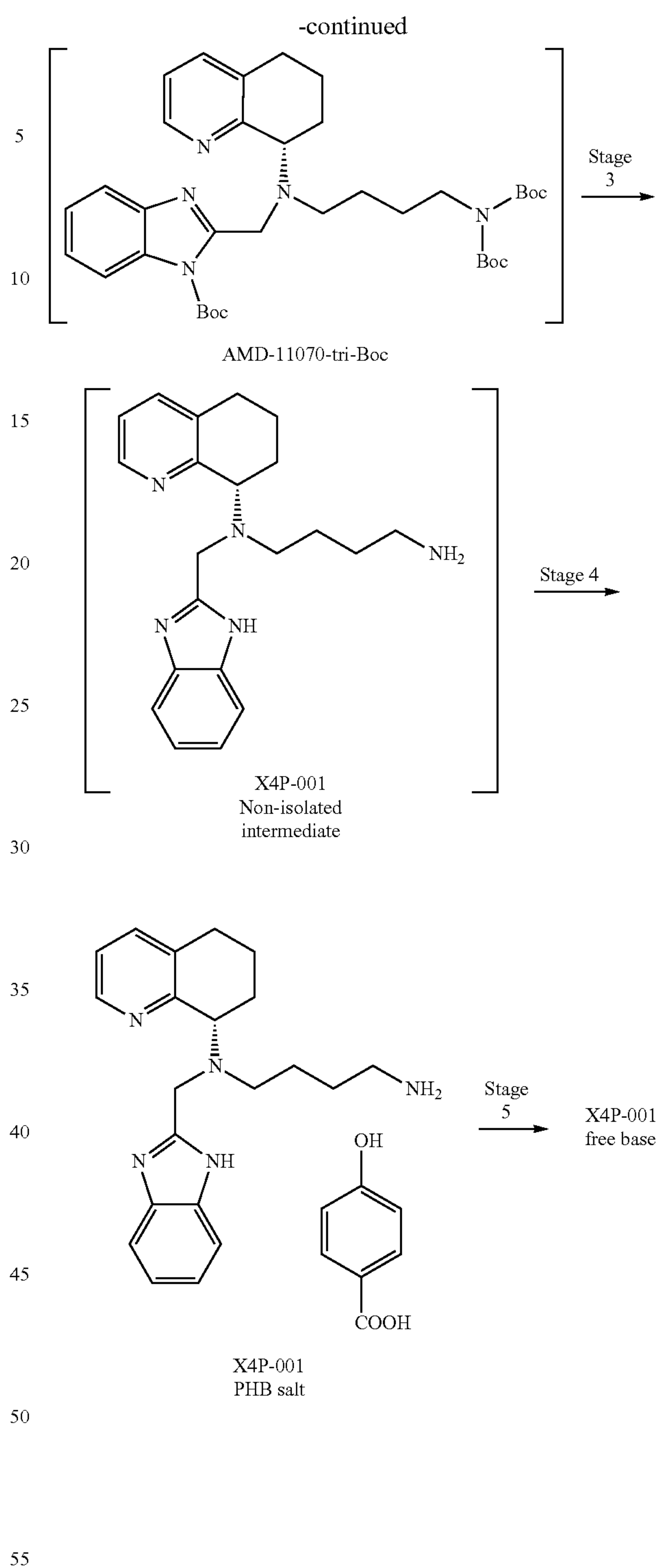
Scheme 11: Synthetic Process 3 for X4P-001.
