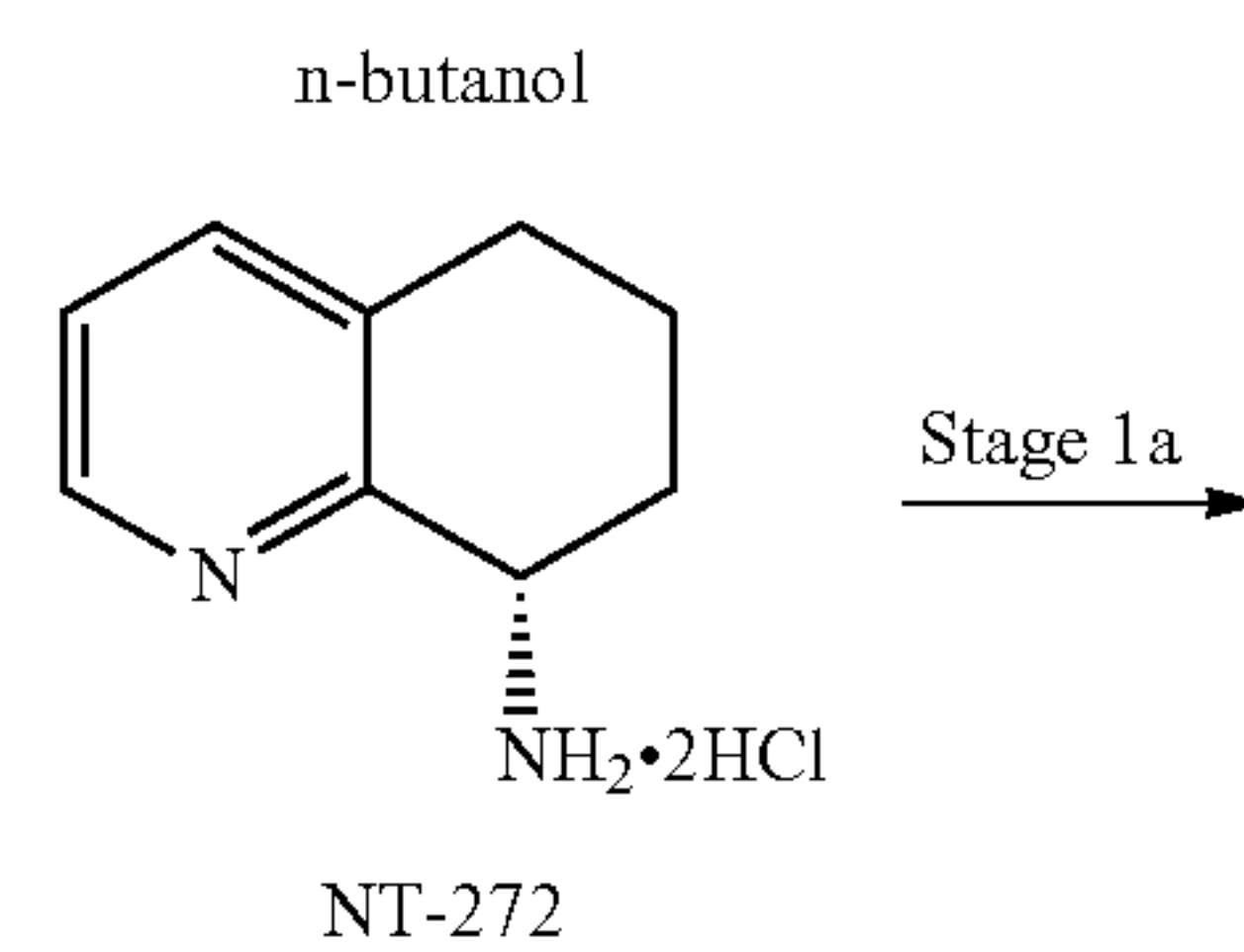
Scheme 11: Synthetic Process 3 for X4P-001.
