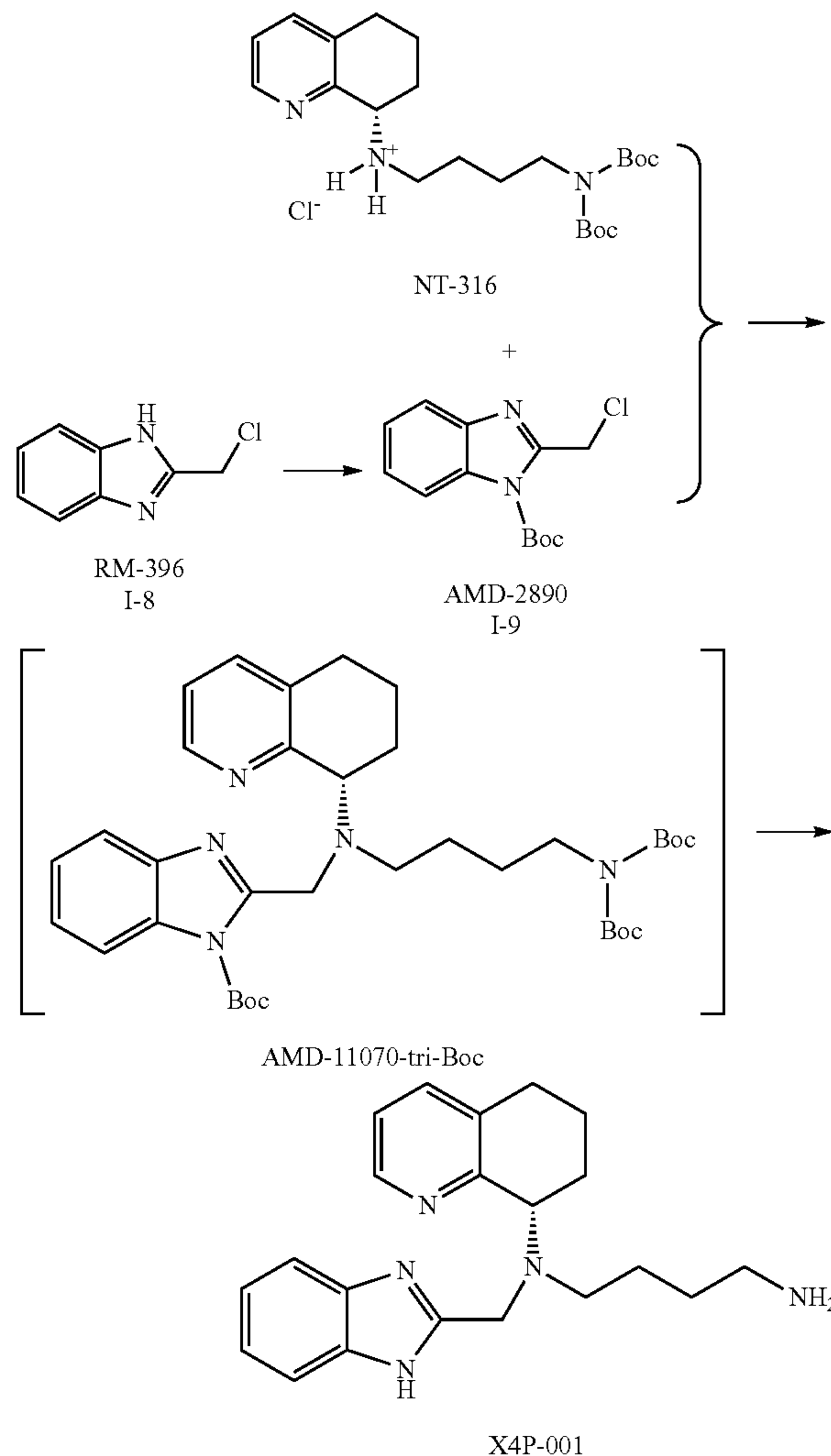
Scheme 8: Late steps in the synthesis of X4P-001.
