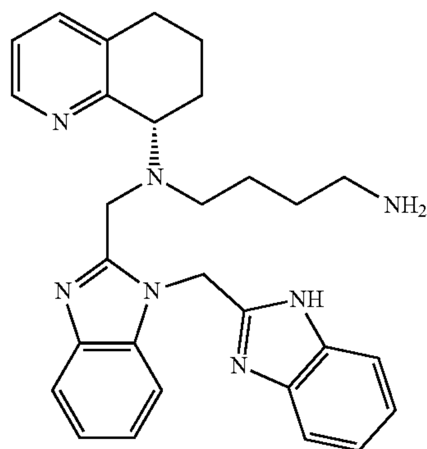
(S)-N¹-(((1H-benzo[d]imidazol-2-yl)methyl)-1H-benzo[d]imidazol-2-yl)methyl)-N¹-(5,6,7,8-tetrahydroquinolin-8-yl)butane-1,4-diamine
