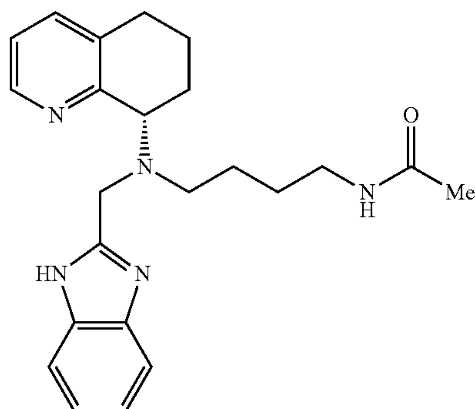
acetamide C
