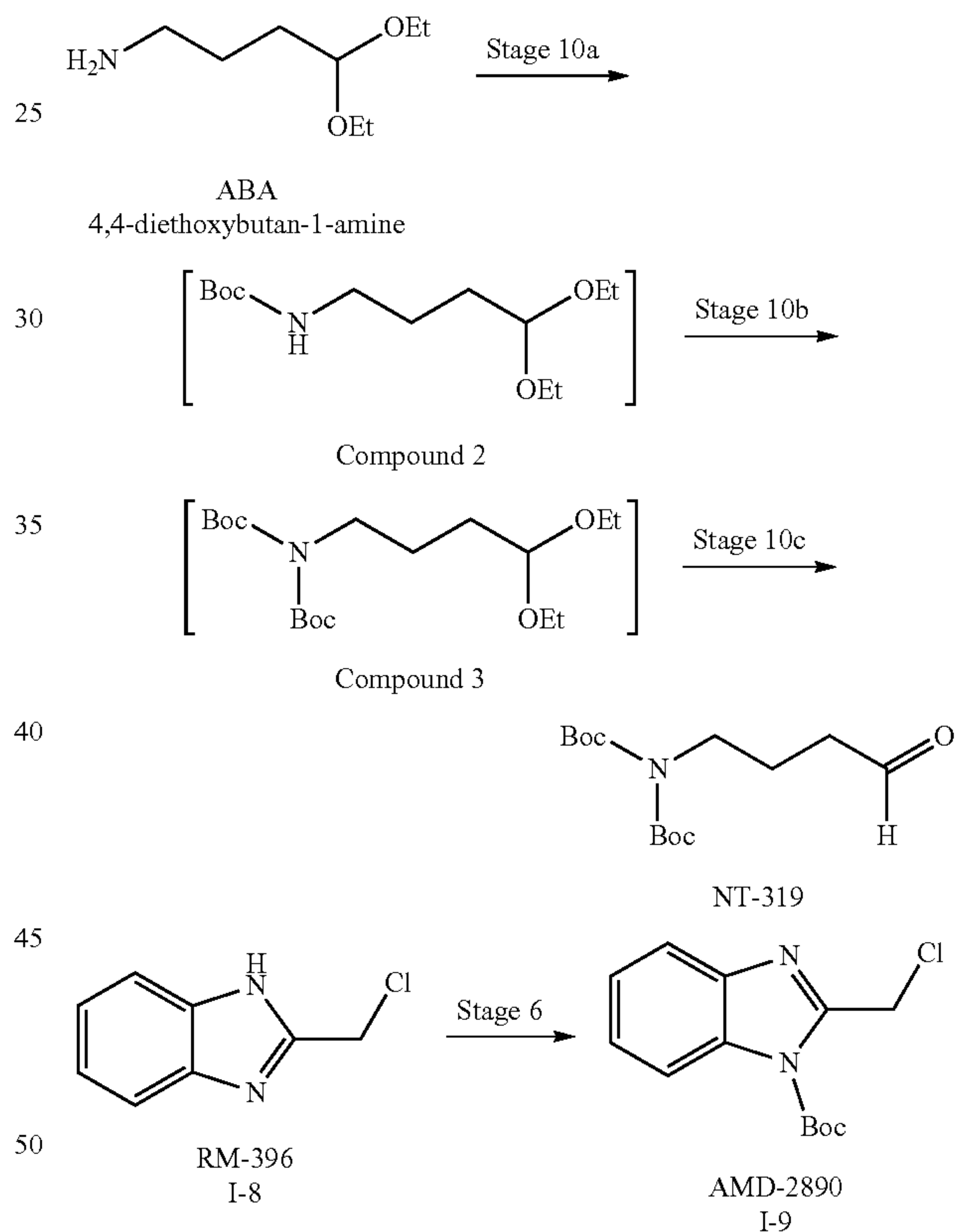
Scheme 12: Synthesis of NT-319 and AMD-2890.
