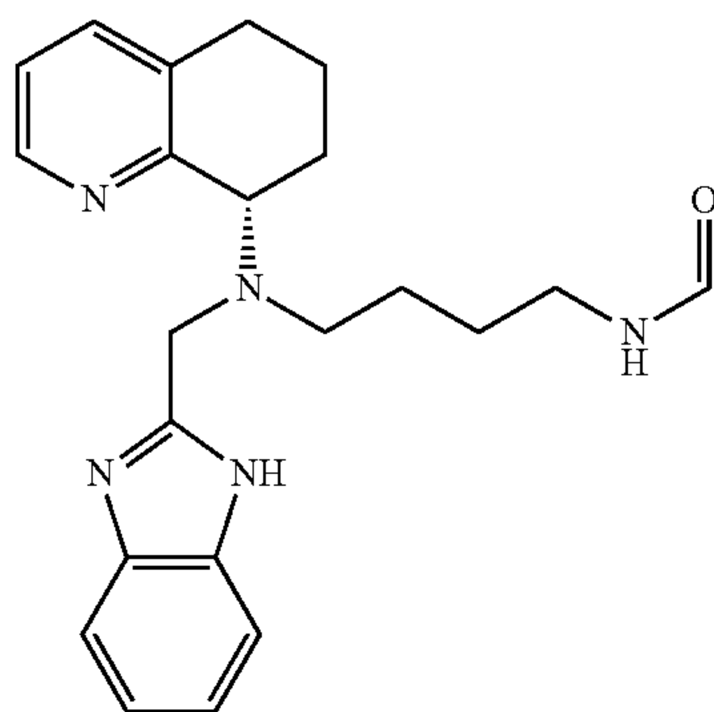
(S)-N-(4-(((1H-benzo[d]imidazol-2-yl)methyl)(5,6,7,8-tetrahydroquinolin-8-yl)amino)butyl)formamide
