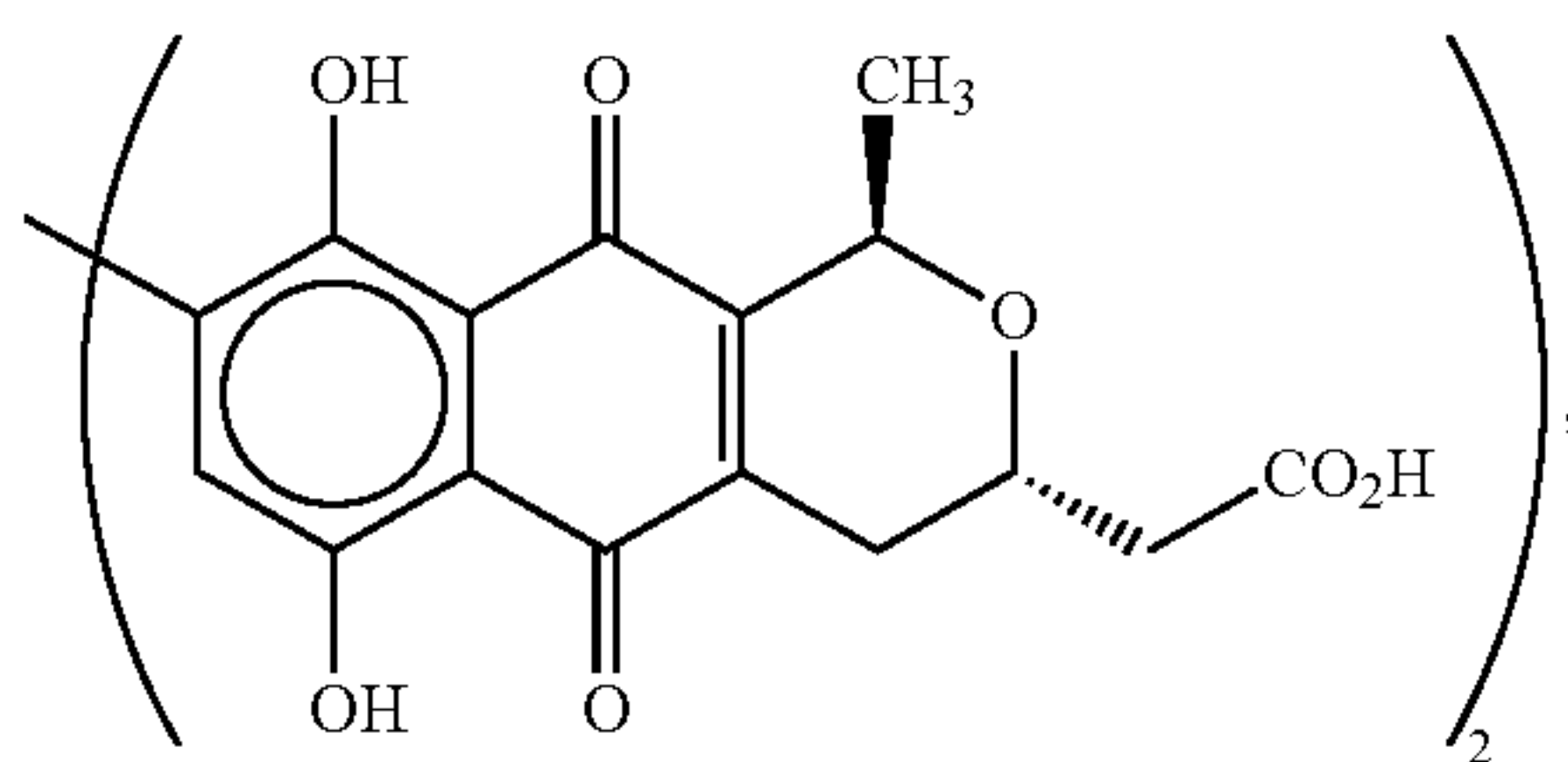
actinorhodin
