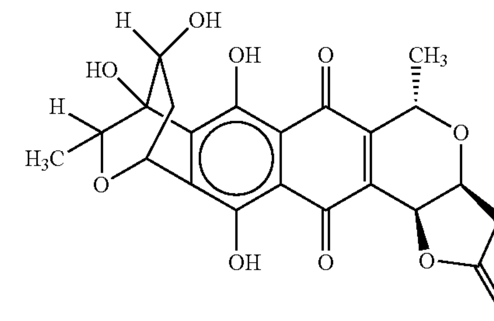
granaticin A
