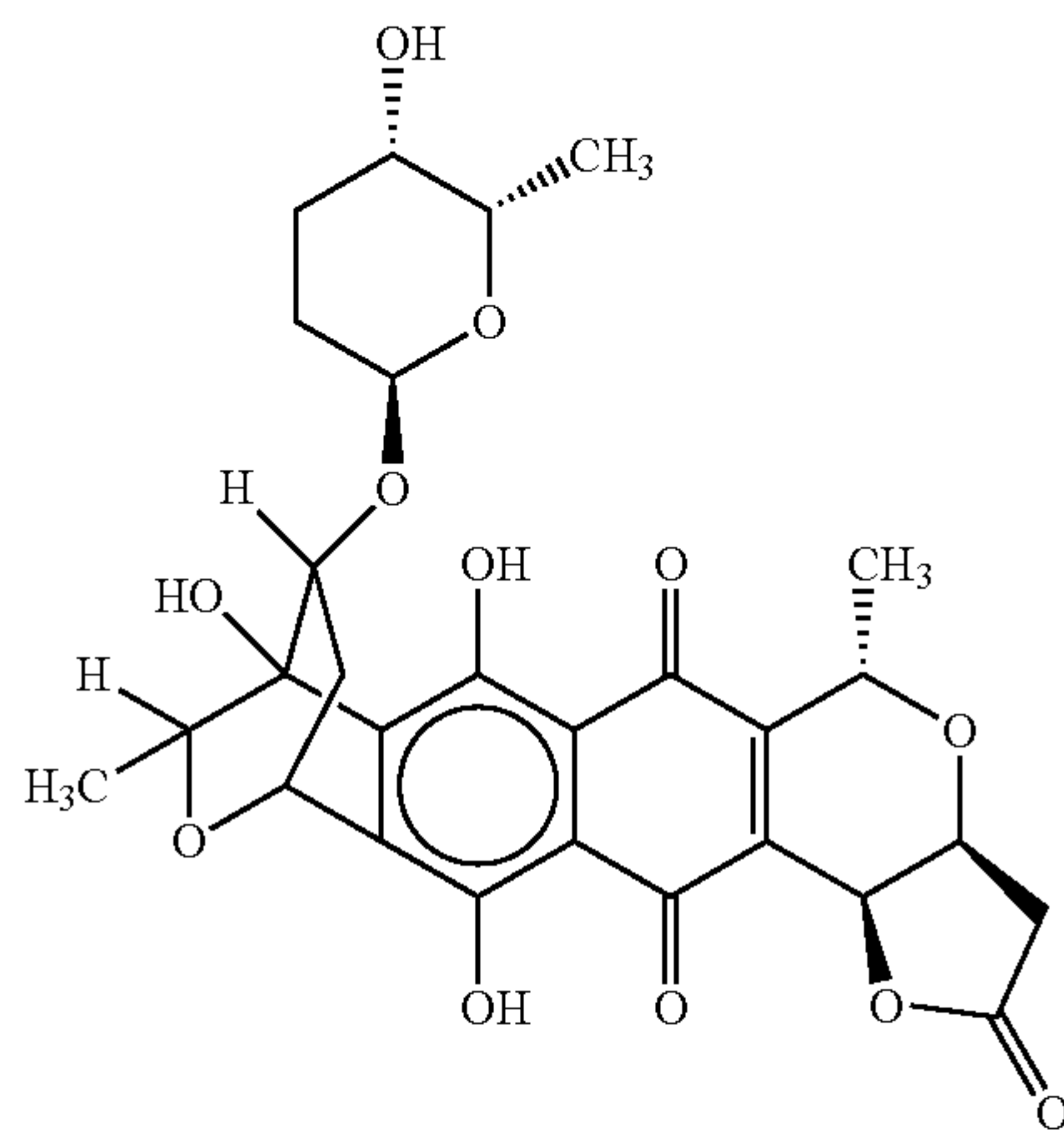
granaticin B
