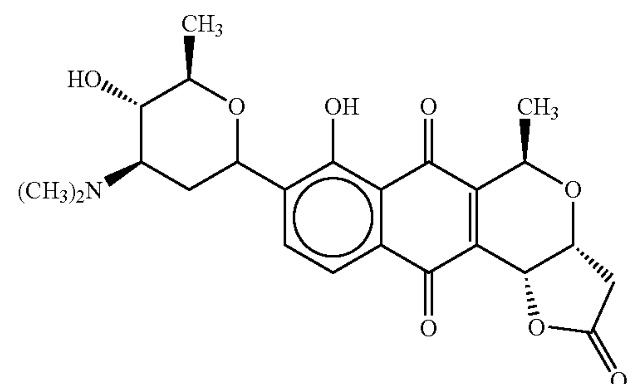
medermycin
