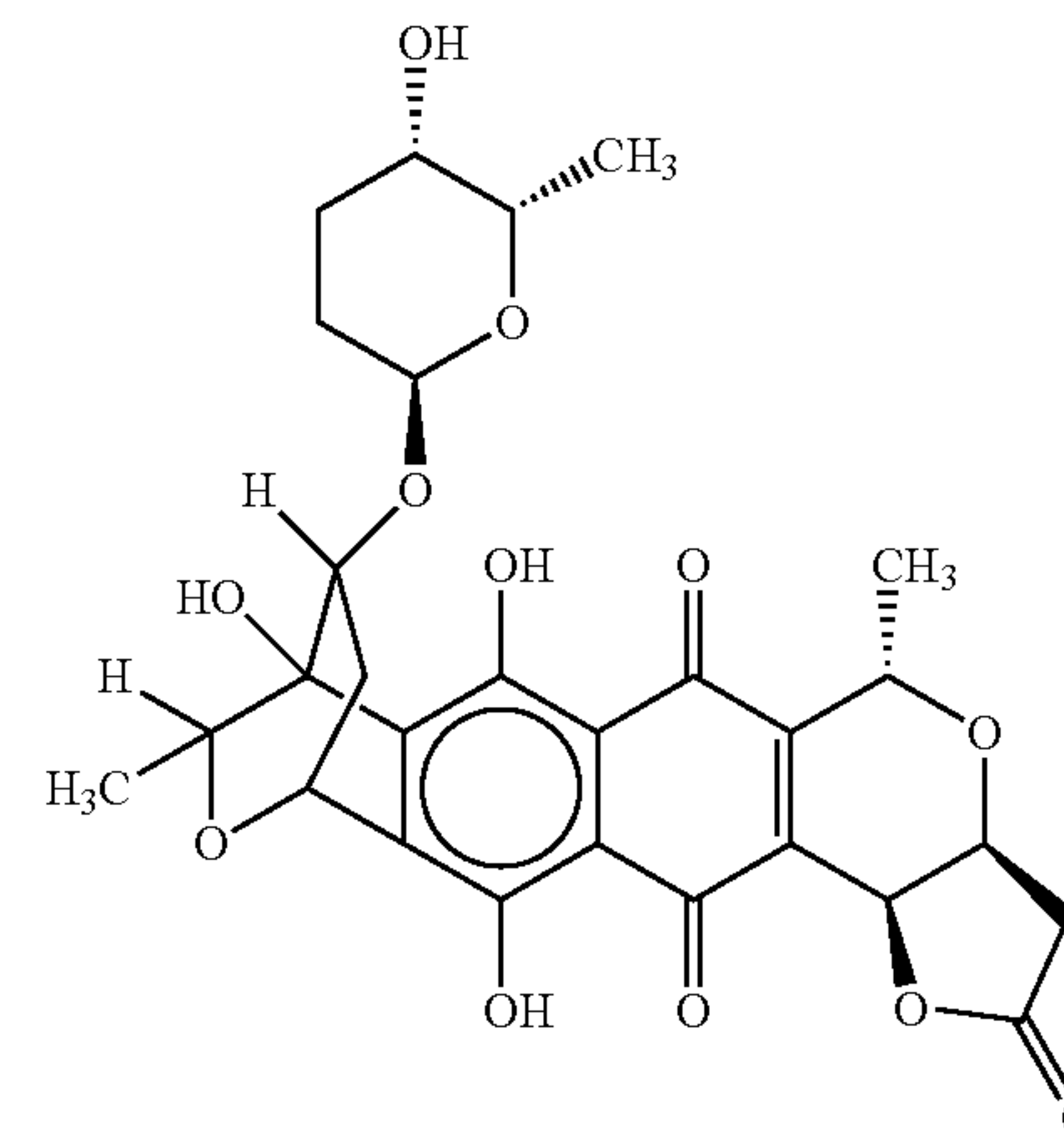
granaticin B
