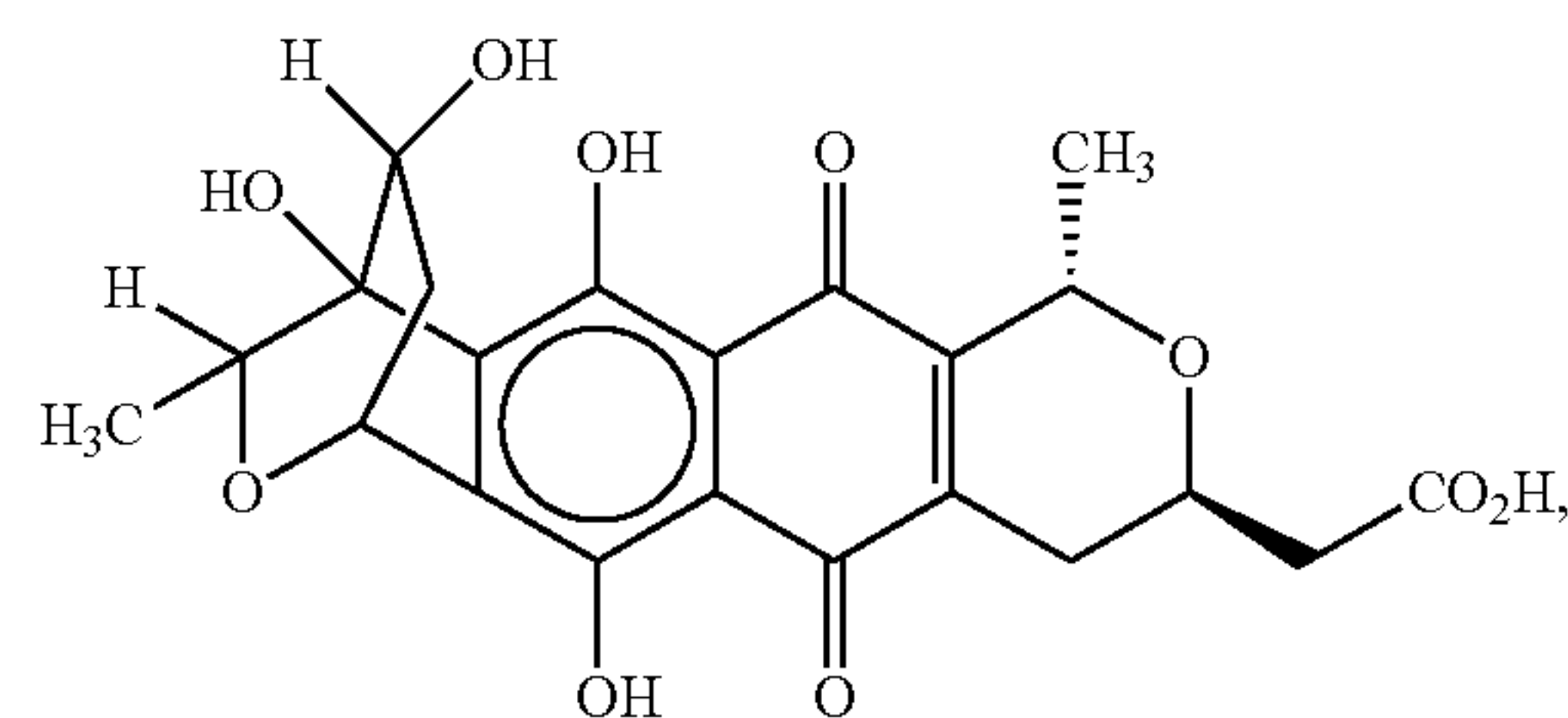
dihydrogranaticin A
